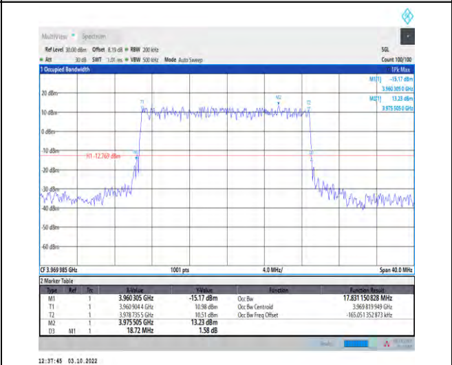
1-N77-3700-3980--30-20-H-2-DFT-PI2BPSK-Outer_Full -50@0-Ant1-17.831-18.720-<20-PASS
