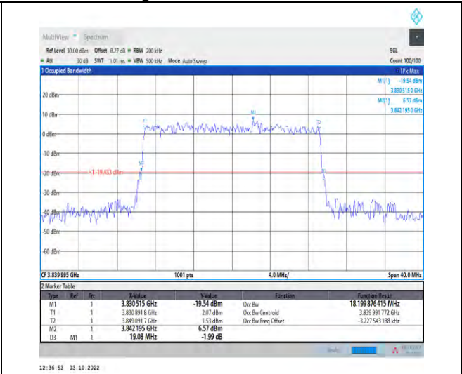
1-N77-3700-3980--30-20-M-9-CP-256QAM-Outer_Full -51@0-Ant1-18.2-19.080-<20-PASS
