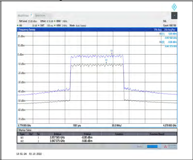
1-N77-3700-3980--30-100-H-2-CP-256QAM-Outer_ Full-273@0-Ant1-9.86-100%-0.00-9.86-PASS-≤13
