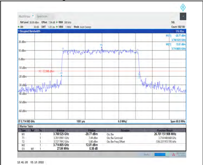
1-N77-3700-3980--30-30-L-3-DFT-16QAM-Outer_Full-75@0-Ant1-26.701-27.840-≤30-PASS
