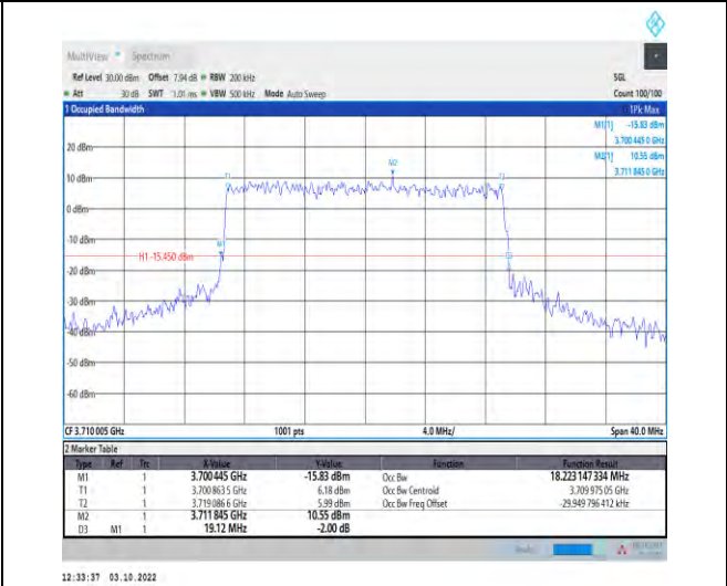
1-N77-3700-3980--30-20-L-8-CP-64QAM-Outer_Full-51@0-Ant1-18.223-19.120-<=20-PASS
