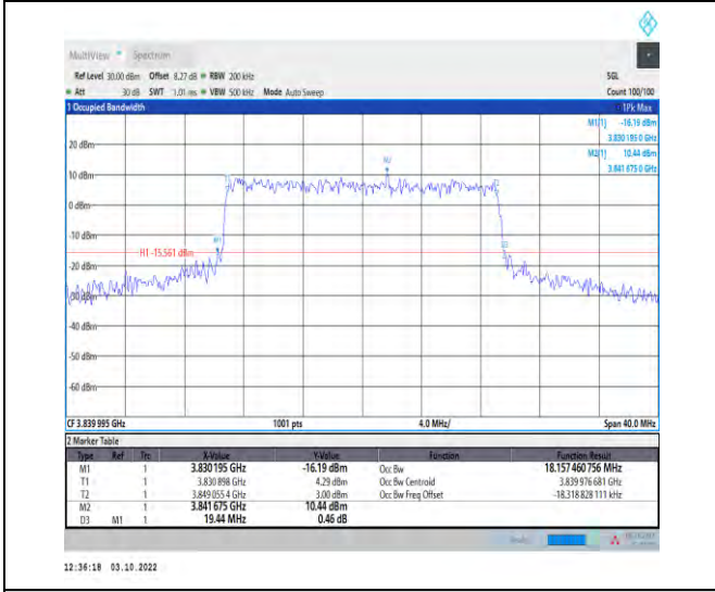
1-N77-3700-3980--30-20-M-6-CP-QPSK-Outer_Full-51@0-Ant1-18.157-19.440-<=20-PASS
