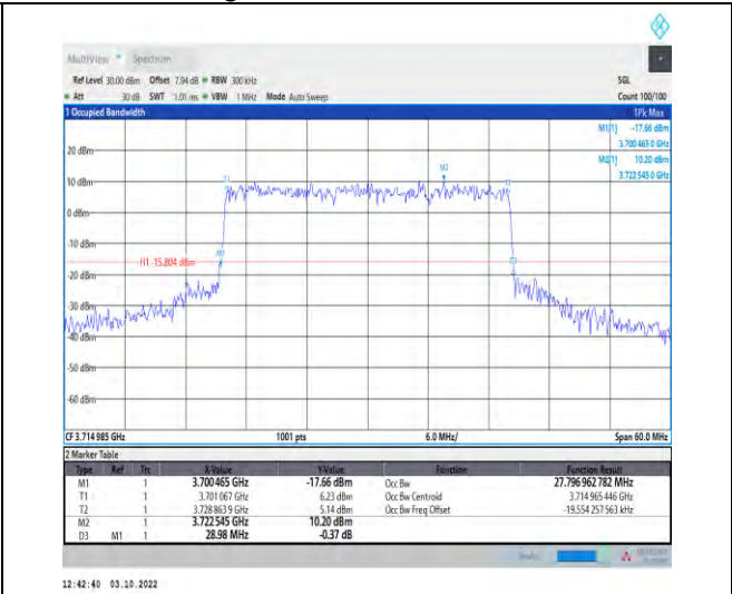
1-N77-3700-3980--30-30-L-7-CP-16QAM-Outer_Full -78@0-Ant1-27.797-28.980-<math>\leq</math>30-PASS
