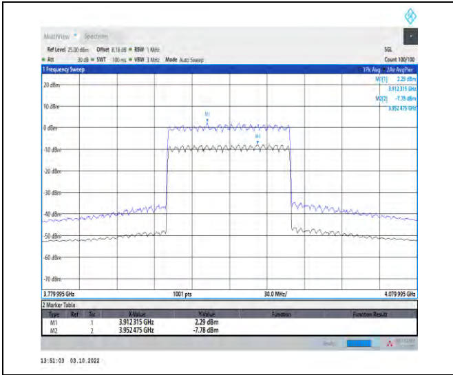
1-N77-3700-3980--30-100-H-1-DFT-256QAM-Outer_ Full-270@0-Ant1-10.07-100%-0.00-10.07-PASS-≤13
