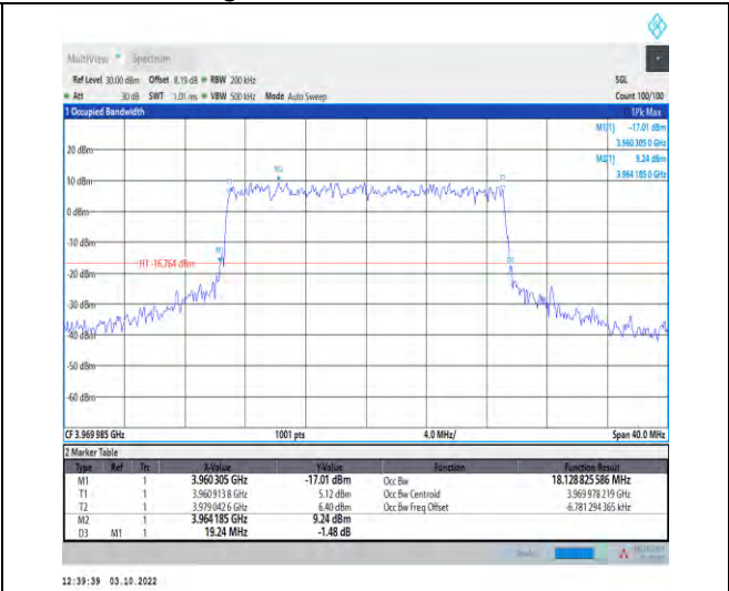
1-N77-3700-3980--30-20-H-8-CP-64QAM-Outer_Full -51@0-Ant1-18.129-19.240-≤20-PASS
