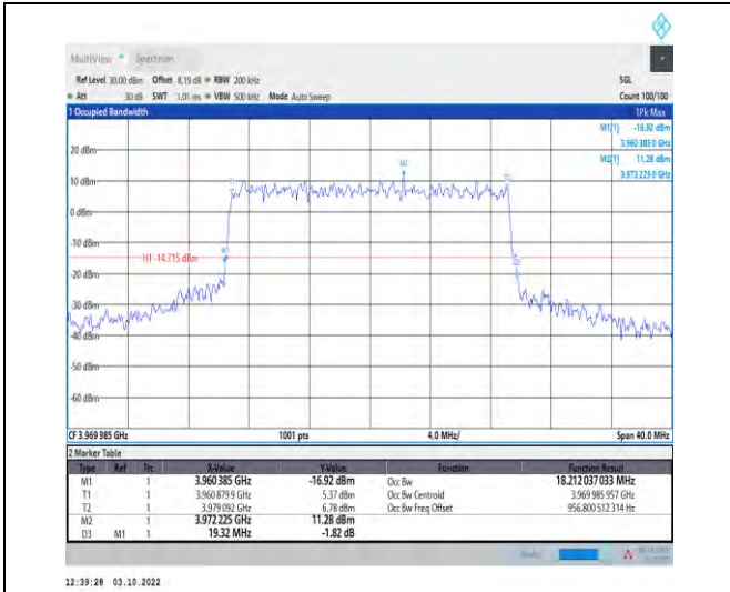
1-N77-3700-3980--30-20-H-7-CP-16QAM-Outer_Full -51@0-Ant1-18.212-19.320-≤20-PASS
