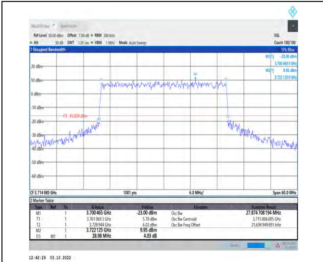
1-N77-3700-3980--30-30-L-6-CP-QPSK-Outer_Full-7 8@0-Ant1-27.875-28.980-<math>\leq</math>30-PASS
