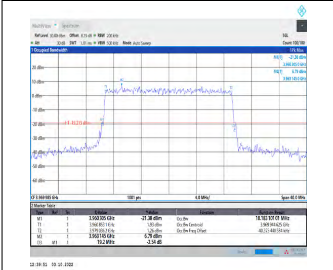
1-N77-3700-3980--30-20-H-9-CP-256QAM-Outer_Fu II-51@0-Ant1-18.183-19.200-≤20-PASS
