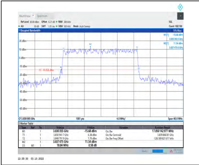
1-N77-3700-3980--30-20-M-4-DFT-64QAM-Outer_Fu II-50@0-Ant1-17.85-18.840-<=20-PASS
