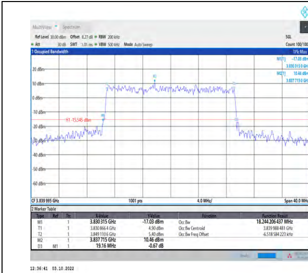
1-N77-3700-3980--30-20-M-8-CP-64QAM-Outer_Full -51@0-Ant1-18.244-19.160-<20-PASS
