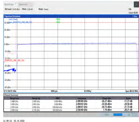
1-N41--30-80-L-3-DFT-PI2BPSK-Outer_Full-216@0-Ant1-1--PASS-see graph
