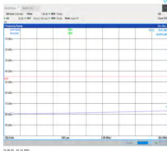
1-N41--30-100-M-1-DFT-PI2BPSK-Inner_1RB_Left-1 @1-0.15-30-Ant1-29.97--76.67--45-PASS
