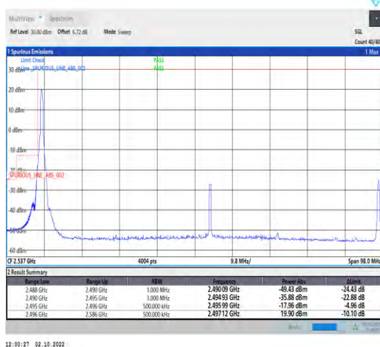
1-N41--30-90-L-4-CP-QPSK-Edge_1RB_Left-1@0-Ant1-1--PASS-see graph
