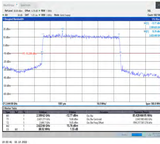
1-N41--30-90-H-2-DFT-PI2BPSK-Outer_Full-240@0-A Ant1-85.428-88.920-≤90-PASS
