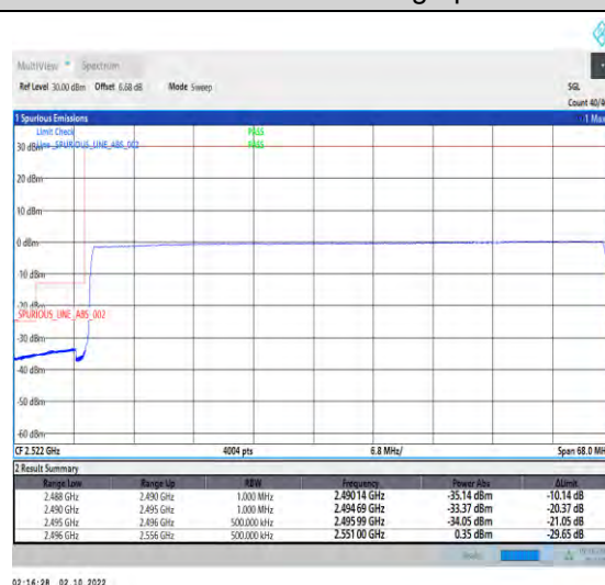
1-N41--30-60-L-6-CP-QPSK-Outer_Full-162@0-Ant1-1--PASS-see graph
