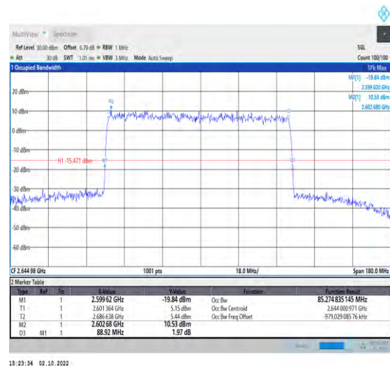
1-N41--30-90-H-5-DFT-256QAM-Outer_Full-240@0-A Ant1-85.275-88.920-≤90-PASS
