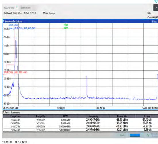
1-N41--30-100-L-4-CP-QPSK-Edge_1RB_Left-1@0-Ant1-1--PASS-see graph
