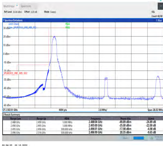
1-N41--30-20-L-4-CP-QPSK-Edge_1RB_Left-1@0-Ant1-1--PASS-see graph
