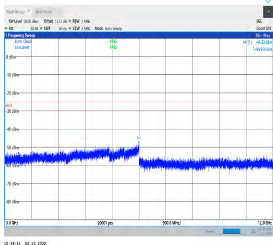
1-N41--30-100-L-1-DFT-PI2BPSK-Inner_1RB_Left-1 @1-3000-12000-Ant1-7496.85--48.33--25-PASS
