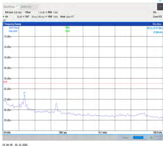
1-N41--30-100-L-1-DFT-PI2BPSK-Inner_1RB_Left-1 @1-0.009-0.15-Ant1-0.03--67.57--55-PASS
