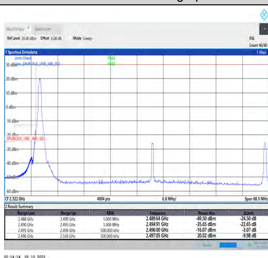
1-N41--30-60-L-4-CP-QPSK-Edge_1RB_Left-1@0-Ant1-1--PASS-see graph
