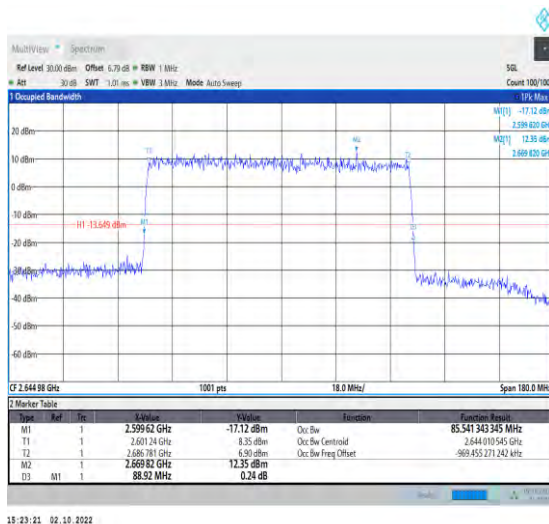
1-N41--30-90-H-4-DFT-64QAM-Outer_Full-240@0-A nt1-85.541-88.920-≤90-PASS
