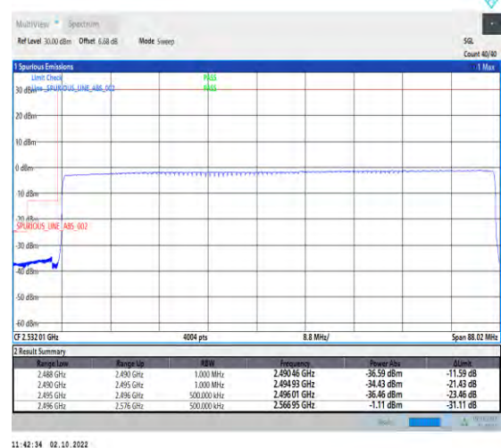
1-N41--30-80-L-6-CP-QPSK-Outer_Full-217@0-Ant1-1--PASS-see graph
