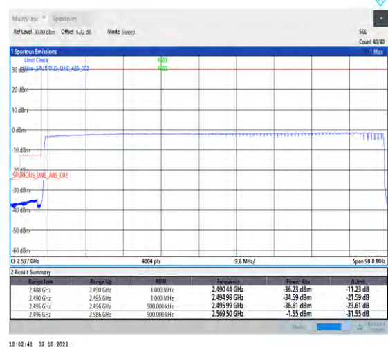
1-N41--30-90-L-6-CP-QPSK-Outer_Full-245@0-Ant1-1--PASS-see graph
