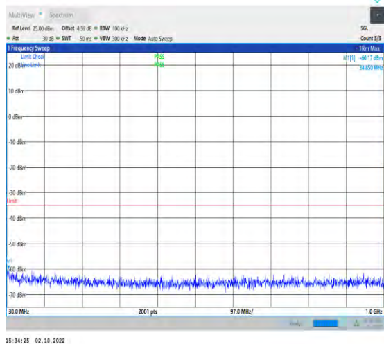
1-N41--30-100-L-1-DFT-PI2BPSK-Inner_1RB_Left-1 @1-30-1000-Ant1-34.85--60.17--35-PASS
