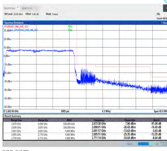
1-N41--30-20-H-6-CP-QPSK-Outer_Full-51@0-Ant1-1--PASS-see graph
