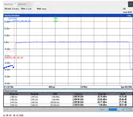
1-N41--30-90-L-3-DFT-PI2BPSK-Outer_Full-240@0-Ant1-1--PASS-see graph
