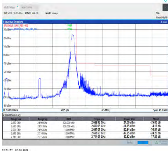
1-N41--30-20-H-2-DFT-PI2BPSK-Edge_1RB_Right-1@50-Ant1-1--PASS-see graph
