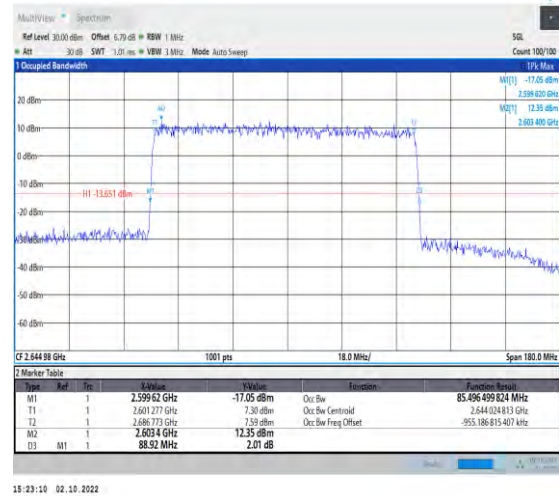
1-N41--30-90-H-3-DFT-16QAM-Outer_Full-240@0-A nt1-85.496-88.920-≤90-PASS
