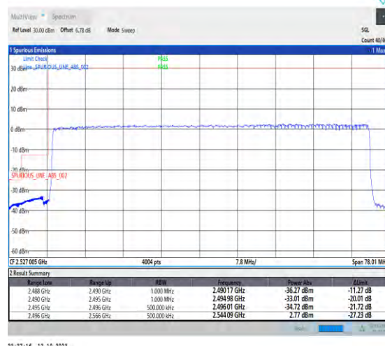
1-N41--30-70-L-3-DFT-PI2BPSK-Outer_Full-180@0-Ant1-1--PASS-see graph
