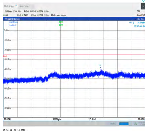
1-N41--30-100-L-1-DFT-PI2BPSK-Inner_1RB_Left-1 @1-12000-27000-Ant1-22207.00--39.59--25-PASS
