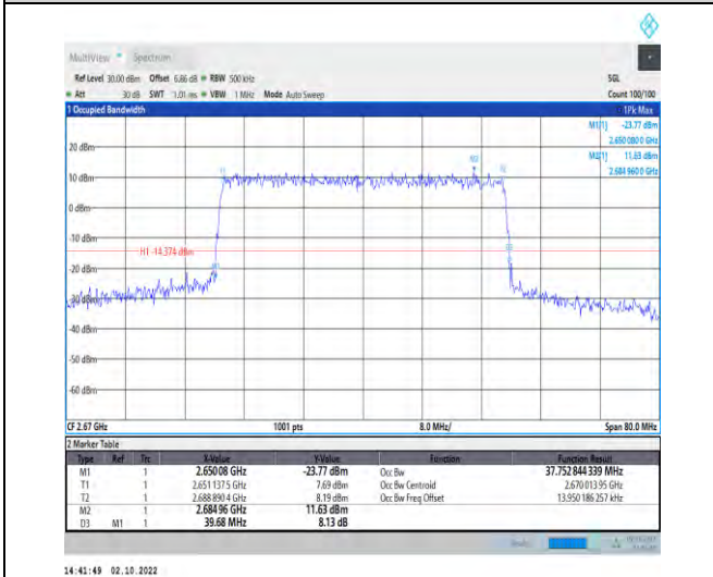
1-N41--30-40-H-7-CP-16QAM-Outer_Full-106@0-An t1-37.753-39.680-<math>\leq 40</math>-PASS
