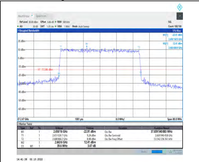
1-N41--30-40-H-6-CP-QPSK-Outer_Full-106@0-Ant 1-37.84-39.600-<math>\leq 40</math>-PASS
