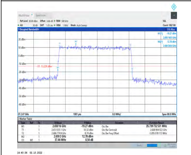
1-N41--30-40-H-3-DFT-16QAM-Outer_Full-100@0-A nt1-35.74-37.440-<math>\leq 40</math>-PASS
