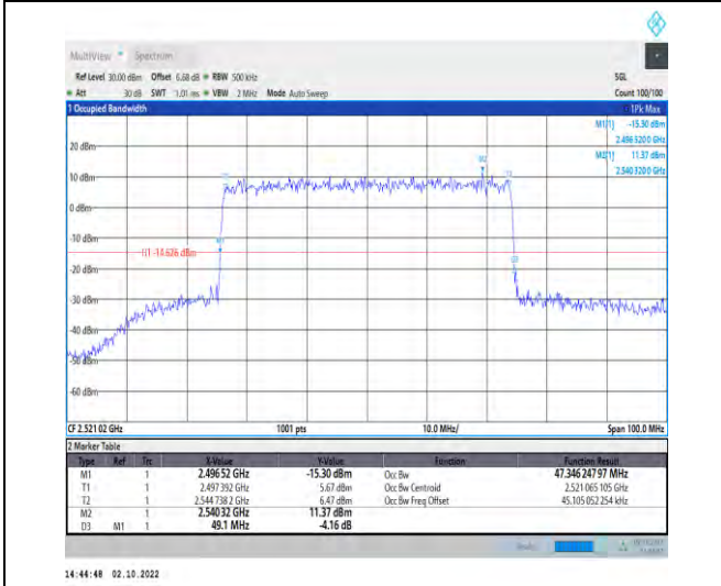
1-N41--30-50-L-6-CP-QPSK-Outer_Full-133@0-Ant1 -47.346-49.100- \leq 50 -PASS
