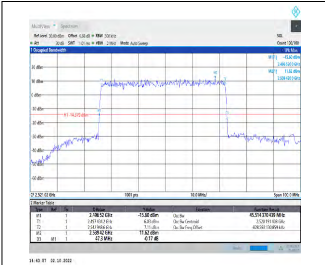
1-N41--30-50-L-4-DFT-64QAM-Outer_Full-128@0-A nt1-45.514-47.300- \leq 50 -PASS
