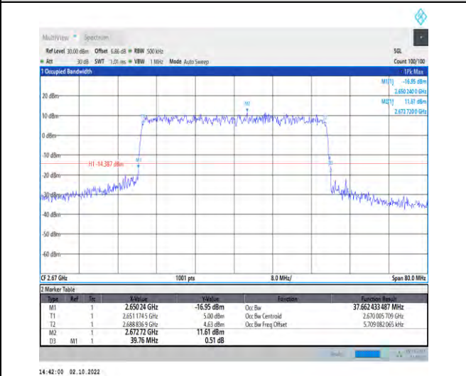
1-N41--30-40-H-8-CP-64QAM-Outer_Full-106@0-An t1-37.662-39.760-<math>\leq 40</math>-PASS
