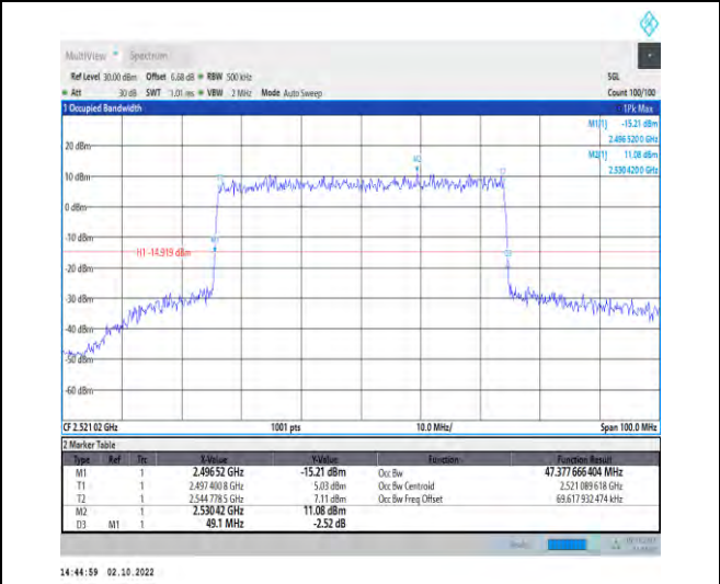
1-N41--30-50-L-7-CP-16QAM-Outer_Full-133@0-Ant1 t1-47.378-49.100- \leq 50 -PASS
