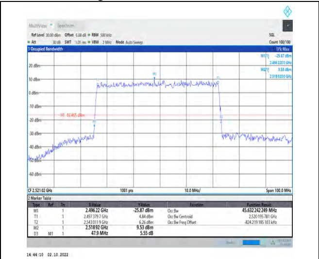
1-N41--30-50-L-5-DFT-256QAM-Outer_Full-128@0-A nt1-45.632-47.900- \leq 50 -PASS
