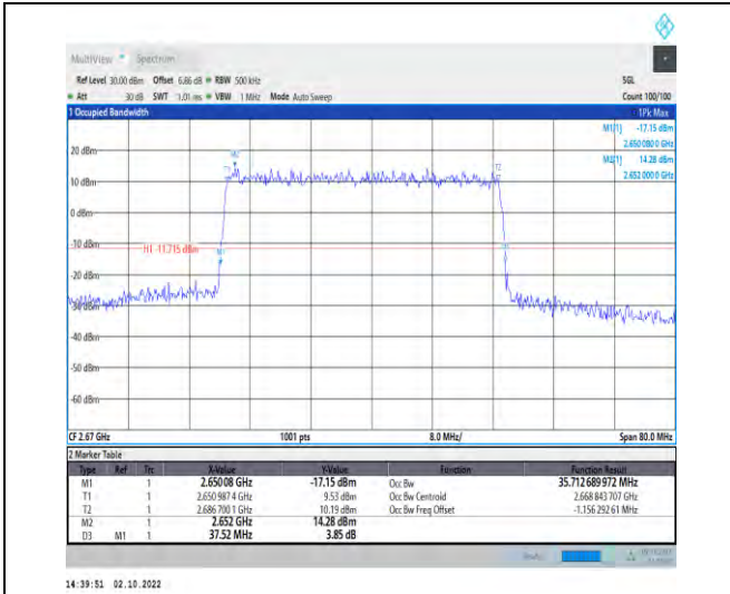
1-N41--30-40-H-1-DFT-QPSK-Outer_Full-100@0-An t1-35.713-37.520-<math>\leq 40</math>-PASS
