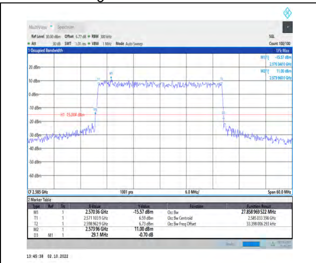
1-N38--30-30-L-7-CP-16QAM-Outer_Full-78@0-Ant1-1.27.859-29.100-<=30-PASS
