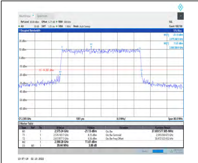
1-N38--30-40-M-6-CP-QPSK-Outer_Full-106@0-Ant 1-37.694-39.440-≤40-PASS
