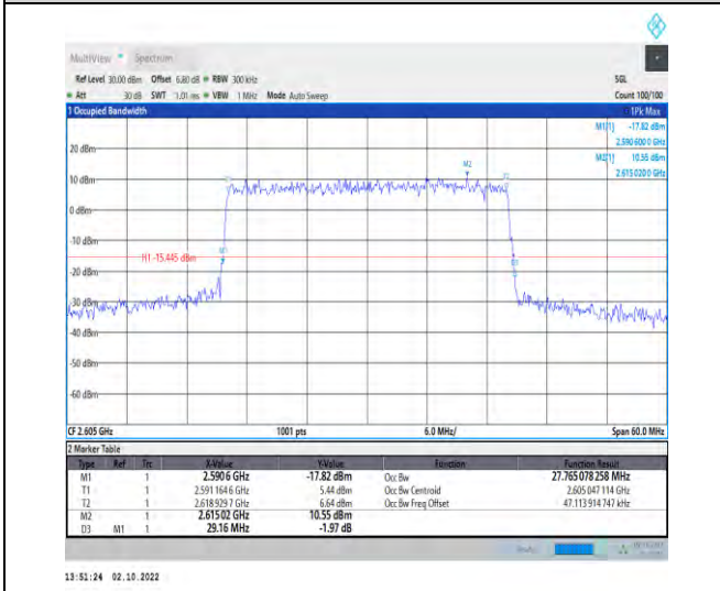
1-N38--30-30-H-6-CP-QPSK-Outer_Full-78@0-Ant1- 27.765-29.160-<30-PASS
