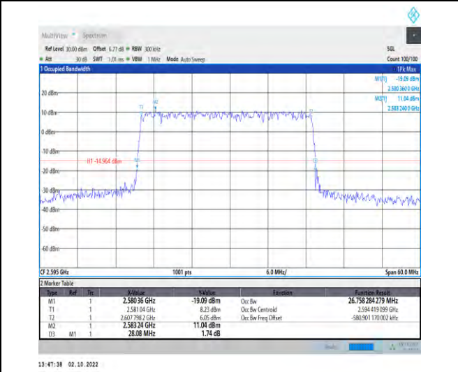
1-N38--30-30-M-4-DFT-64QAM-Outer_Full-75@0-Ant 1-26.758-28.080-≤30-PASS
