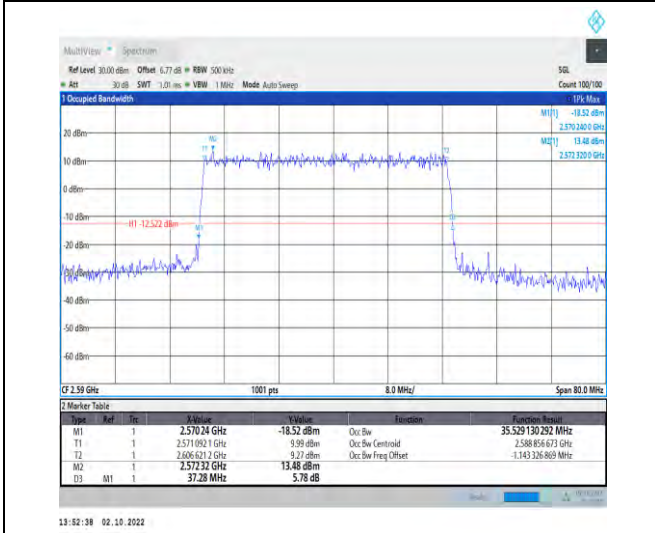
1-N38--30-40-L-1-DFT-QPSK-Outer_Full-100@0-Ant 1-35.529-37.280-≤40-PASS
