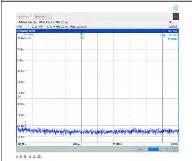
1-N38--30-40-H-1-DFT-PI2BPSK-Inner_1RB_Left-1 @1-30-1000-Ant1-83.35--59.71--35-PASS
