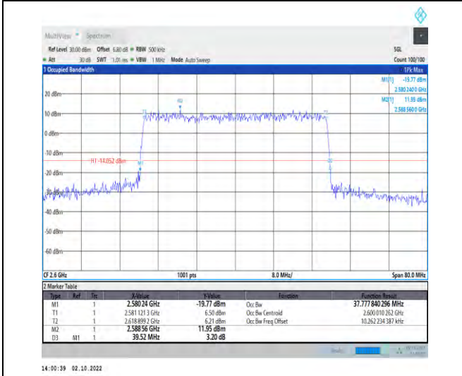
1-N38--30-40-H-7-CP-16QAM-Outer_Full-106@0-Ant1-37.778-39.520-<math>\leq 40</math>-PASS
