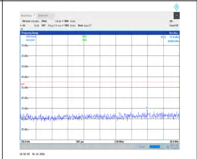
1-N38--30-40-M-1-DFT-PI2BPSK-Inner_1RB_Left-1 @1-0.15-30-Ant1-23.94--72.78--45-PASS
