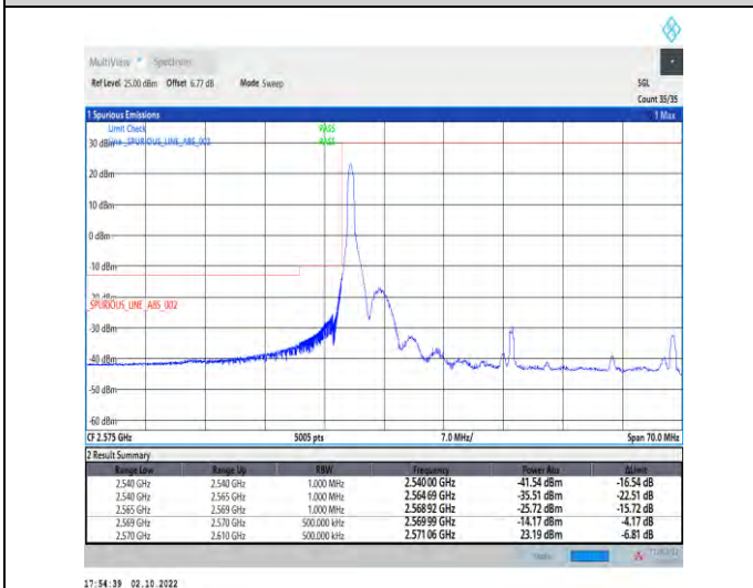
1-N38--30-40-L-4-CP-QPSK-Edge_1RB_Left-1@0-Ant1-1--PASS-see graph
