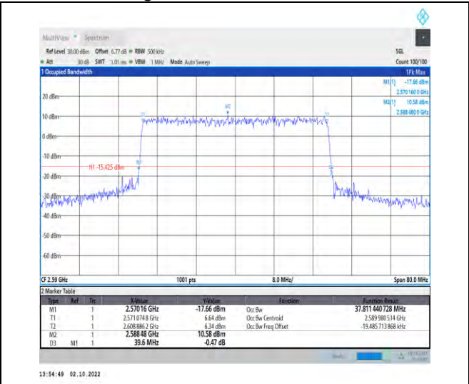
1-N38--30-40-L-8-CP-64QAM-Outer_Full-106@0-An t1-37.811-39.600-≤40-PASS
