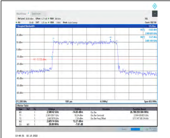
1-N38--30-30-M-1-DFT-QPSK-Outer_Full-75@0-Ant 1-26.78-28.080-≤30-PASS
