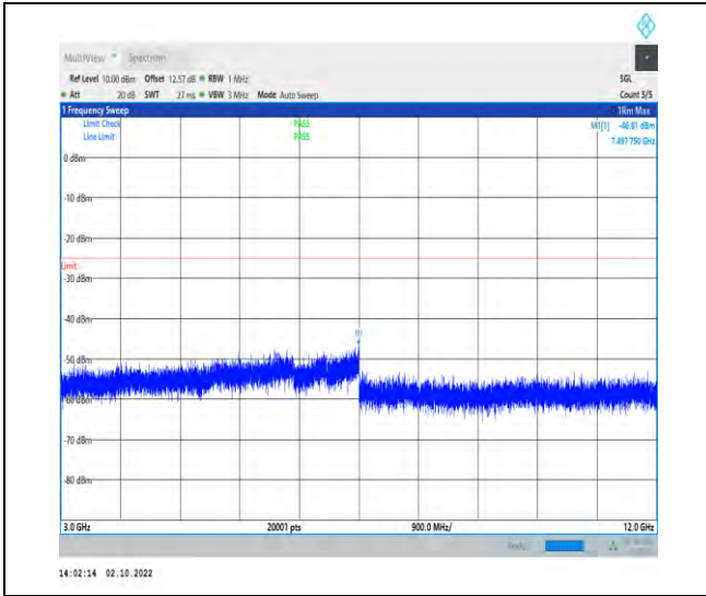
1-N38--30-40-L-1-DFT-PI2BPSK-Inner_1RB_Left-1 @1-3000-12000-Ant1-7497.75--46.81--25-PASS
