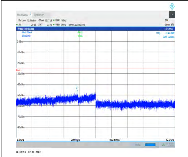
1-N38--30-40-M-1-DFT-PI2BPSK-Inner_1RB_Left-1 @1-3000-12000-Ant1-6455.55--47.27--25-PASS
