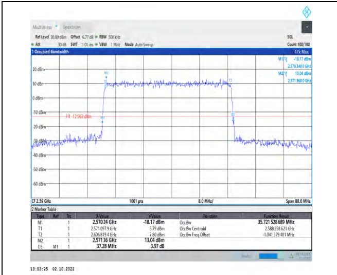
1-N38--30-40-L-3-DFT-16QAM-Outer_Full-100@0-A nt1-35.722-37.280-≤40-PASS
