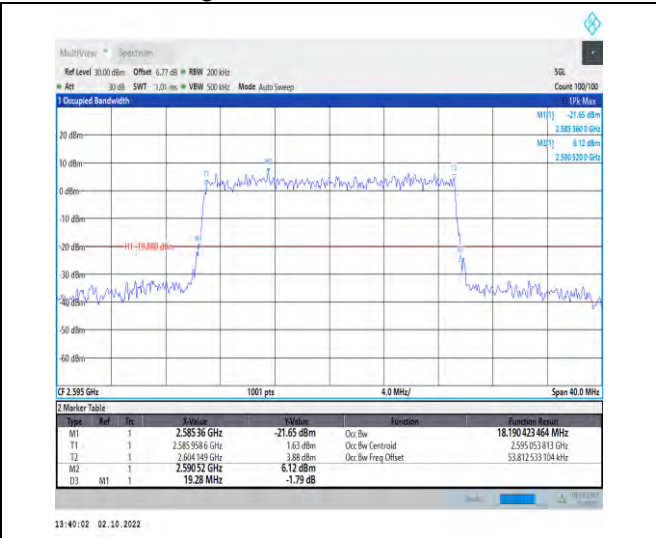
1-N38--30-20-M-9-CP-256QAM-Outer_Full-51@0-A nt1-18.19-19.280-≤20-PASS
