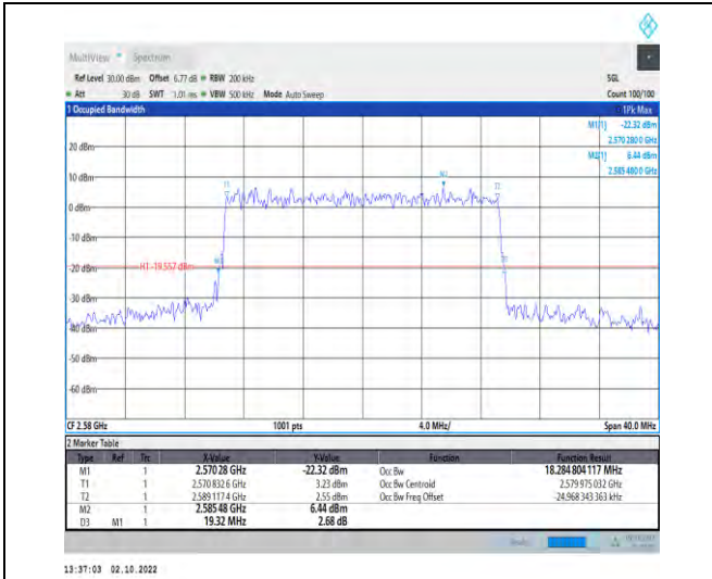
1-N38--30-20-L-9-CP-256QAM-Outer_Full-51@0-Ant 1-18.285-19.320-≤20-PASS
