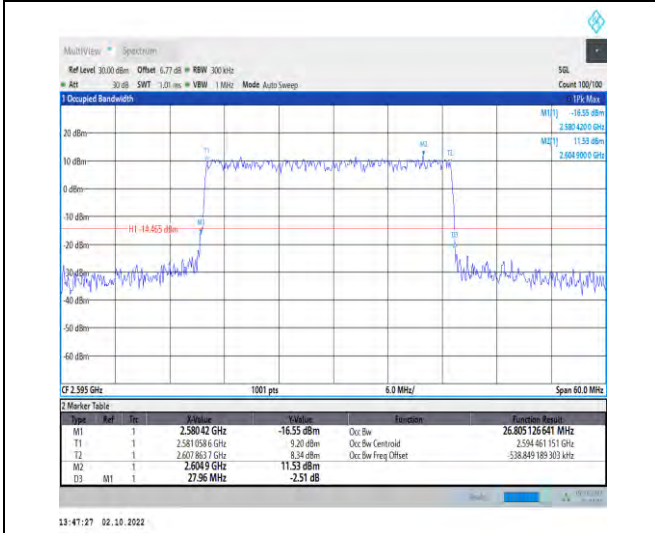
1-N38--30-30-M-3-DFT-16QAM-Outer_Full-75@0-Ant 1-26.805-27.960-≤30-PASS
