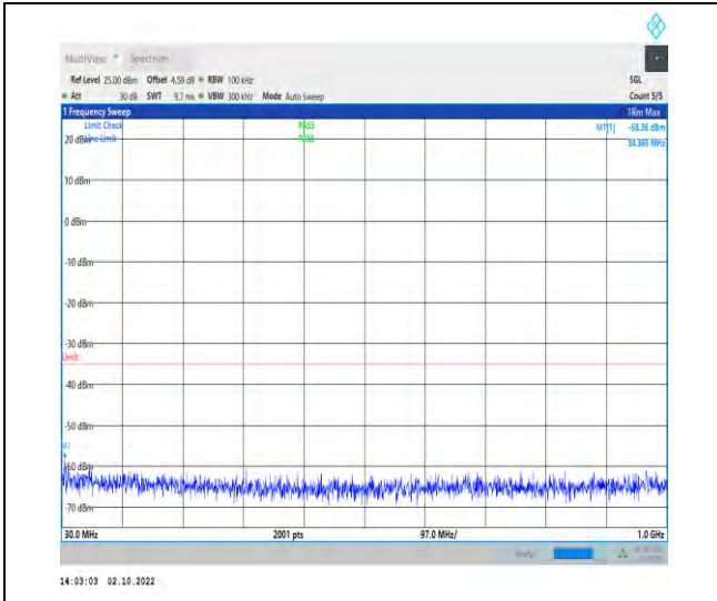
1-N38--30-40-M-1-DFT-PI2BPSK-Inner_1RB_Left-1 @1-30-1000-Ant1-34.37--58.36--35-PASS
