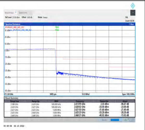
1-N38--30-40-H-6-CP-QPSK-Outer_Full-106@0-Ant1-1--PASS-see graph
