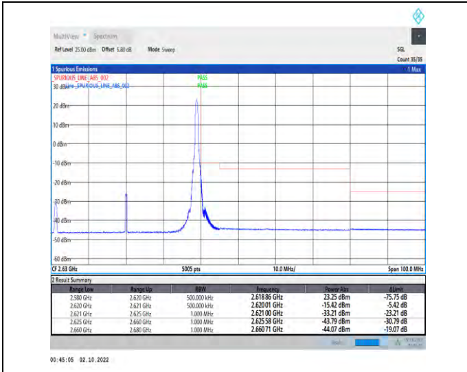
1-N38--30-40-H-2-DFT-PI2BPSK-Edge_1RB_Right-1@105-Ant1-1--PASS-see graph
