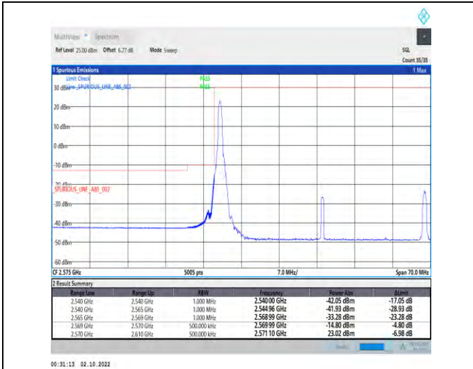
1-N38--30-40-L-1-DFT-PI2BPSK-Edge_1RB_Left-1@0-Ant1-1--PASS-see graph
