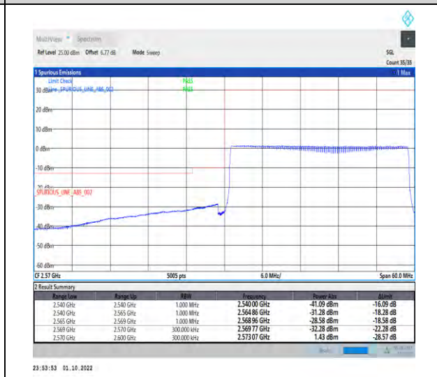
1-N38--30-30-L-6-CP-QPSK-Outer_Full-78@0-Ant1-1--PASS-see graph
