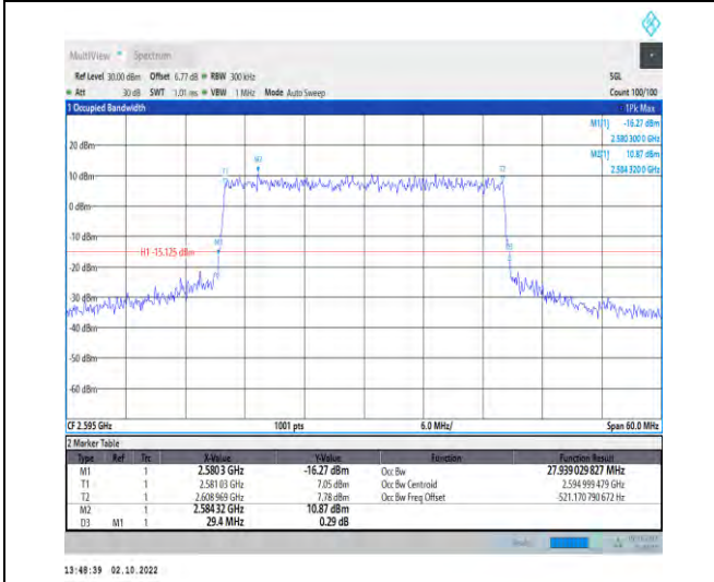
1-N38--30-30-M-7-CP-16QAM-Outer_Full-78@0-Ant 1-27.939-29.400-≤30-PASS
