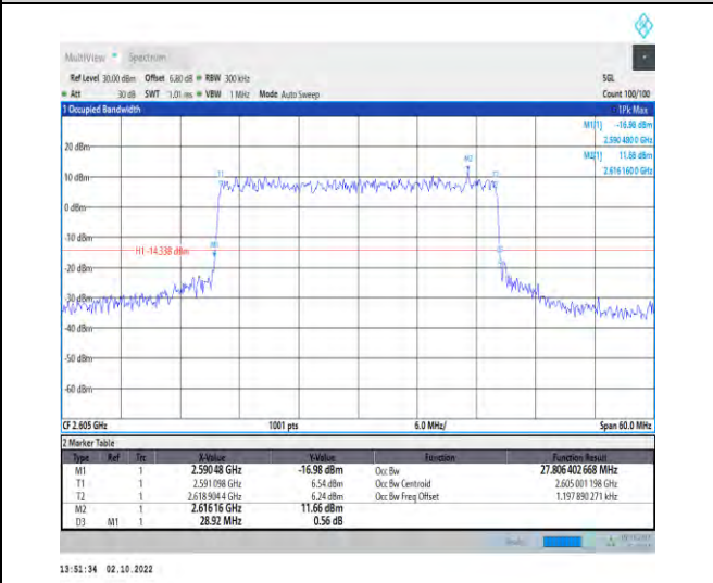
1-N38--30-30-H-7-CP-16QAM-Outer_Full-78@0-Ant 1-27.806-28.920-<30-PASS
