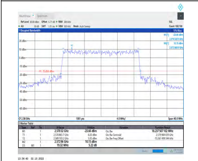
1-N38--30-20-L-7-CP-16QAM-Outer_Full-51@0-Ant1 -18.238-19.320-≤20-PASS
