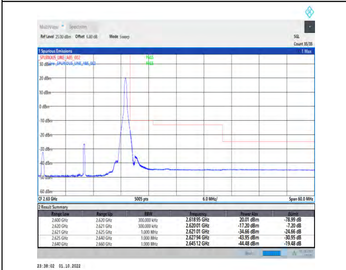
1-N38--30-20-H-5-CP-QPSK-Edge_1RB_Right-1@50-Ant1-1--PASS-see graph
