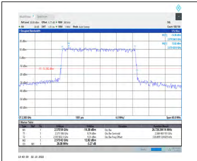
1-N38--30-30-L-6-CP-QPSK-Outer_Full-78@0-Ant1-59.438-60.000-<=30-PASS
