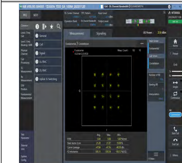
1-N38--30-40-M-7-CP-16QAM-Outer_Full-106@0-Ant1-see graph-PASS
