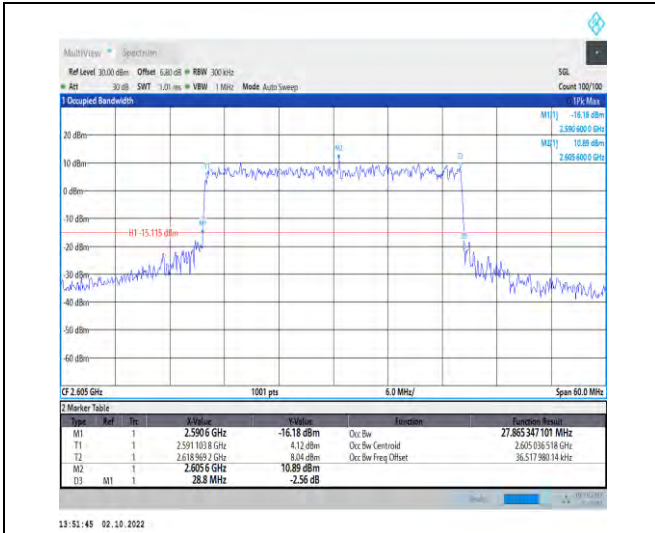
1-N38--30-30-H-8-CP-64QAM-Outer_Full-78@0-Ant 1-27.865-28.800-≤30-PASS
