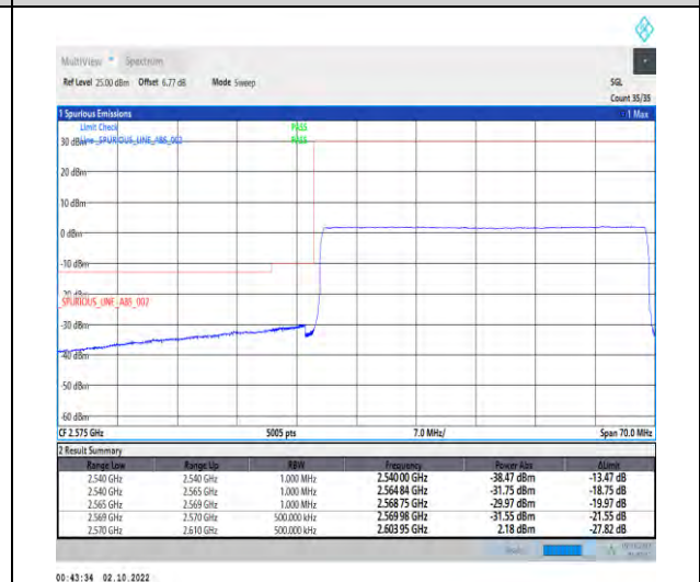
1-N38--30-40-L-6-CP-QPSK-Outer_Full-106@0-Ant1-1--PASS-see graph
