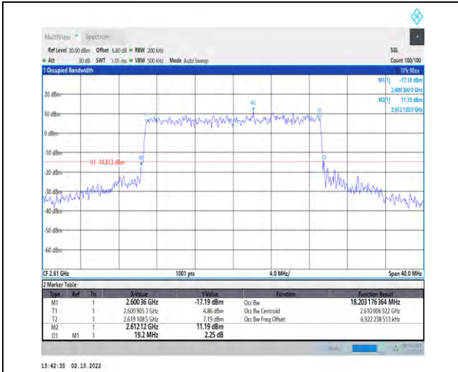
1-N38--30-20-H-7-CP-16QAM-Outer_Full-51@0-Ant 1-18.203-19.200-≤20-PASS
