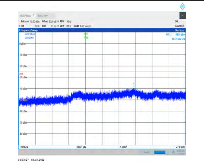
1-N38--30-40-M-1-DFT-PI2BPSK-Inner_1RB_Left-1 @1-12000-27000-Ant1-22375.00--38.84--25-PASS
