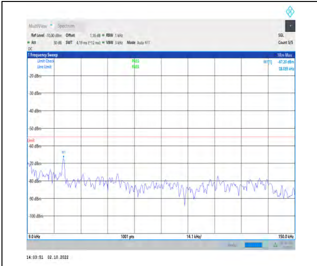
1-N38--30-40-H-1-DFT-PI2BPSK-Inner_1RB_Left-1 @1-0.009-0.15-Ant1-0.03--67.20--55-PASS
