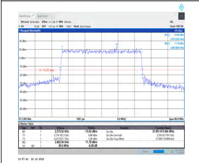
1-N38--30-40-M-8-CP-64QAM-Outer_Full-106@0-Ant 1-37.851-39.600-≤40-PASS
