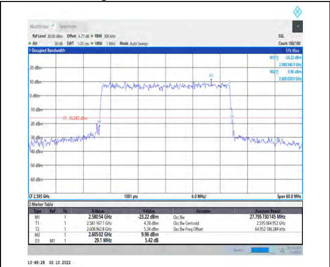
1-N38--30-30-M-6-CP-QPSK-Outer_Full-78@0-Ant1 -27.796-29.100-≤30-PASS
