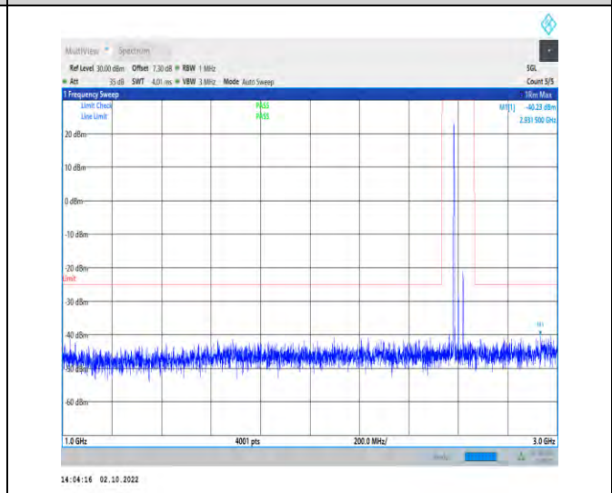
1-N38--30-40-H-1-DFT-PI2BPSK-Inner_1RB_Left-1 @1-1000-3000-Ant1-2931.50--40.23--25-PASS
