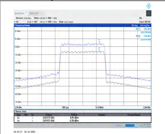
1-N38--30-40-H-2-CP-256QAM-Outer_Full-106@0-Ant1-10.29-19.4%-7.12-3.17-PASS-≤13
