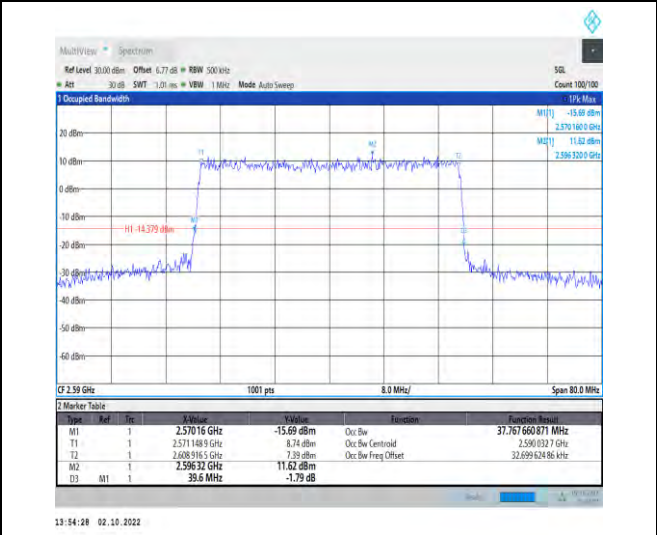
1-N38--30-40-L-6-CP-QPSK-Outer_Full-106@0-Ant 1-37.768-39.600-≤40-PASS
