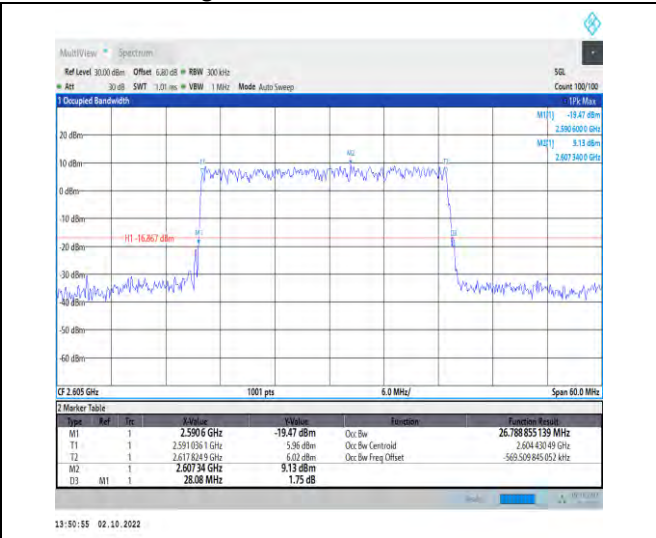
1-N38--30-30-H-5-DFT-256QAM-Outer_Full-75@0-Ant nt1-26.789-28.080-<30-PASS
