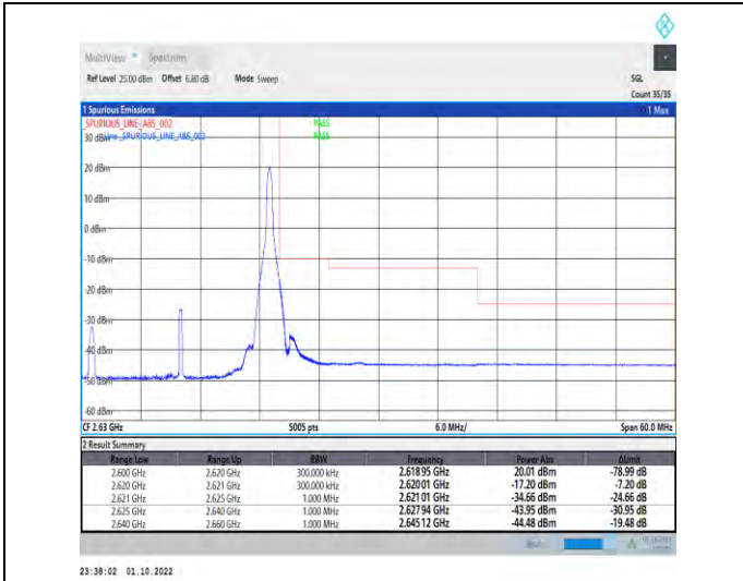
1-N38--30-20-H-2-DFT-PI2BPSK-Edge_1RB_Right-1@50-Ant1-1--PASS-see graph
