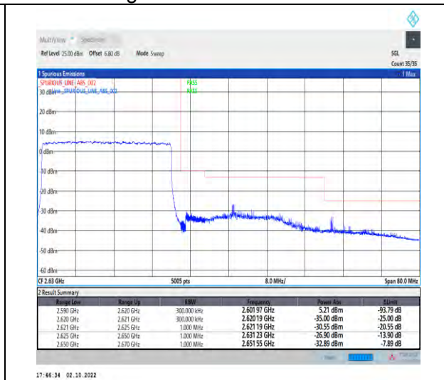
1-N38--30-30-H-3-DFT-PI2BPSK-Outer_Full-75@0-Ant1-1--PASS-see graph
