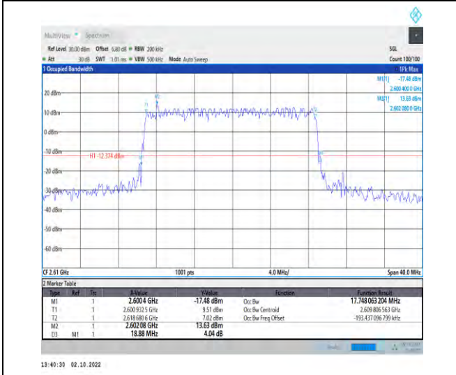
1-N38--30-20-H-1-DFT-QPSK-Outer_Full-50@0-Ant 1-17.748-18.880-≤20-PASS
