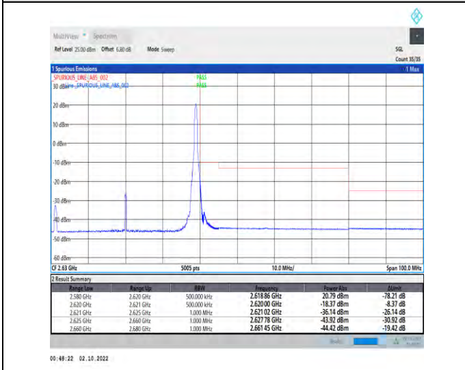
1-N38--30-40-H-5-CP-QPSK-Edge_1RB_Right-1@105-Ant1-1--PASS-see graph
