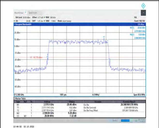
1-N38--30-30-L-5-DFT-256QAM-Outer_Full-75@0-A nt1-26.589-28.080-≤30-PASS
