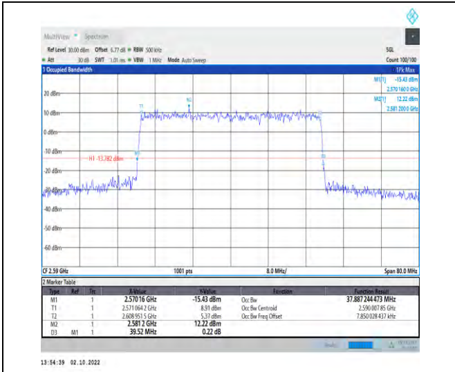
1-N38--30-40-L-7-CP-16QAM-Outer_Full-106@0-Ant 1-37.887-39.520-≤40-PASS
