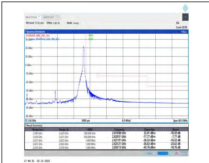
1-N38--30-30-H-2-DFT-PI2BPSK-Edge_1RB_Right-1@77-Ant1-1--PASS-see graph
