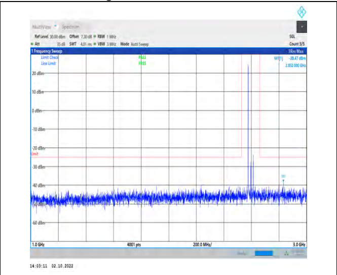
1-N38--30-40-M-1-DFT-PI2BPSK-Inner_1RB_Left-1 @1-1000-3000-Ant1-2832.00--38.47--25-PASS
