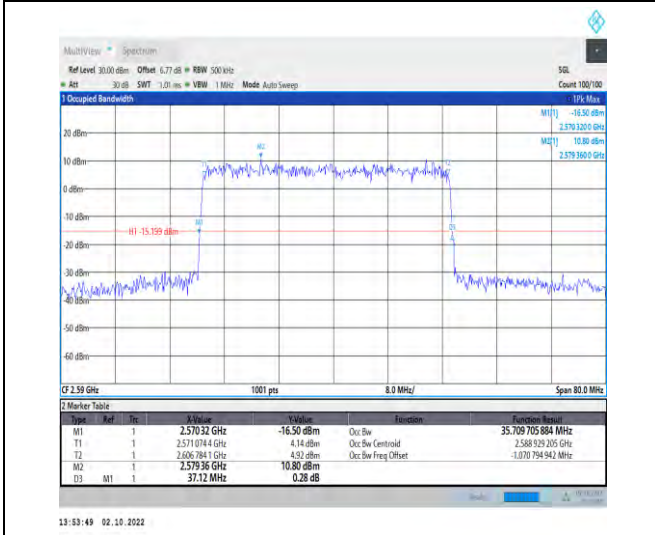
1-N38--30-40-L-5-DFT-256QAM-Outer_Full-100@0- Ant1-35.71-37.120-≤40-PASS
