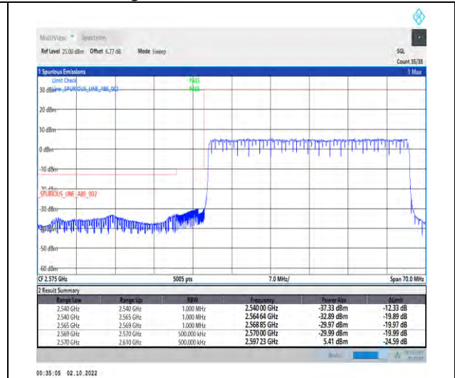
1-N38--30-40-L-3-DFT-PI2BPSK-Outer_Full-100@0-Ant1-1--PASS-see graph
