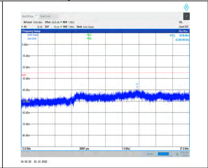
1-N38--30-40-L-1-DFT-PI2BPSK-Inner_1RB_Left-1@ 1-12000-27000-Ant1-22339.50--38.38--25-PASS
