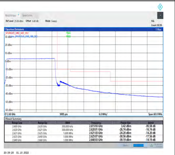
1-N38--30-20-H-6-CP-QPSK-Outer_Full-51@0-Ant1-1--PASS-see graph
