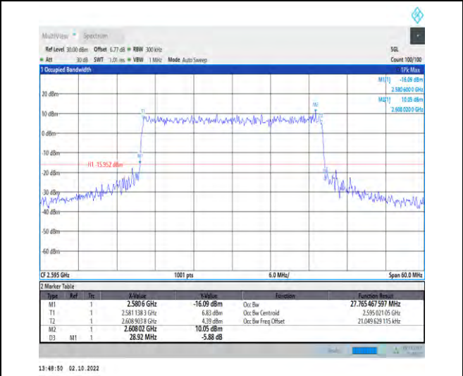
1-N38--30-30-M-8-CP-64QAM-Outer_Full-78@0-Ant 1-27.765-28.920-≤30-PASS
