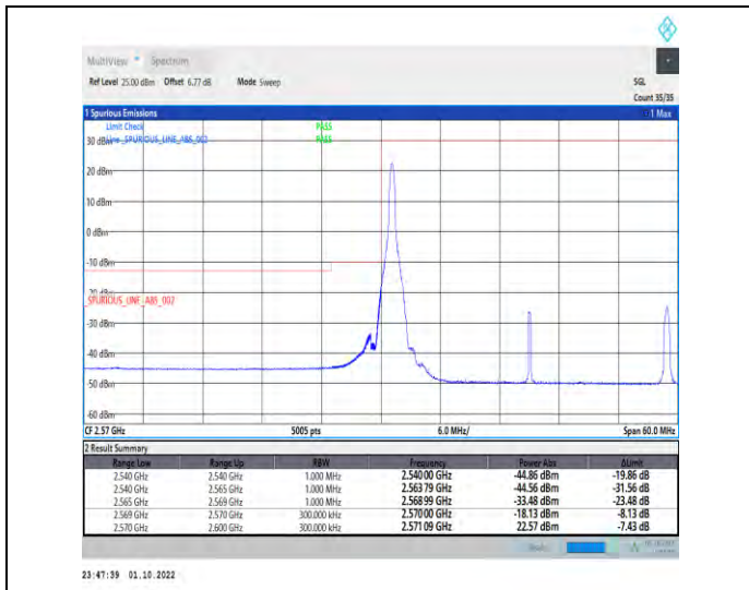
1-N38--30-30-L-1-DFT-PI2BPSK-Edge_1RB_Left-1@0-Ant1-1--PASS-see graph
