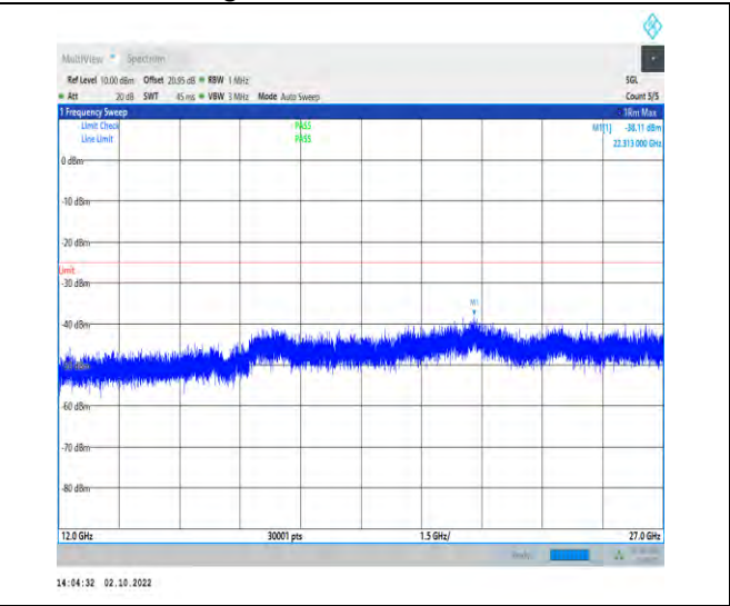
1-N38--30-40-H-1-DFT-PI2BPSK-Inner_1RB_Left-1 @1-12000-27000-Ant1-22313.00--38.11--25-PASS
