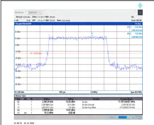
1-N38--30-20-M-2-DFT-PI2BPSK-Outer_Full-50@0-Ant1 1-17.788-19.120-≤20-PASS
