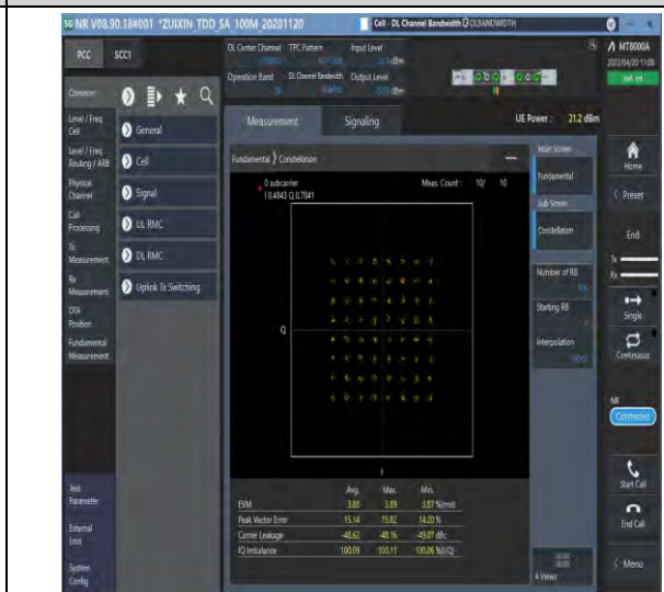
1-N38--30-40-M-8-CP-64QAM-Outer_Full-106@0-Ant1-see graph-PASS
