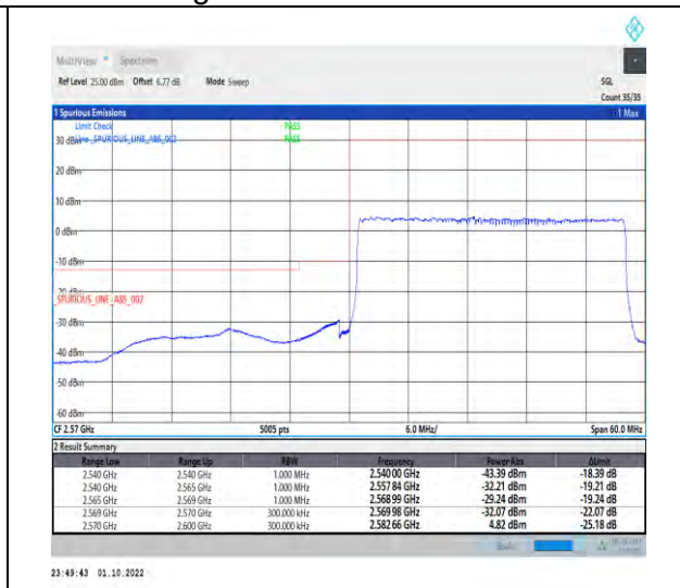
1-N38--30-30-L-3-DFT-PI2BPSK-Outer_Full-75@0-Ant1-1--PASS-see graph
