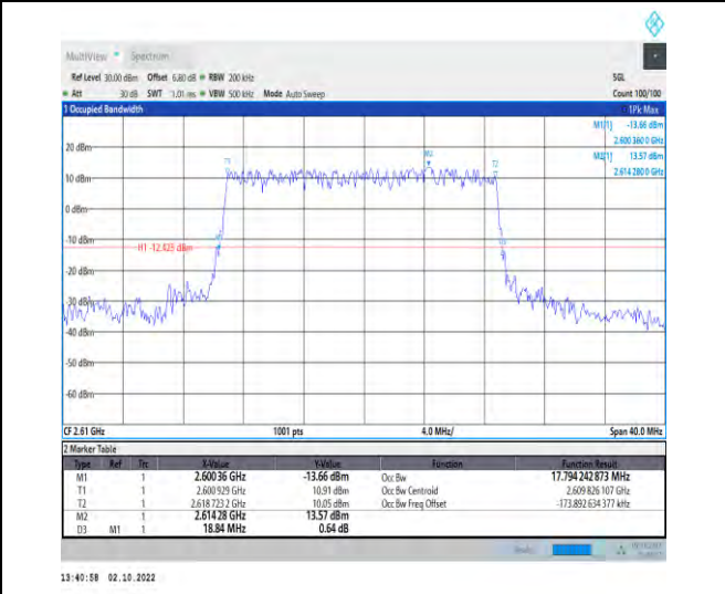
1-N38--30-20-H-2-DFT-PI2BPSK-Outer_Full-50@0-Ant 1-17.794-18.840-≤20-PASS
