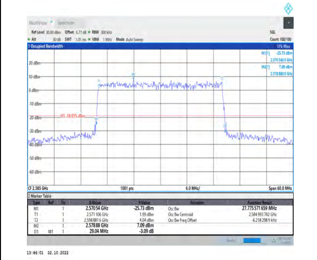
1-N38--30-30-L-9-CP-256QAM-Outer_Full-78@0-Ant1-27.776-29.040-<=30-PASS
