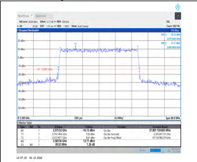
1-N38--30-40-M-7-CP-16QAM-Outer_Full-106@0-Ant 1-37.801-39.520-≤40-PASS
