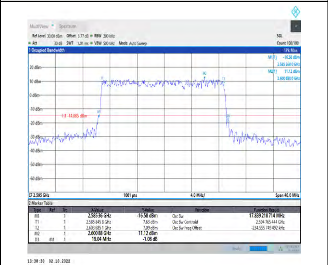
1-N38--30-20-M-3-DFT-16QAM-Outer_Full-50@0-Ant1 1-17.839-19.040-≤20-PASS
