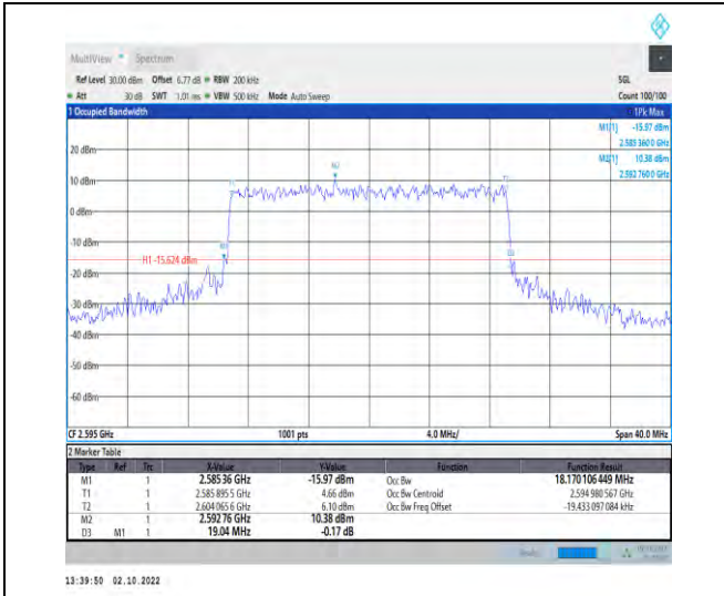
1-N38--30-20-M-8-CP-64QAM-Outer_Full-51@0-Ant 1-18.17-19.040-≤20-PASS
