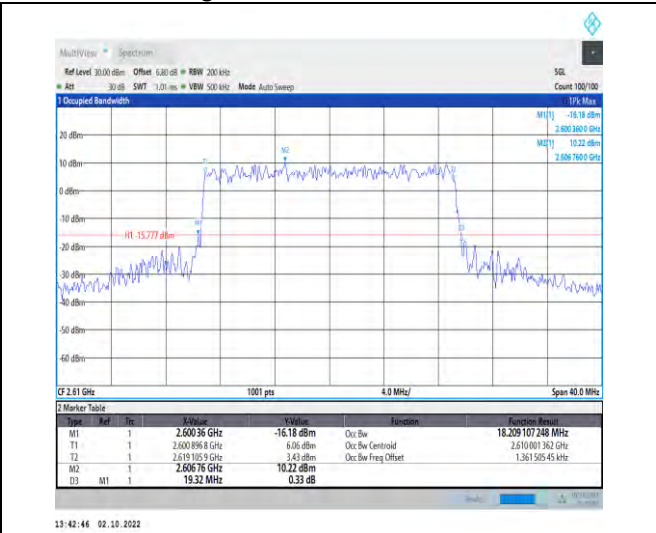
1-N38--30-20-H-8-CP-64QAM-Outer_Full-51@0-Ant 1-18.209-19.320-≤20-PASS
