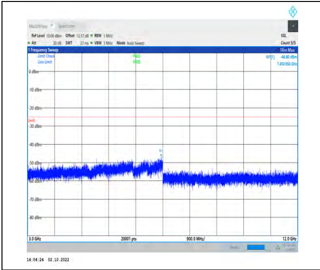
1-N38--30-40-H-1-DFT-PI2BPSK-Inner_1RB_Left-1 @1-3000-12000-Ant1-7450.05--46.80--25-PASS
