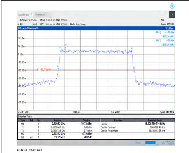
1-N38--30-20-H-9-CP-256QAM-Outer_Full-51@0-Ant t1-18.209-19.320-≤20-PASS
