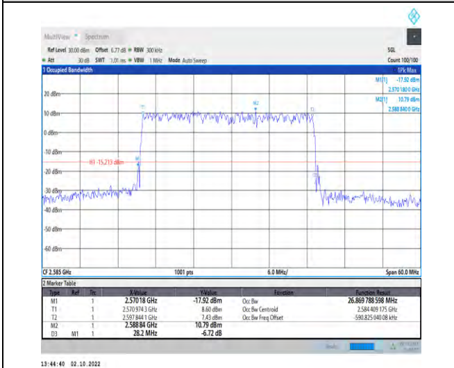
1-N38--30-30-L-4-DFT-64QAM-Outer_Full-75@0-Ant 1-26.87-28.200-≤30-PASS
