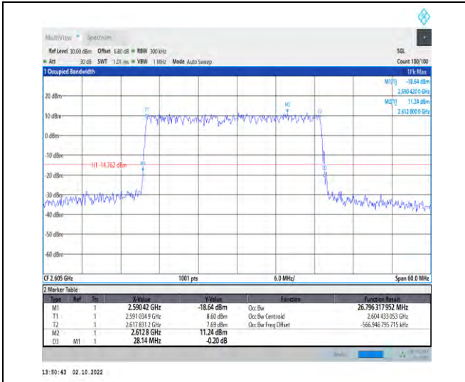
1-N38--30-30-H-4-DFT-64QAM-Outer_Full-75@0-Ant t1-26.796-28.140-<30-PASS
