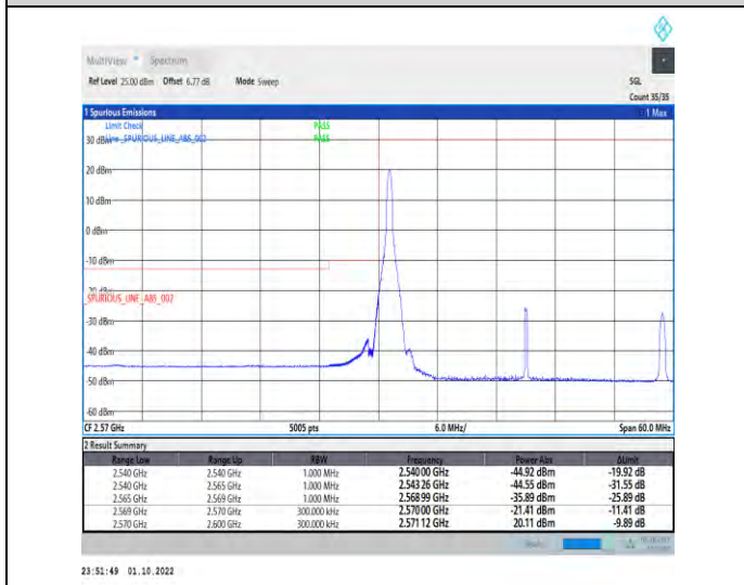
1-N38--30-30-L-4-CP-QPSK-Edge_1RB_Left-1@0-Ant1-1--PASS-see graph
