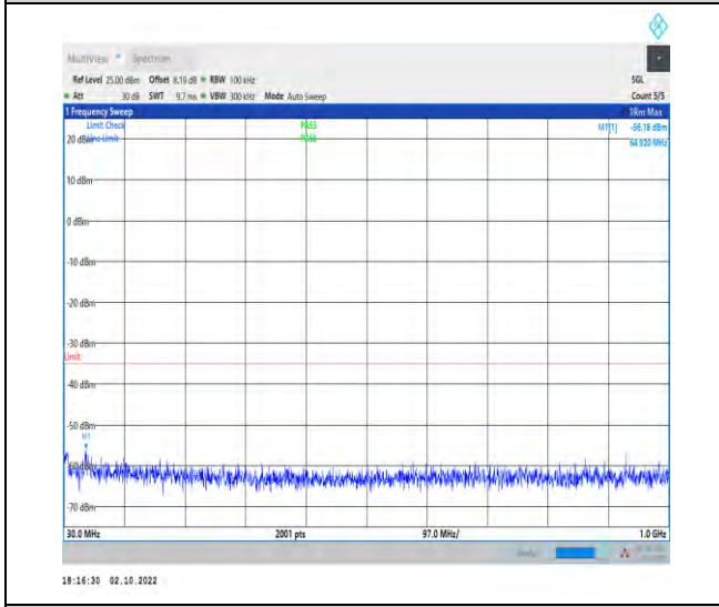
1-N7--15-50-H-1-DFT-PI2BPSK-Inner_1RB_Left-1 @1-30-1000-Ant1-64.92--56.18--35-PASS
