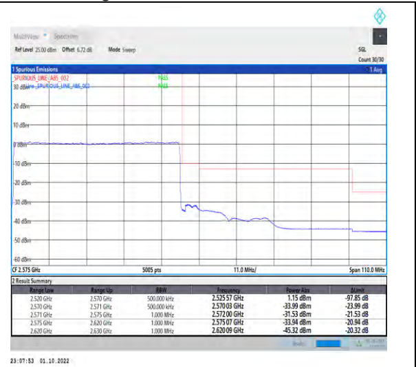
1-N7--15-50-H-3-DFT-PI2BPSK-Outer_Full-270@0-Ant1-1--PASS-see graph
