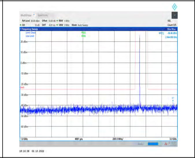
1-N7--15-50-H-1-DFT-PI2BPSK-Inner_1RB_Left-1@ 1-1000-3000-Ant1-2944.00--36.46--25-PASS
