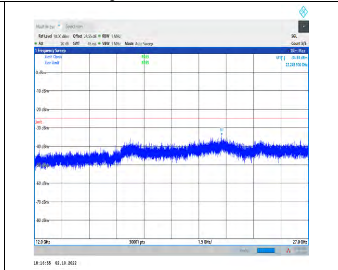
1-N7--15-50-H-1-DFT-PI2BPSK-Inner_1RB_Left-1@ 1-12000-27000-Ant1-22245.50--34.33--25-PASS
