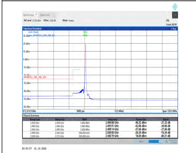
1-N7--15-50-L-4-CP-QPSK-Edge_1RB_Left-1@0-Ant1-1--PASS-see graph
