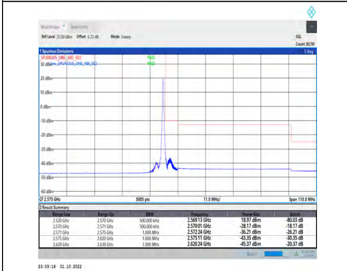
1-N7--15-50-H-5-CP-QPSK-Edge_1RB_Right-1@269-Ant1-1--PASS-see graph
