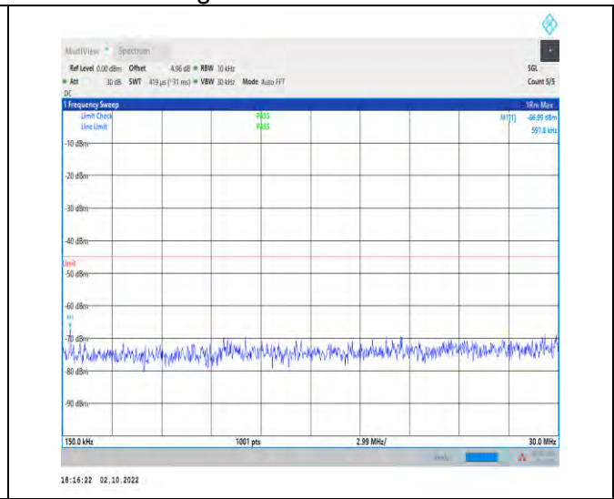
1-N7--15-50-H-1-DFT-PI2BPSK-Inner_1RB_Left-1@ 1-0.15-30-Ant1-0.60--66.99--45-PASS
