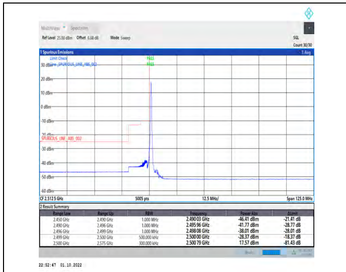
1-N7--15-50-L-1-DFT-PI2BPSK-Edge_1RB_Left-1@0-Ant1-1--PASS-see graph
