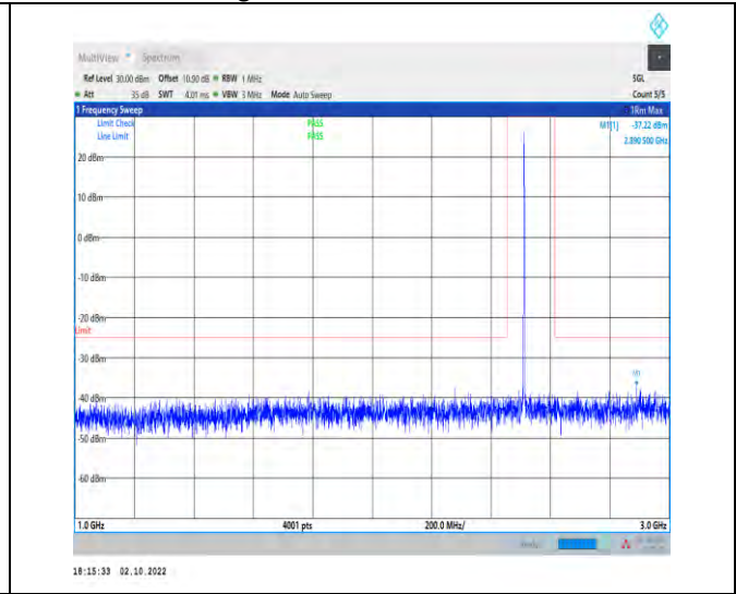
1-N7--15-50-M-1-DFT-PI2BPSK-Inner_1RB_Left-1 @ 1-1000-3000-Ant1-2890.50--37.22--25-PASS
