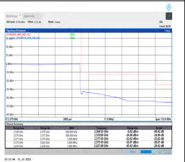
1-N7--15-50-H-6-CP-QPSK-Outer_Full-270@0-Ant1-1--PASS-see graph
