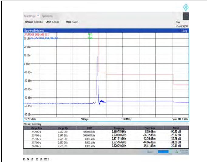
1-N7--15-50-H-2-DFT-PI2BPSK-Edge_1RB_Right-1@2 69-Ant1-1--PASS-see graph
