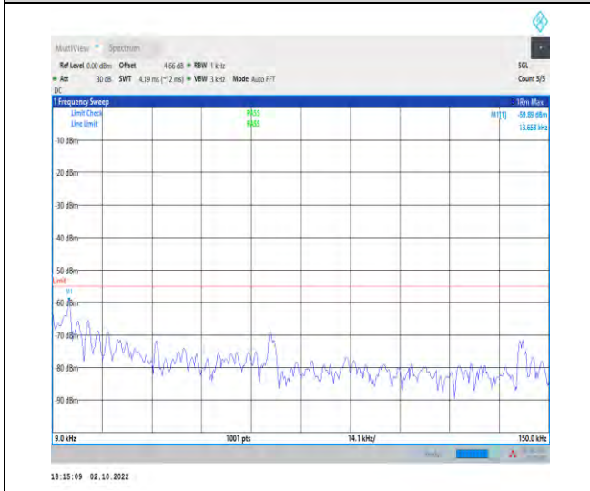
1-N7--15-50-M-1-DFT-PI2BPSK-Inner_1RB_Left-1 @ 1-0.009-0.15-Ant1-0.01--59.89--55-PASS
