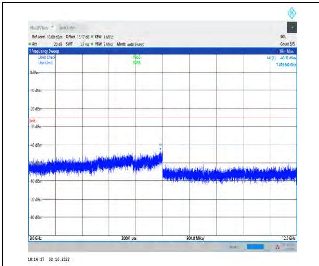
1-N7--15-50-L-1-DFT-PI2BPSK-Inner_1RB_Left-1@ 1-3000-12000-Ant1-7429.80--43.37--25-PASS
