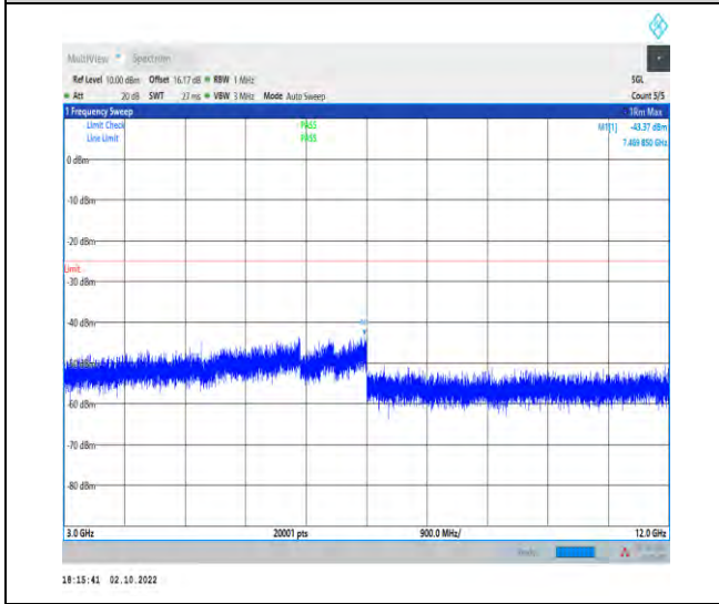
1-N7--15-50-M-1-DFT-PI2BPSK-Inner_1RB_Left-1 @ 1-3000-12000-Ant1-7469.85--43.37--25-PASS
