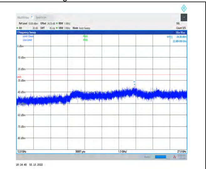
1-N7--15-50-L-1-DFT-PI2BPSK-Inner_1RB_Left-1@ 1-12000-27000-Ant1-22389.00--34.38--25-PASS
