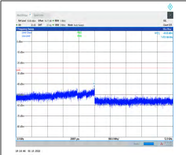
1-N7--15-50-H-1-DFT-PI2BPSK-Inner_1RB_Left-1 @ 1-3000-12000-Ant1-7472.10--43.02--25-PASS
