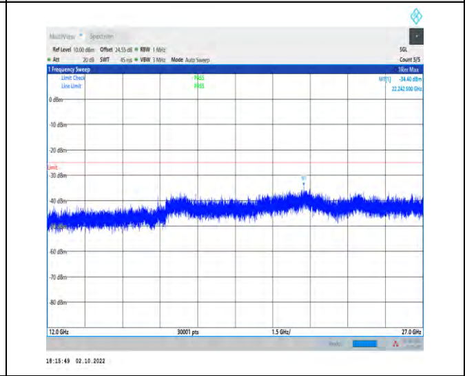
1-N7--15-50-M-1-DFT-PI2BPSK-Inner_1RB_Left-1 @ 1-12000-27000-Ant1-22242.50--34.40--25-PASS
