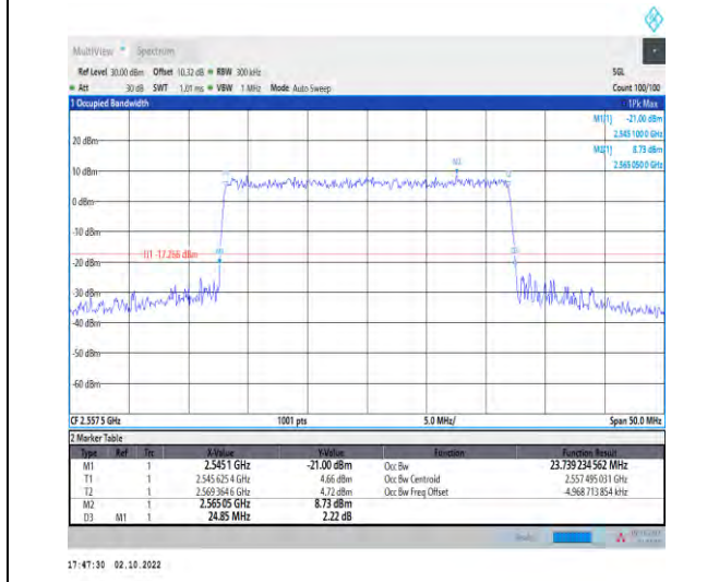
1-N7--15-25-H-9-CP-256QAM-Outer_Full-133@0-Ant t1-23.739-24.850-≤25-PASS
