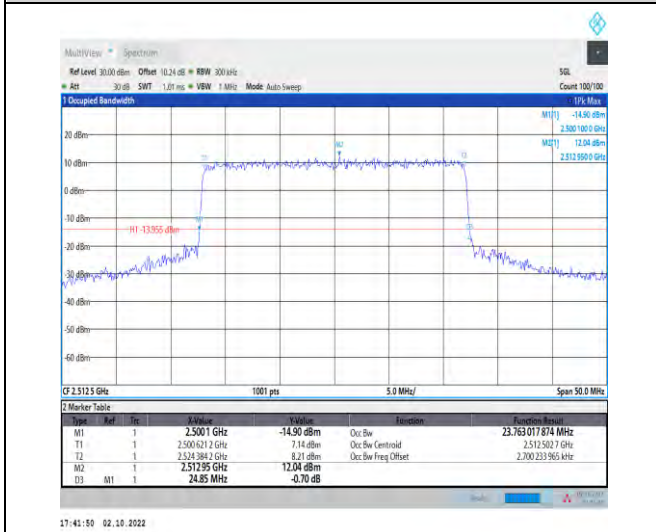
1-N7--15-25-L-7-CP-16QAM-Outer_Full-133@0-Ant 1-23.763-24.850-≤25-PASS
