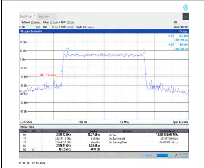
1-N7--15-20-M-9-CP-256QAM-Outer_Full-106@0-A nt1-18.924-19.720-≤20-PASS
