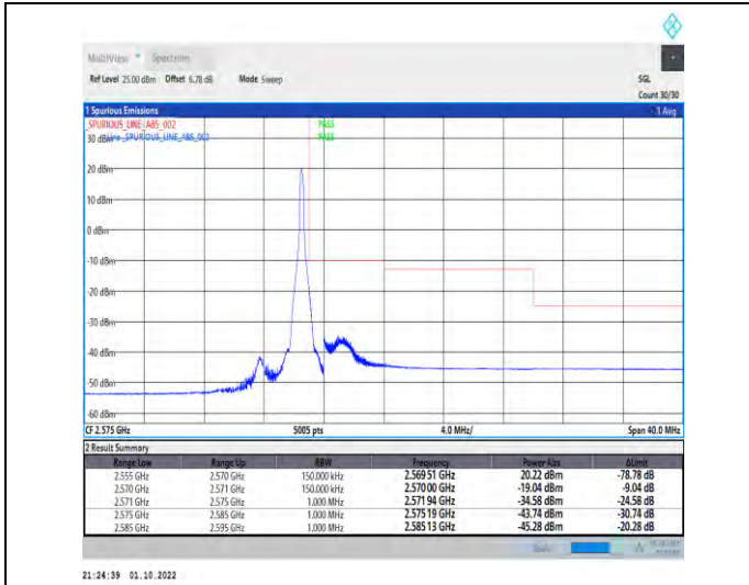
1-N7--15-15-H-2-DFT-PI2BPSK-Edge_1RB_Right-1@78-Ant1-1--PASS-see graph
