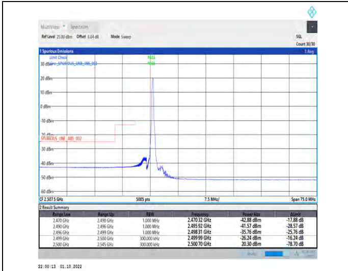
1-N7--15-30-L-1-DFT-PI2BPSK-Edge_1RB_Left-1@0-Ant1-1--PASS-see graph
