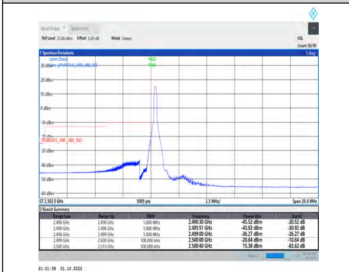
1-N7--15-10-L-4-CP-QPSK-Edge_1RB_Left-1@0-Ant1-1--PASS-see graph
