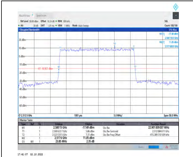
1-N7--15-25-L-5-DFT-256QAM-Outer_Full-128@0-A nt1-22.902-23.850-≤25-PASS
