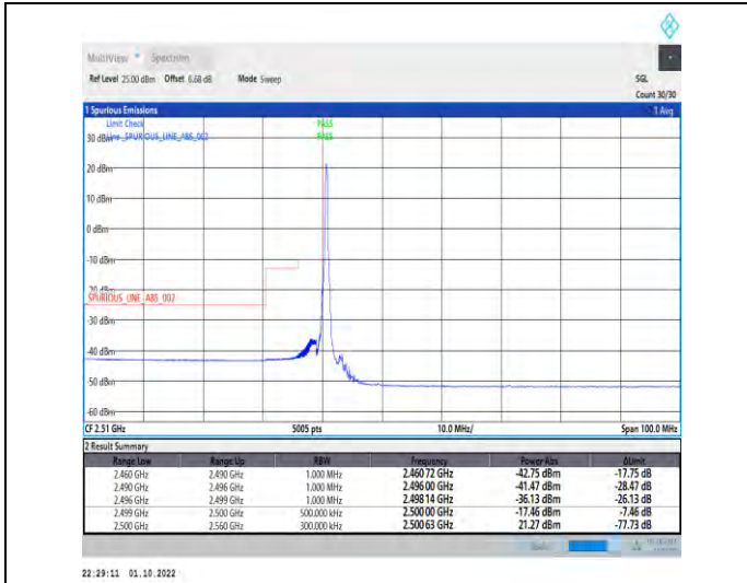
1-N7--15-40-L-1-DFT-PI2BPSK-Edge_1RB_Left-1@0-Ant1-1--PASS-see graph
