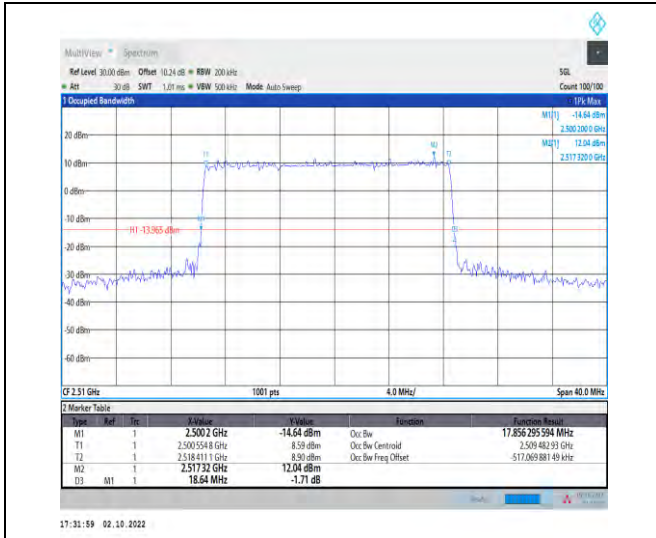
1-N7--15-20-L-4-DFT-64QAM-Outer_Full-100@0-Ant 1-17.856-18.640-≤20-PASS
