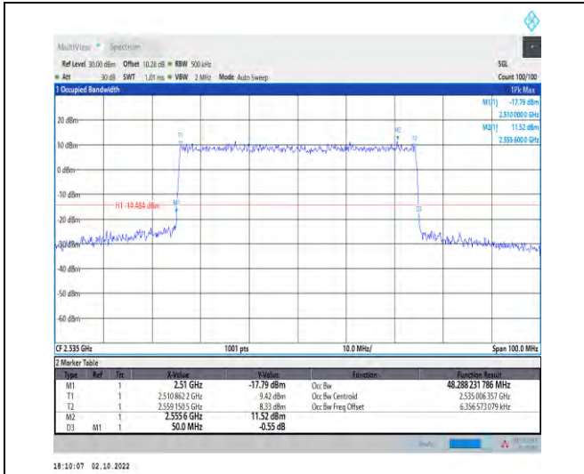
1-N7--15-50-M-7-CP-16QAM-Outer_Full-270@0-Ant 1-48.288-50.000-≤50-PASS
