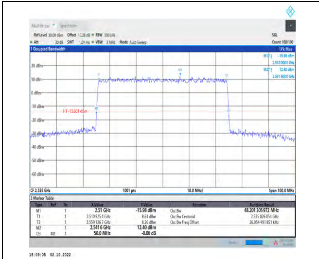
1-N7--15-50-M-3-DFT-16QAM-Outer_Full-270@0-An t1-48.201-50.000-<=50-PASS
