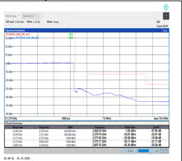
1-N7--15-30-H-3-DFT-PI2BPSK-Outer_Full-160@0-Ant1-1--PASS-see graph
