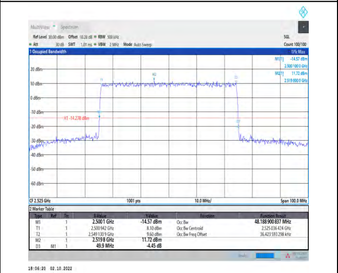
1-N7--15-50-L-3-DFT-16QAM-Outer_Full-270@0-Ant 1-48.189-49.900-<=50-PASS
