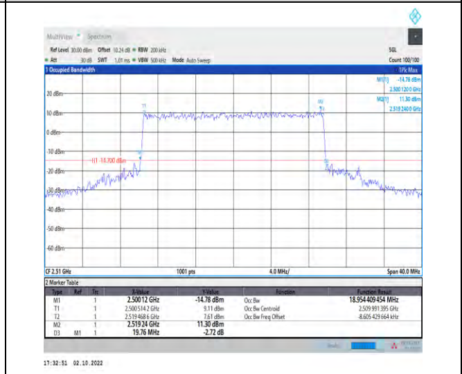
1-N7--15-20-L-7-CP-16QAM-Outer_Full-106@0-Ant 1-18.954-19.760-≤20-PASS
