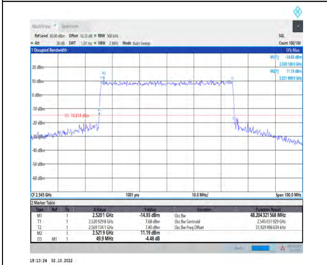
1-N7--15-50-H-8-CP-64QAM-Outer_Full-270@0-Ant 1-48.204-49.900-≤50-PASS
