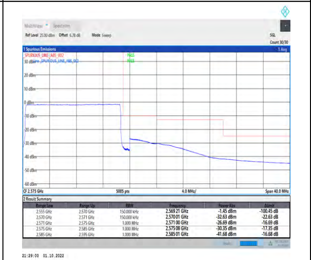
1-N7--15-15-H-6-CP-QPSK-Outer_Full-79@0-Ant1-1--PASS-see graph
