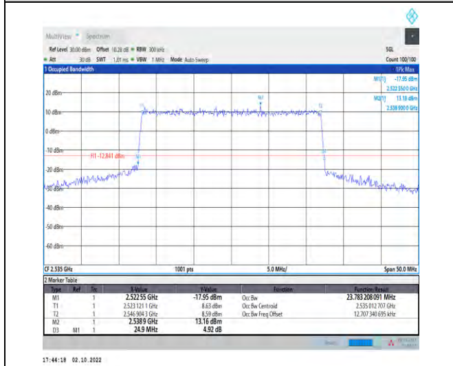
1-N7--15-25-M-6-CP-QPSK-Outer_Full-133@0-Ant1-23.783-24.900-<25-PASS
