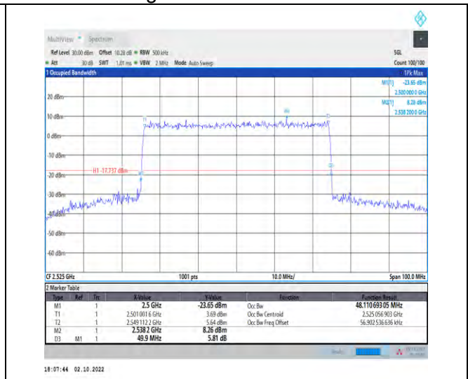
1-N7--15-50-L-9-CP-256QAM-Outer_Full-270@0-Ant t1-48.111-49.900-≤50-PASS
