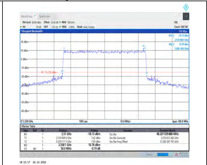
1-N7--15-50-M-8-CP-64QAM-Outer_Full-270@0-Ant 1-48.208-50.000-≤50-PASS
