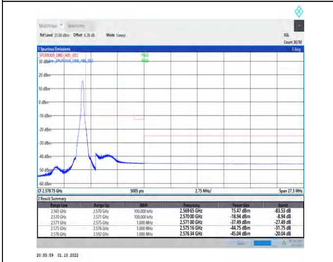
1-N7--15-5-H-5-CP-QPSK-Edge_1RB_Right-1@24-Ant1-1--PASS-see graph
