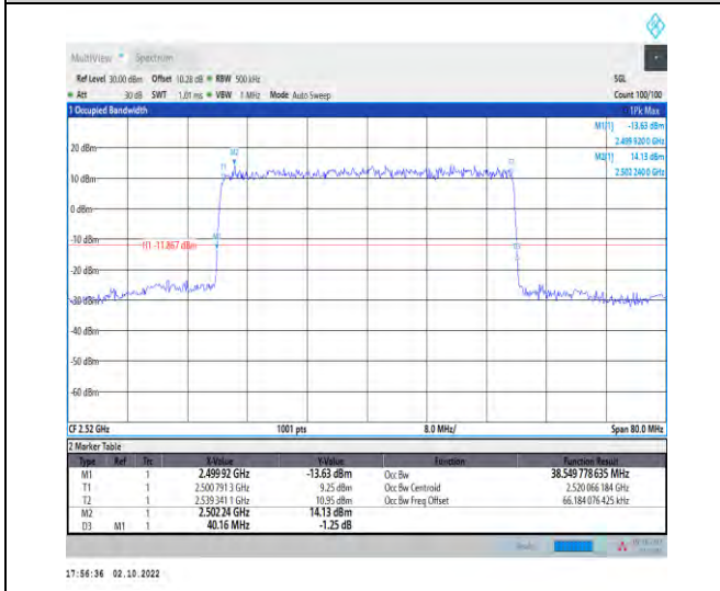
1-N7--15-40-L-1-DFT-QPSK-Outer_Full-216@0-Ant1 -38.55-40.160-≤40-PASS
