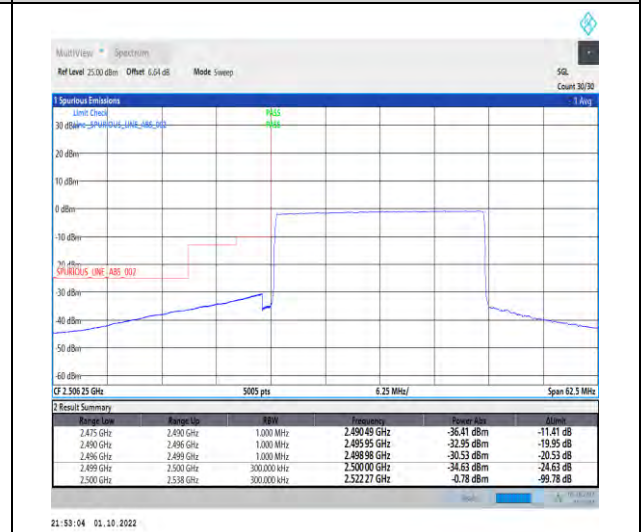
1-N7--15-25-L-6-CP-QPSK-Outer_Full-133@0-Ant1-1--PASS-see graph
