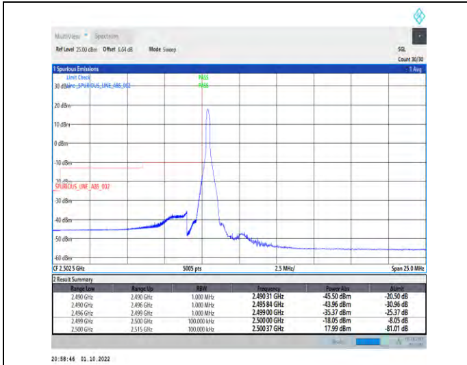
1-N7--15-10-L-1-DFT-PI2BPSK-Edge_1RB_Left-1@0-Ant1-1--PASS-see graph
