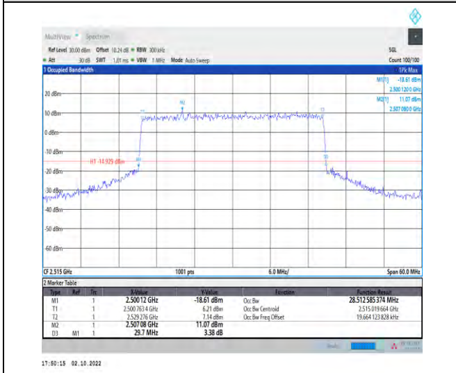
1-N7--15-30-L-8-CP-64QAM-Outer_Full-160@0-Ant1-128.513-29.700-≤30-PASS
