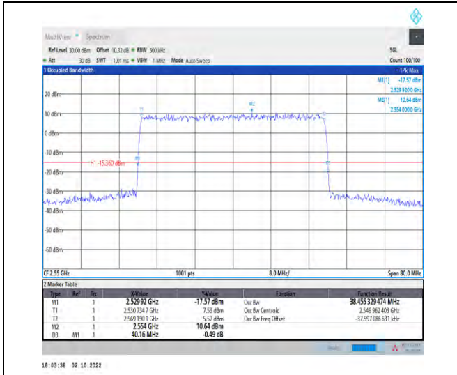
1-N7--15-40-H-5-DFT-256QAM-Outer_Full-216@0-A nt1-38.455-40.160-≤40-PASS
