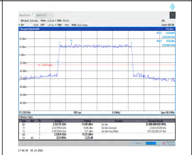
1-N7--15-25-M-3-DFT-16QAM-Outer_Full-128@0-An t1-22.868-23.900-≤25-PASS
