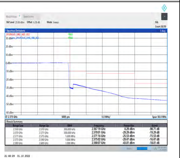
1-N7--15-20-H-6-CP-QPSK-Outer_Full-106@0-Ant1-1--PASS-see graph
