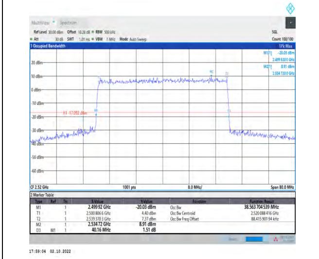
1-N7--15-40-L-9-CP-256QAM-Outer_Full-216@0-An t1-38.564-40.160-≤40-PASS
