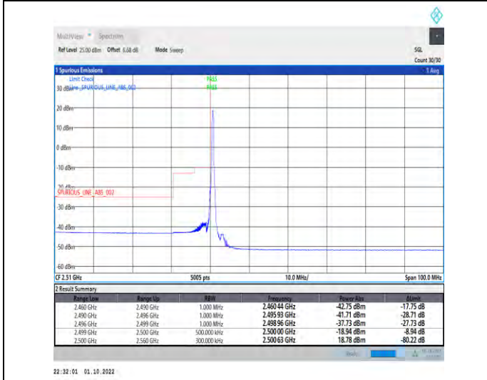
1-N7--15-40-L-4-CP-QPSK-Edge_1RB_Left-1@0-Ant1-1--PASS-see graph
