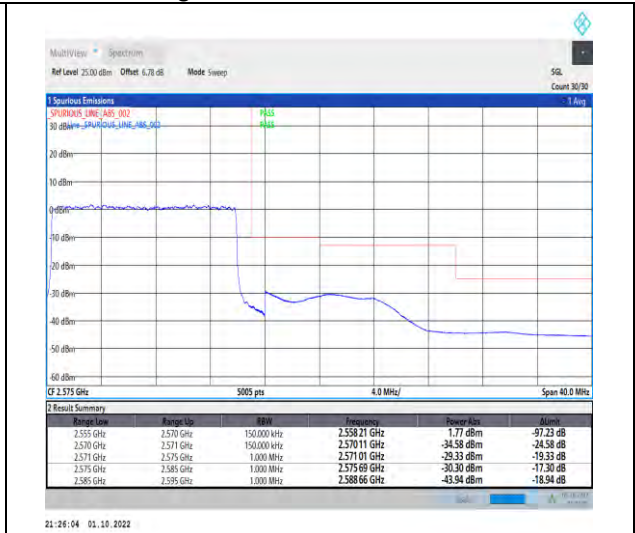
1-N7--15-15-H-3-DFT-PI2BPSK-Outer_Full-75@0-Ant1-1--PASS-see graph
