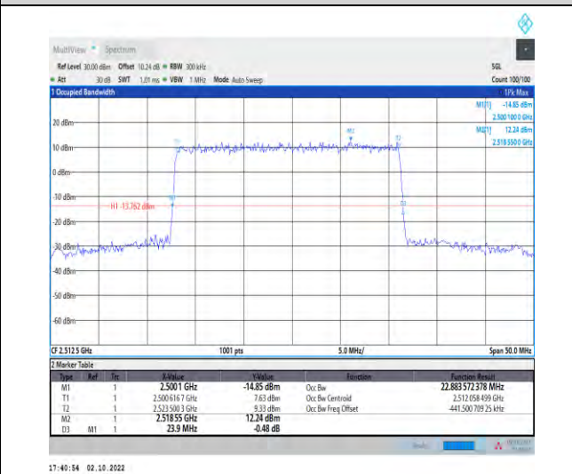
1-N7--15-25-L-4-DFT-64QAM-Outer_Full-128@0-Ant1 1-22.884-23.900-≤25-PASS
