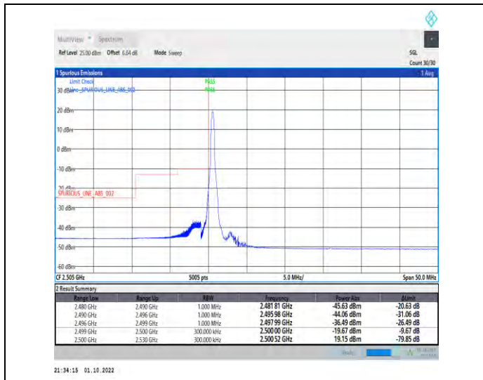
1-N7--15-20-L-1-DFT-PI2BPSK-Edge_1RB_Left-1@0-Ant1-1--PASS-see graph
