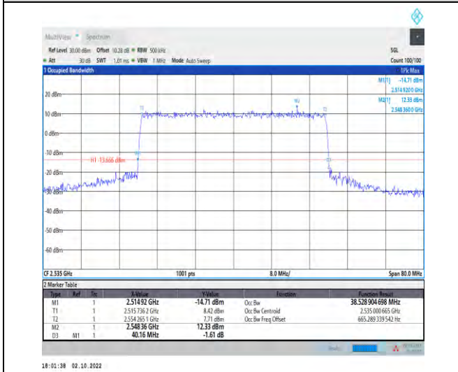
1-N7--15-40-M-8-CP-64QAM-Outer_Full-216@0-Ant 1-38.529-40.160-≤40-PASS
