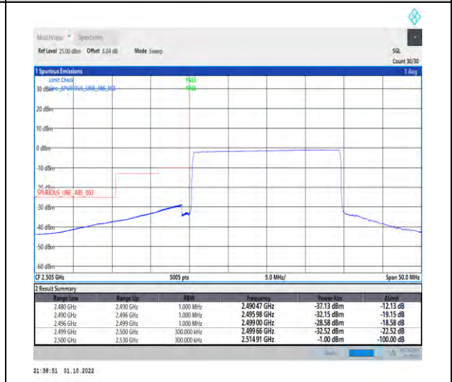
1-N7--15-20-L-6-CP-QPSK-Outer_Full-106@0-Ant1-1--PASS-see graph
