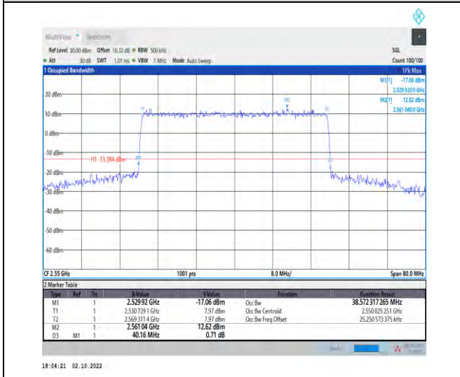
1-N7--15-40-H-7-CP-16QAM-Outer_Full-216@0-Ant 1-38.572-40.160-≤40-PASS
