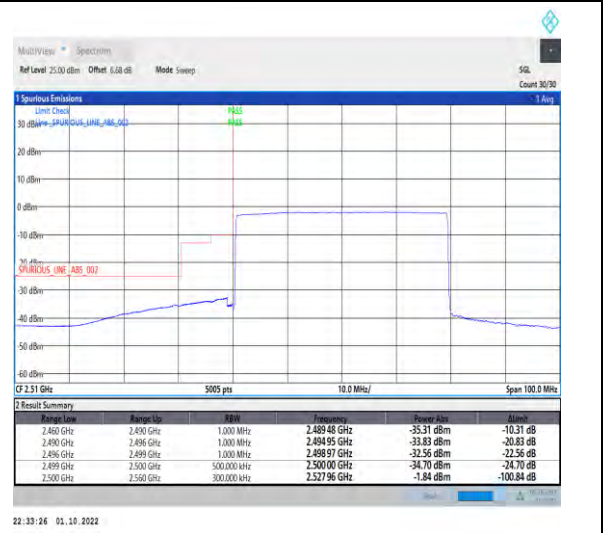
1-N7--15-40-L-6-CP-QPSK-Outer_Full-216@0-Ant1-1--PASS-see graph
