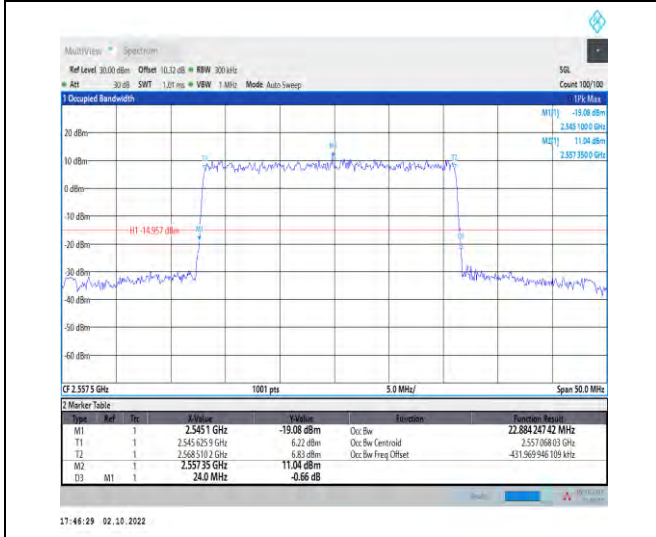
1-N7--15-25-H-5-DFT-256QAM-Outer_Full-128@0-A nt1-22.884-24.000-<25-PASS
