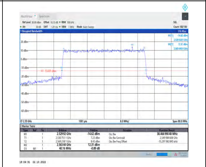
1-N7--15-40-H-8-CP-64QAM-Outer_Full-216@0-Ant 1-38.467-40.160-≤40-PASS
