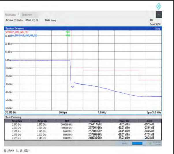
1-N7--15-30-H-6-CP-QPSK-Outer_Full-160@0-Ant1-1--PASS-see graph
