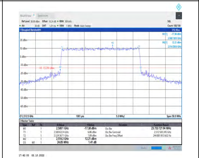
1-N7--15-25-L-8-CP-64QAM-Outer_Full-133@0-Ant 1-23.734-24.850-≤25-PASS
