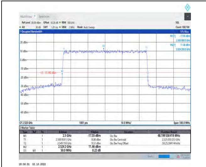
1-N7--15-50-L-4-DFT-64QAM-Outer_Full-270@0-Ant 1-48.2-50.000-≤50-PASS
