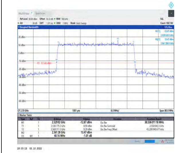
1-N7--15-40-H-3-DFT-16QAM-Outer_Full-216@0-Ant t1-38.536-40.160-≤40-PASS
