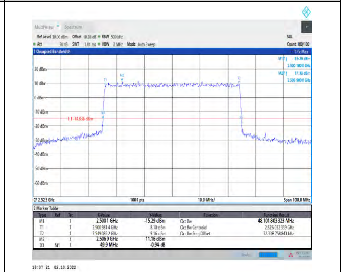
1-N7--15-50-L-7-CP-16QAM-Outer_Full-270@0-Ant 1-48.102-49.900-≤50-PASS
