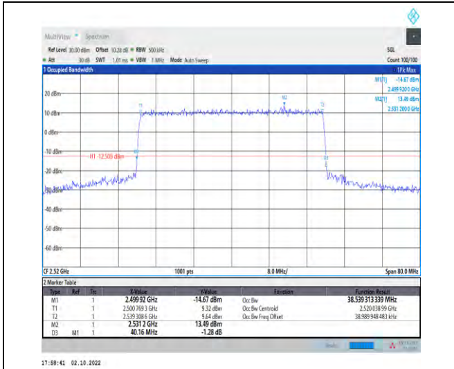
1-N7--15-40-L-7-CP-16QAM-Outer_Full-216@0-Ant 1-38.539-40.160-≤40-PASS
