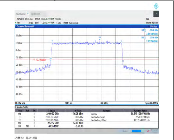
1-N7--15-40-L-8-CP-64QAM-Outer_Full-216@0-Ant 1-38.545-40.160-≤40-PASS
