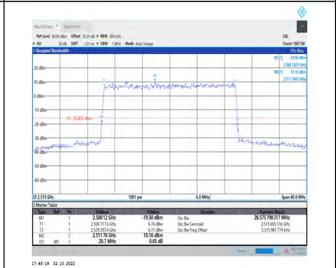
1-N7--15-30-L-5-DFT-256QAM-Outer_Full-160@0-A nt1-28.576-29.700-≤30-PASS
