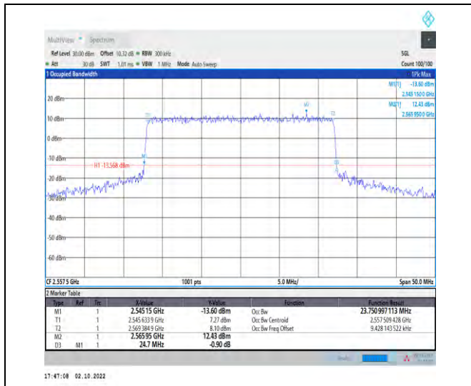
1-N7--15-25-H-7-CP-16QAM-Outer_Full-133@0-Ant 1-23.751-24.700-≤25-PASS
