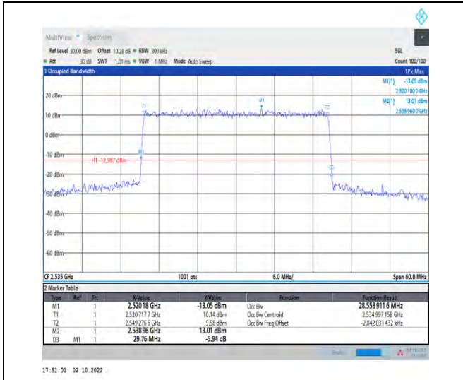
1-N7--15-30-M-1-DFT-QPSK-Outer_Full-160@0-Ant t1-28.559-29.760-≤30-PASS
