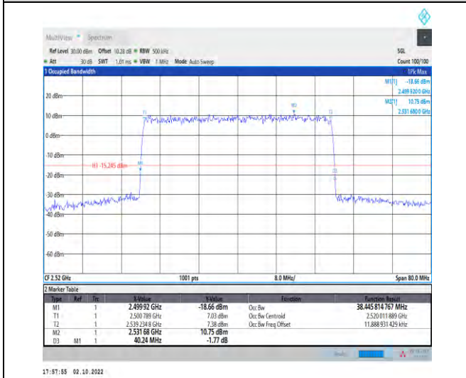
1-N7--15-40-L-5-DFT-256QAM-Outer_Full-216@0-A nt1-38.446-40.240-≤40-PASS
