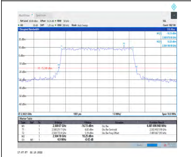
1-N7--15-5-L-7-CP-16QAM-Outer_Full-25@0-Ant1-4 .482-4.900-≤5-PASS
