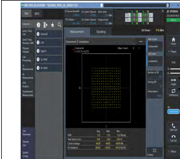
1-N7-PC3-15-50-M-9-CP-256QAM-Outer_Full-270@0-Ant1-see graph-PASS
