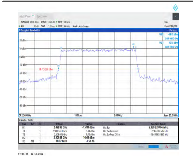
1-N7--15-10-L-8-CP-64QAM-Outer_Full-52@0-Ant1- 9.321-10.020-≤10-PASS
