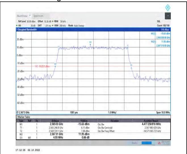
1-N7--15-5-H-4-DFT-64QAM-Outer_Full-25@0-Ant1- 4.477-4.930-≤5-PASS
