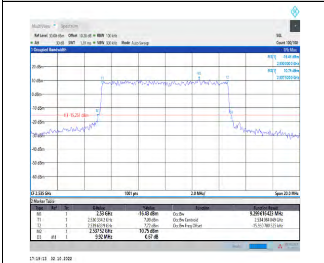
1-N7--15-10-M-7-CP-16QAM-Outer_Full-52@0-Ant1 -9.3-9.920-≤10-PASS
