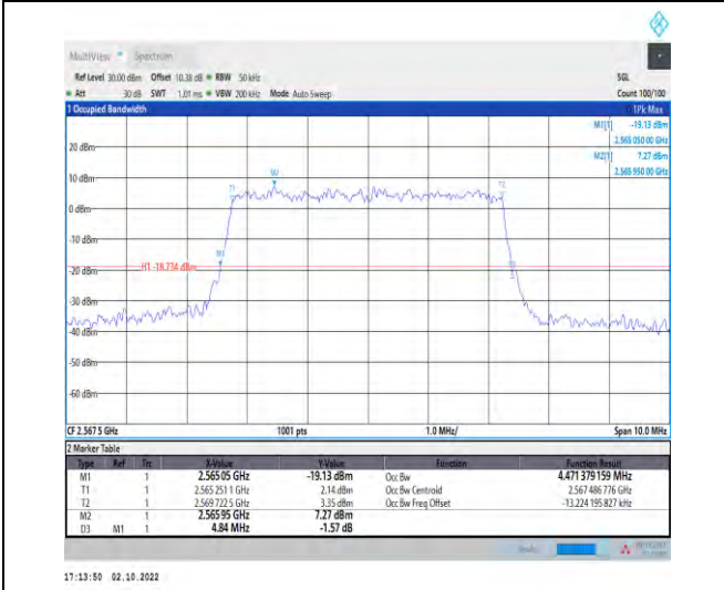
1-N7--15-5-H-9-CP-256QAM-Outer_Full-25@0-Ant1-4 4.471-4.840-≤5-PASS
