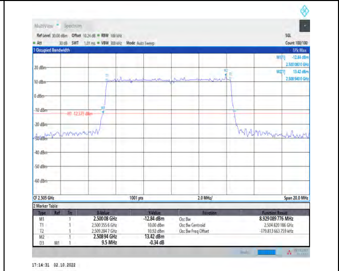
1-N7--15-10-L-1-DFT-QPSK-Outer_Full-50@0-Ant1- 8.929-9.500-≤10-PASS
