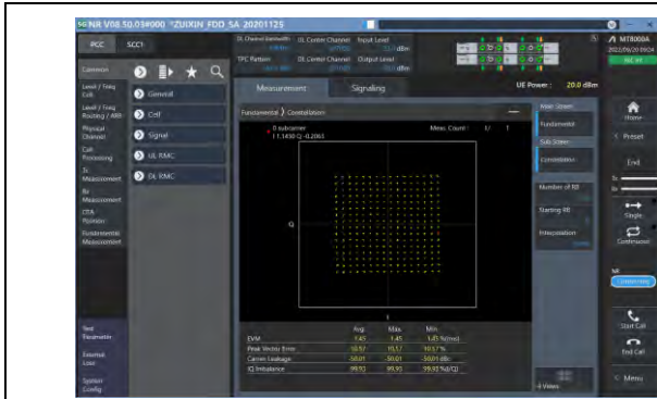
1-N7-PC3-15-50-M-5-DFT-256QAM-Outer_Full-270@0-Ant1-see graph-PASS
