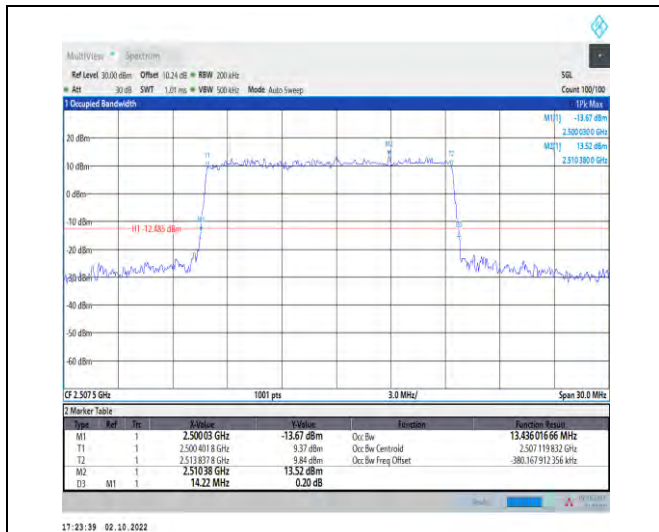
1-N7--15-15-L-3-DFT-16QAM-Outer_Full-75@0-Ant1 -13.436-14.220-≤15-PASS
