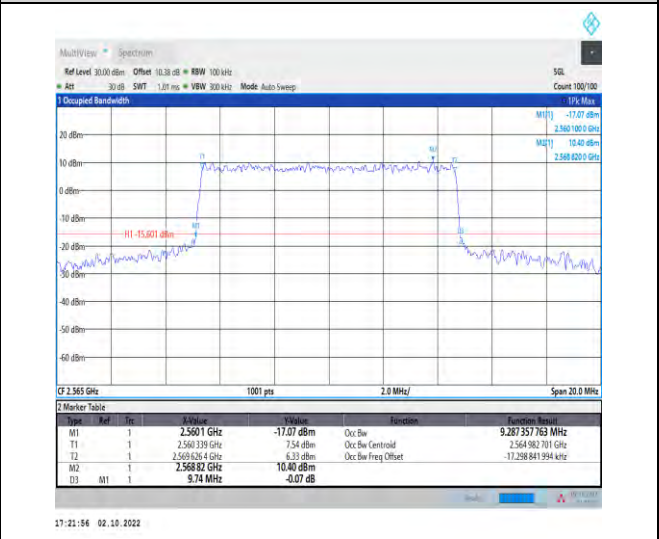
1-N7--15-10-H-7-CP-16QAM-Outer_Full-52@0-Ant1- 9.287-9.740≤10-PASS
