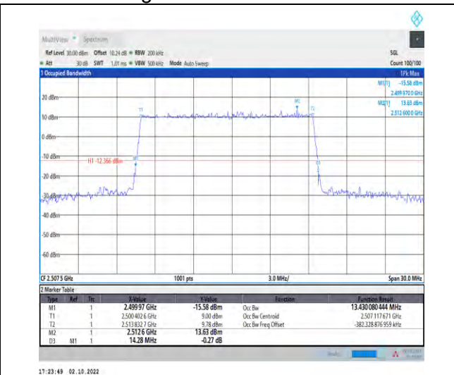
1-N7--15-15-L-4-DFT-64QAM-Outer_Full-75@0-Ant1 -13.43-14.280-≤15-PASS
