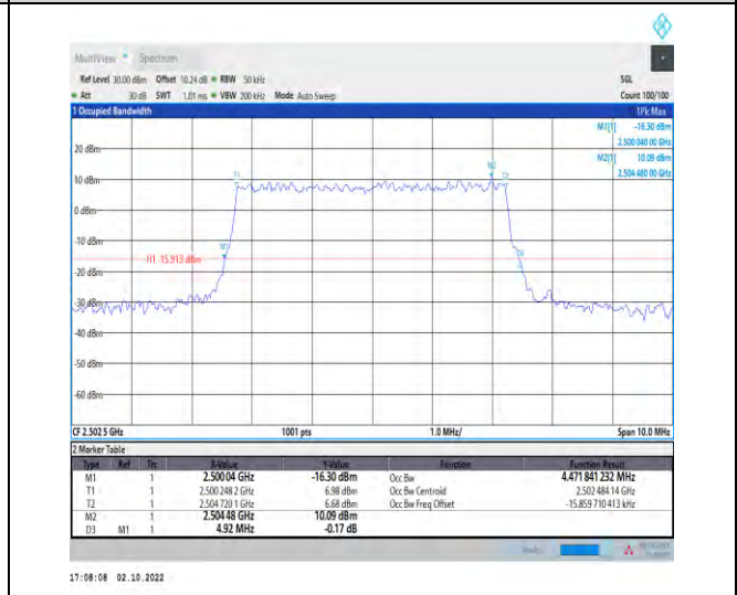
1-N7--15-5-L-8-CP-64QAM-Outer_Full-25@0-Ant1-4 .472-4.920-≤5-PASS
