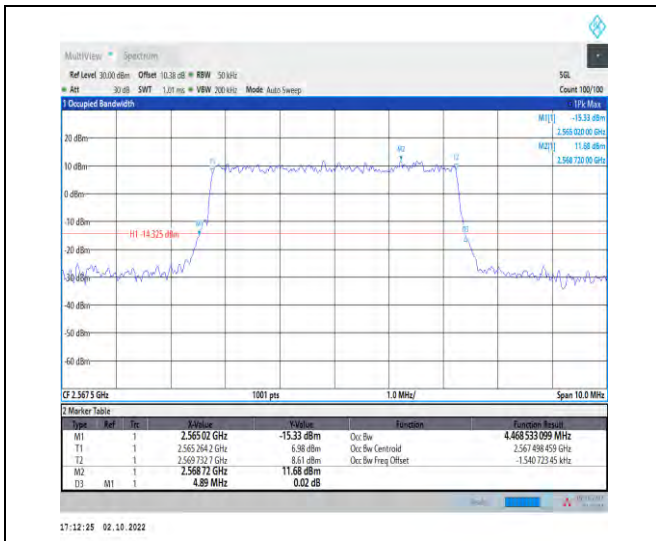
1-N7--15-5-H-3-DFT-16QAM-Outer_Full-25@0-Ant1- 4.469-4.890-≤5-PASS
