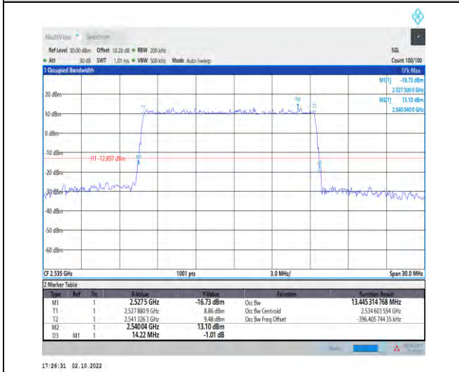
1-N7--15-15-M-4-DFT-64QAM-Outer_Full-75@0-Ant 1-13.445-14.220-≤15-PASS
