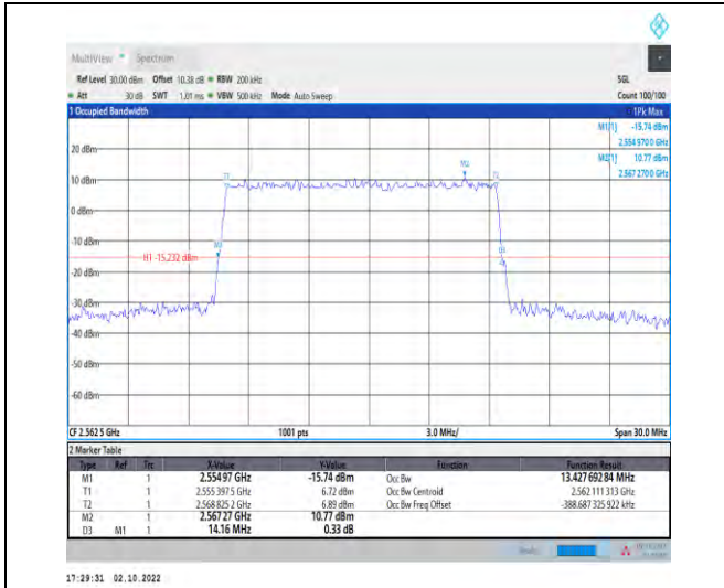
1-N7--15-15-H-5-DFT-256QAM-Outer_Full-75@0-Ant1-t1-13.428-14.160-<=15-PASS
