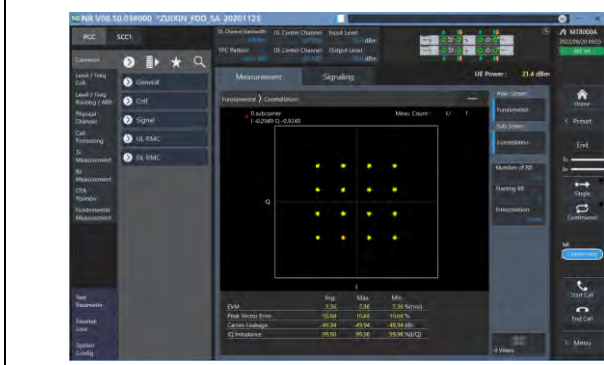
1-N7-PC3-15-50-M-7-CP-16QAM-Outer_Full-270@0-Ant1-see graph-PASS
