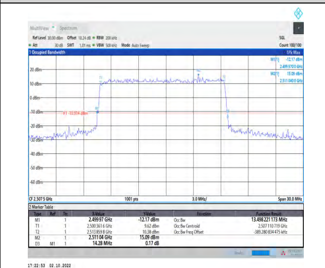
1-N7--15-15-L-6-CP-QPSK-Outer_Full-79@0-Ant1-2 9.667-30.000-≤15-PASS
