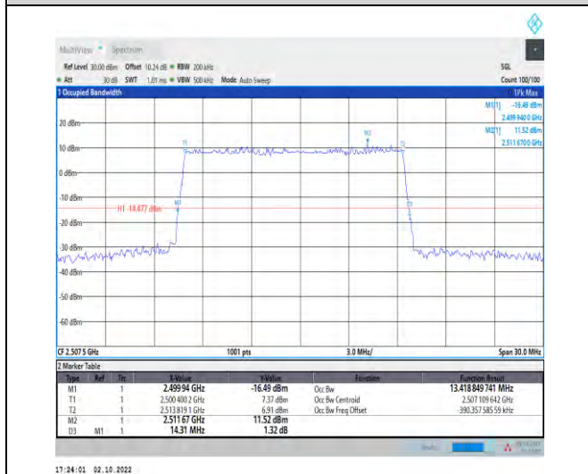
1-N7--15-15-L-5-DFT-256QAM-Outer_Full-75@0-Ant 1-13.419-14.310-≤15-PASS
