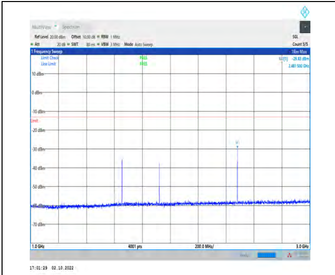
1-N5-PC3-15-20-M-1-DFT-PI2BPSK-Inner_1RB_Left -1@1-1000-3000-Ant1-2481.50--29.83--13-PASS
