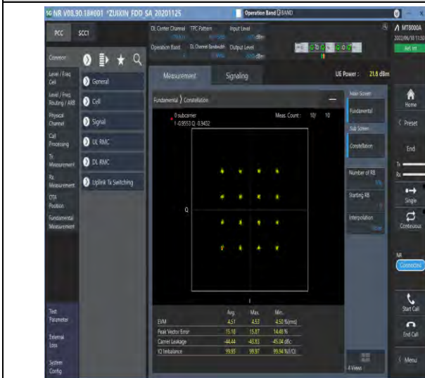
1-N5--15-20-M-7-CP-16QAM-Outer_Full-106@0-Ant1-see graph-PASS
