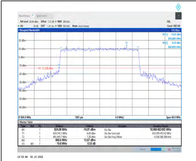
1-N5-PC3-15-20-L-8-CP-64QAM-Outer_Full-106@0-Ant1-18.9-19.800-<math>\leq 20</math>-PASS
