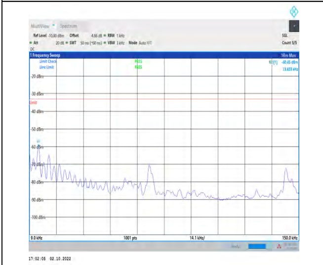
1-N5-PC3-15-20-H-1-DFT-PI2BPSK-Inner_1RB_Left -1@1-0.009-0.15-Ant1-0.01--60.45--33-PASS
