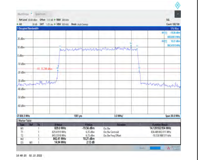
1-N5-PC3-15-15-M-9-CP-256QAM-Outer_Full-79@0-A Ant1-14.14-14.940-≤15-PASS
