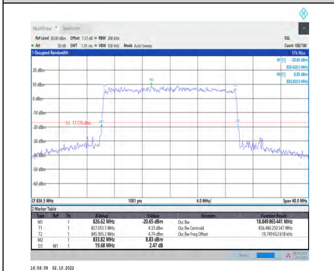
1-N5-PC3-15-20-M-9-CP-256QAM-Outer_Full-106@0 -Ant1-18.85-19.680-≤20-PASS
