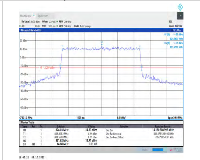
1-N5-PC3-15-15-L-8-CP-64QAM-Outer_Full-79@0-Ant1-14.151-14.880-≤15-PASS
