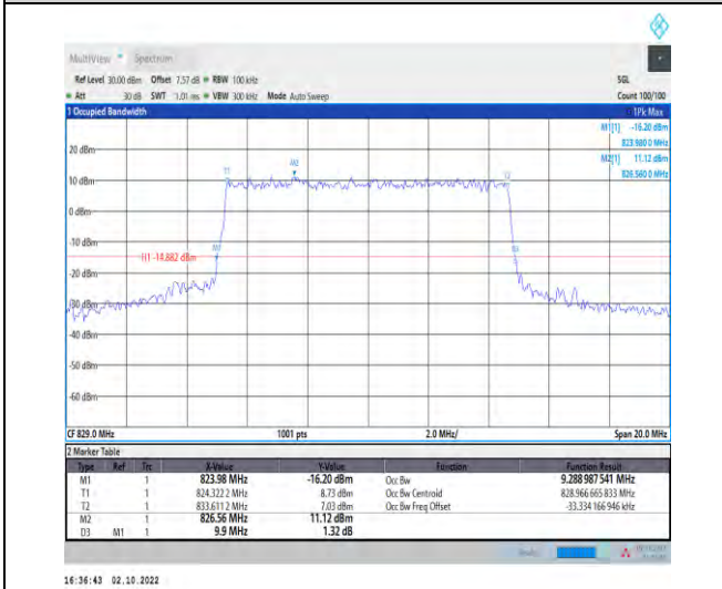
1-N5-PC3-15-10-L-8-CP-64QAM-Outer_Full-52@0-A Ant1-9.289-9.900-≤10-PASS
