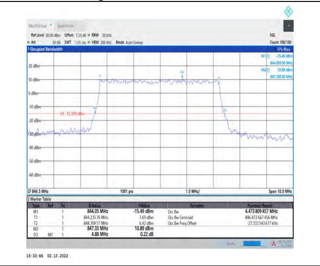
1-N5-PC3-15-5-H-8-CP-64QAM-Outer_Full-25@0-A nt1-4.474-4.880-≤5-PASS
