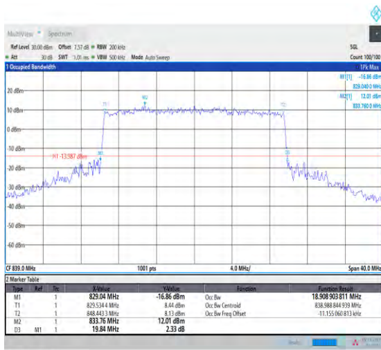
1-N5-PC3-15-20-H-6-CP-QPSK-Outer_Full-106@0-Ant1-39.667-40.000-≤20-FAIL
