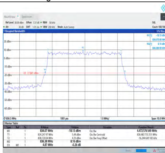
1-N5-PC3-15-5-M-9-CP-256QAM-Outer_Full-25@0-A nt1-4.473-4.870-<math>\leq</math>5-PASS
