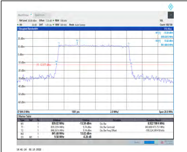
1-N5-PC3-15-10-H-4-DFT-64QAM-Outer_Full-50@0 -Ant1-8.922-9.580-≤10-PASS
