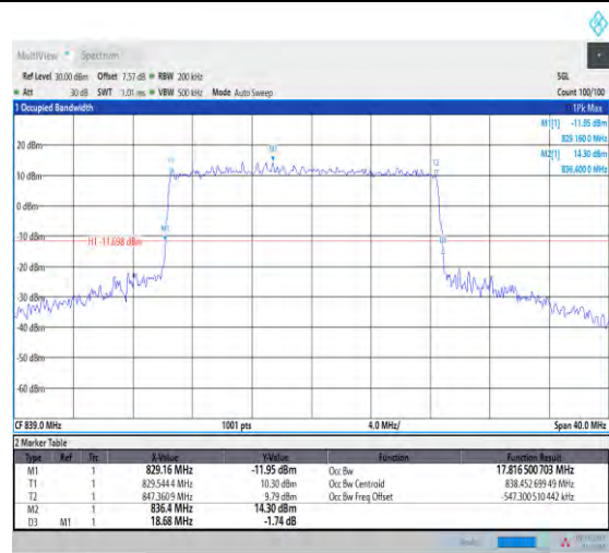
1-N5-PC3-15-20-H-3-DFT-16QAM-Outer_Full-100 @0-Ant1-17.817-18.680-≤20-PASS
