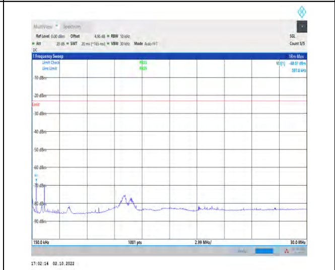
1-N5-PC3-15-20-H-1-DFT-PI2BPSK-Inner_1RB_Left -1@1-0.15-30-Ant1-0.60--68.07--23-PASS
