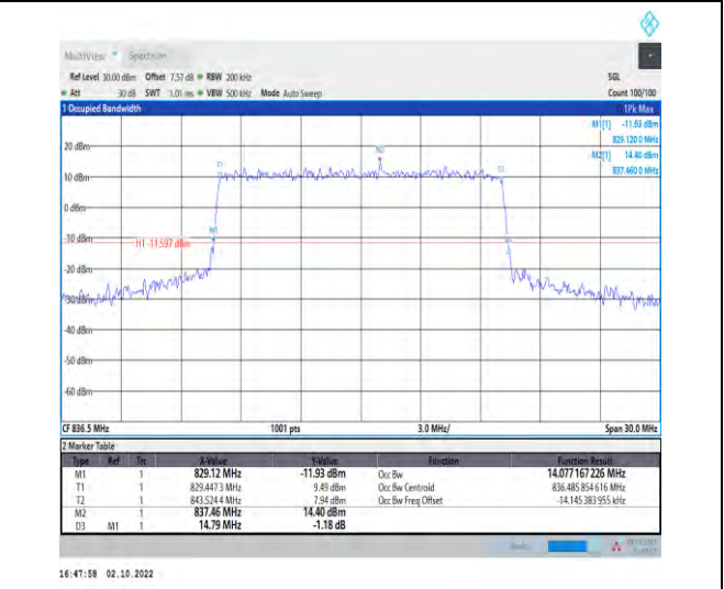
1-N5-PC3-15-15-M-7-CP-16QAM-Outer_Full-79@0-A Ant1-14.077-14.790-≤15-PASS
