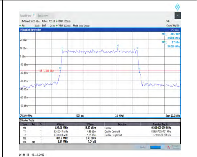
1-N5-PC3-15-10-L-9-CP-256QAM-Outer_Full-52@0-A Ant1-9.306-9.840-≤10-PASS
