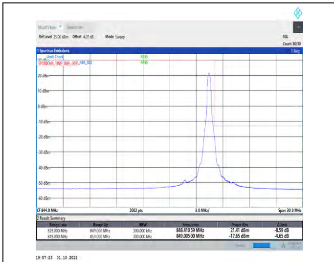
1-N5-PC3-15-20-H-2-DFT-PI2BPSK-Edge_1RB_Right-1@105-Ant1-1-seegraph-PASS-see graph
