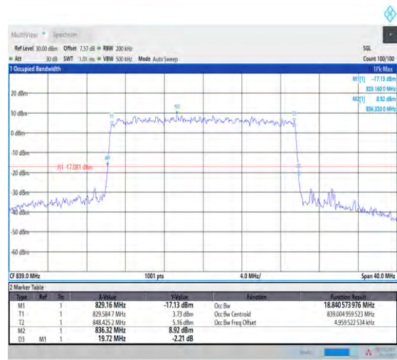
1-N5-PC3-15-20-H-7-CP-16QAM-Outer_Full-106@0-Ant1-18.928-19.760-≤20-PASS
