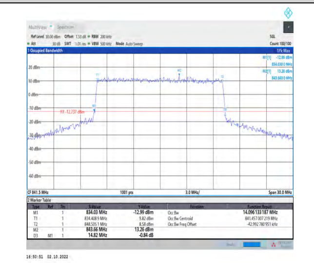
1-N5-PC3-15-15-H-8-CP-64QAM-Outer_Full-79@0- Ant1-14.096-14.820-≤15-PASS
