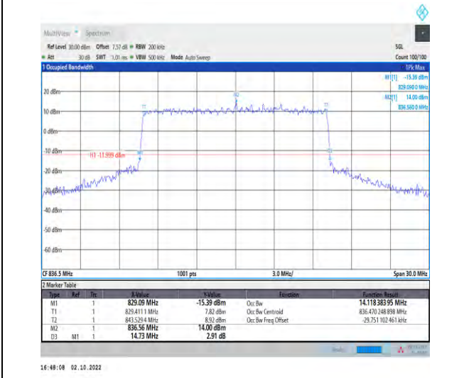
1-N5-PC3-15-15-M-8-CP-64QAM-Outer_Full-79@0-A Ant1-14.118-14.730-≤15-PASS
