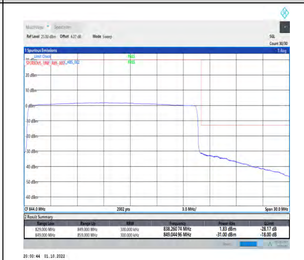
1-N5-PC3-15-20-H-6-CP-QPSK-Outer_Full-106@0-Ant1-1-seegraph-PASS-see graph
