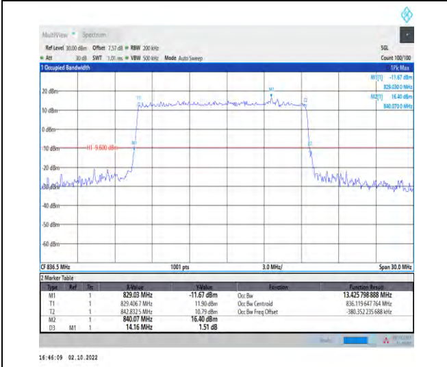
1-N5-PC3-15-15-M-6-CP-QPSK-Outer_Full-79@0-A Ant1-29.686-30.000-≤15-FAIL
