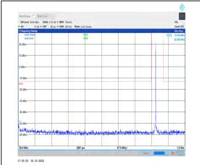
1-N5-PC3-15-20-H-1-DFT-PI2BPSK-Inner_1RB_Left -1@1-30-1000-Ant1-32.43--51.56--13-PASS
