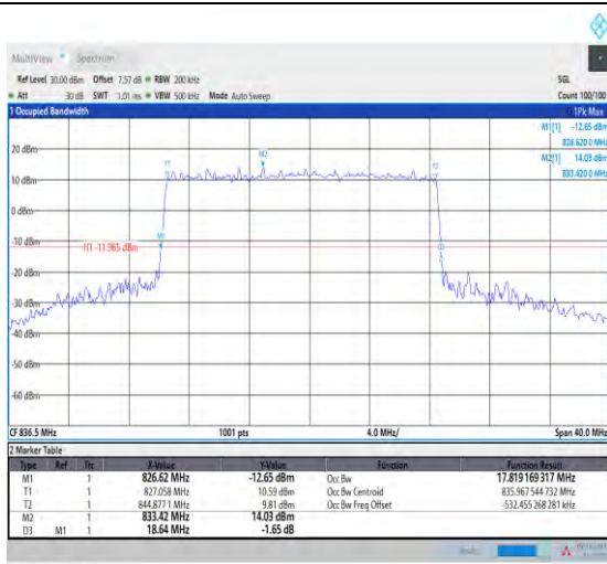
1-N5-PC3-15-20-M-3-DFT-16QAM-Outer_Full-100@ 0-Ant1-17.819-18.640-≤20-PASS
