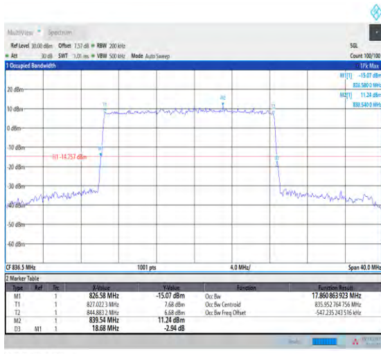
1-N5-PC3-15-20-M-5-DFT-256QAM-Outer_Full-100 @0-Ant1-17.861-18.680-≤20-PASS
