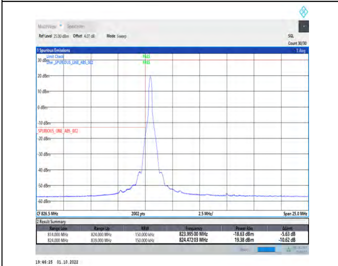
1-N5-PC3-15-15-L-4-CP-QPSK-Edge_1RB_Left-1@0-Ant1-1-seegraph-PASS-see graph
