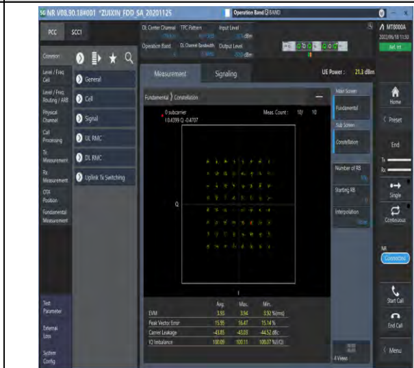
1-N5--15-20-M-8-CP-64QAM-Outer_Full-106@0-Ant1-see graph-PASS
