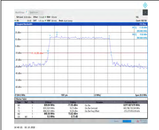
1-N5-PC3-15-10-H-6-CP-QPSK-Outer_Full-52@0-A nt1-19.794-20.000-≤10-FAIL
