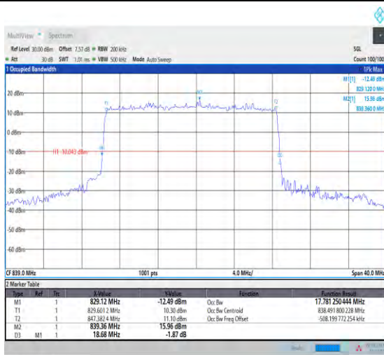
1-N5-PC3-15-20-H-2-DFT-PI2BPSK-Outer_Full-100 @0-Ant1-17.781-18.680-≤20-PASS
