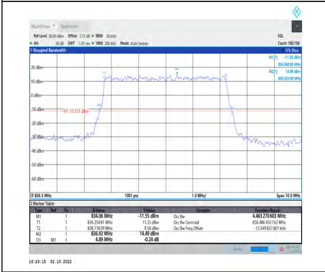
1-N5-PC3-15-5-M-2-DFT-PI2BPSK-Outer_Full-25@0-Ant1-4.463-4.890-≤5-PASS
