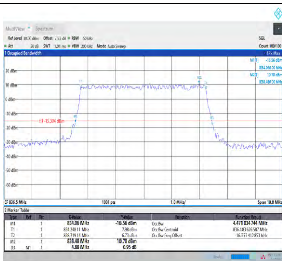
1-N5-PC3-15-5-M-8-CP-64QAM-Outer_Full-25@0-A nt1-4.471-4.880-<math>\leq</math>5-PASS
