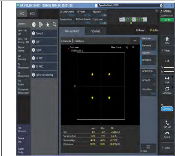
1-N5--15-20-M-6-CP-QPSK-Outer_Full-106@0-Ant1-see graph-PASS
