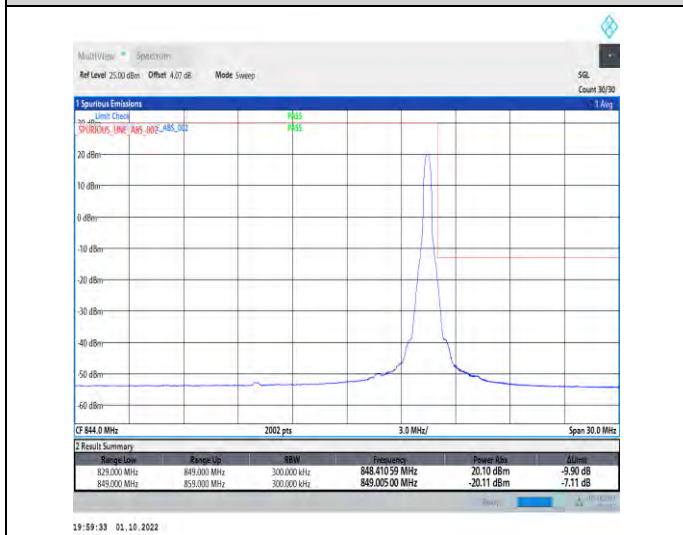
1-N5-PC3-15-20-H-5-CP-QPSK-Edge_1RB_Right-1@105-Ant1-1-seegraph-PASS-see graph
