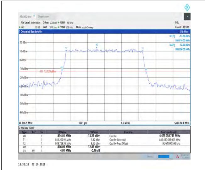
1-N5-PC3-15-5-H-3-DFT-16QAM-Outer_Full-25@0-Ant1-4.475-4.910-≤5-PASS
