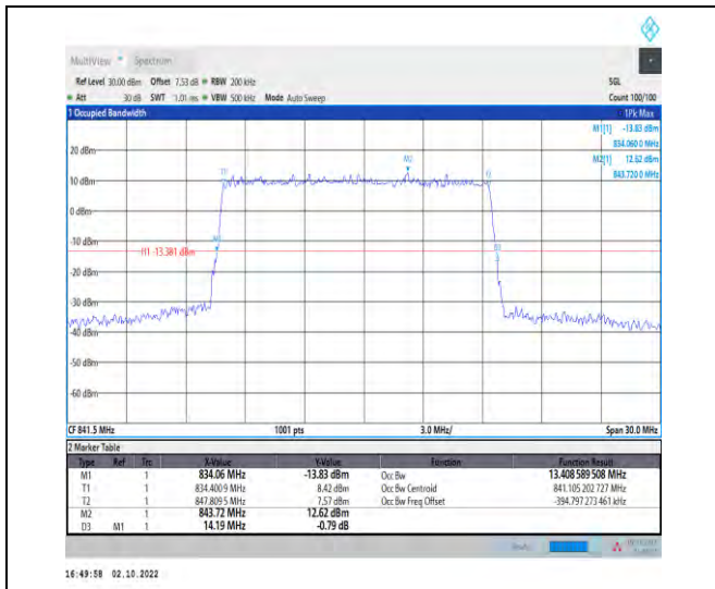
1-N5-PC3-15-15-H-5-DFT-256QAM-Outer_Full-75@ 0-Ant1-13.409-14.190-≤15-PASS
