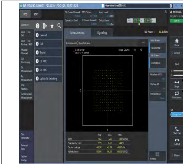
1-N5--15-20-M-5-DFT-256QAM-Outer_Full-100@0-Ant1-see graph-PASS
