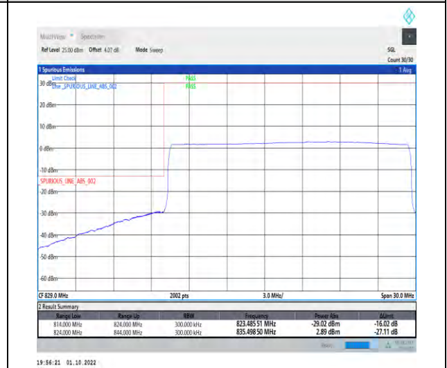
1-N5-PC3-15-20-L-6-CP-QPSK-Outer_Full-106@0-Ant1-1-seegraph-PASS-see graph
