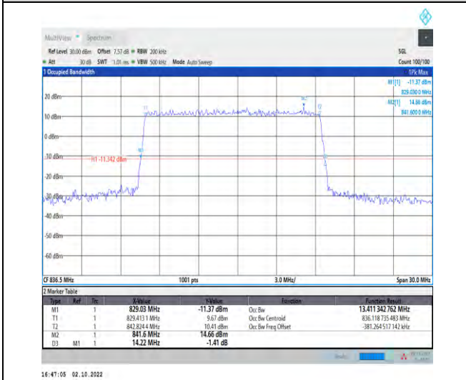
1-N5-PC3-15-15-M-4-DFT-64QAM-Outer_Full-75@0-Ant1-13.411-14.220-≤15-PASS
