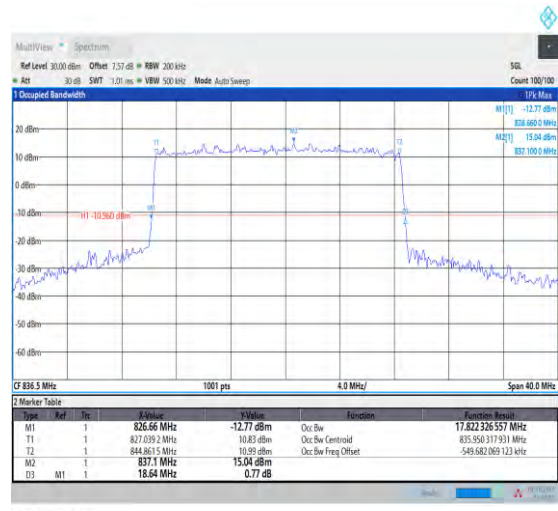
1-N5-PC3-15-20-M-6-CP-QPSK-Outer_Full-106@0- Ant1-39.615-40.000-≤20-FAIL
