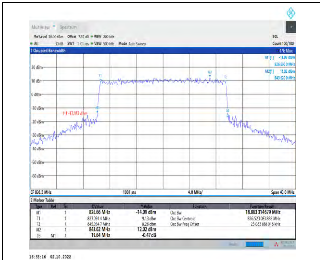
1-N5-PC3-15-20-M-7-CP-16QAM-Outer_Full-106@0 -Ant1-18.863-19.640-≤20-PASS
