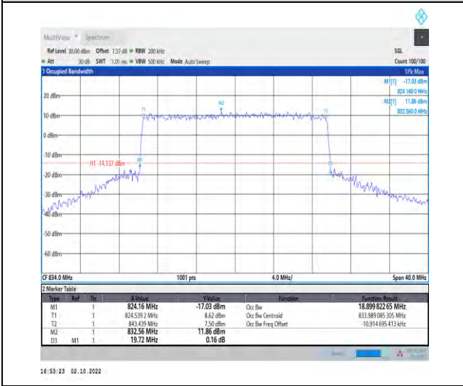
1-N5-PC3-15-20-L-6-CP-QPSK-Outer_Full-106@0-Ant1-18.9-19.720-≤20-PASS
