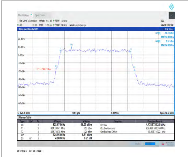
1-N5-PC3-15-5-L-9-CP-256QAM-Outer_Full-25@0-Ant1-4.478-4.980-≤5-PASS
