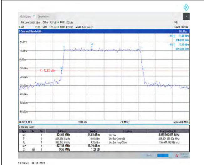
1-N5-PC3-15-10-L-4-DFT-64QAM-Outer_Full-50@0-Ant1-8.936-9.560-≤10-PASS
