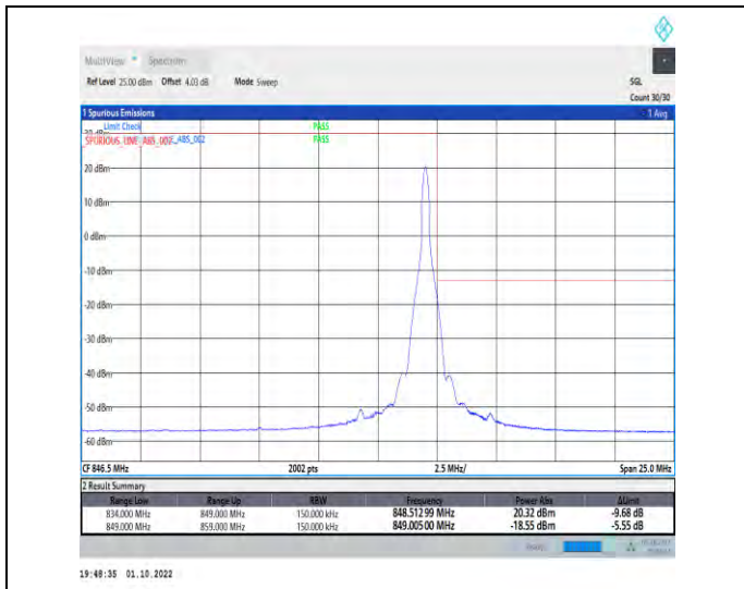
1-N5-PC3-15-15-H-2-DFT-PI2BPSK-Edge_1RB_Right-1@78-Ant1-1-seegraph-PASS-see graph
