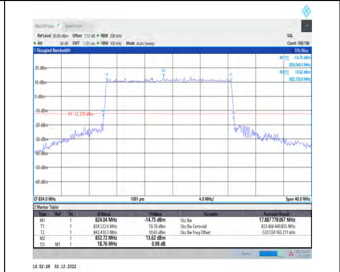
1-N5-PC3-15-20-L-3-DFT-16QAM-Outer_Full-100@ 0-Ant1-17.888-18.760-≤20-PASS
