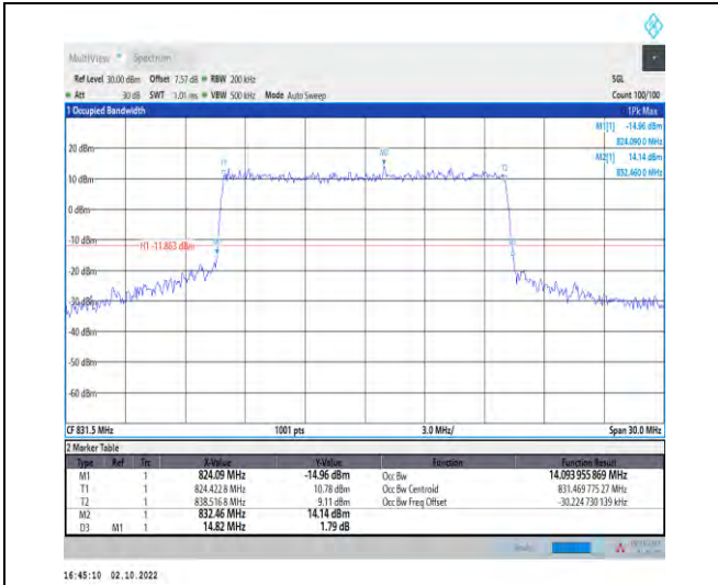
1-N5-PC3-15-15-L-7-CP-16QAM-Outer_Full-79@0-Ant1-14.094-14.820-≤15-PASS
