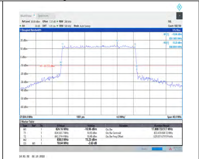
1-N5-PC3-15-20-L-1-DFT-QPSK-Outer_Full-100@0- Ant1-17.809-18.640-≤20-PASS
