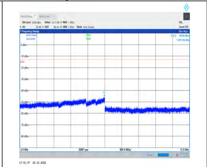
1-N5-PC3-15-20-M-1-DFT-PI2BPSK-Inner_1RB_Left -1@1-3000-12000-Ant1-7476.15--45.04--13-PASS
