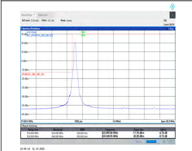
1-N5-PC3-15-20-L-4-CP-QPSK-Edge_1RB_Left-1@0-Ant1-1-seegraph-PASS-see graph
