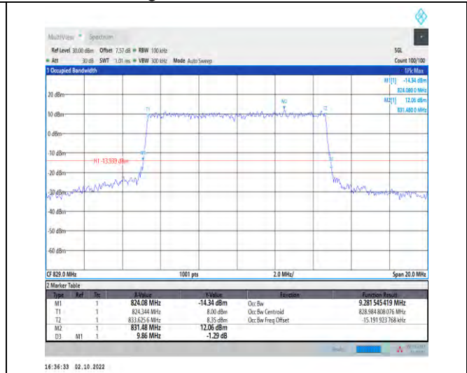
1-N5-PC3-15-10-L-7-CP-16QAM-Outer_Full-52@0-A nt1-9.282-9.860-≤10-PASS
