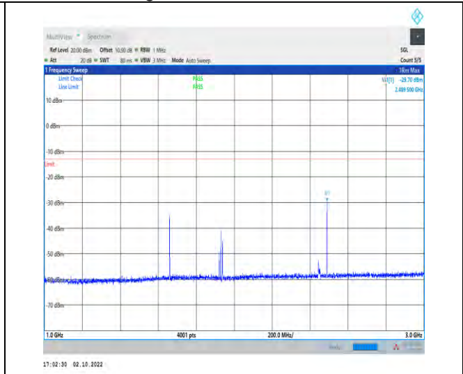
1-N5-PC3-15-20-H-1-DFT-PI2BPSK-Inner_1RB_Left -1@1-1000-3000-Ant1-2489.50--29.70--13-PASS
