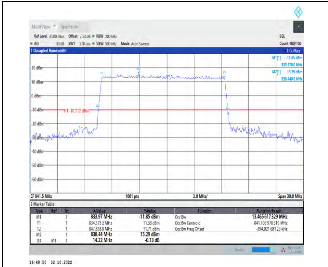
1-N5-PC3-15-15-H-1-DFT-QPSK-Outer_Full-75@0-Ant1-13.466-14.220-≤15-PASS
