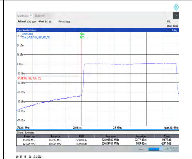
1-N5-PC3-15-15-L-6-CP-QPSK-Outer_Full-79@0-Ant1-1-seegraph-PASS-see graph
