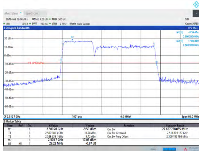
7-7-10MHz-20MHz-QPSK-QPSK-20805-20949-50RB#0-100RB#0
