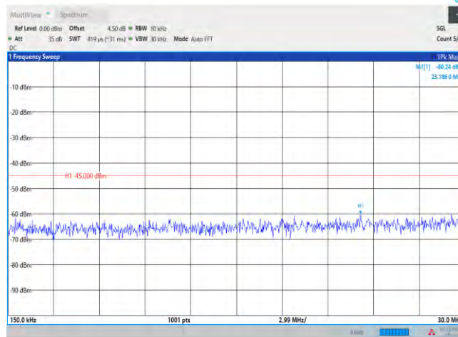
7-7-20MHz-20MHz-QPSK-QPSK-20850-21048-1RB#0-0RB#0-0.15~30MHz
