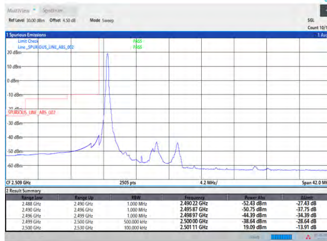
7-7-10MHz-20MHz-QPSK-QPSK-20805-20949-50RB#0-100RB#0
