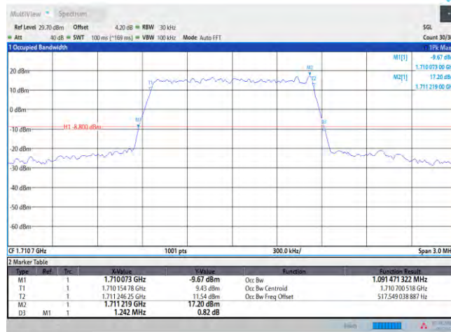
Band66-1.4MHz-QPSK-132272-6RB#0
