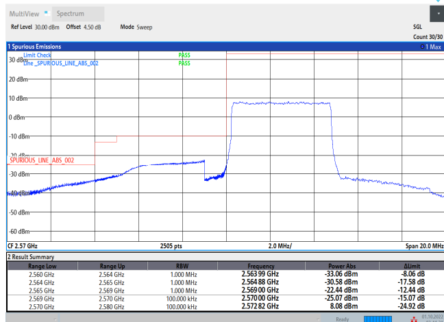
Band38-5MHz-QPSK-37775-25RB#0
