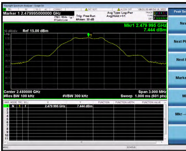
GFSK (BLE 1Mbps) HIGH CHANNEL, CARRIER LEVEL
