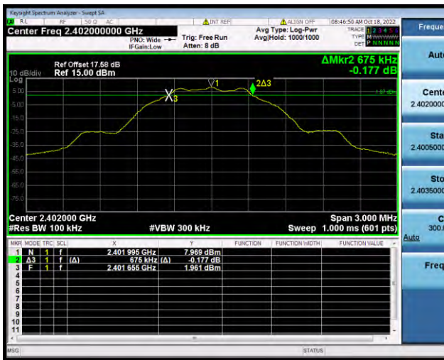
GFSK (BLE 1Mbps) LOW CHANNEL
