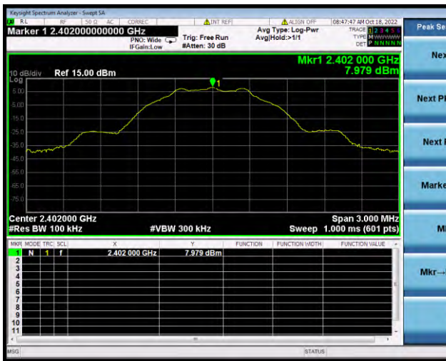
GFSK (BLE 1Mbps) LOW CHANNEL, CARRIER LEVEL
