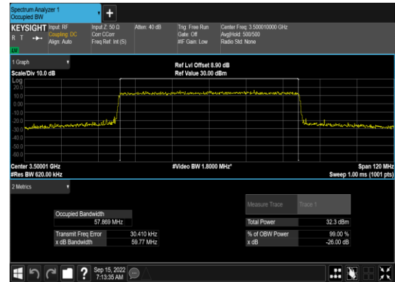
N78(60M)_DFT-s- OFDM_QPSK_Outer_Full_Mid_CH
