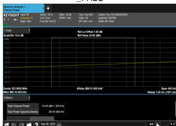
N5(20M)_DFT-s-OFDM_BPSK_Edge_1RB_Left_Low_CH_CHP_PASS
