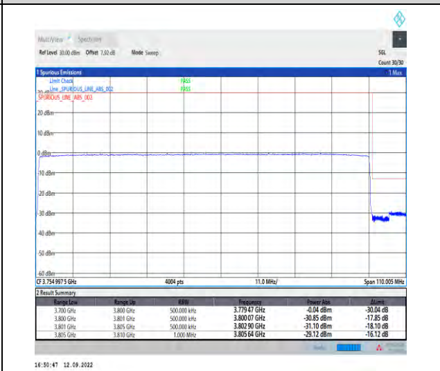
1-N78-3700-3800--30-100-H-6-CP-QPSK-Outer_F ull-273@0-Ant1-1--PASS-see graph
