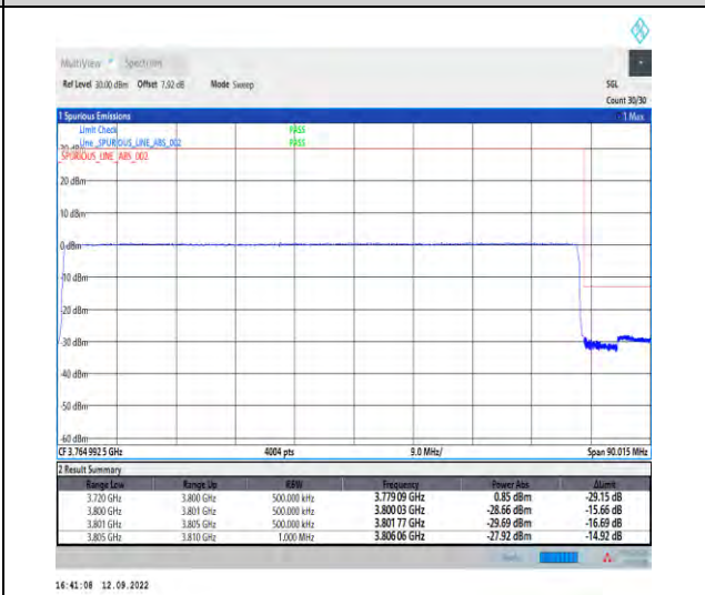
1-N78-3700-3800--30-80-H-6-CP-QPSK-Outer_Ful l-217@0-Ant1-1--PASS-see graph
