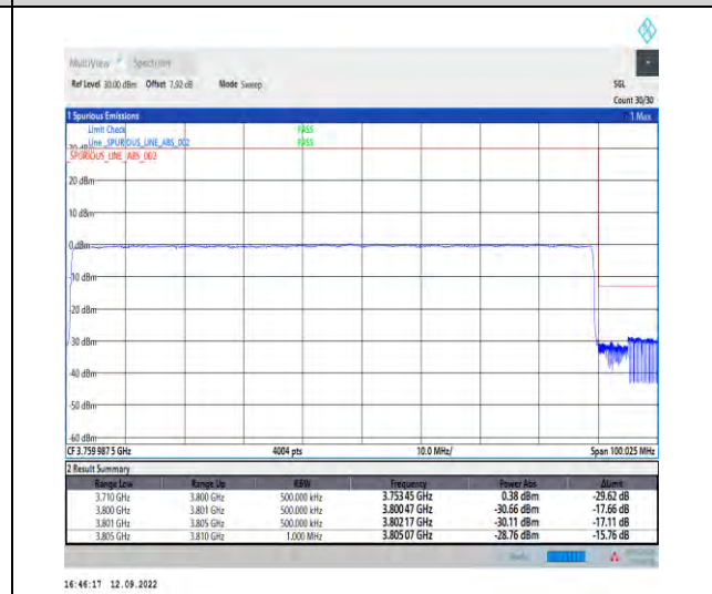
1-N78-3700-3800--30-90-H-6-CP-QPSK-Outer_Ful l-245@0-Ant1-1--PASS-see graph
