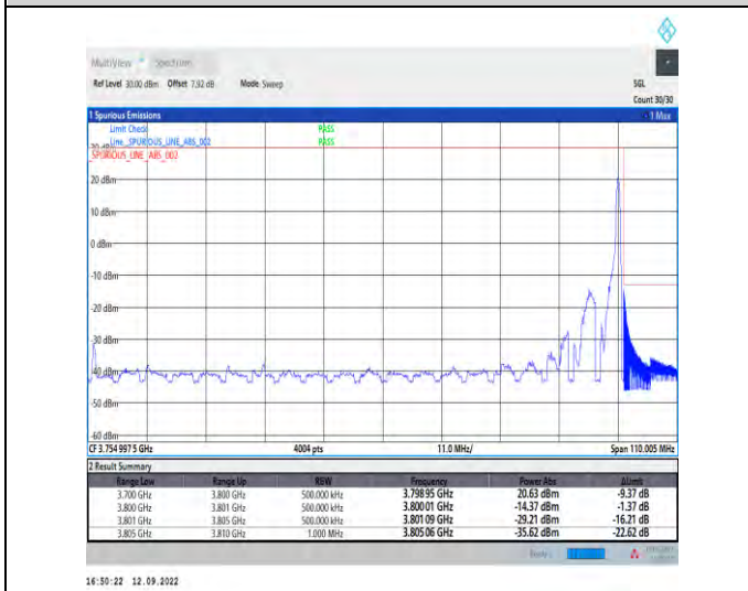
1-N78-3700-3800--30-100-H-5-CP-QPSK-Edge_1RB_ Right-1@272-Ant1-1--PASS-see graph
