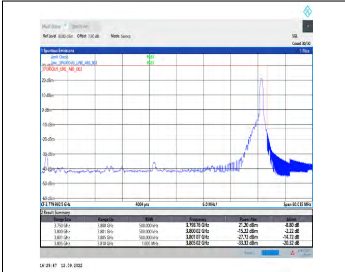
1-N78-3700-3800--30-50-H-2-DFT-PI2BPSK-Edge_1R B_Right-1@132-Ant1-1--PASS-see graph
