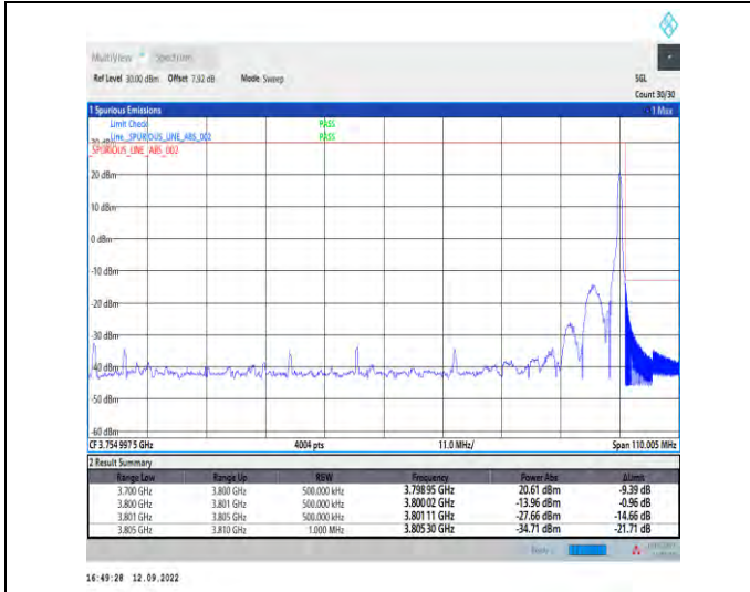
1-N78-3700-3800--30-100-H-2-DFT-PI2BPSK-Edge_1 RB_Right-1@272-Ant1-1--PASS-see graph
