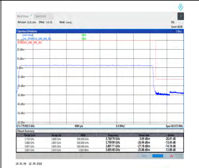
1-N78-3700-3800--30-50-H-6-CP-QPSK-Outer_Ful l-133@0-Ant1-1--PASS-see graph
