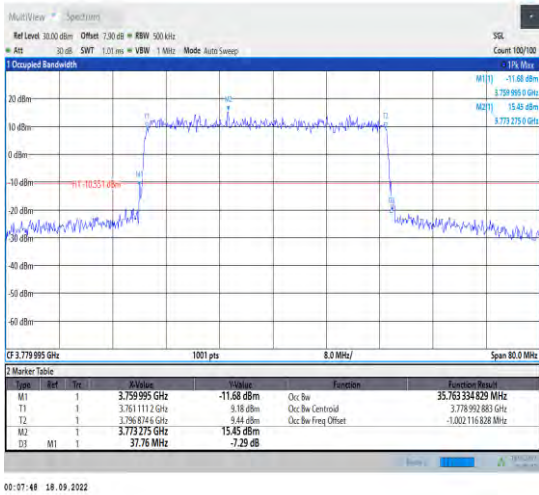
1-N78-3700-3800--30-40-H-1-DFT-QPSK-Outer_Full -100@0-Ant1-35.763-37.760-<40-PASS
