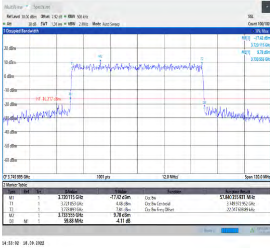
1-N78-3700-3800--30-60-M-8-CP-64QAM-Outer_Full-162@0-Ant1-57.84-59.880-≤60-PASS
