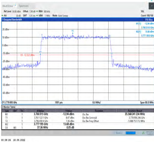
1-N78-3700-3800--30-40-H-3-DFT-16QAM-Outer_Fu II-100@0-Ant1-35.568-37.360-<40-PASS
