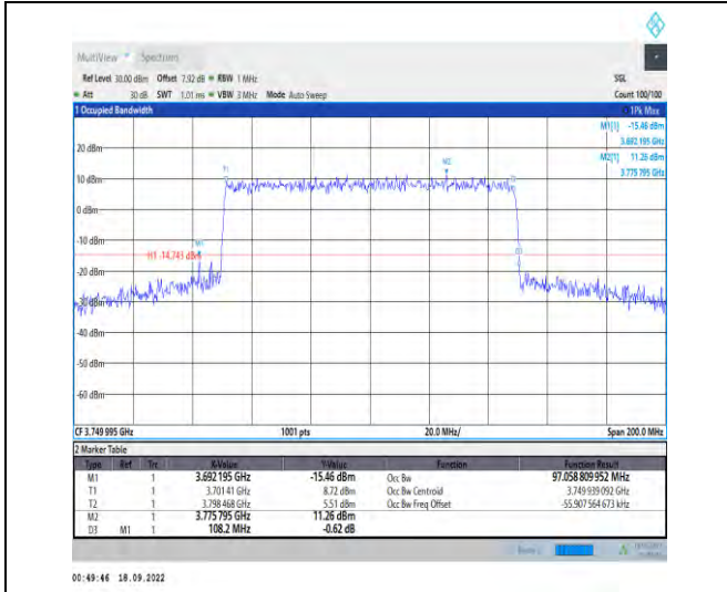
1-N78-3700-3800--30-100-M-7-CP-16QAM-Outer_Full-273@0-Ant1-97.059-108.200-≤100-PASS
