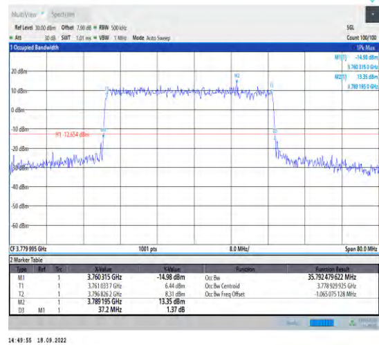
1-N78-3700-3800--30-40-H-4-DFT-64QAM-Outer_Fu II-100@0-Ant1-35.792-37.200-<40-PASS
