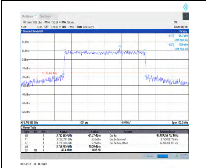
1-N78-3700-3800--30-50-M-7-CP-16QAM-Outer_Full I-133@0-Ant1-47.469-49.400-≤50-PASS
