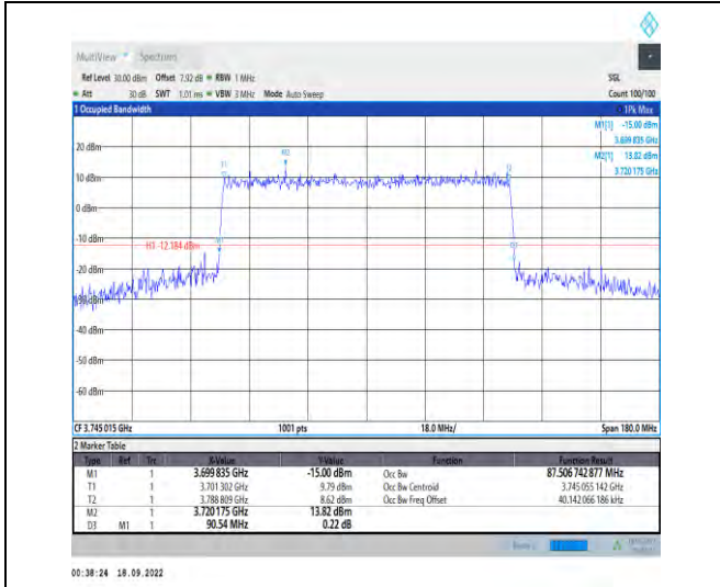
1-N78-3700-3800--30-90-L-7-CP-16QAM-Outer_Full -245@0-Ant1-87.507-90.540-≤90-PASS
