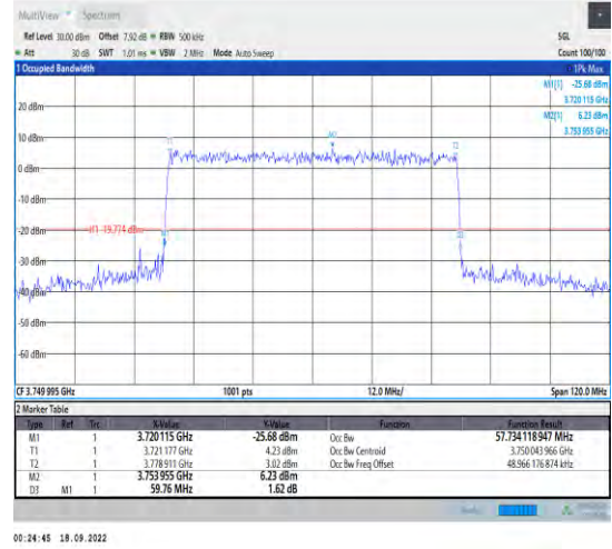
1-N78-3700-3800--30-60-M-9-CP-256QAM-Outer_Full-162@0-Ant1-57.734-59.760-≤60-PASS
