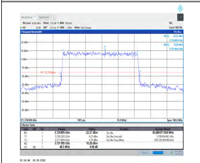
1-N78-3700-3800--30-50-M-5-DFT-256QAM-Outer_Full-128@0-Ant1-45.689-48.500-≤50-PASS
