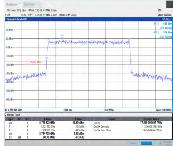
1-N78-3700-3800--30-80-H-9-CP-256QAM-Outer_Fu II-217@0-Ant1-77.36-80.320-<80-PASS
