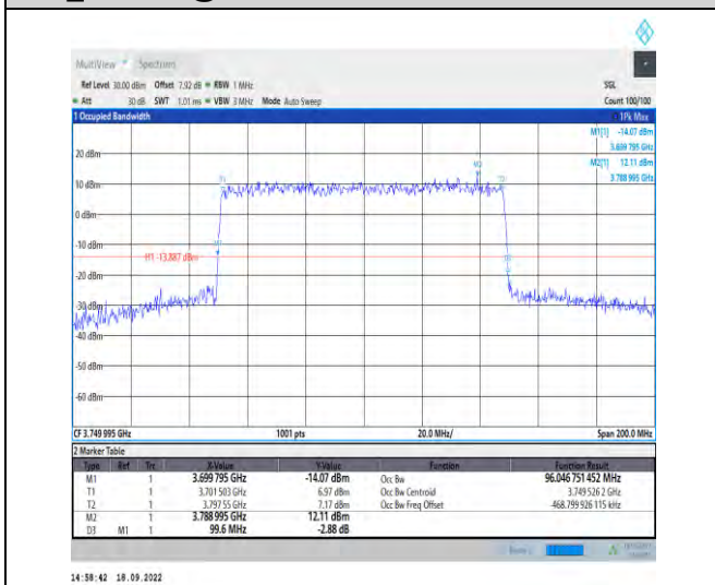
1-N78-3700-3800--30-100-H-4-DFT-64QAM-Outter_Full-270@0-Ant1-96.047-99.600-≤100-PASS
