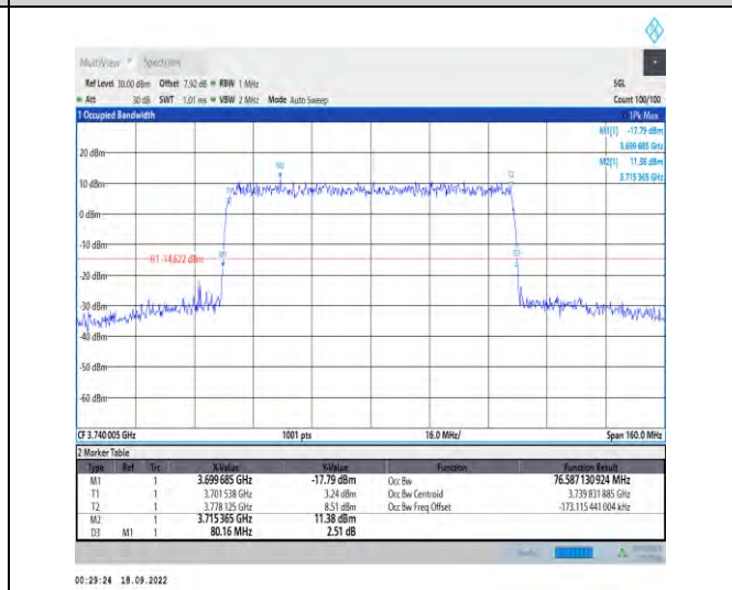
1-N78-3700-3800--30-80-L-5-DFT-256QAM-Outer_Full-216@0-Ant1-76.587-80.160-<80-PASS
