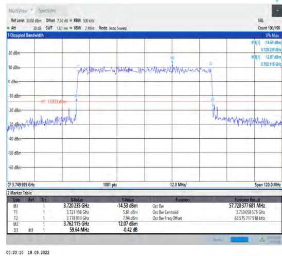
1-N78-3700-3800--30-60-M-3-DFT-16QAM-Outer_Full ull-162@0-Ant1-57.72-59.640-≤60-PASS
