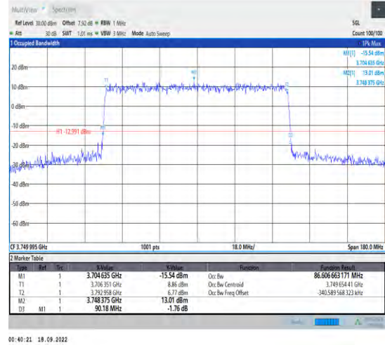
1-N78-3700-3800--30-90-M-3-DFT-16QAM-Outer_F ull-243@0-Ant1-86.607-90.180-<90-PASS
