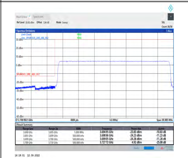
1-N78-3700-3800--30-30-L-6-CP-QPSK-Outer_Full-75@0-Ant1-1--PASS-see graph
