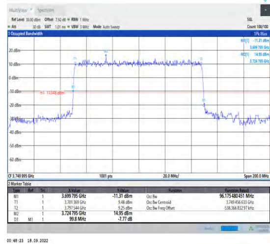
1-N78-3700-3800--30-100-M-2-DFT-PI2BPSK-Outer _Full-270@0-Ant1-96.175-99.800-≤100-PASS
