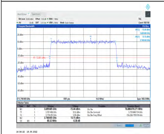
1-N78-3700-3800--30-80-L-4-DFT-64QAM-Outer_Full-216@0-Ant1-76.886-80.320-<80-PASS
