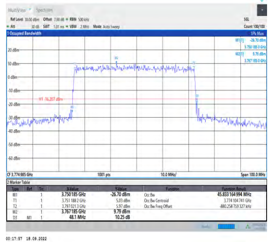
1-N78-3700-3800--30-50-H-5-DFT-256QAM-Oute... ull-128@0-Ant1-45.833-48.100-<50-PASS
