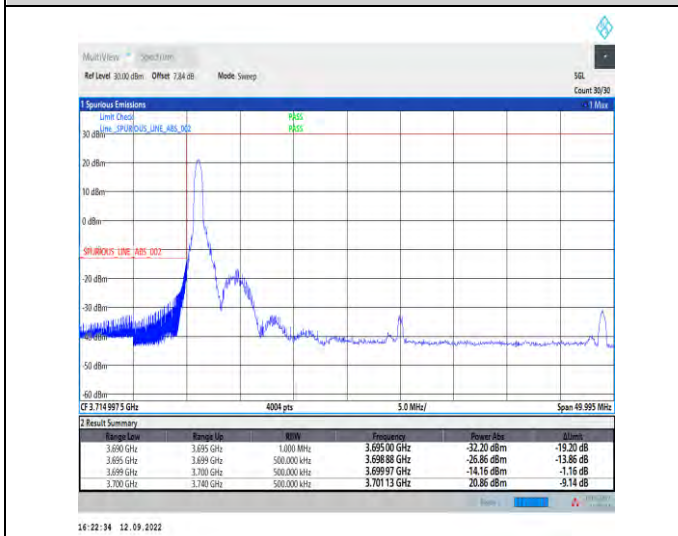
1-N78-3700-3800--30-40-L-4-CP-QPSK-Edge_1RB_L_eff-1@0-Ant1-1--PASS-see graph
