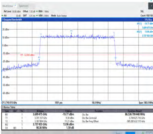
1-N78-3700-3800--30-90-L-1-DFT-QPSK-Outer_Full-243@0-Ant1-86.537-90.360-<90-PASS
