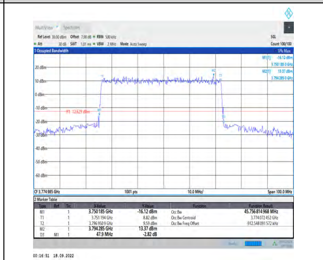
1-N78-3700-3800--30-50-H-1-DFT-QPSK-Outer_Full -128@0-Ant1-45.757-47.900-≤50-PASS
