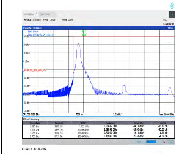
1-N78-3700-3800--30-20-L-4-CP-QPSK-Edge_1RB_L_eff-1@0-Ant1-1--PASS-see graph
