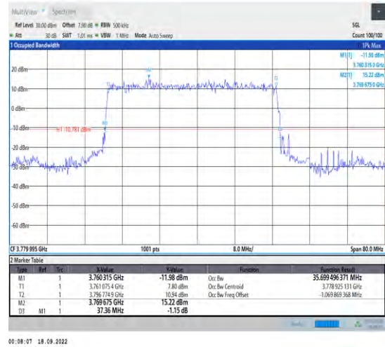
1-N78-3700-3800--30-40-H-2-DFT-PI2BPSK-Outer_Full -100@0-Ant1-35.699-37.360-<40-PASS
