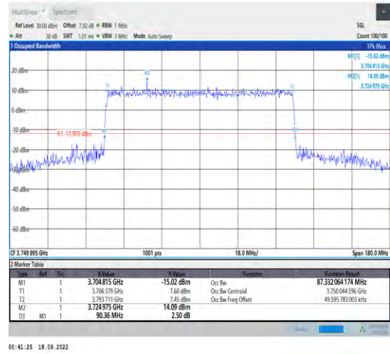
1-N78-3700-3800--30-90-M-7-CP-16QAM-Outer_Full-245@0-Ant1-87.332-90.360-<90-PASS
