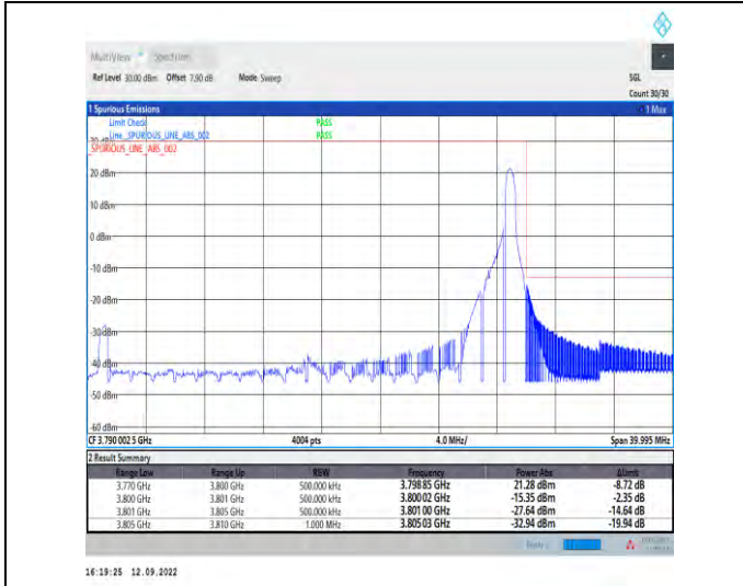
1-N78-3700-3800--30-30-H-2-DFT-PI2BPSK-Edge_1R_B_Right-1@77-Ant1-1--PASS-see graph
