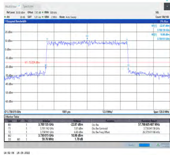
1-N78-3700-3800--30-60-L-4-DFT-64QAM-Outer_Full-162@0-Ant1-57.799-59.760-≤60-PASS
