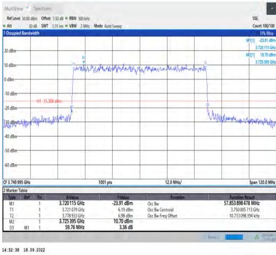
1-N78-3700-3800--30-60-M-4-DFT-64QAM-Outer_Full-162@0-Ant1-57.854-59.760-≤60-PASS
