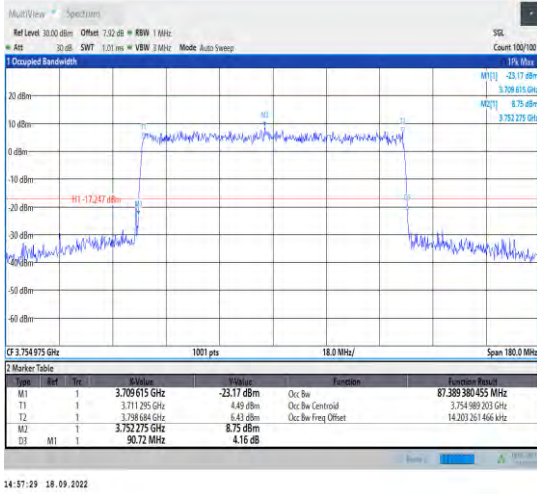
1-N78-3700-3800--30-90-H-9-CP-256QAM-Outer_Full-245@0-Ant1-87.389-90.720-<=90-PASS
