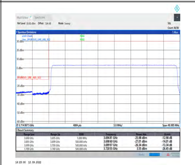
1-N78-3700-3800--30-40-L-6-CP-QPSK-Outer_Full-106@0-Ant1-1--PASS-see graph
