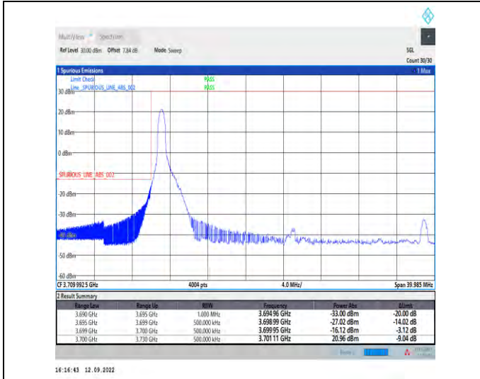
1-N78-3700-3800--30-30-L-1-DFT-PI2BPSK-Edge_1R_B_Left-1@0-Ant1-1--PASS-see graph
