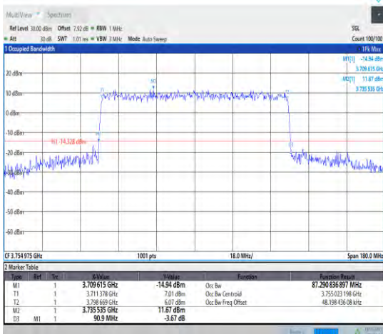
1-N78-3700-3800--30-90-H-7-CP-16QAM-Outer_Full-245@0-Ant1-87.291-90.900-<90-PASS
