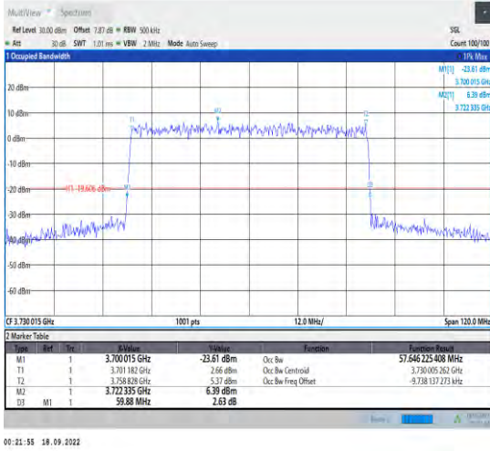
1-N78-3700-3800--30-60-L-9-CP-256QAM-Outer_Fu Il-162@0-Ant1-57.646-59.880-≤60-PASS
