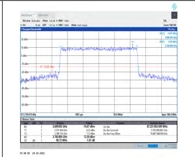
1-N78-3700-3800--30-90-L-8-CP-64QAM-Outer_Full -245@0-Ant1-87.252-90.720-≤90-PASS
