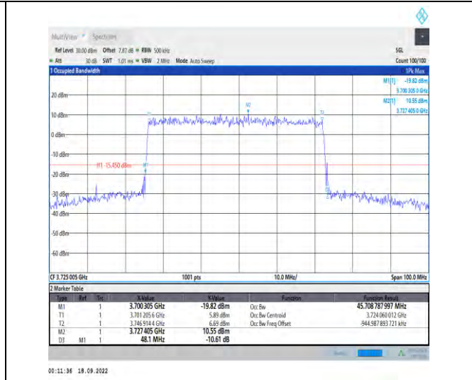
1-N78-3700-3800--30-50-L-5-DFT-256QAM-Outer_F uII-128@0-Ant1-45.709-48.100-≤50-PASS
