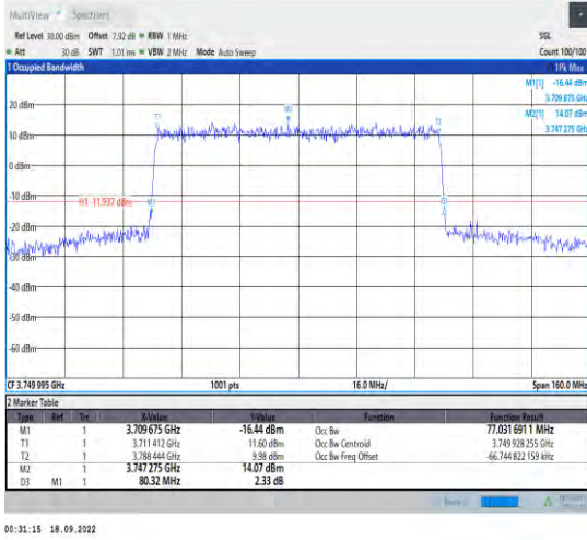
1-N78-3700-3800--30-80-M-1-DFT-QPSK-Outer_Full-216@0-Ant1-77.032-80.320-<80-PASS
