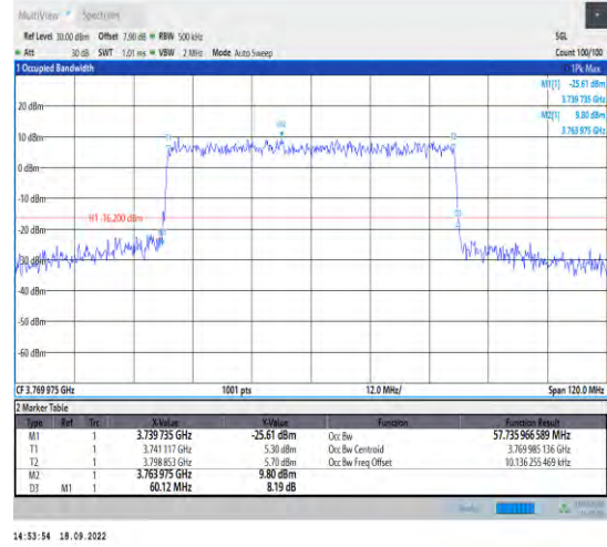
1-N78-3700-3800--30-60-H-8-CP-64QAM-Outer_Full -162@0-Ant1-57.736-60.120-<60-PASS
