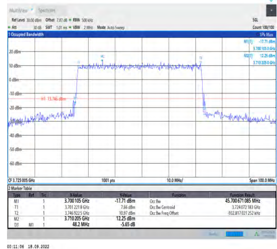
1-N78-3700-3800--30-50-L-3-DFT-16QAM-Outer_Full-128@0-Ant1-45.701-48.200-<math>\leq 50</math>-PASS
