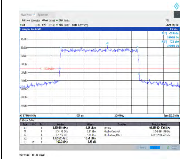
1-N78-3700-3800--30-100-M-5-DFT-256QAM-Outer_Full-270@0-Ant1-95.87-100.000-<100-PASS
