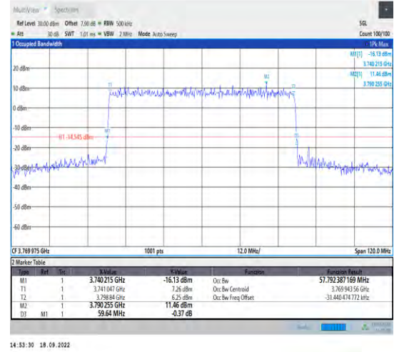
1-N78-3700-3800--30-60-H-4-DFT-64QAM-Outer_Fu II-162@0-Ant1-57.792-59.640-<60-PASS
