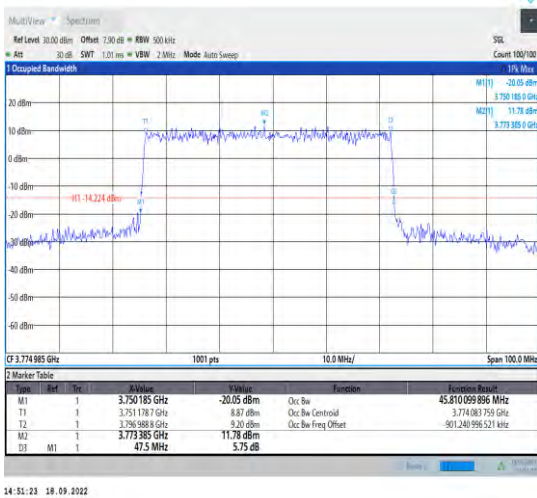
1-N78-3700-3800--30-50-H-4-DFT-64QAM-Oute... ll-128@0-Ant1-45.81-47.500-<50-PASS
