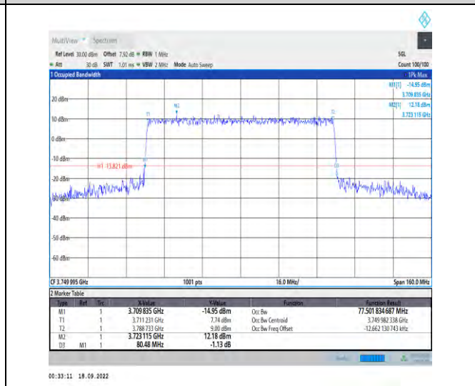
1-N78-3700-3800--30-80-M-8-CP-64QAM-Outer_Full-217@0-Ant1-77.502-80.480-≤80-PASS
