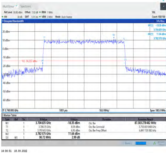
1-N78-3700-3800--30-90-M-8-CP-64QAM-Outer_Full-245@0-Ant1-87.303-90.720-<90-PASS
