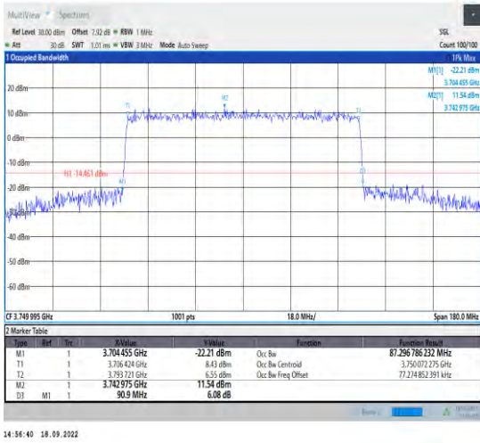
1-N78-3700-3800--30-90-M-6-CP-QPSK-Outer_Full-245@0-Ant1-87.297-90.900-<90-PASS
