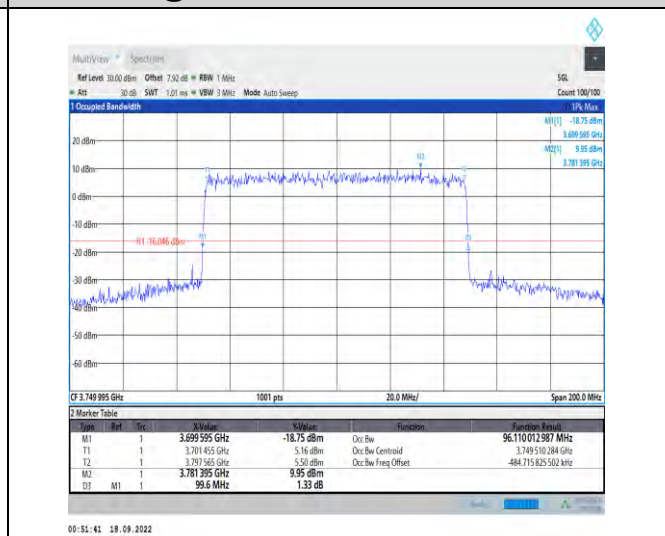
1-N78-3700-3800--30-100-H-5-DFT-256QAM-Outter_Full-270@0-Ant1-96.11-99.600-≤100-PASS
