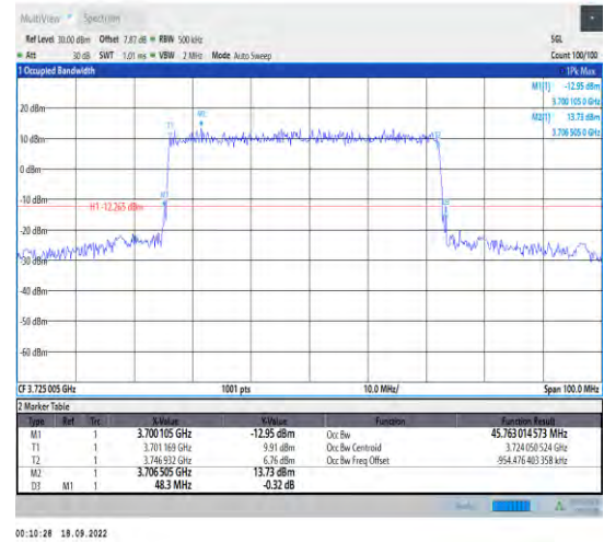
1-N78-3700-3800--30-50-L-1-DFT-QPSK-Outer_Full-128@0-Ant1-45.763-48.300-<math>\leq 50</math>-PASS
