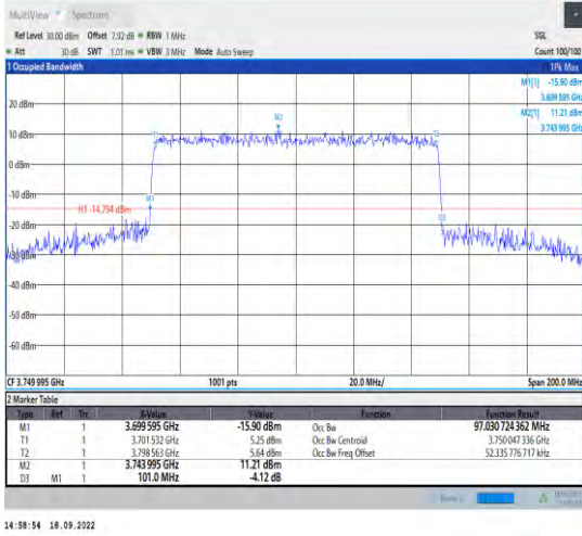
1-N78-3700-3800--30-100-H-6-CP-QPSK-Outer_Full-273@0-Ant1-97.031-101.000-≤100-PASS
