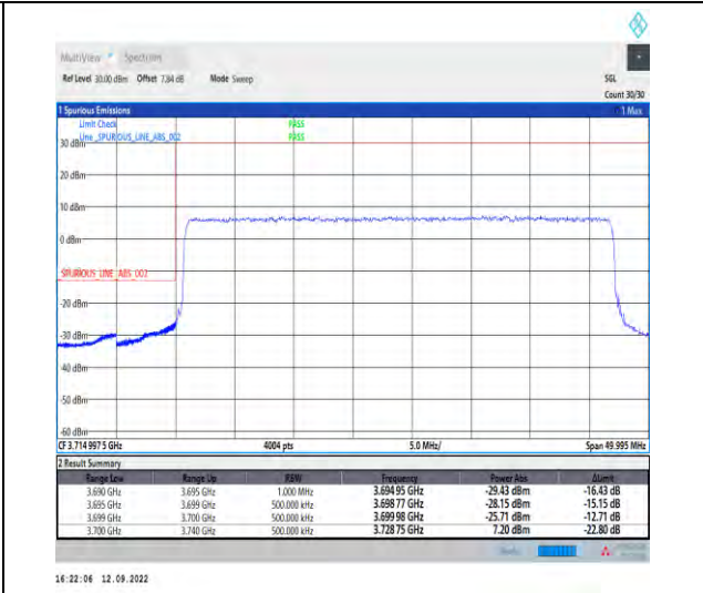
1-N78-3700-3800--30-40-L-3-DFT-PI2BPSK-Outer_Full-100@0-Ant1-1--PASS-see graph
