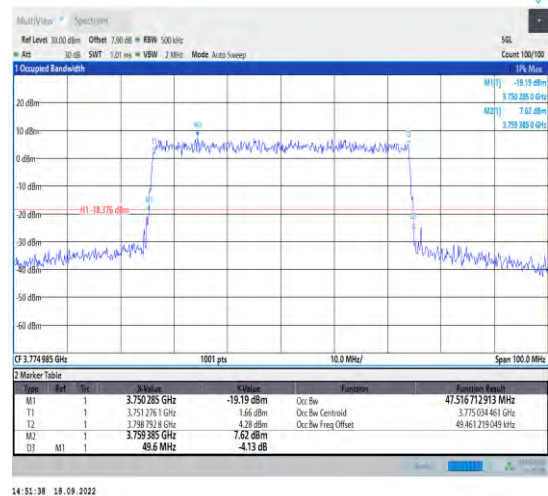
1-N78-3700-3800--30-50-H-9-CP-256QAM-Outer_Fu ll-133@0-Ant1-47.517-49.600-<50-PASS
