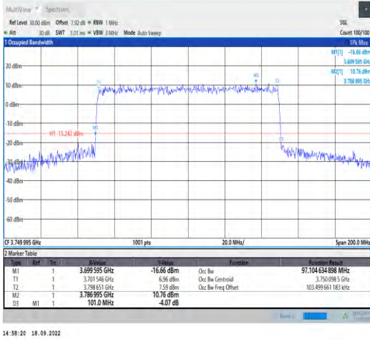
1-N78-3700-3800--30-100-L-8-CP-64QAM-Outer_Fu ll-273@0-Ant1-97.105-101.000-≤100-PASS
