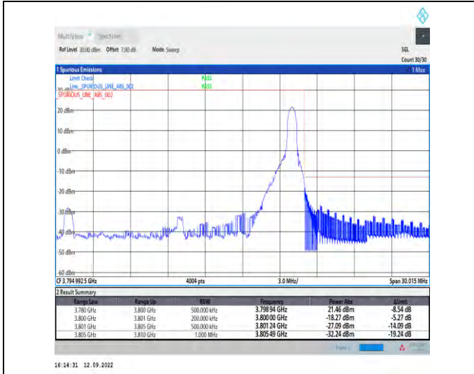
1-N78-3700-3800--30-20-H-2-DFT-PI2BPSK-Edge_1R_B_Right-1@50-Ant1-1--PASS-see graph
