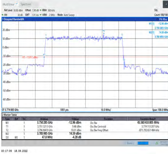
1-N78-3700-3800--30-50-H-2-DFT-PI2BPSK-Oute... Full-128@0-Ant1-45.583-47.800-<50-PASS
