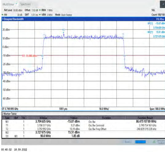
1-N78-3700-3800--30-90-M-2-DFT-PI2BPSK-Outer_F Full-243@0-Ant1-86.475-90.000-<90-PASS
