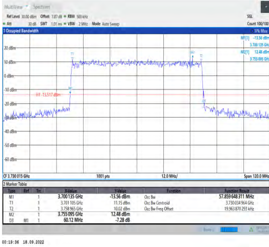
1-N78-3700-3800--30-60-L-1-DFT-QPSK-Outer_Full-162@0-Ant1-57.86-60.120-≤60-PASS
