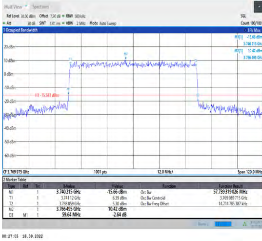
1-N78-3700-3800--30-60-H-7-CP-16QAM-Outer_Full -162@0-Ant1-57.739-59.640-<60-PASS
