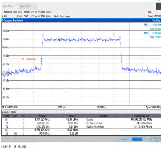
1-N78-3700-3800--30-90-M-4-DFT-64QAM-Outer_F ull-243@0-Ant1-86.598-90.000-<90-PASS
