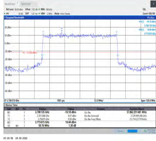
1-N78-3700-3800--30-60-L-2-DFT-PI2BPSK-Outer_Full-162@0-Ant1-57.862-59.760-≤60-PASS
