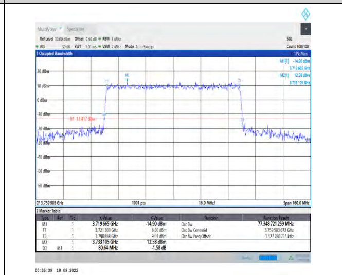
1-N78-3700-3800--30-80-H-7-CP-16QAM-Outer_Full-217@0-Ant1-77.349-80.640-<80-PASS
