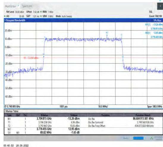
1-N78-3700-3800--30-90-M-5-DFT-256QAM-Outer_F Full-243@0-Ant1-86.605-89.820-<90-PASS
