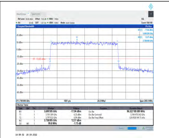
1-N78-3700-3800--30-100-M-4-DFT-64QAM-Outer_Full-270@0-Ant1-96.322-99.800-<100-PASS
