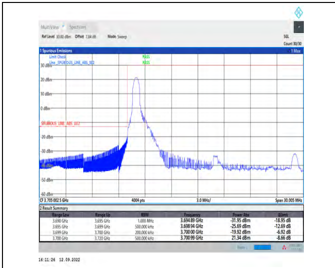
1-N78-3700-3800--30-20-L-1-DFT-PI2BPSK-Edge_1R_B_Left-1@0-Ant1-1--PASS-see graph
