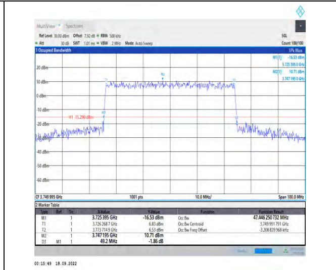
1-N78-3700-3800--30-50-M-8-CP-64QAM-Outer_Full -133@0-Ant1-47.446-49.200-≤50-PASS
