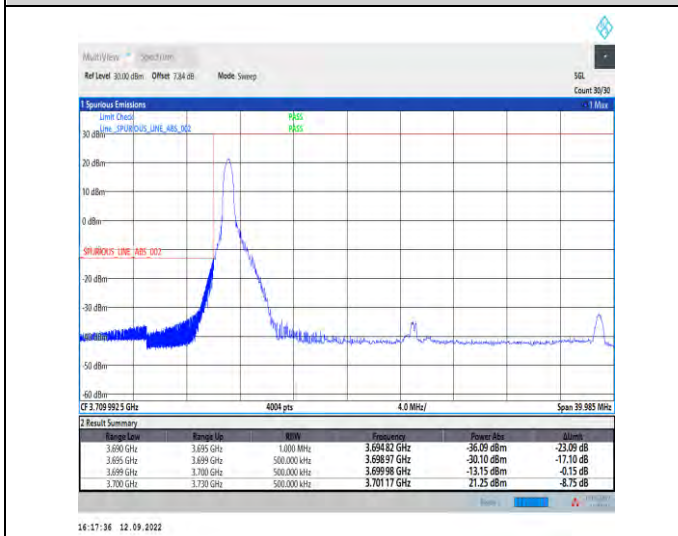
1-N78-3700-3800--30-30-L-4-CP-QPSK-Edge_1RB_L_eff-1@0-Ant1-1--PASS-see graph
