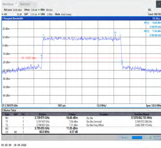
1-N78-3700-3800--30-60-H-3-DFT-16QAM-Outer_Fu II-162@0-Ant1-57.87-60.000-<60-PASS
