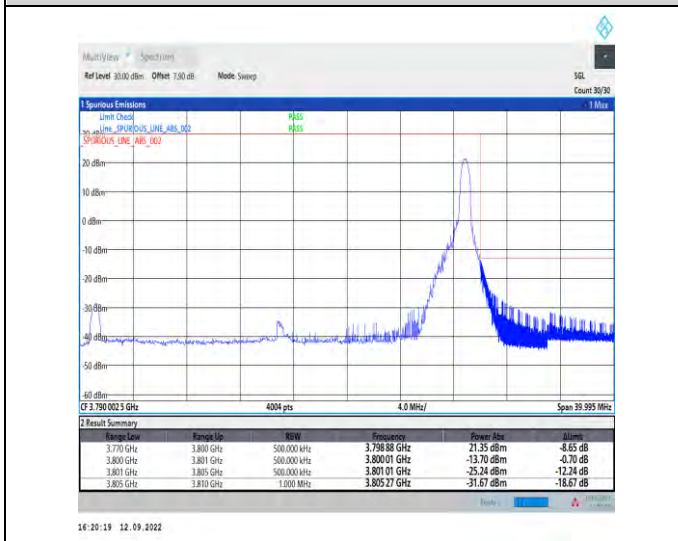
1-N78-3700-3800--30-30-H-5-CP-QPSK-Edge_1RB_R ight-1@77-Ant1-1--PASS-see graph
