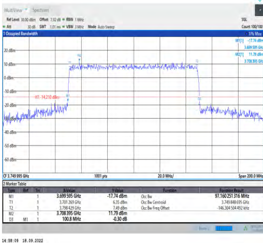
1-N78-3700-3800--30-100-L-6-CP-QPSK-Outer_Full-273@0-Ant1-97.16-100.800-≤100-PASS
