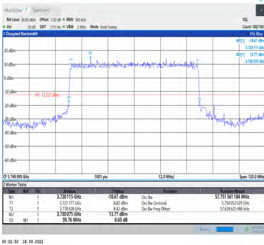
1-N78-3700-3800--30-60-M-2-DFT-PI2BPSK-Outer_Full Full-162@0-Ant1-57.752-59.760-≤60-PASS
