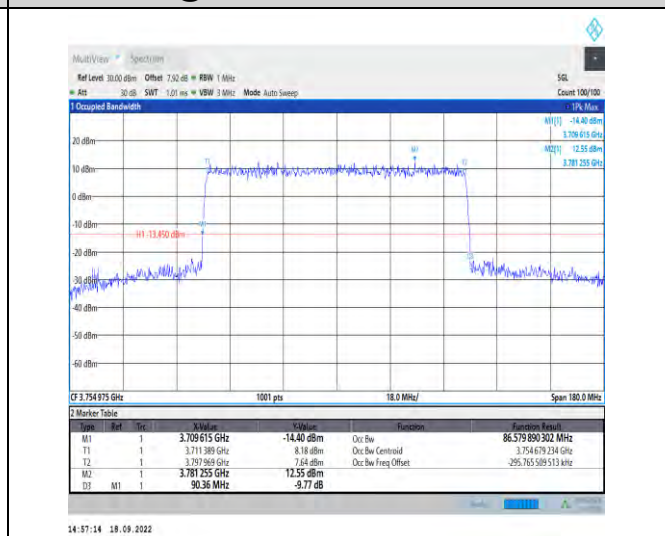
1-N78-3700-3800--30-90-H-4-DFT-64QAM-Outer_Fu II-243@0-Ant1-86.58-90.360-≤90-PASS
