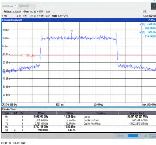
1-N78-3700-3800--30-100-M-1-DFT-QPSK-Outer_F ull-270@0-Ant1-96.092-99.800-≤100-PASS
