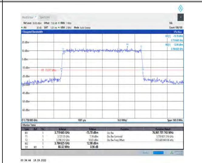
1-N78-3700-3800--30-80-H-3-DFT-16QAM-Outer_Full-216@0-Ant1-76.962-80.320-<80-PASS
