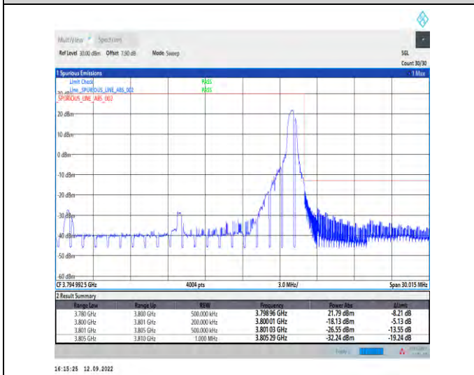
1-N78-3700-3800--30-20-H-5-CP-QPSK-Edge_1RB_R ight-1@50-Ant1-1--PASS-see graph
