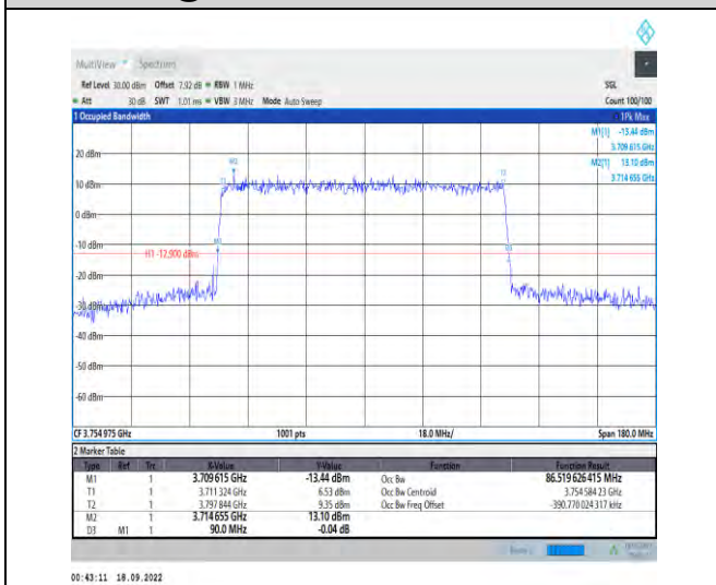
1-N78-3700-3800--30-90-H-3-DFT-16QAM-Outer_Fu II-243@0-Ant1-86.52-90.000-≤90-PASS
