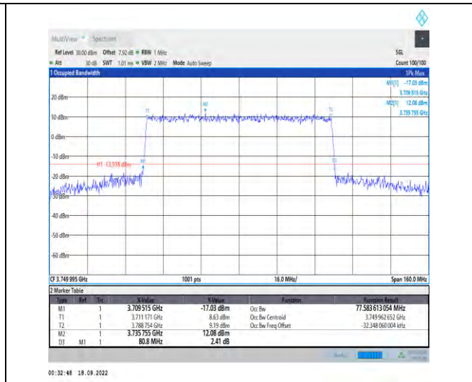
1-N78-3700-3800--30-80-M-6-CP-QPSK-Outer_Full-217@0-Ant1-77.584-80.800-≤80-PASS
