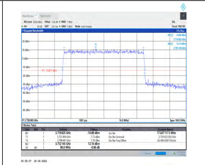
1-N78-3700-3800--30-80-H-5-DFT-256QAM-Outer_F ull-216@0-Ant1-77.037-80.000-<80-PASS
