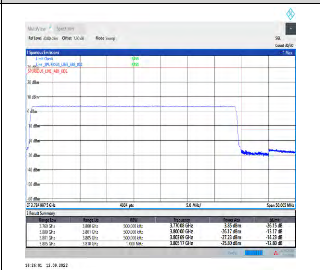
1-N78-3700-3800--30-40-H-6-CP-QPSK-Outer_Ful l-106@0-Ant1-1--PASS-see graph
