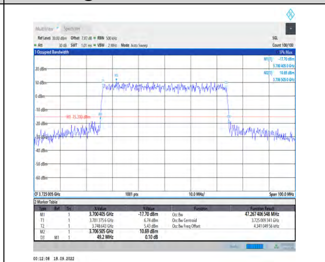
1-N78-3700-3800--30-50-L-7-CP-16QAM-Outer_Full -133@0-Ant1-47.267-49.200-≤50-PASS
