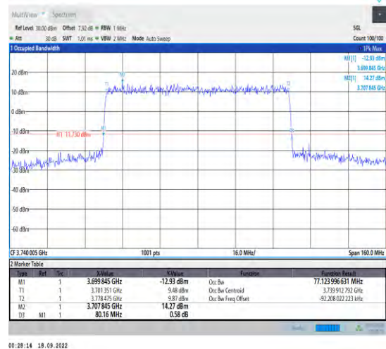
1-N78-3700-3800--30-80-L-1-DFT-QPSK-Outer_Full -216@0-Ant1-77.124-80.160-<80-PASS
