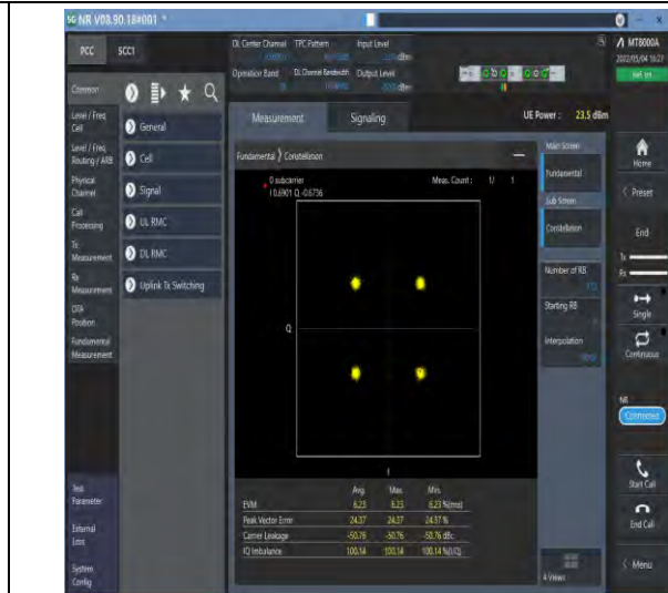
1-N78-3700-3800--30-100-M-6-CP-QPSK-Outer_Fu II-273@0-Ant1-see graph-PASS
