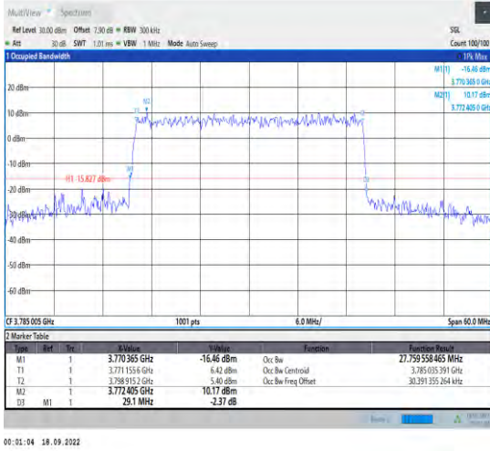
1-N78-3700-3800--30-30-H-8-CP-64QAM-Outer_Full -78@0-Ant1-27.76-29.100-<30-PASS
