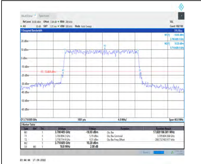
1-N78-3700-3800--30-20-L-5-DFT-256QAM-Outer_Full-50@0-Ant1-17.82-18.800-<20-PASS
