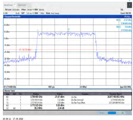
1-N78-3700-3800--30-30-L-5-DFT-256QAM-Outer_Full-75@0-Ant1-26.817-28.200-<30-PASS
