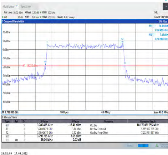
1-N78-3700-3800--30-20-H-9-CP-256QAM-Outer_F ull-51@0-Ant1-18.18-19.040-<20-PASS
