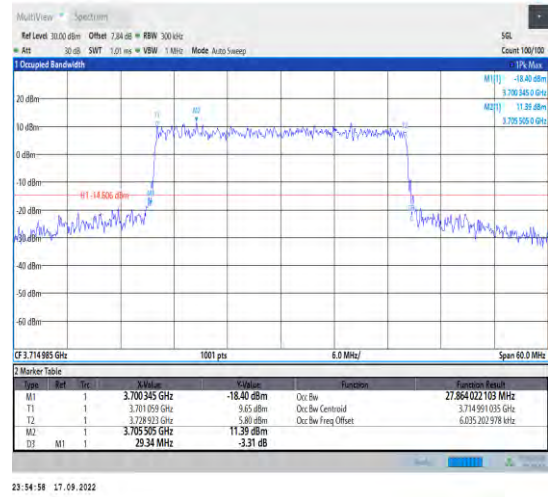
1-N78-3700-3800--30-30-L-7-CP-16QAM-Outer_Full-78@0-Ant1-27.864-29.340-≤30-PASS
