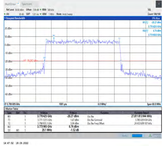
1-N78-3700-3800--30-30-H-9-CP-256QAM-Outer_Fu ll-78@0-Ant1-27.812-29.100-<30-PASS
