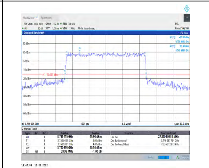
1-N78-3700-3800--30-30-M-8-CP-64QAM-Outer_Full-78@0-Ant1-27.891-28.980-<30-PASS
