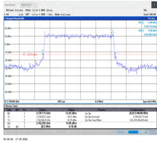
1-N78-3700-3800--30-30-M-2-DFT-PI2BPSK-Outer_Full Full-75@0-Ant1-26.812-28.500-<30-PASS
