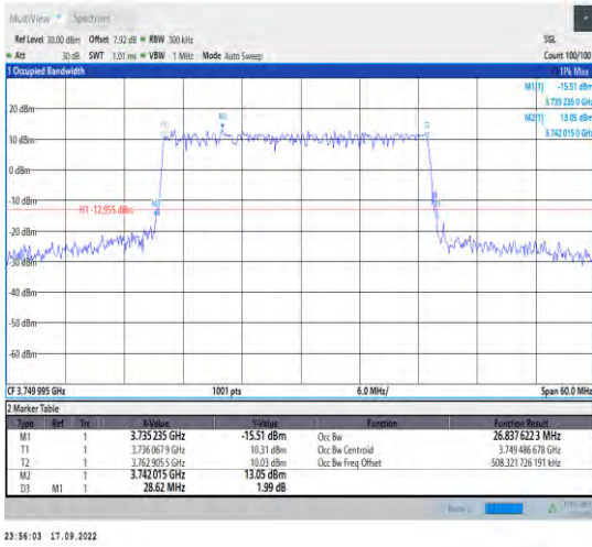
1-N78-3700-3800--30-30-M-1-DFT-QPSK-Outer_Full -75@0-Ant1-26.838-28.620-<30-PASS
