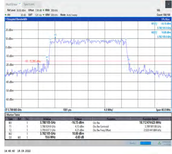
1-N78-3700-3800--30-20-H-8-CP-64QAM-Outer_Full -51@0-Ant1-18.112-19.600-<20-PASS
