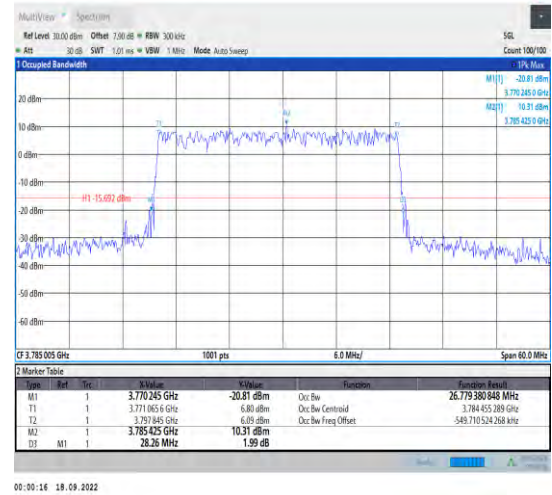
1-N78-3700-3800--30-30-H-5-DFT-256QAM-Outer_F ull-75@0-Ant1-26.779-28.260-<30-PASS
