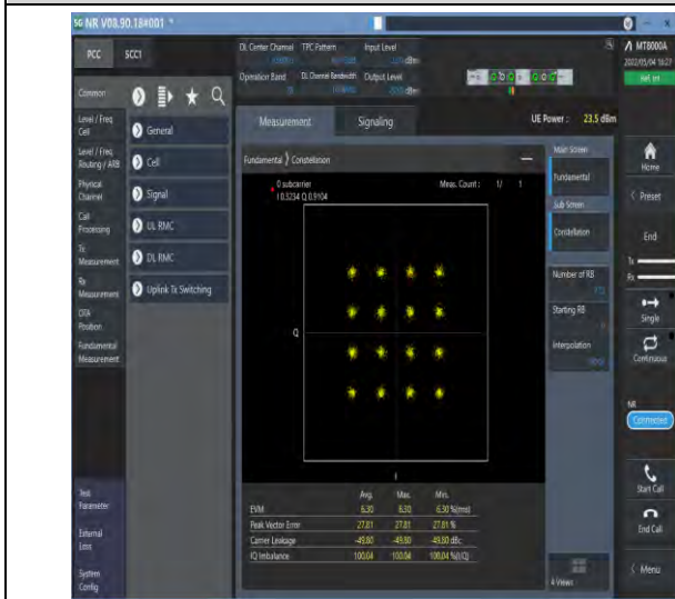
1-N78-3700-3800--30-100-M-7-CP-16QAM-Outer_Fu II-273@0-Ant1-see graph-PASS
