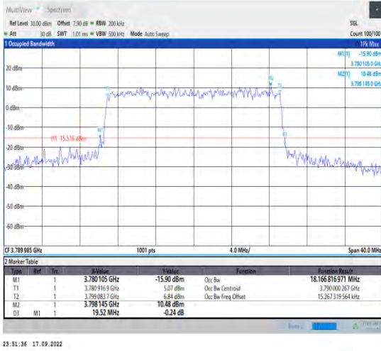
1-N78-3700-3800--30-20-H-7-CP-16QAM-Outer_Full -51@0-Ant1-18.167-19.520-<20-PASS
