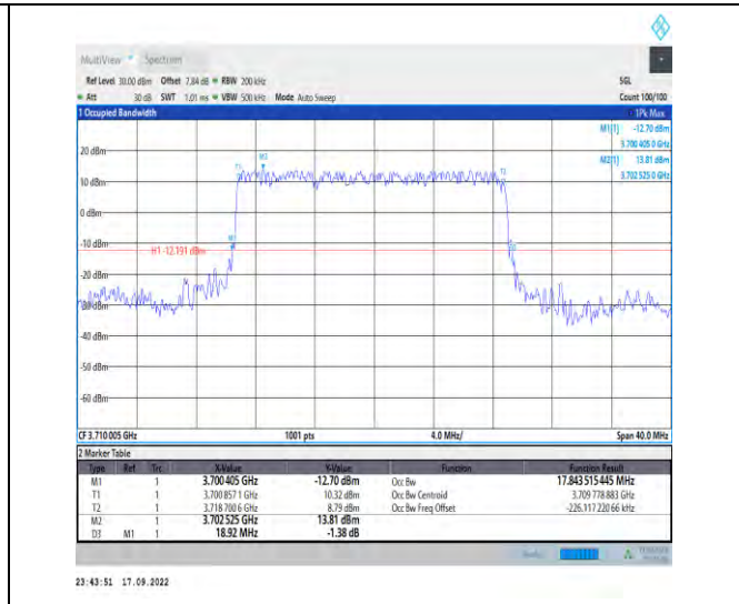
1-N78-3700-3800--30-20-L-2-DFT-PI2BPSK-Outer_Full-50@0-Ant1-17.844-18.920-<=20-PASS
