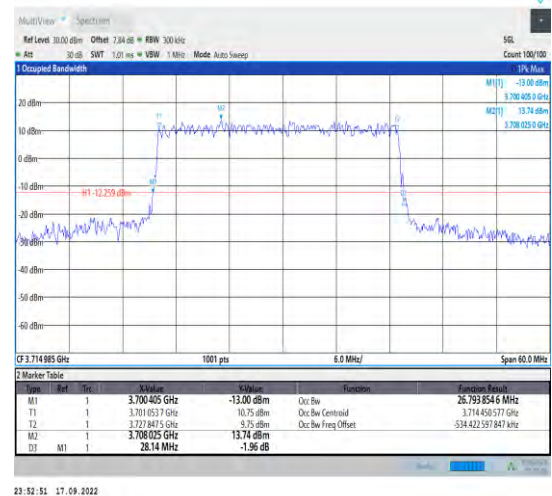
1-N78-3700-3800--30-30-L-1-DFT-QPSK-Outer_Full- 75@0-Ant1-26.794-28.140-<30-PASS
