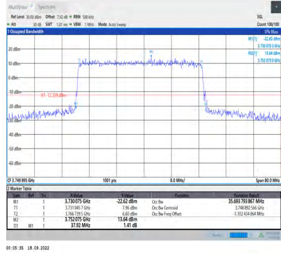
1-N78-3700-3800--30-40-M-3-DFT-16QAM-Outer_Full-100@0-Ant1-35.694-37.920-<40-PASS
