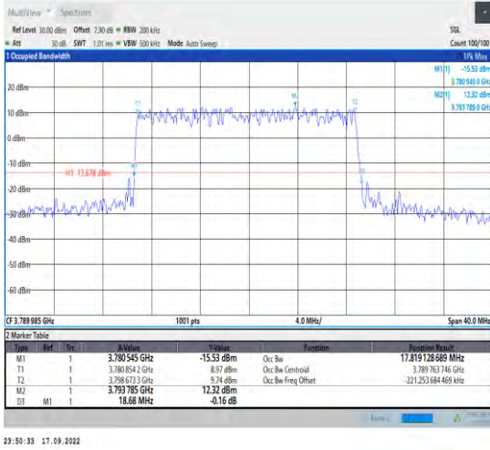
1-N78-3700-3800--30-20-H-3-DFT-16QAM-Outer_Fu II-50@0-Ant1-17.819-18.680-<20-PASS
