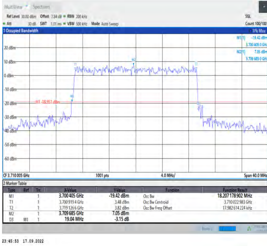
1-N78-3700-3800--30-20-L-9-CP-256QAM-Outer_Fu II-51@0-Ant1-18.207-19.040-<20-PASS
