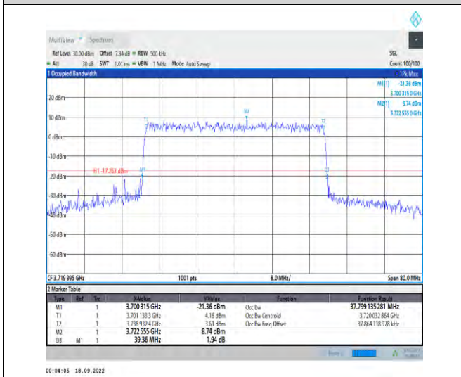
1-N78-3700-3800--30-40-L-9-CP-256QAM-Outer_Fu II-106@0-Ant1-37.799-39.360-<40-PASS
