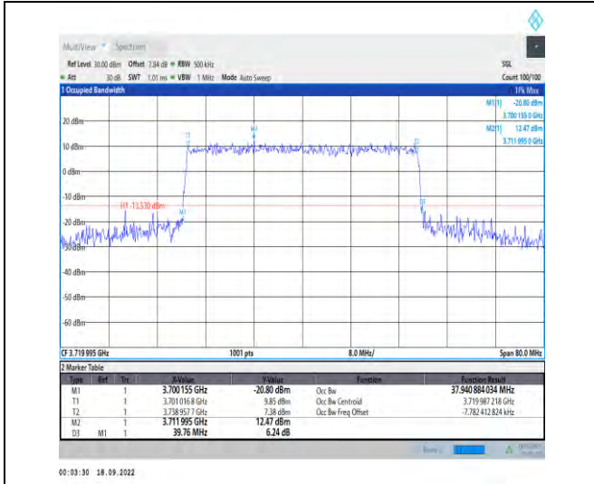
1-N78-3700-3800--30-40-L-7-CP-16QAM-Outer_Full -106@0-Ant1-37.941-39.760-<40-PASS
