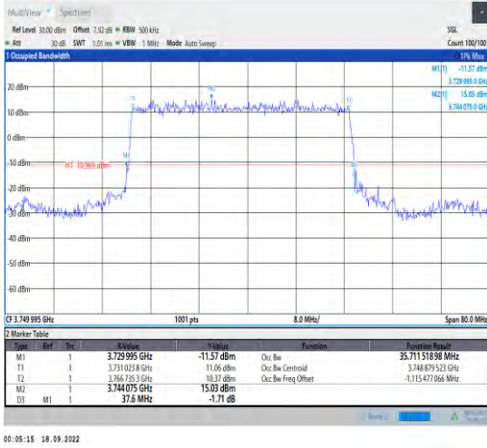
1-N78-3700-3800--30-40-M-2-DFT-PI2BPSK-Outer_Full-100@0-Ant1-35.712-37.600-<40-PASS
