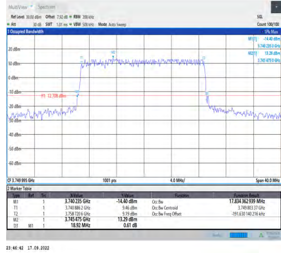
1-N78-3700-3800--30-20-M-1-DFT-QPSK-Outer_Full -50@0-Ant1-17.834-18.920-<20-PASS
