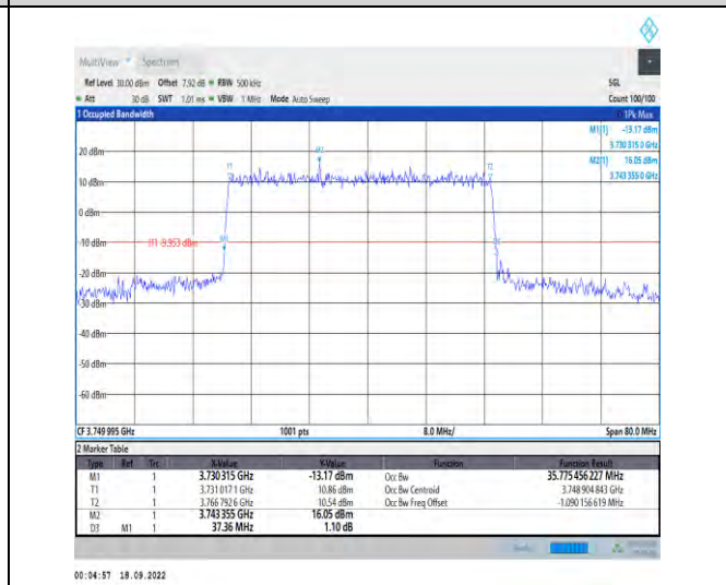
1-N78-3700-3800--30-40-M-1-DFT-QPSK-Outer_Full -100@0-Ant1-35.775-37.360-<40-PASS
