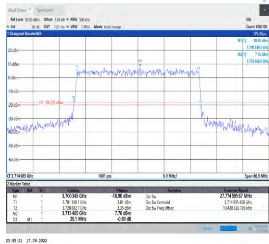
1-N78-3700-3800--30-30-L-9-CP-256QAM-Outer_Fu ll-78@0-Ant1-27.775-29.100-≤30-PASS
