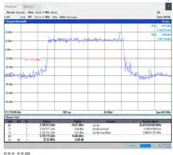
1-N78-3700-3800--30-40-L-2-DFT-PI2BPSK-Outer_F ull-100@0-Ant1-35.675-37.520-<40-PASS
