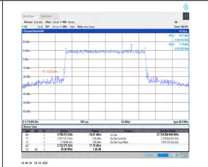
1-N78-3700-3800--30-40-L-8-CP-64QAM-Outer_Full -106@0-Ant1-37.754-39.360-<40-PASS
