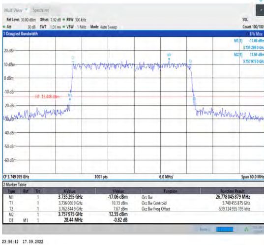
1-N78-3700-3800--30-30-M-3-DFT-16QAM-Outer_Full ull-75@0-Ant1-26.778-28.440-<30-PASS
