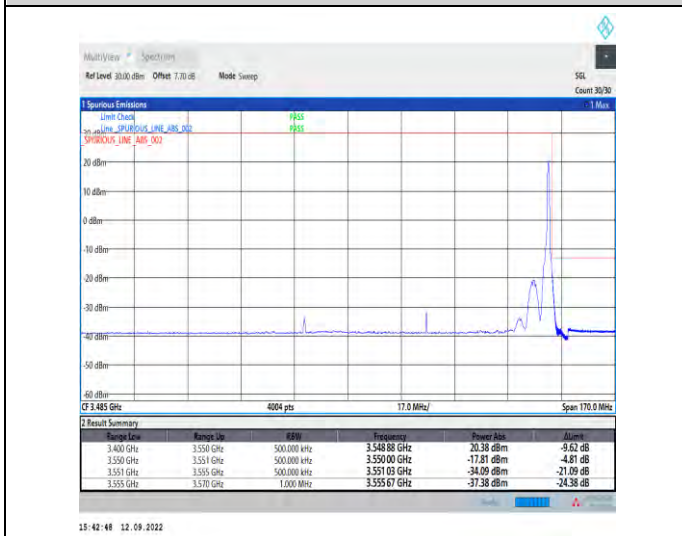
1-N78-3450-3550--30-80-H-5-CP-QPSK-Edge_1RB_Right-1@216-Ant1-1---see graph
