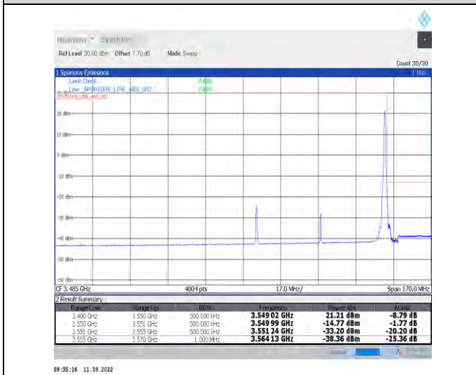
1-N78-3450-3550--30-60-H-5-CP-QPSK-Edge_1RB_Right-1@161-Ant1-1---see graph
