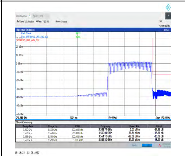
1-N78-3450-3550--30-50-H-6-CP-QPSK-Outer_Full-1133@0-Ant1-1---see graph
