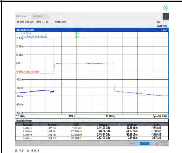
1-N78-3450-3550--30-80-L-6-CP-QPSK-Outer_Full-217@0-Ant1-1---see graph
