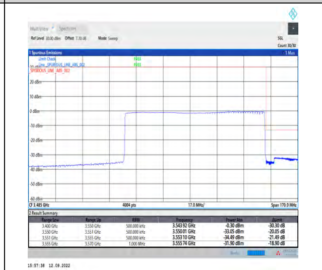
1-N78-3450-3550--30-90-H-6-CP-QPSK-Outer_Full-245@0-Ant1-1---see graph
