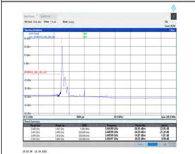
1-N78-3450-3550--30-60-L-4-CP-QPSK-Edge_1RB_Left-1@0-Ant1-1---see graph
