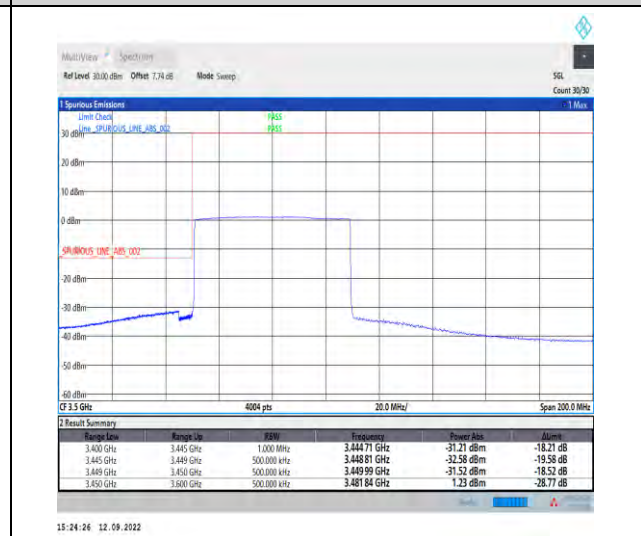
1-N78-3450-3550--30-60-L-6-CP-QPSK-Outer_Full-162@0-Ant1-1---see graph
