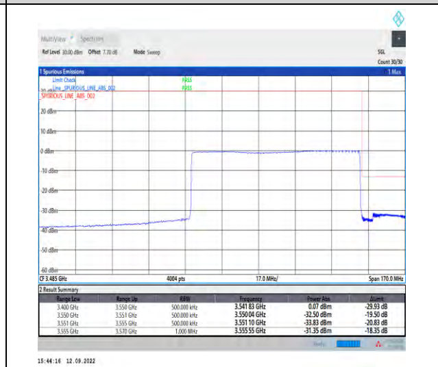
1-N78-3450-3550--30-80-H-6-CP-QPSK-Outer_Full-217@0-Ant1-1---see graph
