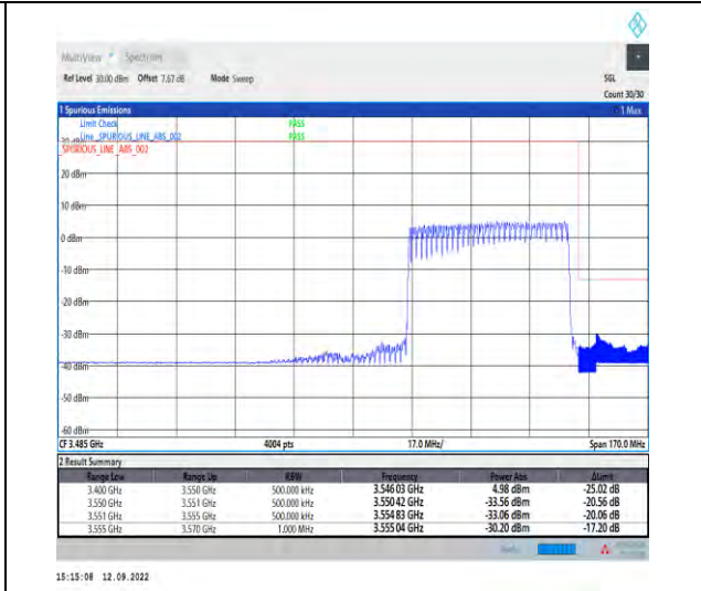
1-N78-3450-3550--30-50-H-3-DFT-PI2BPSK-Outer_Full-128@0-Ant1-1---see graph
