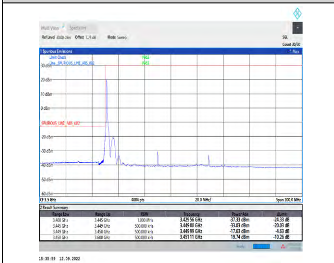
1-N78-3450-3550--30-80-L-4-CP-QPSK-Edge_1RB_Left-1@0-Ant1-1---see graph
