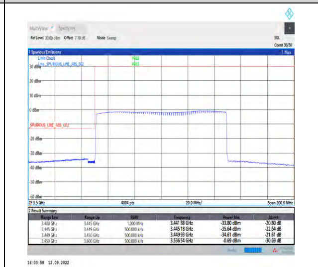
1-N78-3450-3550--30-100-L-6-CP-QPSK-Outer_Full-273@0-Ant1-1---see graph
