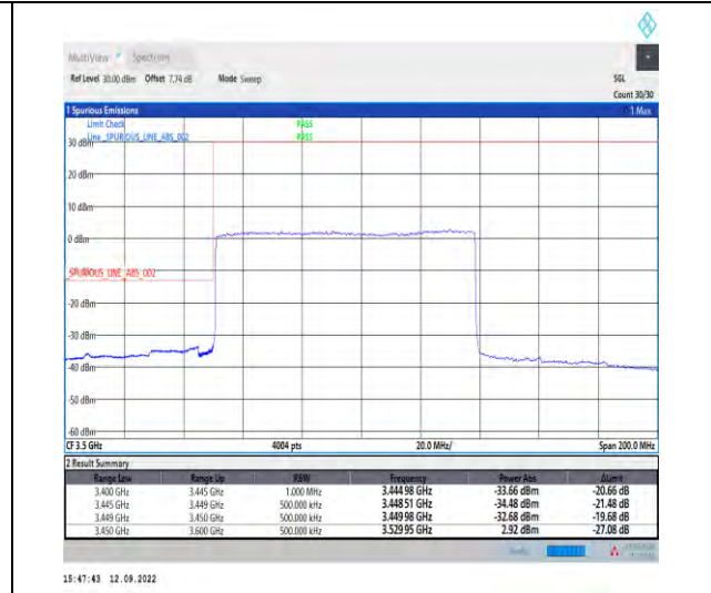
1-N78-3450-3550--30-90-L-3-DFT-PI2BPSK-Outer_Full-243@0-Ant1-1---see graph
