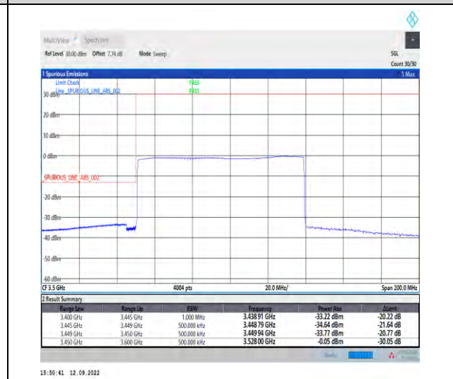
1-N78-3450-3550--30-90-L-6-CP-QPSK-Outer_Full-245@0-Ant1-1---see graph
