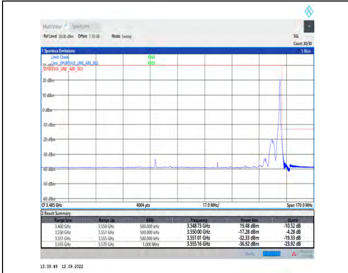
1-N78-3450-3550--30-80-H-2-DFT-PI2BPSK-Edge_1R_B_Right-1@216-Ant1-1---see graph
