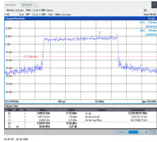
1-N78-3450-3550--30-60-H-8-CP-64QAM-Outer_Full -162@0-Ant1-57.566-59.640-≤60-
