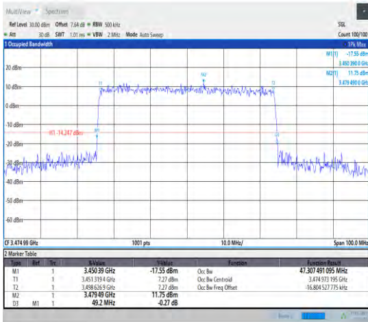
1-N78-3450-3550--30-50-L-8-CP-64QAM-Outer_Full -133@0-Ant1-47.307-49.200-<50-
