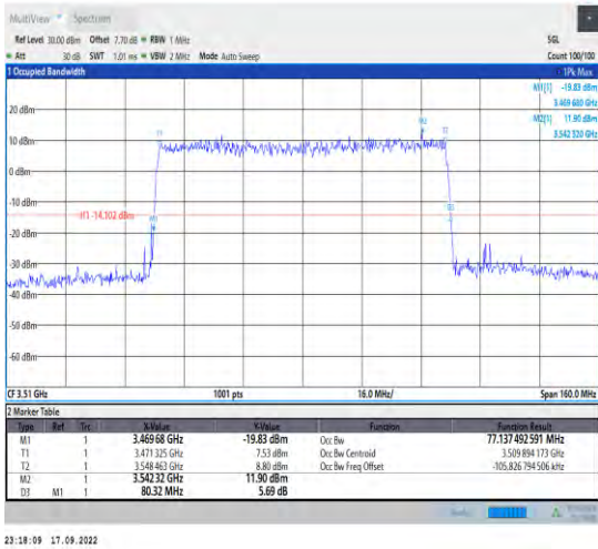
1-N78-3450-3550--30-80-H-8-CP-64QAM-Outer_Full -217@0-Ant1-29.976-31.360-≤80-
