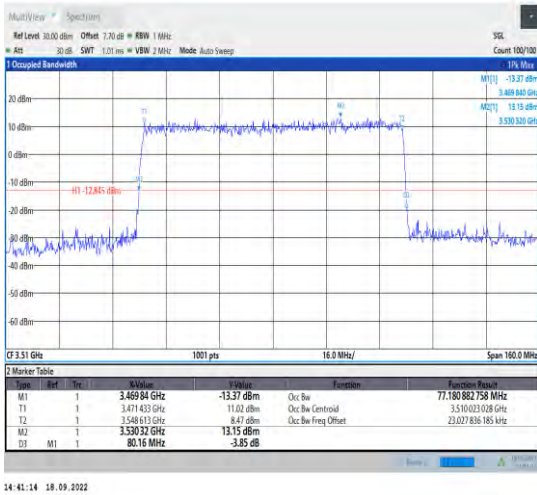
1-N78-3450-3550--30-80-H-4-DFT-64QAM-Outer_Fu ll-216@0-Ant1-77.181-80.160-<80-
