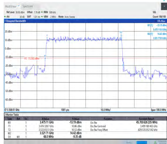
1-N78-3450-3550--30-50-M-2-DFT-PI2BPSK-Outer_Full Full-128@0-Ant1-45.704-48.000-<50-
