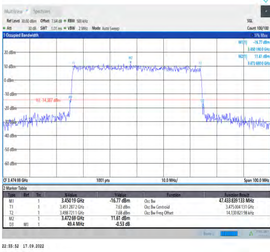
1-N78-3450-3550--30-50-L-6-CP-QPSK-Outer_Full 133@0-Ant1-47.434-49.400-<=50-
