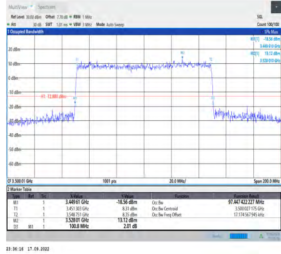
1-N78-3450-3550--30-100-H-7-CP-16QAM-Outer_Fu ll-273@0-Ant1-97.447-100.800-≤100-
