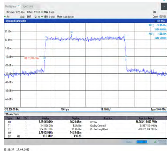
1-N78-3450-3550--30-90-M-1-DFT-QPSK-Outer_Full -243@0-Ant1-86.763-90.000<=90-
