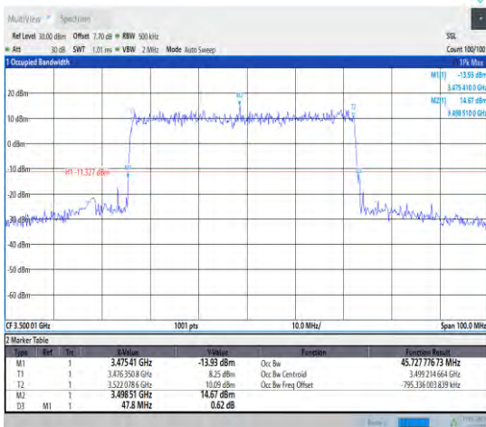
1-N78-3450-3550--30-50-M-1-DFT-QPSK-Outer_Full -128@0-Ant1-45.728-47.800-<50-
