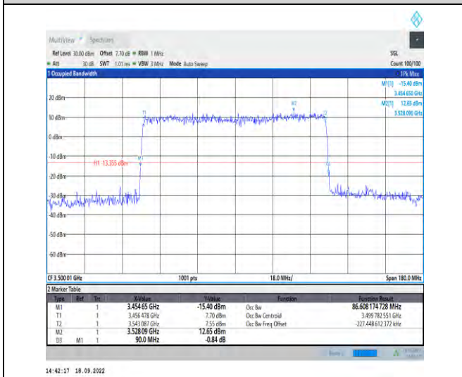
1-N78-3450-3550--30-90-M-4-DFT-64QAM-Oute... ull-243@0-Ant1-86.608-90.000-≤90-
