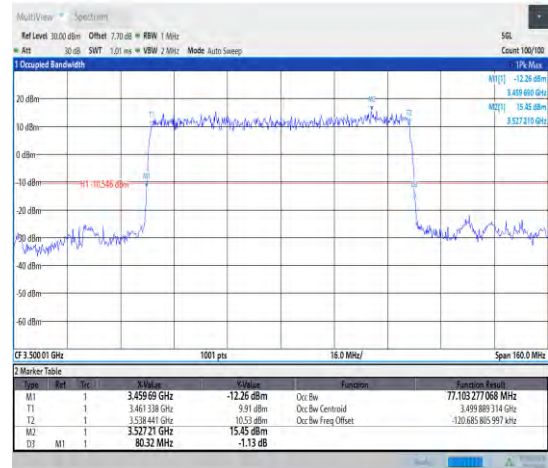
1-N78-3450-3550--30-80-M-2-DFT-PI2BPSK-Outer_Full -216@0-Ant1-77.103-80.320-≤80-
