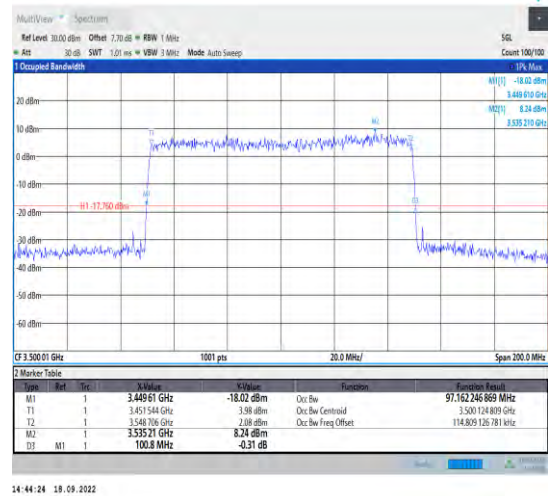
1-N78-3450-3550--30-100-H-9-CP-256QAM-Outer_F ull-273@0-Ant1-97.162-100.800-≤100-
