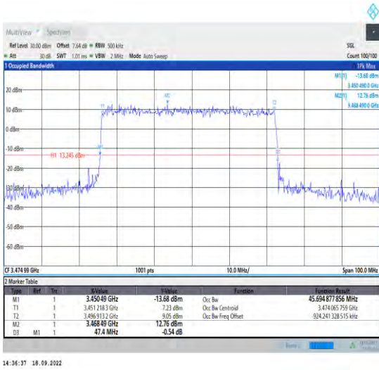
1-N78-3450-3550--30-50-L-4-DFT-64QAM-Outer_Fu II-128@0-Ant1-45.695-47.400-<=50-
