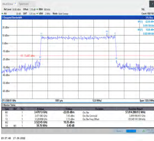
1-N78-3450-3550--30-60-M-8-CP-64QAM-Outer_Ful I-162@0-Ant1-57.814-59.760-≤60-
