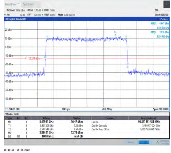
1-N78-3450-3550--30-100-M-4-DFT-64QAM-Outer_Full-270@0-Ant1-96.341-100.000-≤100-
