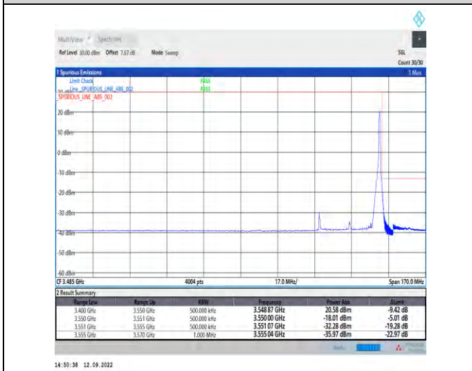
1-N78-3450-3550--30-30-H-5-CP-QPSK-Edge_1RB_Right-1@77-Ant1-1---see graph
