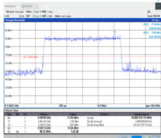
1-N78-3450-3550--30-80-M-4-DFT-64QAM-Outer_Full -216@0-Ant1-76.896-80.320-≤80-
