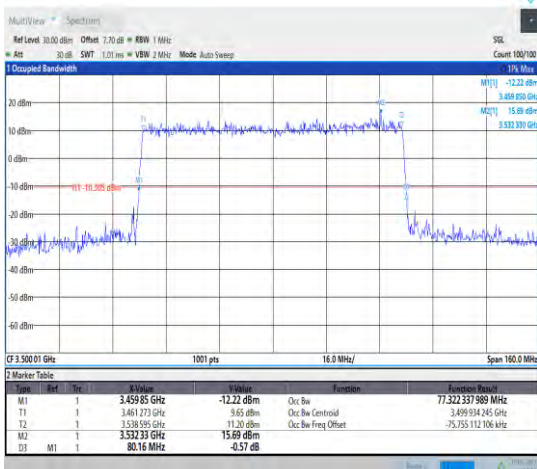
1-N78-3450-3550--30-80-M-3-DFT-16QAM-Outer_Full -216@0-Ant1-77.322-80.160-≤80-
