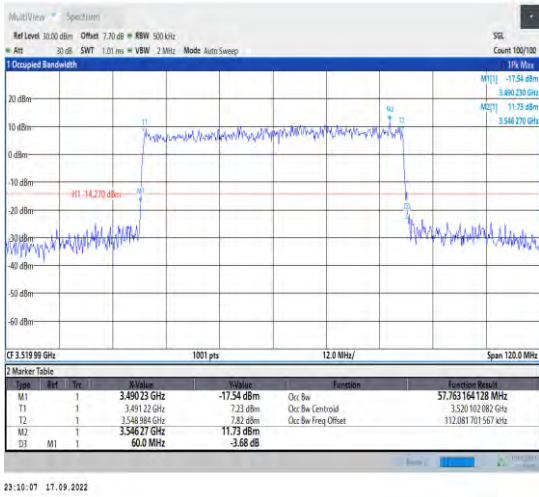
1-N78-3450-3550--30-60-H-7-CP-16QAM-Outer_Full -162@0-Ant1-57.763-60.000-≤60-
