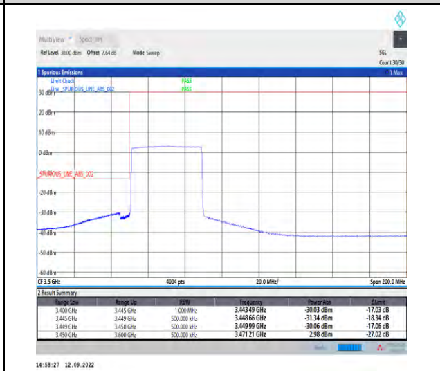
1-N78-3450-3550--30-40-L-6-CP-QPSK-Outer_Full-106@0-Ant1-1---see graph
