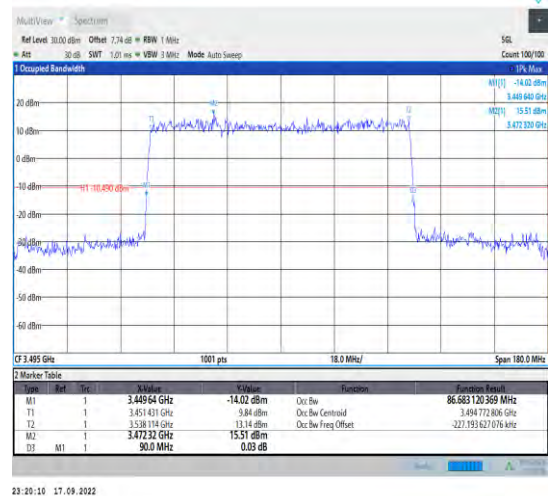
1-N78-3450-3550--30-90-L-2-DFT-PI2BPSK-Outer_F ull-243@0-Ant1-86.683-90.000-≤90-
