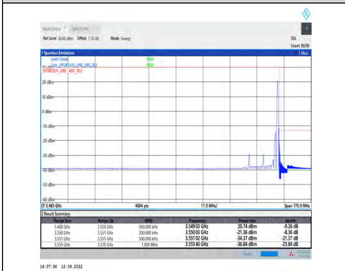
1-N78-3450-3550--30-20-H-5-CP-QPSK-Edge_1RB_Right-1@50-Ant1-1---see graph
