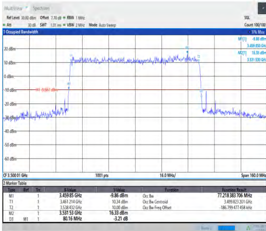
1-N78-3450-3550--30-80-M-1-DFT-QPSK-Outer_Full -216@0-Ant1-77.218-80.160-≤80-
