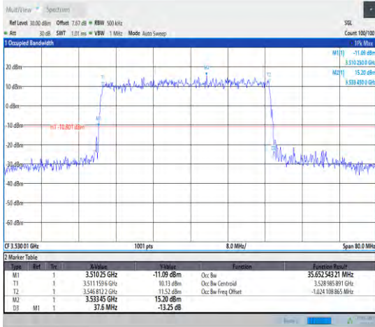
1-N78-3450-3550--30-40-H-1-DFT-QPSK-Outer_Full -100@0-Ant1-35.653-37.600-<40-
