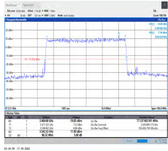
1-N78-3450-3550--30-80-H-5-DFT-256QAM-Outer_F ull-216@0-Ant1-77.137-80.320-<80-
