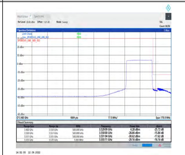
1-N78-3450-3550--30-30-H-6-CP-QPSK-Outer_Full-78@0-Ant1-1---see graph
