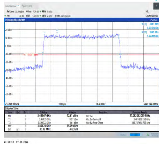
1-N78-3450-3550--30-80-L-1-DFT-QPSK-Outer_Full 216@0-Ant1-77.032-80.320-≤80-
