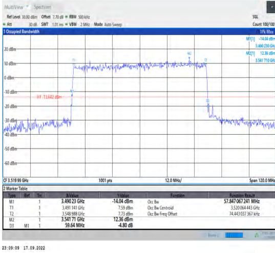
1-N78-3450-3550--30-60-H-3-DFT-16QAM-Outer_Fu II-162@0-Ant1-57.847-59.640-≤60-
