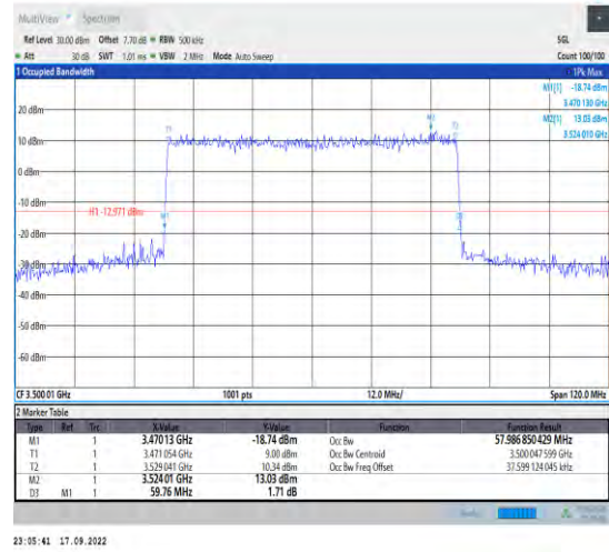
1-N78-3450-3550--30-60-M-1-DFT-QPSK-Outer_Full -162@0-Ant1-57.987-59.760-<60-
