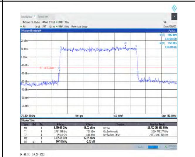
1-N78-3450-3550--30-90-H-4-DFT-64QAM-Outer_Full II-243@0-Ant1-86.702-90.180-≤90-
