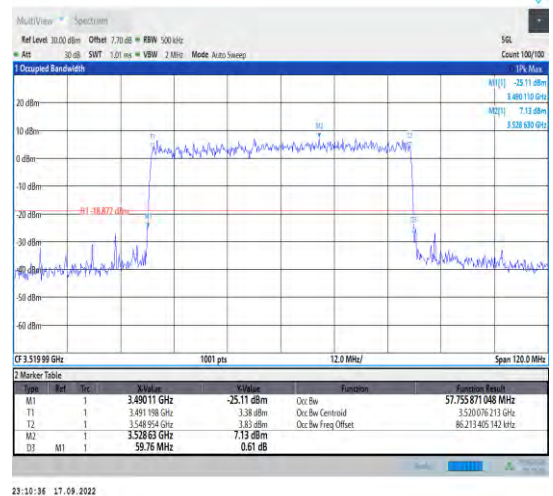
1-N78-3450-3550--30-60-H-6-CP-QPSK-Outer_Full- 162@0-Ant1-58.117-59.640-≤60-
