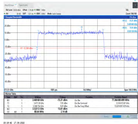
1-N78-3450-3550--30-80-H-7-CP-16QAM-Outer_Full -217@0-Ant1-77.366-80.640-<80-
