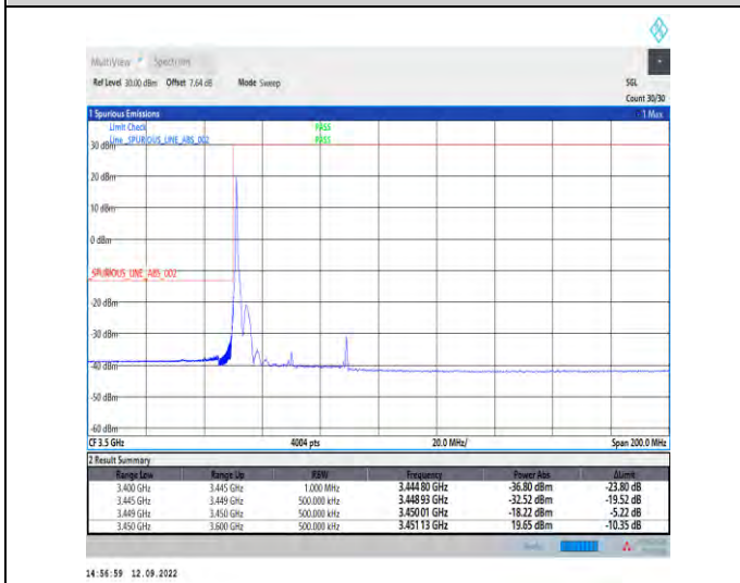
1-N78-3450-3550--30-40-L-4-CP-QPSK-Edge_1RB_Left-1@0-Ant1-1---see graph
