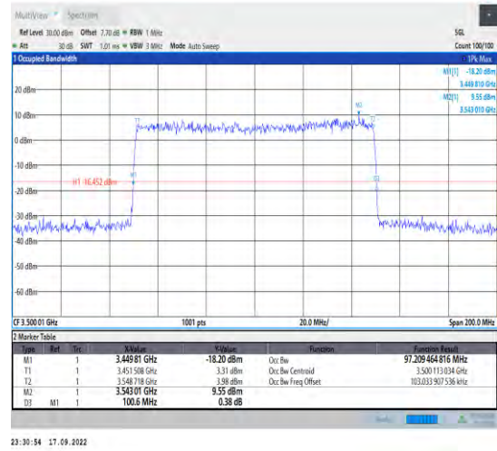
1-N78-3450-3550--30-100-L-9-CP-256QAM-Out-er_F ull-273@0-Ant1-97.209-100.600-≤100-
