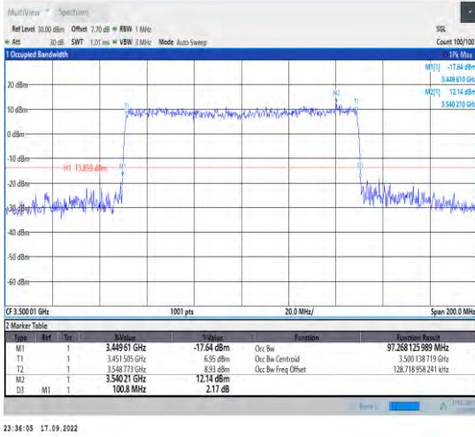
1-N78-3450-3550--30-100-H-6-CP-QPSK-Outer_Full -273@0-Ant1-97.268-100.800-≤100-
