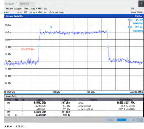
1-N78-3450-3550--30-90-L-4-DFT-64QAM-Outer_Ful l-243@0-Ant1-86.595-89.820-<90-
