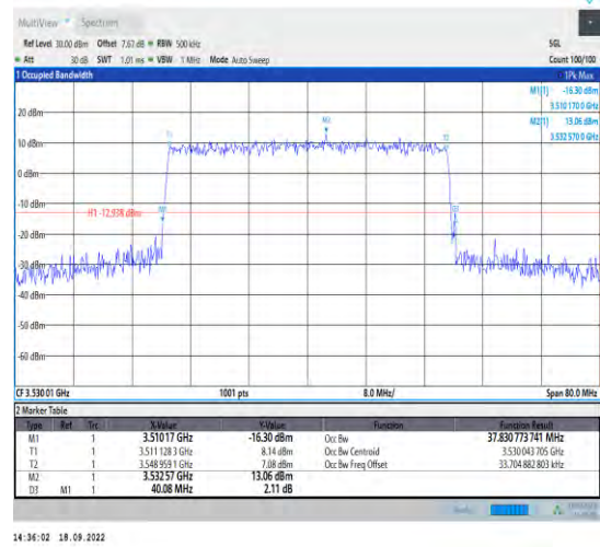
1-N78-3450-3550--30-40-H-8-CP-64QAM-Outer_Full@0-Ant1-37.831-40.080-<40-
