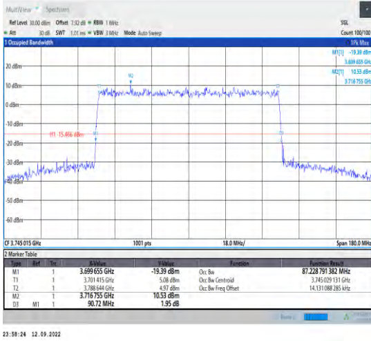
1-N77-3700-3980--30-90-L-9-CP-256QAM-Outer_Fu II-245@0-Ant1-87.229-90.720-<=90-PASS
