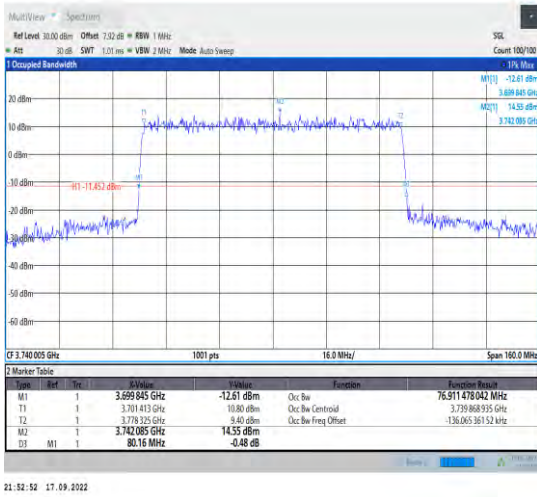
1-N77-3700-3980--30-80-L-4-DFT-64QAM-Outer_Fu II-216@0-Ant1-76.911-80.160-≤80-PASS
