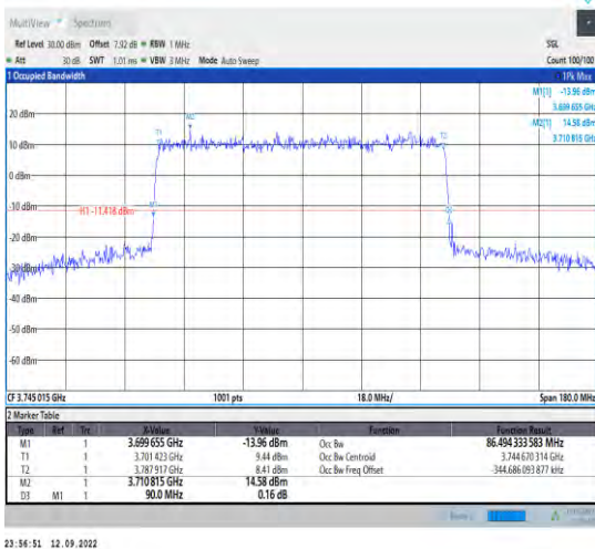
1-N77-3700-3980--30-90-L-3-DFT-16QAM-Outer_Full-243@0-Ant1-86.494-90.000-<90-PASS
