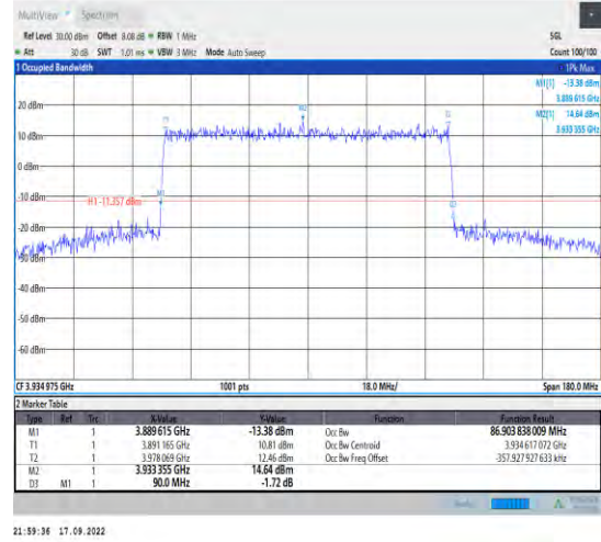
1-N77-3700-3980--30-90-H-4-DFT-64QAM-Outer_Fu II-243@0-Ant1-86.904-90.000-<90-PASS
