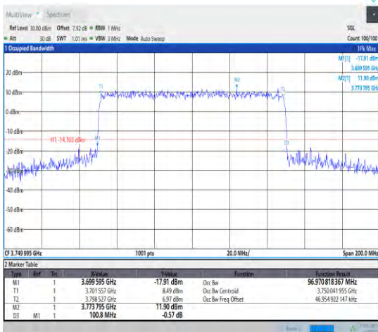
1-N77-3700-3980--30-100-L-8-CP-64QAM-Outer_Fu ll-273@0-Ant1-96.971-100.800-≤100-PASS
