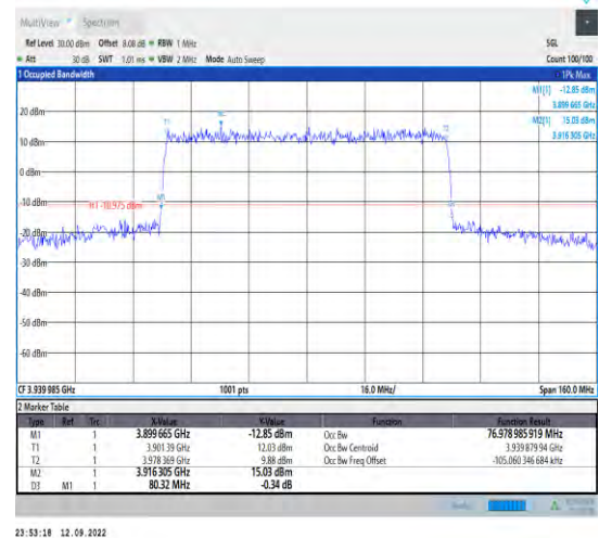
1-N77-3700-3980--30-80-H-1-DFT-QPSK-Outer_Full -216@0-Ant1-76.979-80.320-<80-PASS
