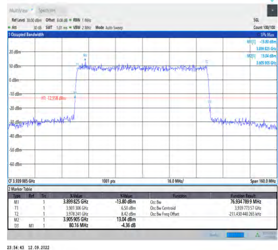
1-N77-3700-3980--30-80-H-5-DFT-256QAM-Outer_Full-216@0-Ant1-76.935-80.160-<80-PASS
