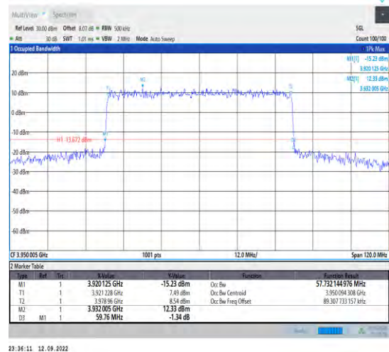
1-N77-3700-3980--30-60-H-1-DFT-QPSK-Outer_Full -162@0-Ant1-57.732-59.760-≤60-PASS
