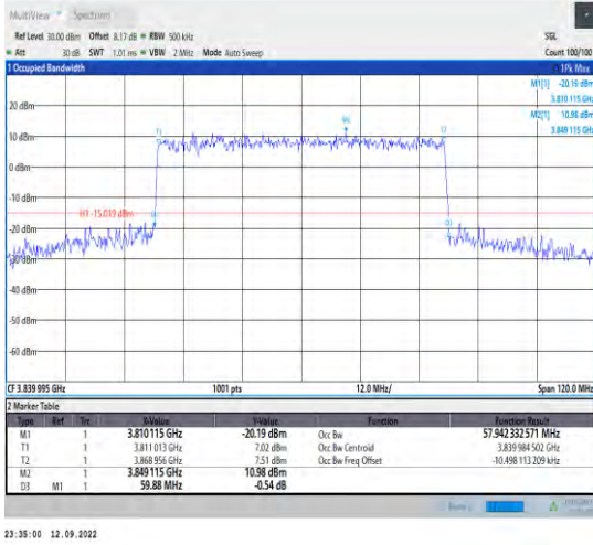
1-N77-3700-3980--30-60-M-7-CP-16QAM-Outer_Full I-162@0-Ant1-57.942-59.880-≤60-PASS
