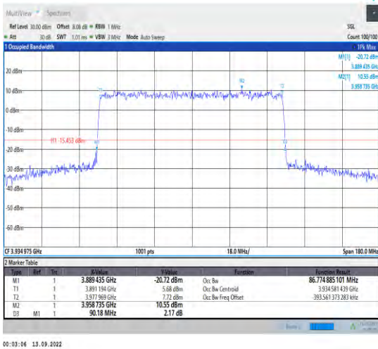
1-N77-3700-3980--30-90-H-5-DFT-256QAM-Outer_Full-243@0-Ant1-86.775-90.180-<90-PASS
