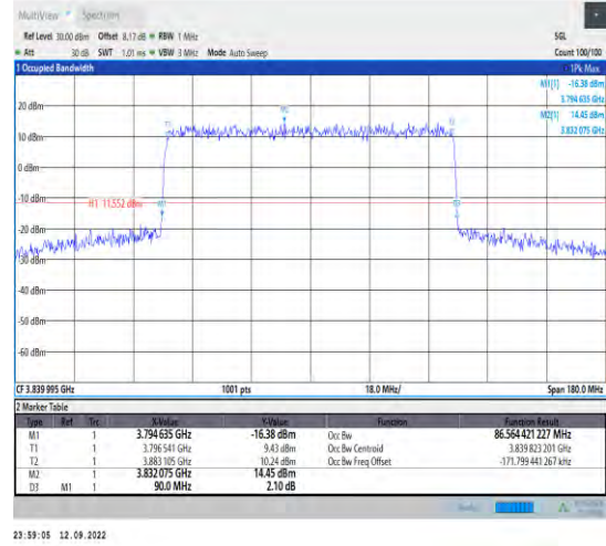
1-N77-3700-3980--30-90-M-1-DFT-QPSK-Outer_Full -243@0-Ant1-86.564-90.000-<=90-PASS
