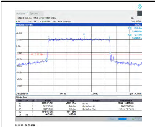
1-N77-3700-3980--30-60-M-1-DFT-QPSK-Outer_Full -162@0-Ant1-57.668-60.000-≤60-PASS
