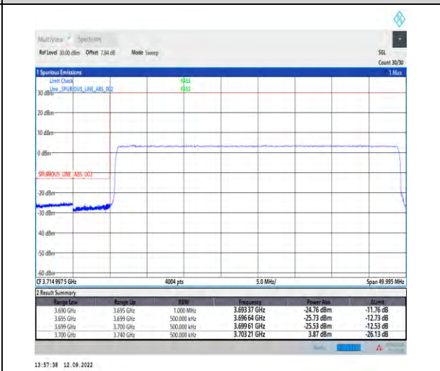
1-N77-3700-3980--30-40-L-6-CP-QPSK-Outer_Full-106@0-Ant1-1--PASS-see graph
