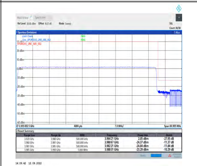
1-N77-3700-3980--30-60-H-6-CP-QPSK-Outer_Ful l-162@0-Ant1-1--PASS-see graph
