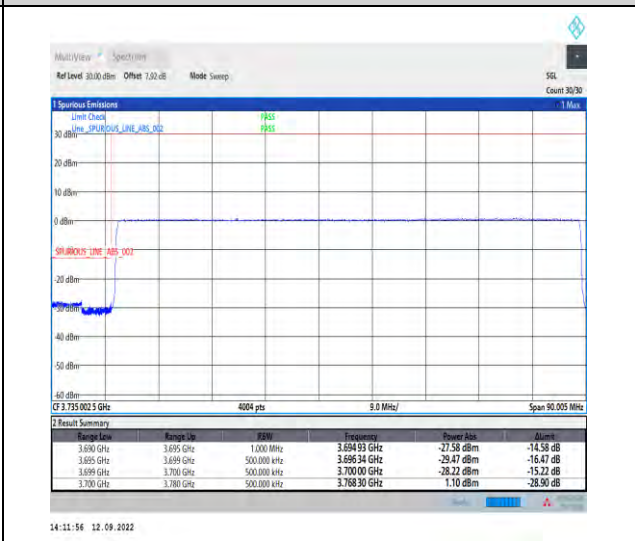
1-N77-3700-3980--30-80-L-6-CP-QPSK-Outer_Ful_l-217@0-Ant1-1--PASS-see graph
