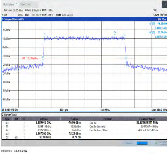
1-N77-3700-3980--30-90-H-3-DFT-16QAM-Outer_Fu II-243@0-Ant1-86.839-90.180-<90-PASS
