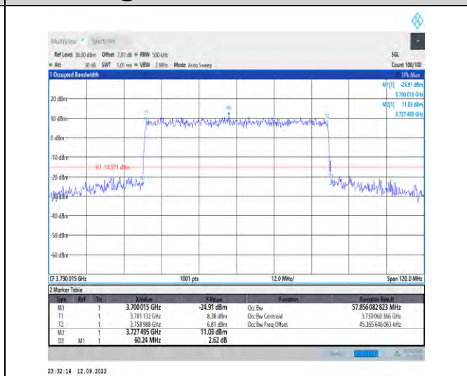
1-N77-3700-3980--30-60-L-7-CP-16QAM-Outer_Full -162@0-Ant1-57.856-60.240-≤60-PASS
