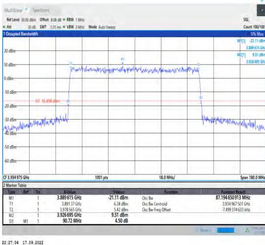
1-N77-3700-3980--30-90-H-9-CP-256QAM-Outer_Full -245@0-Ant1-87.195-90.720-<90-PASS
