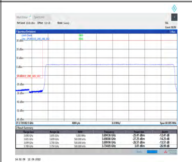
1-N77-3700-3980--30-50-L-6-CP-QPSK-Outer_Full-133@0-Ant1-1--PASS-see graph
