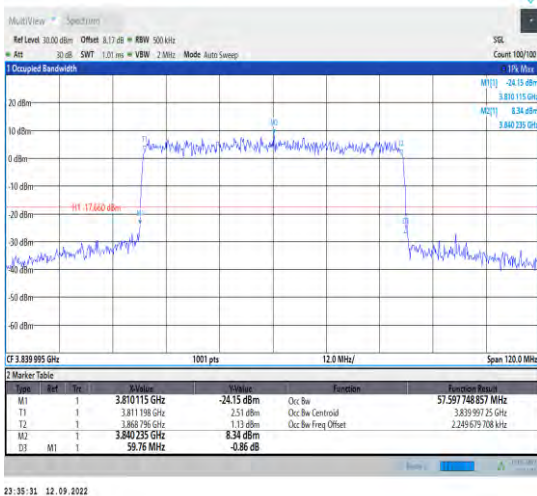
1-N77-3700-3980--30-60-M-9-CP-256QAM-Outer_Full ull-162@0-Ant1-57.598-59.760-≤60-PASS
