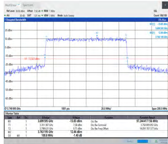
1-N77-3700-3980--30-100-L-7-CP-16QAM-Outer_Fu ll-273@0-Ant1-97.244-100.800-≤100-PASS
