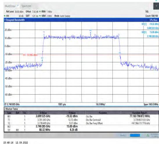
1-N77-3700-3980--30-80-L-3-DFT-16QAM-Outer_Full-216@0-Ant1-77.184-80.320-<=80-PASS
