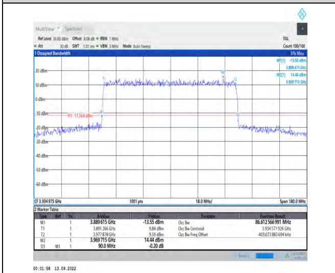
1-N77-3700-3980--30-90-H-1-DFT-QPSK-Outer_Full -243@0-Ant1-86.613-90.000-≤90-PASS
