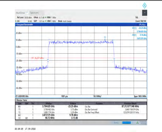
1-N77-3700-3980--30-90-M-9-CP-256QAM-Outer_F ull-245@0-Ant1-87.312-90.720-≤90-PASS
