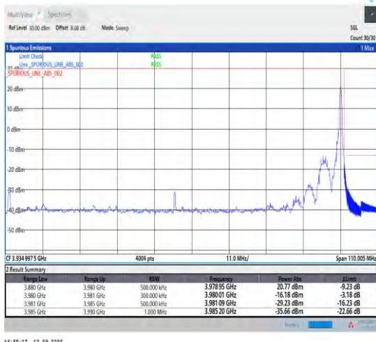
1-N77-3700-3980--30-100-H-5-CP-QPSK-Edge_1RB_Right-1@272-Ant1-1--PASS-see graph
