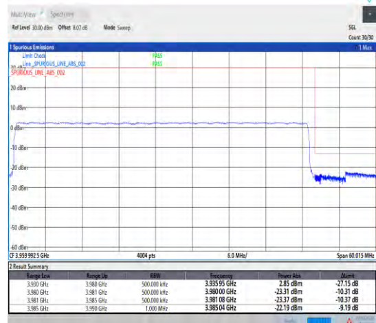
1-N77-3700-3980--30-50-H-6-CP-QPSK-Outer_Full-133@0-Ant1-1--PASS-see graph
