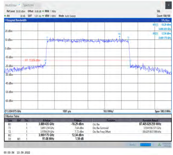
1-N77-3700-3980--30-90-H-8-CP-64QAM-Outer_Full -245@0-Ant1-87.405-91.080-<90-PASS
