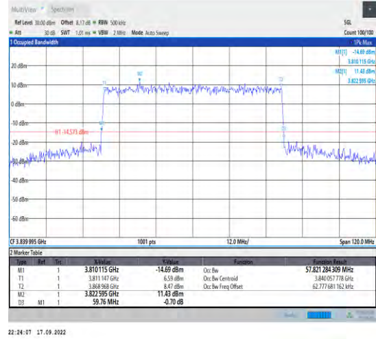
1-N77-3700-3980--30-60-M-8-CP-64QAM-Outer_Full -162@0-Ant1-57.821-59.760-≤60-PASS
