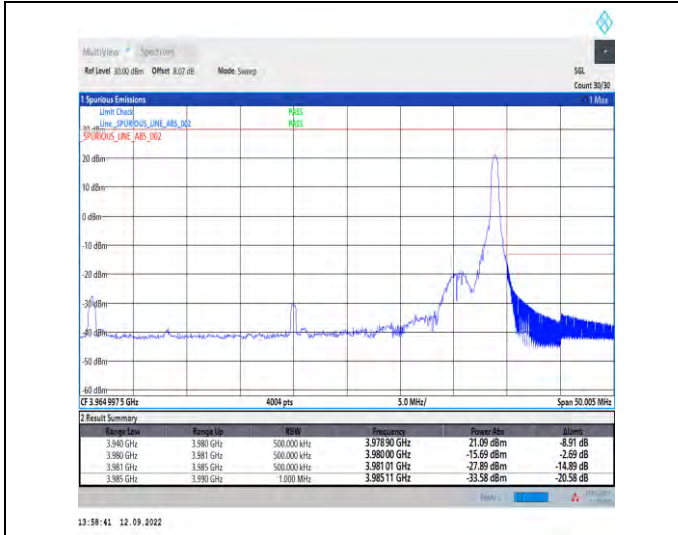
1-N77-3700-3980--30-40-H-2-DFT-PI2BPSK-Edge_1R B_Right-1@105-Ant1-1--PASS-see graph
