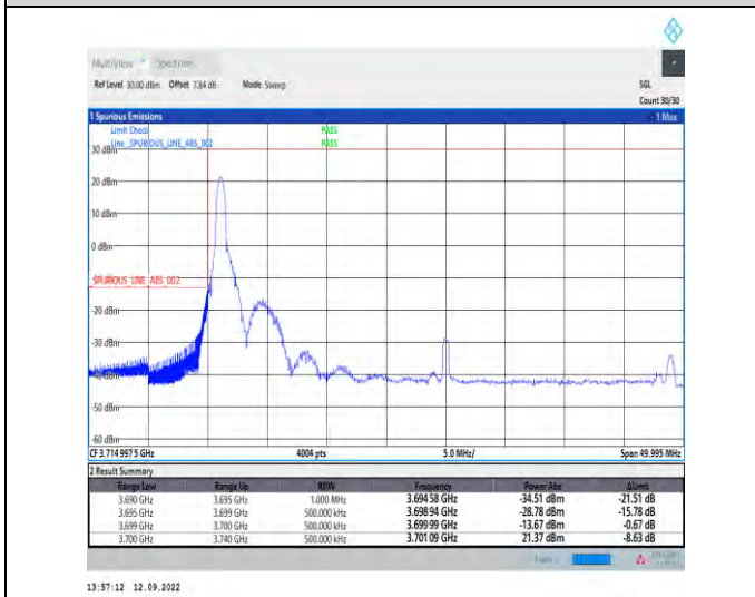
1-N77-3700-3980--30-40-L-4-CP-QPSK-Edge_1RB_L_eff-1@0-Ant1-1--PASS-see graph
