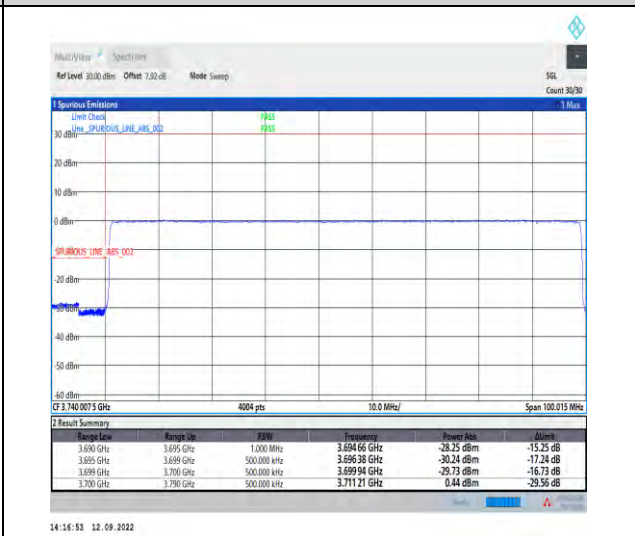
1-N77-3700-3980--30-90-L-6-CP-QPSK-Outer_Full-245@0-Ant1-1--PASS-see graph
