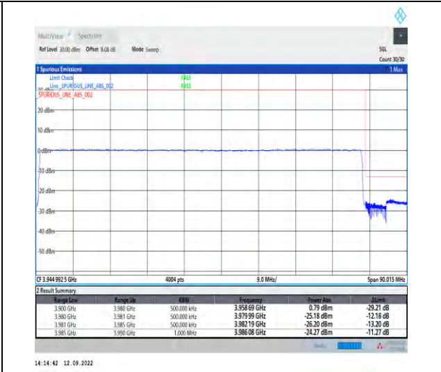
1-N77-3700-3980--30-80-H-3-DFT-PI2BPSK-Outer_Full-216@0-Ant1-1--PASS-see graph
