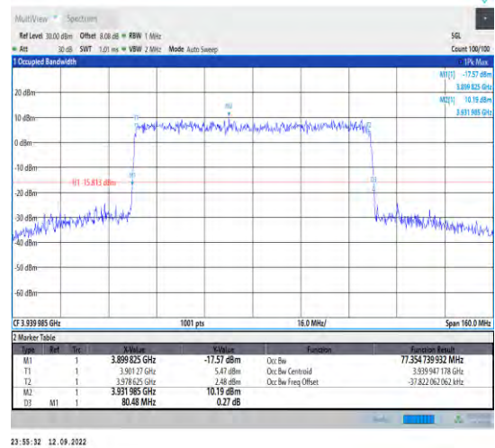
1-N77-3700-3980--30-80-H-9-CP-256QAM-Outer_Fu ll-217@0-Ant1-77.355-80.480-<80-PASS
