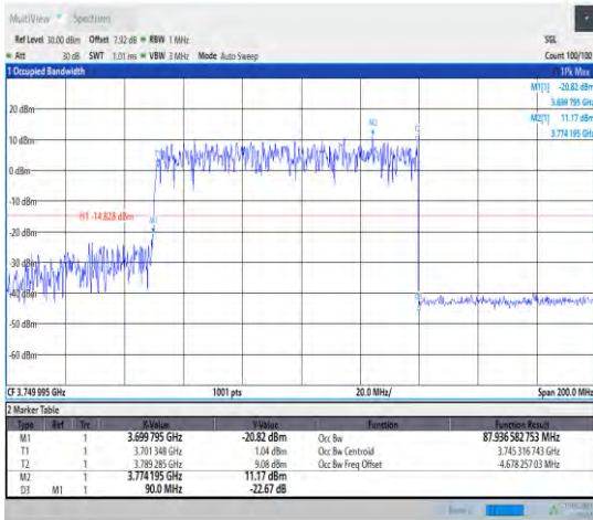
1-N77-3700-3980--30-100-L-6-CP-QPSK-Outer_Full -273@0-Ant1-87.937-90.000-≤100-PASS
