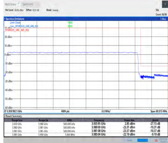
1-N77-3700-3980--30-50-H-3-DFT-PI2BPSK-Outer_Full-128@0-Ant1-1--PASS-see graph
