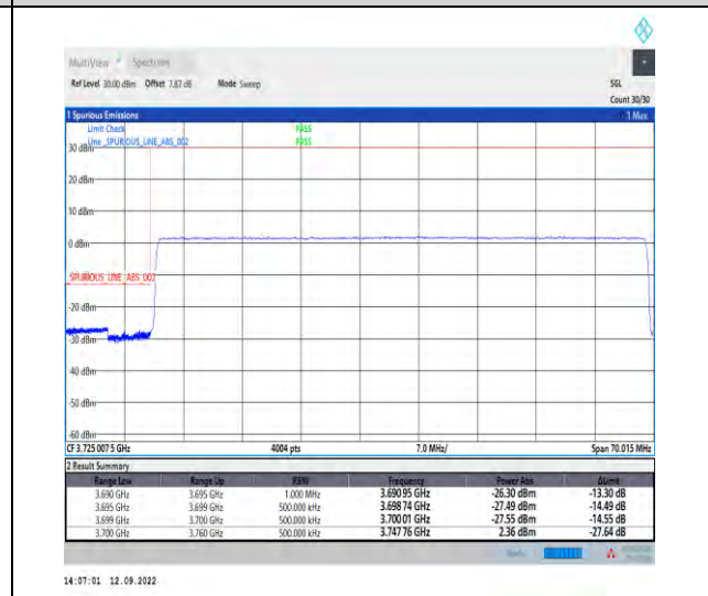
1-N77-3700-3980--30-60-L-6-CP-QPSK-Outer_Full-162@0-Ant1-1--PASS-see graph
