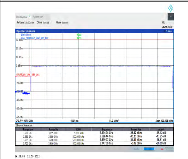
1-N77-3700-3980--30-100-L-6-CP-QPSK-Outer_Full-273@0-Ant1-1--PASS-see graph
