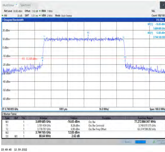
1-N77-3700-3980--30-80-L-8-CP-64QAM-Outer_Full -217@0-Ant1-77.273-80.640-<80-PASS
