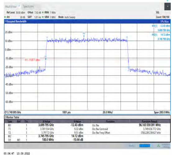
1-N77-3700-3980--30-100-L-1-DFT-QPSK-Outer_Full -270@0-Ant1-96.166-100.000-<100-PASS
