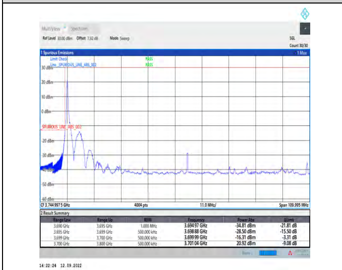
1-N77-3700-3980--30-100-L-4-CP-QPSK-Edge_1RB_Left-1@0-Ant1-1--PASS-see graph
