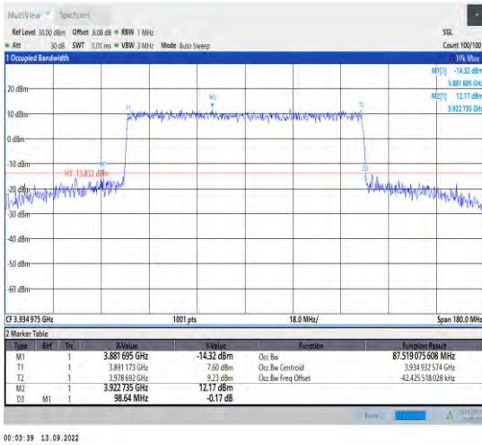
1-N77-3700-3980--30-90-H-7-CP-16QAM-Outer_Full -245@0-Ant1-87.519-98.640-<90-PASS
