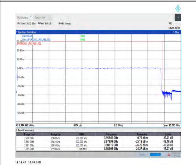
1-N77-3700-3980--30-80-H-6-CP-QPSK-Outer_Ful l-217@0-Ant1-1--PASS-see graph
