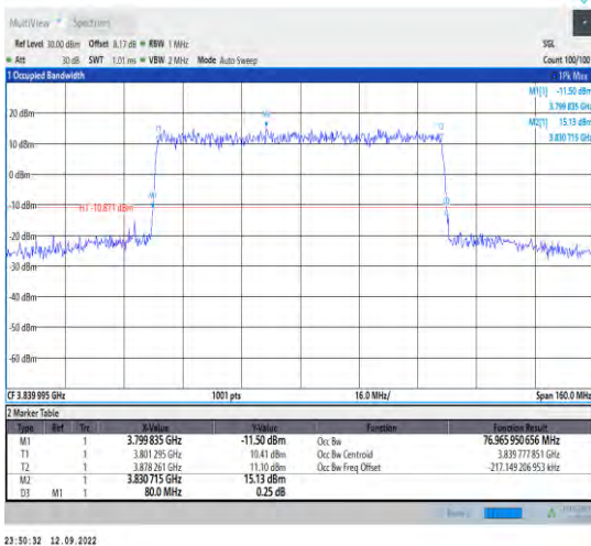
1-N77-3700-3980--30-80-M-1-DFT-QPSK-Outer_Full -216@0-Ant1-76.966-80.000-<80-PASS
