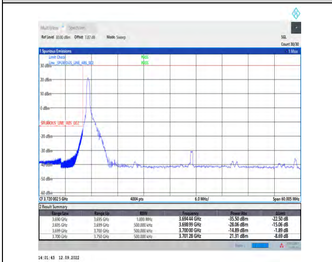
1-N77-3700-3980--30-50-L-4-CP-QPSK-Edge_1RB_L_eff-1@0-Ant1-1--PASS-see graph
