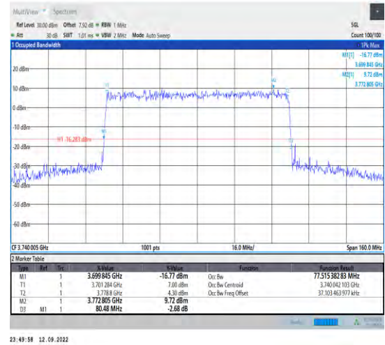
1-N77-3700-3980--30-80-L-9-CP-256QAM-Outer_Fu ll-217@0-Ant1-77.515-80.480-<80-PASS
