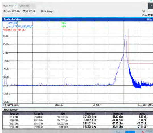
1-N77-3700-3980--30-50-H-5-CP-QPSK-Edge_1RB_Right-1@132-Ant1-1--PASS-see graph
