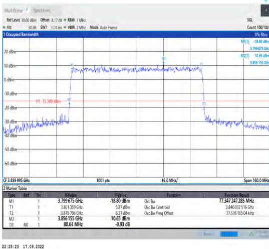
1-N77-3700-3980--30-80-M-9-CP-256QAM-Outer_Full ull-217@0-Ant1-77.347-80.640-<80-PASS
