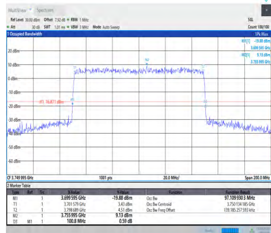
1-N77-3700-3980--30-100-L-9-CP-256QAM-Outer_F ull-273@0-Ant1-97.11-100.800-≤100-PASS
