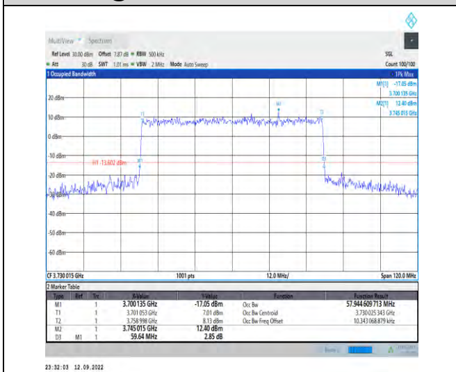
1-N77-3700-3980--30-60-L-6-CP-QPSK-Outer_Full 162@0-Ant1-57.945-59.640-≤60-PASS
