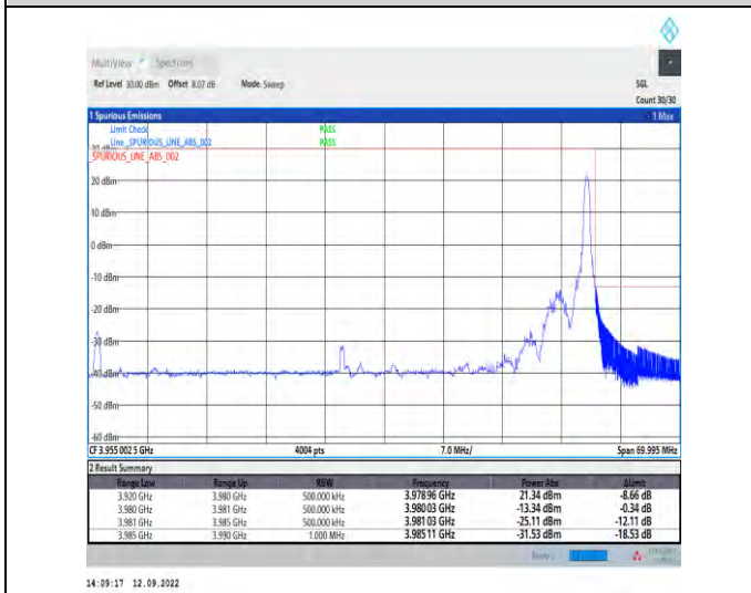
1-N77-3700-3980--30-60-H-5-CP-QPSK-Edge_1RB_R ight-1@161-Ant1-1--PASS-see graph
