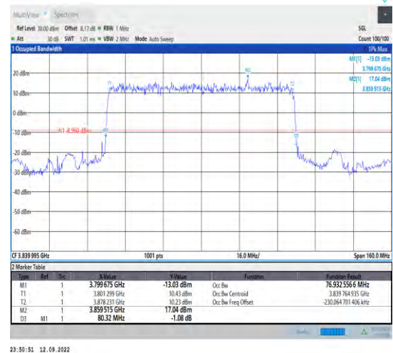
1-N77-3700-3980--30-80-M-2-DFT-PI2BPSK-Outer_Full Full-216@0-Ant1-76.933-80.320-<80-PASS
