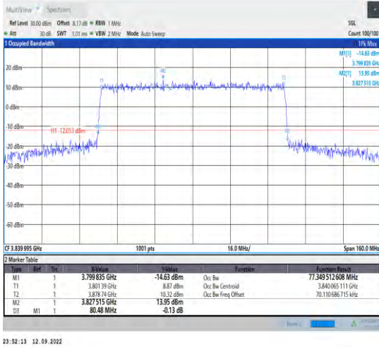
1-N77-3700-3980--30-80-M-7-CP-16QAM-Outer_Full I-217@0-Ant1-77.35-80.480-<80-PASS
