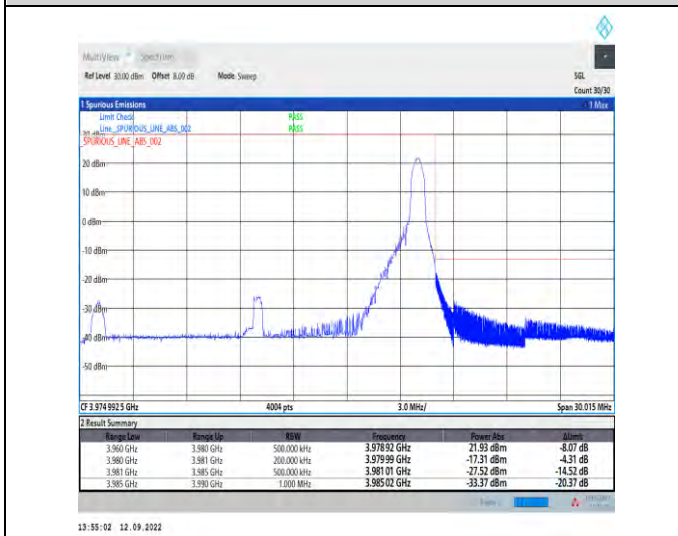
1-N77-3700-3980--30-20-H-5-CP-QPSK-Edge_1RB_Right-1@50-Ant1-1--PASS-see graph
