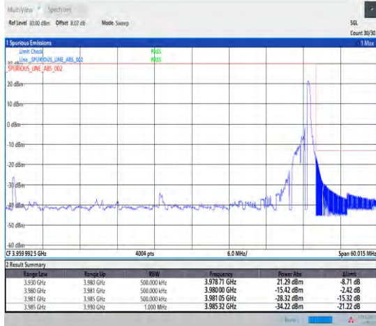
1-N77-3700-3980--30-50-H-2-DFT-PI2BPSK-Edge_1R_B_Right-1@132-Ant1-1--PASS-see graph
