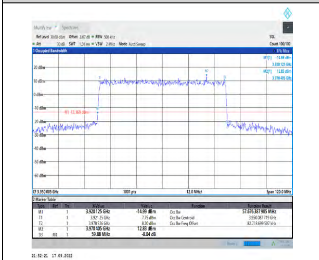
1-N77-3700-3980--30-60-H-4-DFT-64QAM-Outer_Full-162@0-Ant1-57.676-59.880-<60-PASS
