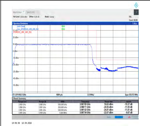
1-N77-3700-3980--30-20-H-3-DFT-PI2BPSK-Outer_Full-50@0-Ant1-1--PASS-see graph
