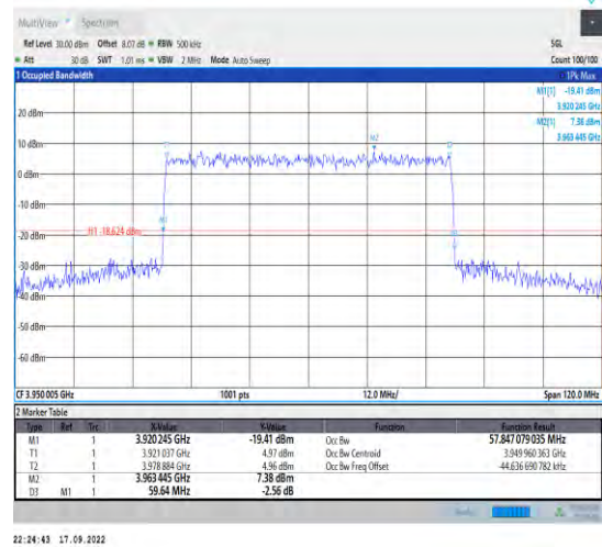
1-N77-3700-3980--30-60-H-9-CP-256QAM-Outer_Fu ll-162@0-Ant1-57.847-59.640-<60-PASS
