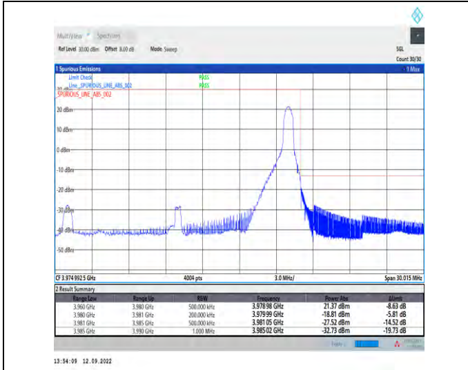
1-N77-3700-3980--30-20-H-2-DFT-PI2BPSK-Edge_1R_B_Right-1@50-Ant1-1--PASS-see graph
