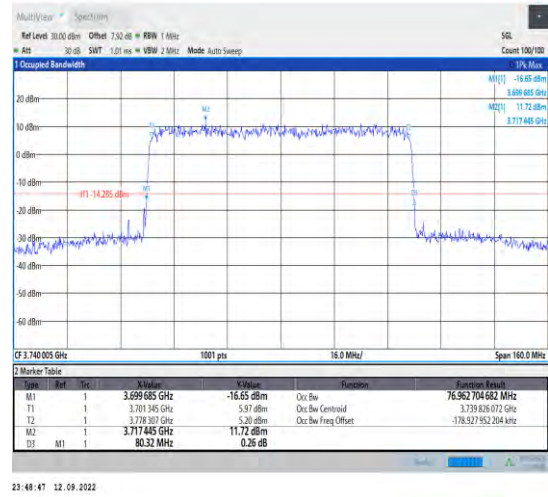
1-N77-3700-3980--30-80-L-5-DFT-256QAM-Outer_F ull-216@0-Ant1-76.963-80.320-≤80-PASS
