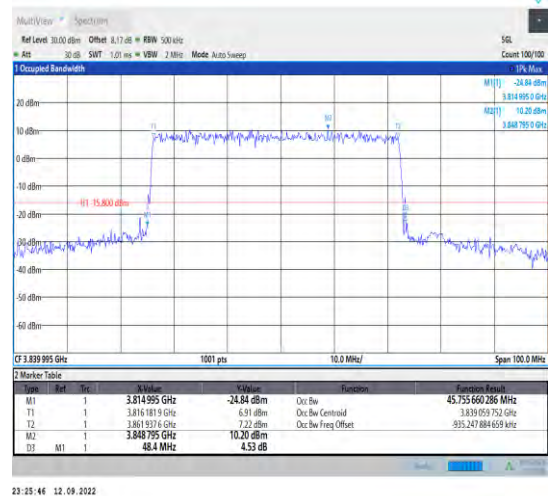
1-N77-3700-3980--30-50-M-5-DFT-256QAM-Outer_F Full-128@0-Ant1-45.756-48.400-<=50-PASS
