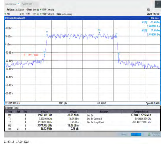
1-N77-3700-3980--30-20-H-4-DFT-64QAM-Outer_Fu II-50@0-Ant1-17.808-18.920-<20-PASS
