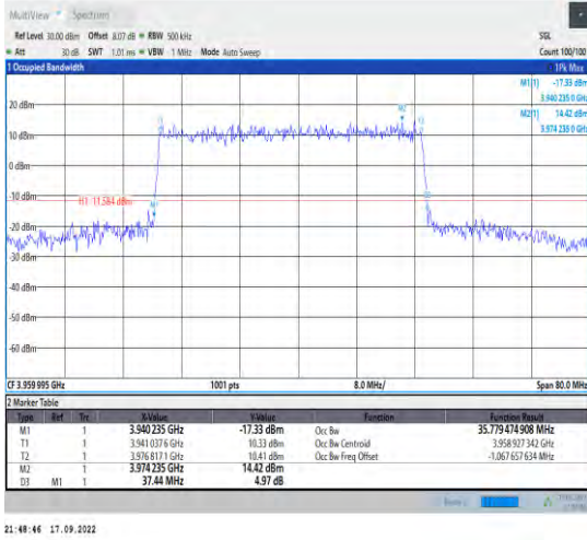
1-N77-3700-3980--30-40-H-4-DFT-64QAM-Outer_Fu II-100@0-Ant1-35.779-37.440-<40-PASS
