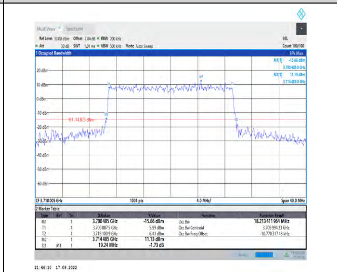
1-N77-3700-3980--30-20-L-8-CP-64QAM-Outer_Full-51@0-Ant1-18.213-19.240-≤20-PASS
