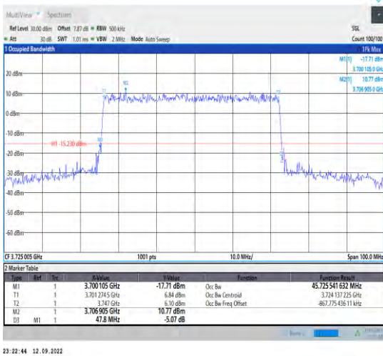
1-N77-3700-3980--30-50-L-5-DFT-256QAM-Outer_F ull-128@0-Ant1-45.726-47.800-≤50-PASS
