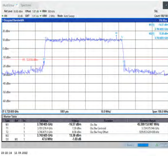
1-N77-3700-3980--30-50-L-3-DFT-16QAM-Outer_Fu I1-128@0-Ant1-45.599-47.600-≤50-PASS
