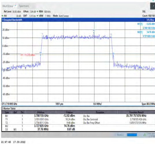
1-N77-3700-3980--30-40-L-4-DFT-64QAM-Outer_Full-100@0-Ant1-35.792-37.760-<40-PASS
