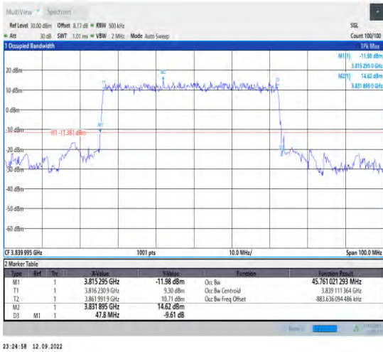
1-N77-3700-3980--30-50-M-2-DFT-PI2BPSK-Outer_F Full-128@0-Ant1-45.761-47.800-<=50-PASS
