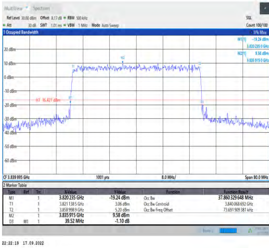
1-N77-3700-3980--30-40-M-9-CP-256QAM-Outer_Full-106@0-Ant1-37.86-39.520-<40-PASS
