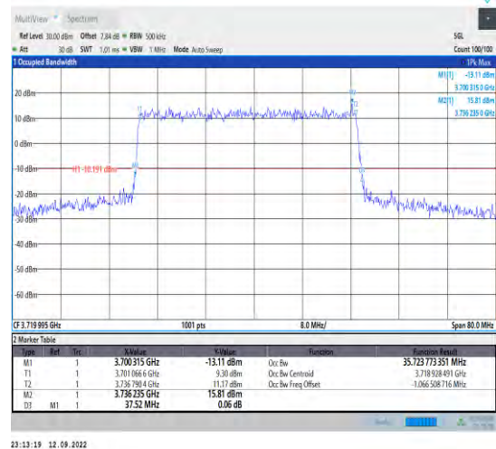
1-N77-3700-3980--30-40-L-1-DFT-QPSK-Outer_Full 100@0-Ant1-35.724-37.520-≤40-PASS
