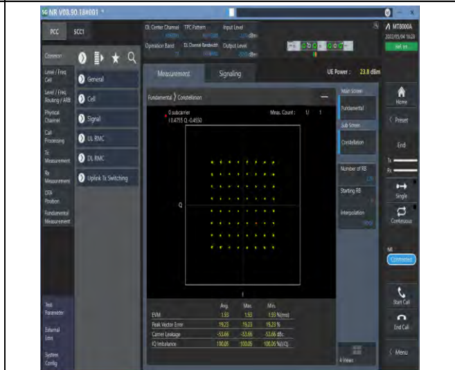
1-N77-3700-3980-PC2-30-100-M-4-DFT-64QAM-Out_Full-270@0-Ant1-see graph-PASS
