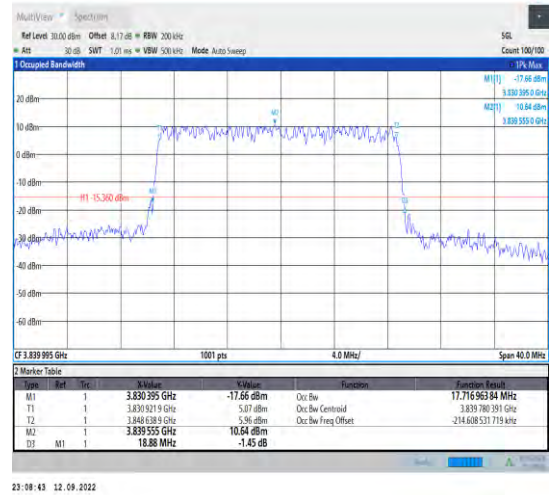
1-N77-3700-3980--30-20-M-5-DFT-256QAM-Outer_Full-50@0-Ant1-17.717-18.880-≤20-PASS
