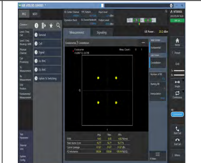
1-N77-3700-3980-PC2-30-100-M-6-CP-QPSK-Outer_Full-273@0-Ant1-see graph-PASS
