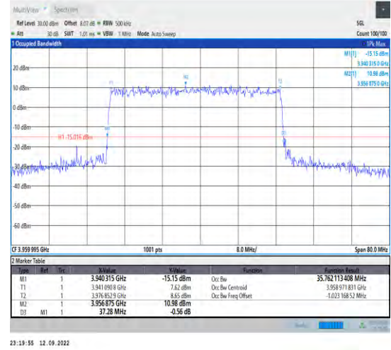
1-N77-3700-3980--30-40-H-5-DFT-256QAM-Outer_F ull-100@0-Ant1-35.762-37.280-<40-PASS
