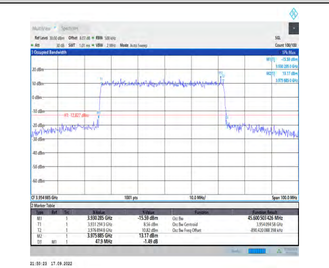
1-N77-3700-3980--30-50-H-4-DFT-64QAM-Outer_Fu II-128@0-Ant1-45.601-47.900-≤50-PASS
