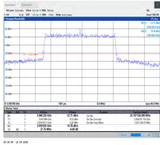
1-N77-3700-3980--30-40-H-1-DFT-QPSK-Outer_Full-100@0-Ant1-35.748-37.760-<40-PASS
