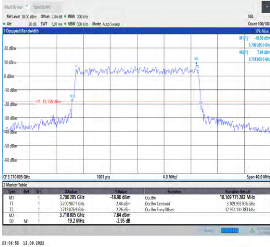
1-N77-3700-3980--30-20-L-9-CP-256QAM-Outer_Fu II-51@0-Ant1-18.17-19.200-<20-PASS
