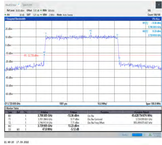
1-N77-3700-3980--30-50-L-4-DFT-64QAM-Outer_Ful I1-128@0-Ant1-45.629-47.800-≤50-PASS
