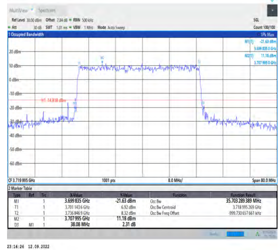
1-N77-3700-3980--30-40-L-5-DFT-256QAM-Outer_Full-100@0-Ant1-35.703-38.080-<40-PASS
