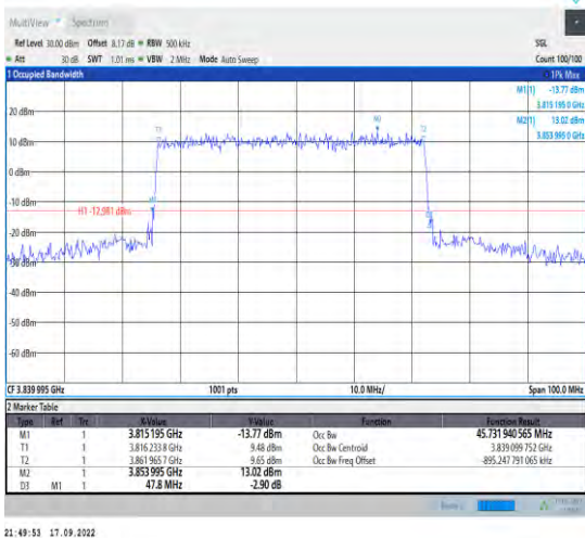
1-N77-3700-3980--30-50-M-4-DFT-64QAM-Outer_F ull-128@0-Ant1-45.732-47.800-<=50-PASS
