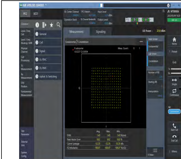
1-N77-3700-3980-PC2-30-100-M-5-DFT-256QAM-Outer_Full-270@0-Ant1-see graph-PASS
