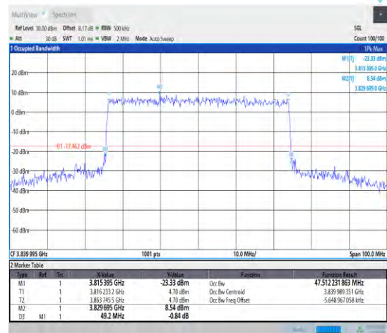
1-N77-3700-3980--30-50-M-9-CP-256QAM-Outer_Full-133@0-Ant1-47.512-49.200-<50-PASS
