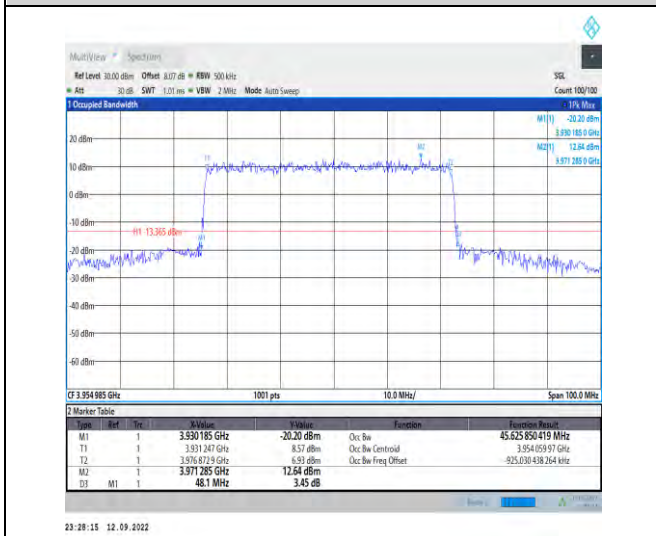
1-N77-3700-3980--30-50-H-3-DFT-16QAM-Outer_Fu II-128@0-Ant1-45.626-48.100-≤50-PASS
