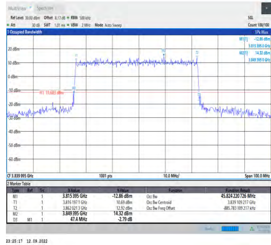
1-N77-3700-3980--30-50-M-3-DFT-16QAM-Outer_F ull-128@0-Ant1-45.824-47.400-<=50-PASS
