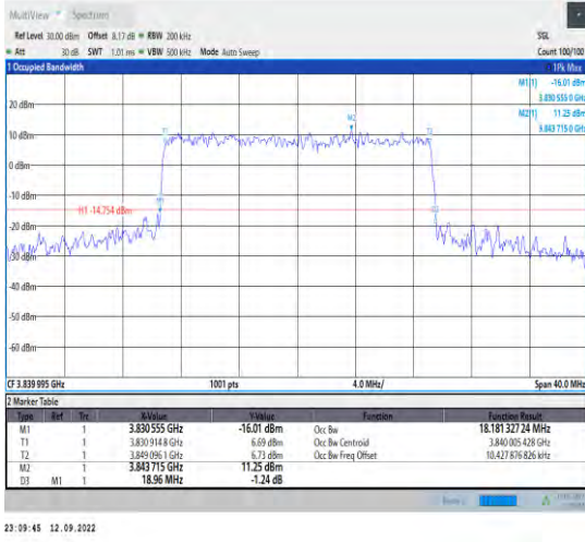
1-N77-3700-3980--30-20-M-8-CP-64QAM-Outer_Full-51@0-Ant1-18.181-18.960-<20-PASS
