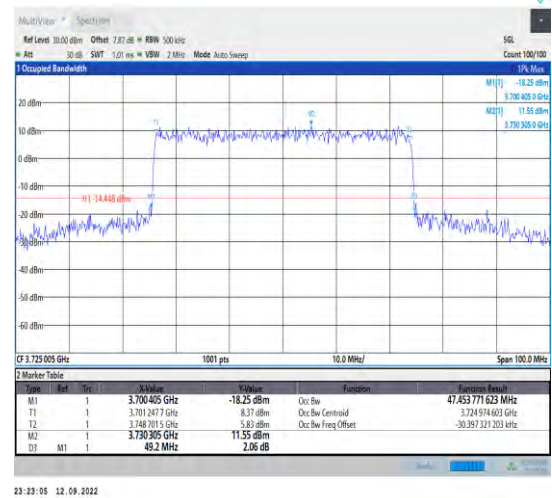
1-N77-3700-3980--30-50-L-6-CP-QPSK-Outer_Full-1 33@0-Ant1-47.454-49.200-≤50-PASS
