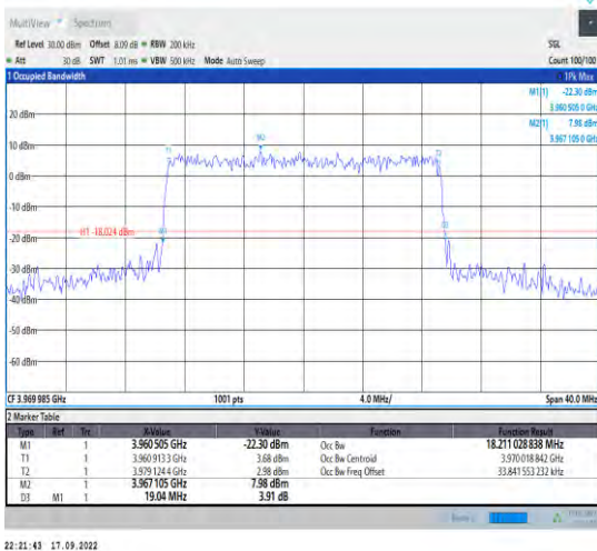
1-N77-3700-3980--30-20-H-9-CP-256QAM-Outer_Full -51@0-Ant1-18.211-19.040-≤20-PASS
