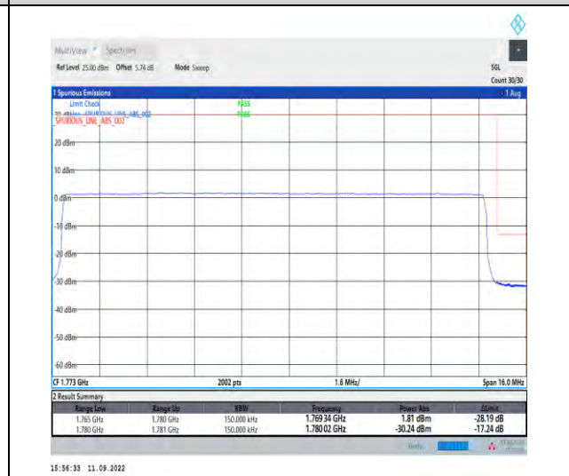
1-N66--15-15-H-6-CP-QPSK-Outer_Full-79@0-Ant1-1-seegraph-PASS-see graph
