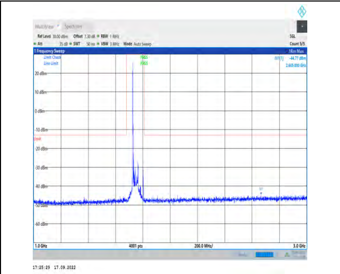
1-N66--15-40-M-1-DFT-PI2BPSK-Inner_1RB_Left-1 @1-1000-3000-Ant1-2665.00--44.77--13-PASS
