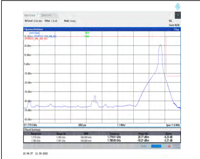
1-N66--15-10-H-2-DFT-PI2BPSK-Edge_1RB_Right-1@51-Ant1-1-seegraph-PASS-see graph
