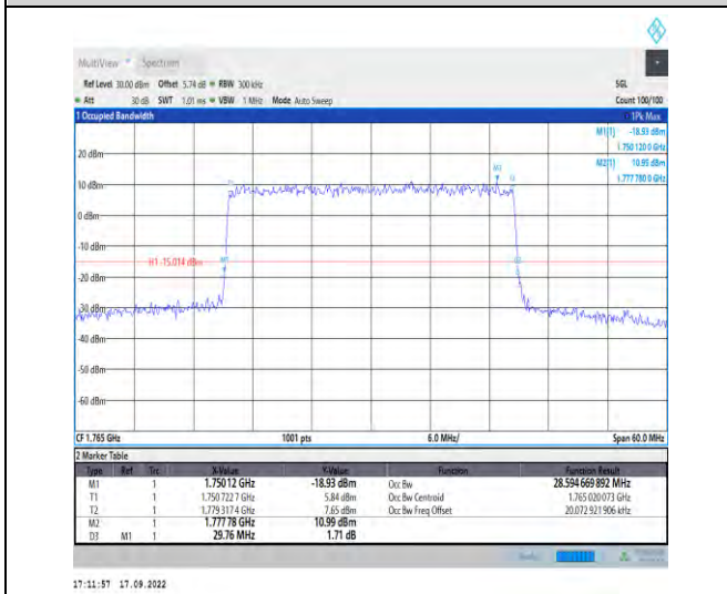
1-N66--15-30-H-5-DFT-256QAM-Outer_Full-160@0-A Ant1-28.595-29.760-≤30-PASS
