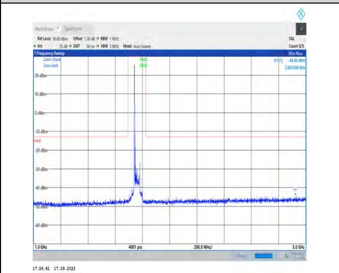
1-N66--15-40-H-1-DFT-PI2BPSK-Inner_1RB_Left-1 @ 1-1000-3000-Ant1-2923.50--44.43--13-PASS
