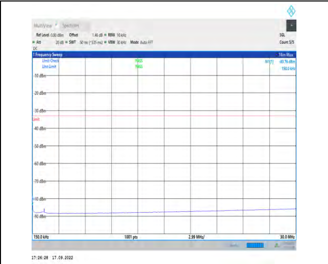
1-N66--15-40-H-1-DFT-PI2BPSK-Inner_1RB_Left-1 @ 1-0.15-30-Ant1-0.15--83.76--33-PASS
