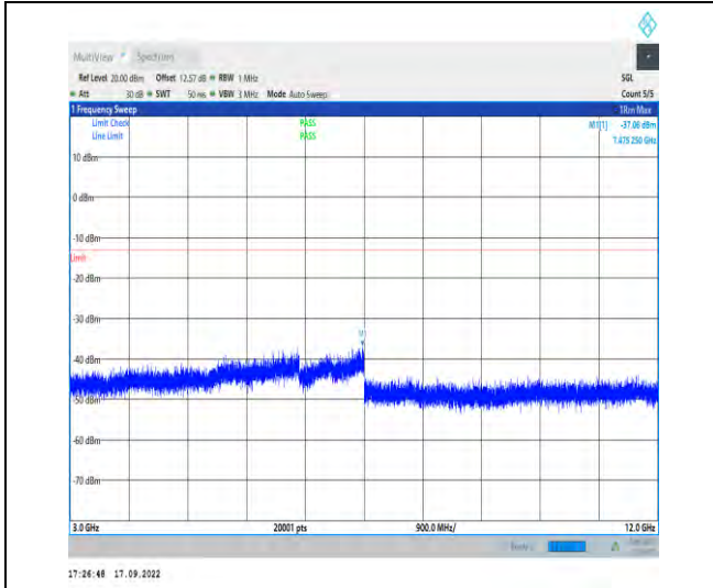
1-N66--15-40-H-1-DFT-PI2BPSK-Inner_1RB_Left-1 @ 1-3000-12000-Ant1-7475.25--37.06--13-PASS
