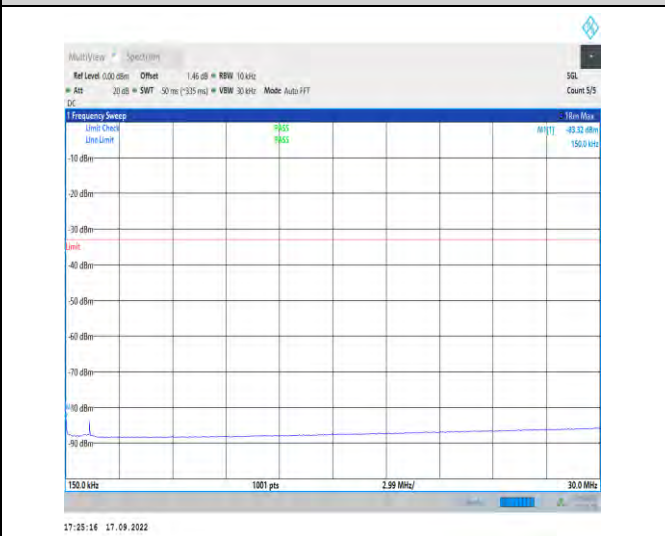
1-N66--15-40-M-1-DFT-PI2BPSK-Inner_1RB_Left-1 @ 1-0.15-30-Ant1-0.15--83.32--33-PASS
