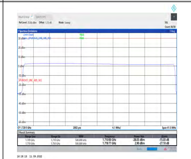
1-N66--15-40-L-6-CP-QPSK-Outer_Full-216@0-Ant1-1-seegraph-PASS-see graph
