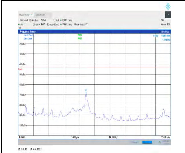
1-N66--15-40-H-1-DFT-PI2BPSK-Inner_1RB_Left-1 @ 1-0.009-0.15-Ant1-0.07--68.81--43-PASS
