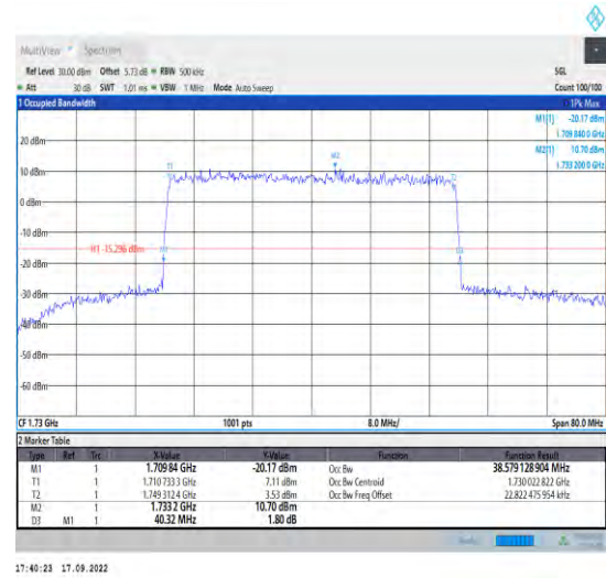
1-N66--15-40-L-9-CP-256QAM-Outer_Full-216@0-Ant1 nt1-38.579-40.320-<40-PASS
