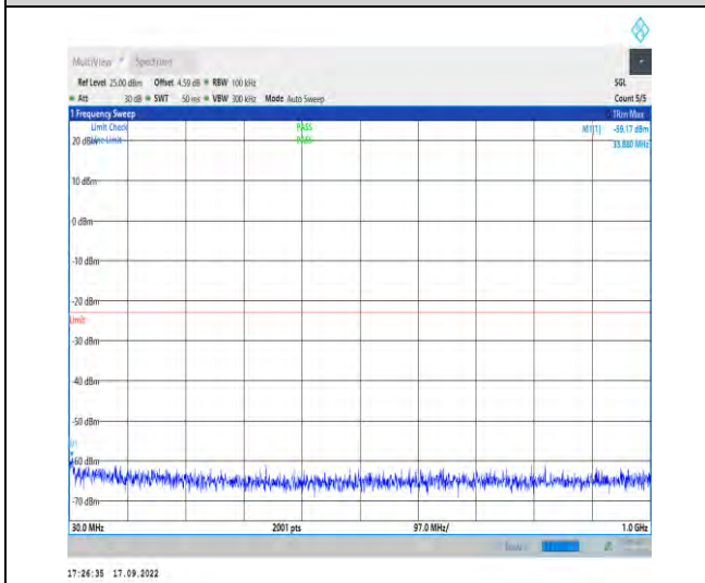
1-N66--15-40-H-1-DFT-PI2BPSK-Inner_1RB_Left-1 @ 1-30-1000-Ant1-33.88--59.17--23-PASS
