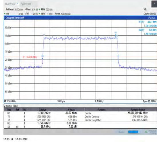
1-N66--15-30-M-9-CP-256QAM-Outer_Full-160@0- Ant1-28.621-29.700-≤30-PASS
