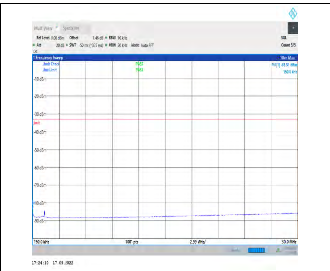
1-N66--15-40-L-1-DFT-PI2BPSK-Inner_1RB_Left-1@ 1-0.15-30-Ant1-0.15--83.51--33-PASS
