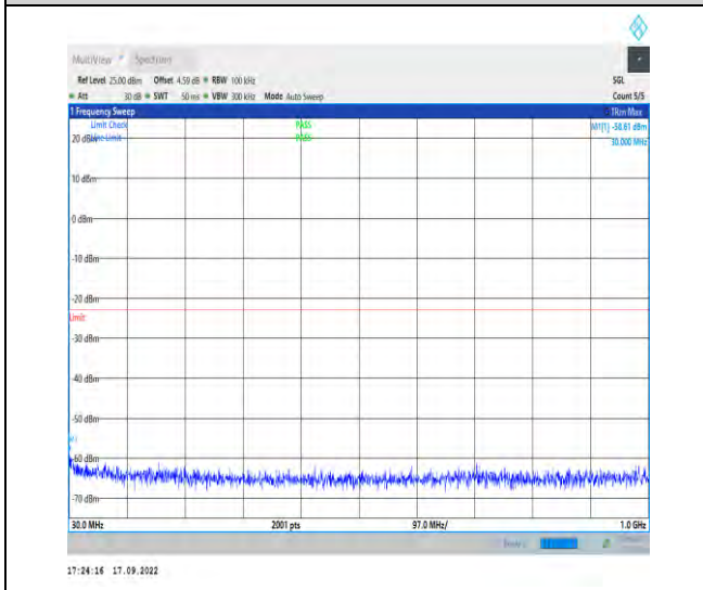
1-N66--15-40-L-1-DFT-PI2BPSK-Inner_1RB_Left-1 @1-30-1000-Ant1-30.00--58.61--23-PASS
