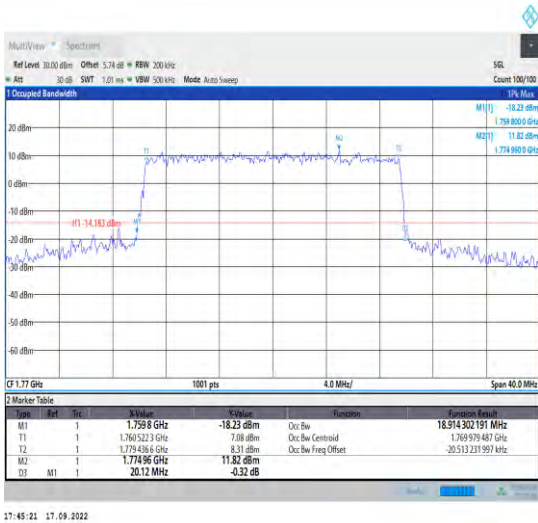
1-N66--15-20-H-8-CP-64QAM-Outer_Full-106@0-An t1-18.914-20.120-≤20-PASS
