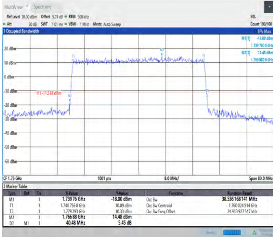
1-N66--15-40-H-4-DFT-64QAM-Outer_Full-216@0-A nt1-38.536-40.480-≤40-PASS
