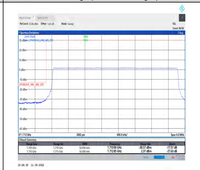
1-N66--15-5-L-6-CP-QPSK-Outer_Full-25@0-Ant1-1-seegraph-PASS-see graph
