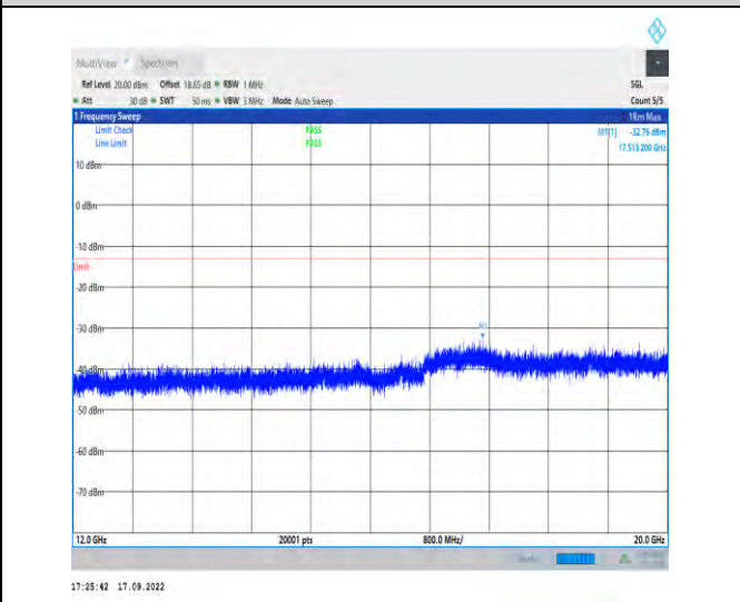
1-N66--15-40-M-1-DFT-PI2BPSK-Inner_1RB_Left-1 @1-12000-20000-Ant1-17513.20--32.76--13-PASS
