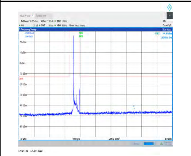
1-N66--15-40-L-1-DFT-PI2BPSK-Inner_1RB_Left-1@ 1-1000-3000-Ant1-2501.50--44.08--13-PASS
