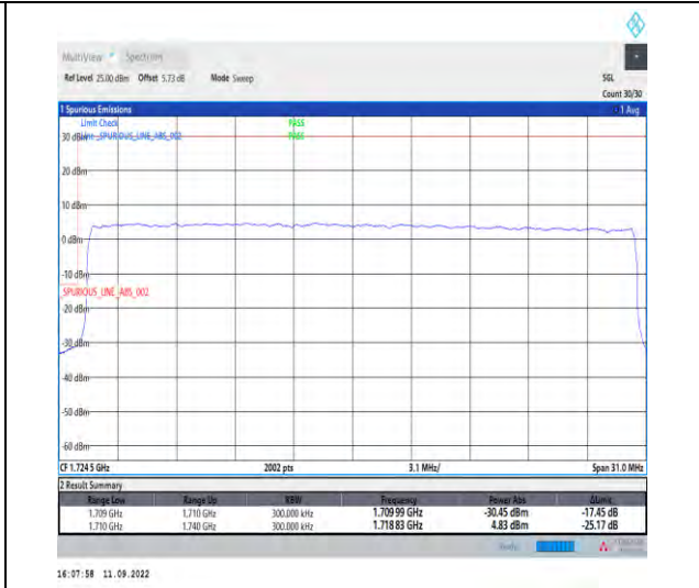
1-N66--15-30-L-3-DFT-PI2BPSK-Outer_Full-160@0-Ant1-1-seegraph-PASS-see graph
