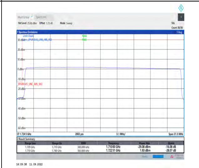
1-N66--15-30-L-6-CP-QPSK-Outer_Full-160@0-Ant1-1-seegraph-PASS-see graph
