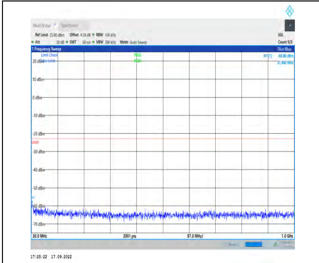
1-N66--15-40-M-1-DFT-PI2BPSK-Inner_1RB_Left-1 @1-30-1000-Ant1-31.94--58.80--23-PASS
