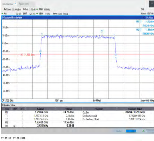
1-N66--15-30-L-5-DFT-256QAM-Outer_Full-160@0-Ant1-28.495-29.580-<30-PASS
