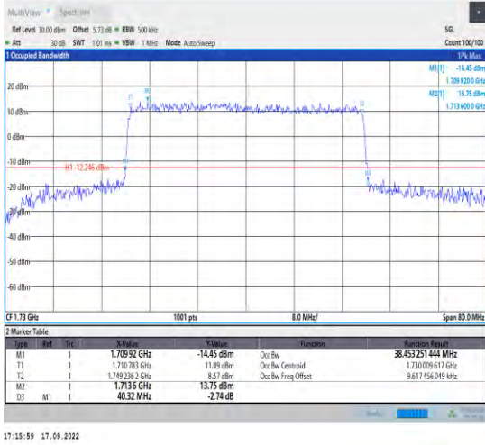
1-N66--15-40-L-6-CP-QPSK-Outer_Full-216@0-Ant1 -38.453-40.320-<40-PASS
