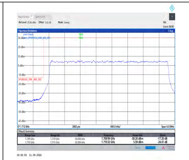
1-N66--15-5-L-3-DFT-PI2BPSK-Outer_Full-25@0-Ant1-1-seegraph-PASS-see graph
