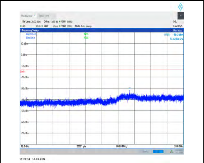
1-N66--15-40-H-1-DFT-PI2BPSK-Inner_1RB_Left-1 @ 1-12000-20000-Ant1-17362.80--33.43--13-PASS
