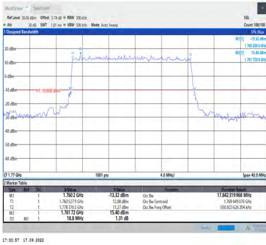
1-N66--15-20-H-2-DFT-PI2BPSK-Outer_Full-100@0-Ant1-17.842-18.800-≤20-PASS
