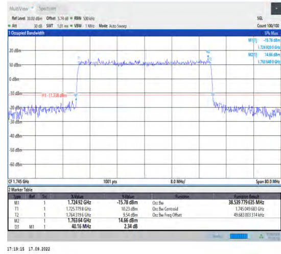
1-N66--15-40-M-6-CP-QPSK-Outer_Full-216@0-Ant 1-38.54-40.160-<40-PASS
