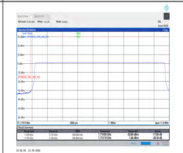
1-N66--15-10-L-6-CP-QPSK-Outer_Full-52@0-Ant1-1-seegraph-PASS-see graph
