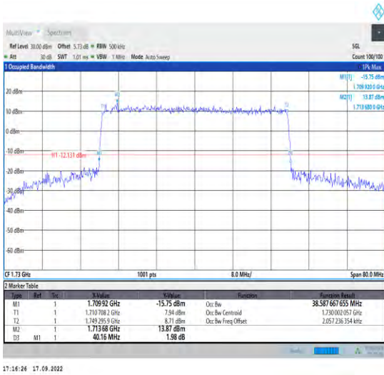
1-N66--15-40-L-8-CP-64QAM-Outer_Full-216@0-Ant1 t1-38.588-40.160-<40-PASS
