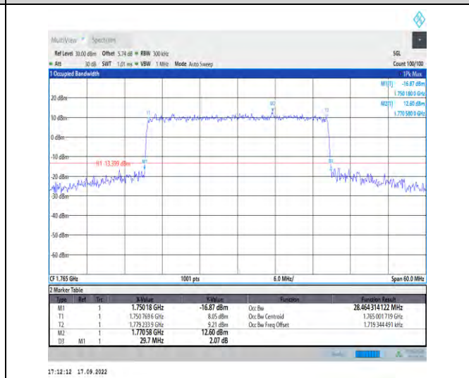
1-N66--15-30-H-6-CP-QPSK-Outer_Full-160@0-Ant 1-28.464-29.700-≤30-PASS
