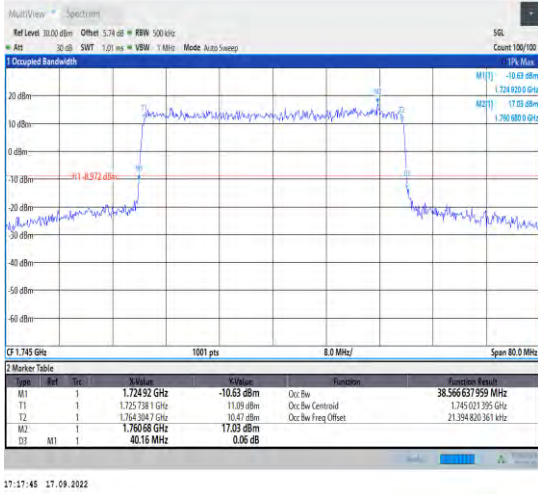
1-N66--15-40-M-1-DFT-QPSK-Outer_Full-216@0-An t1-38.567-40.160-≤40-PASS
