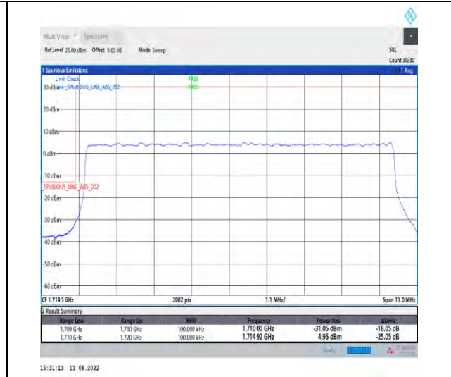
1-N66--15-10-L-3-DFT-PI2BPSK-Outer_Full-50@0-Ant1-1-seegraph-PASS-see graph
