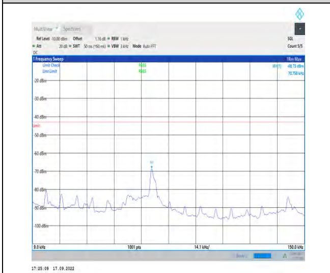
1-N66--15-40-M-1-DFT-PI2BPSK-Inner_1RB_Left-1 @ 1-0.009-0.15-Ant1-0.07--68.73--43-PASS
