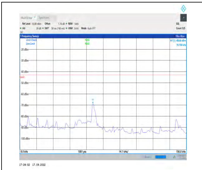
1-N66--15-40-L-1-DFT-PI2BPSK-Inner_1RB_Left-1 @1-0.009-0.15-Ant1-0.07--68.66--43-PASS
