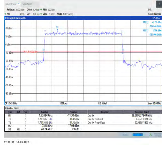
1-N66--15-40-M-2-DFT-PI2BPSK-Outer_Full-216@0-Ant1-38.669-40.240-≤40-PASS
