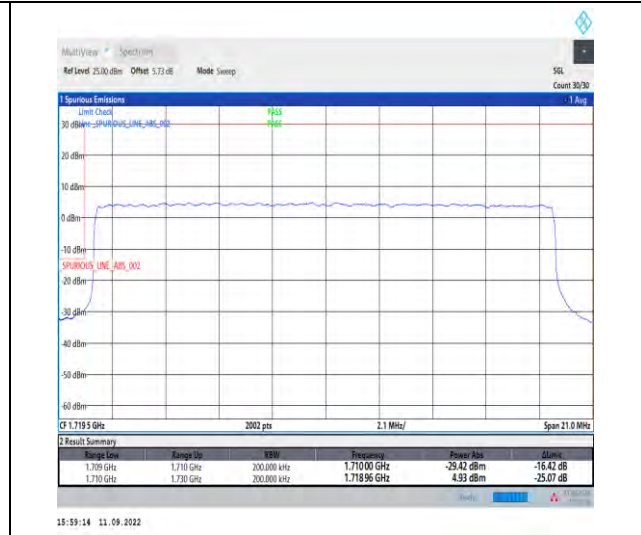
1-N66--15-20-L-3-DFT-PI2BPSK-Outer_Full-100@0-Ant1-1-seegraph-PASS-see graph
