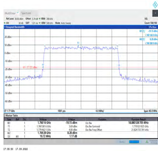
1-N66--15-20-H-9-CP-256QAM-Outer_Full-106@0-A nt1-18.881-19.720-≤20-PASS
