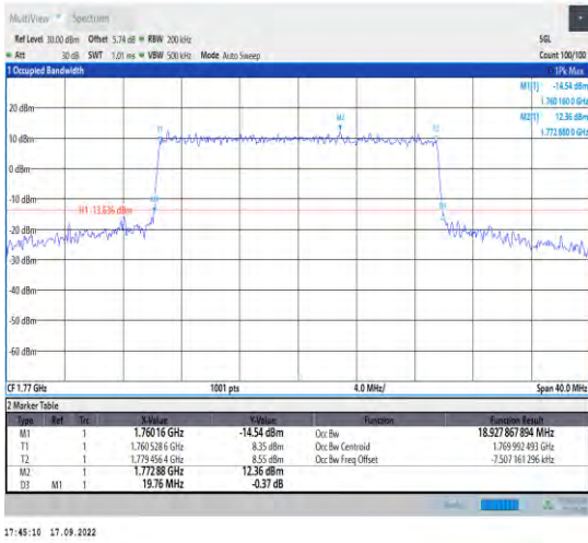
1-N66--15-20-H-6-CP-QPSK-Outer_Full-106@0-Ant t1-18.928-19.760-≤20-PASS
