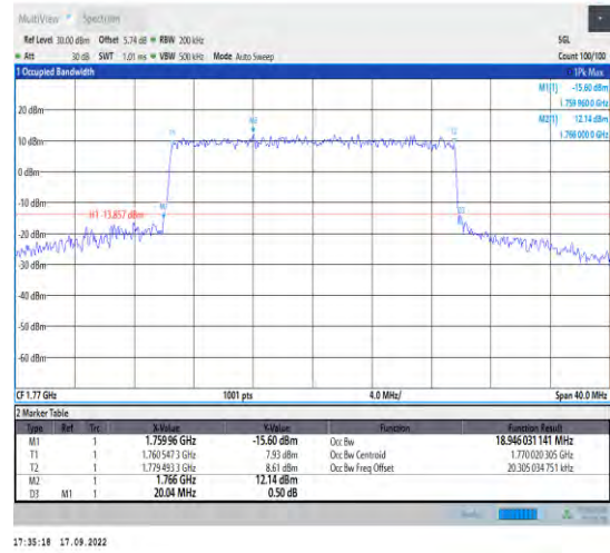
1-N66--15-20-H-7-CP-16QAM-Outer_Full-106@0-An t1-18.946-20.040-≤20-PASS
