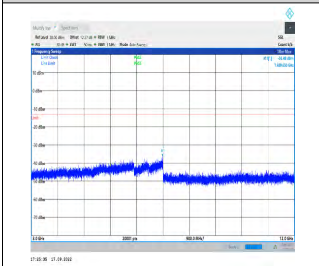
1-N66--15-40-M-1-DFT-PI2BPSK-Inner_1RB_Left-1 @1-3000-12000-Ant1-7489.65--36.48--13-PASS
