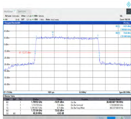
1-N66--15-40-L-3-DFT-16QAM-Outer_Full-216@0-Ant1-38.614-40.320-<40-PASS
