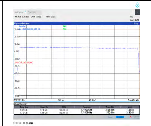
1-N66--15-40-L-3-DFT-PI2BPSK-Outer_Full-216@0-Ant1-1-seegraph-PASS-see graph
