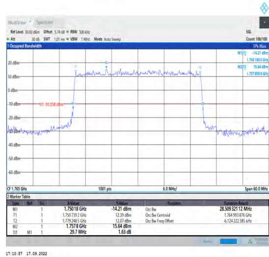
1-N66--15-30-H-2-DFT-PI2BPSK-Outer_Full-160@0- Ant1-28.509-29.700-≤30-PASS
