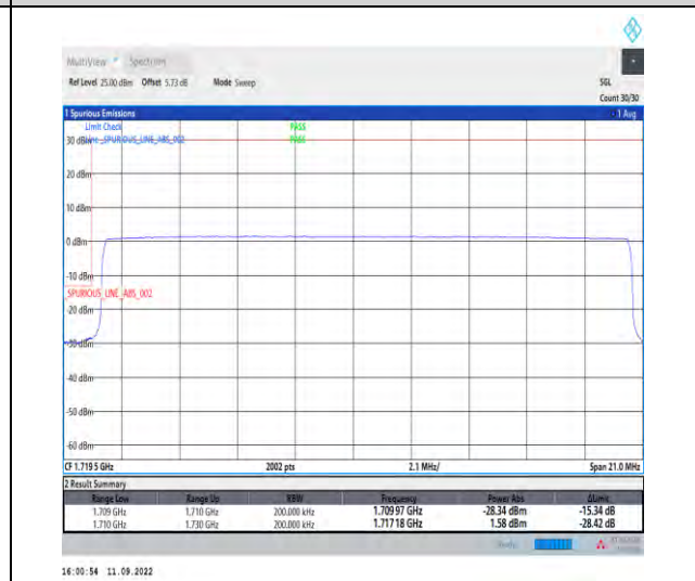
1-N66--15-20-L-6-CP-QPSK-Outer_Full-106@0-Ant1-1-seegraph-PASS-see graph
