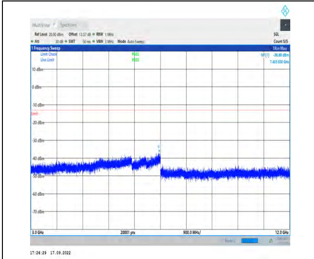
1-N66--15-40-L-1-DFT-PI2BPSK-Inner_1RB_Left-1 @ 1-3000-12000-Ant1-7463.55--36.89--13-PASS
