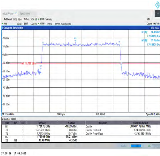
1-N66--15-40-M-3-DFT-16QAM-Outer_Full-216@0-A nt1-38.607-40.480-≤40-PASS
