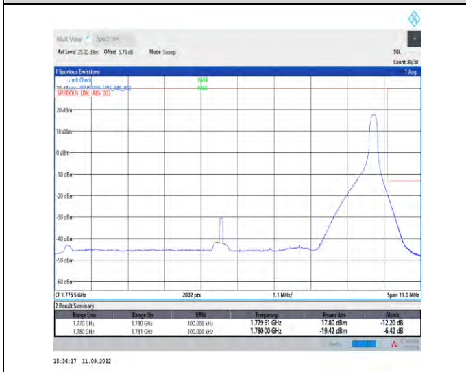
1-N66--15-10-H-5-CP-QPSK-Edge_1RB_Right-1@51-Ant1-1-seegraph-PASS-see graph
