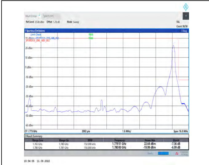
1-N66--15-15-H-2-DFT-PI2BPSK-Edge_1RB_Right-1@78-Ant1-1-seegraph-PASS-see graph
