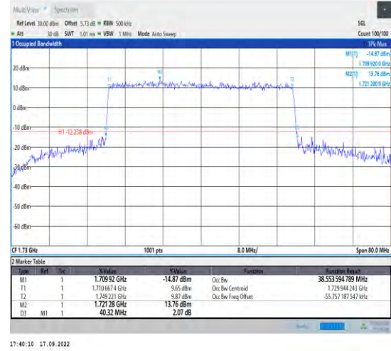
1-N66--15-40-L-7-CP-16QAM-Outer_Full-216@0-Ant1 t1-38.554-40.320-<40-PASS
