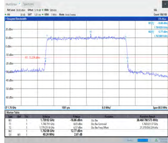
1-N66--15-40-H-5-DFT-256QAM-Outer_Full-216@0-A Ant1-38.461-40.240-≤40-PASS
