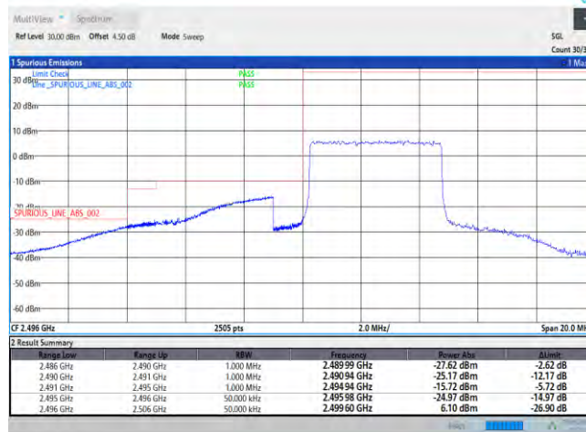
Band41-5MHz-QPSK-39675-25RB#0
