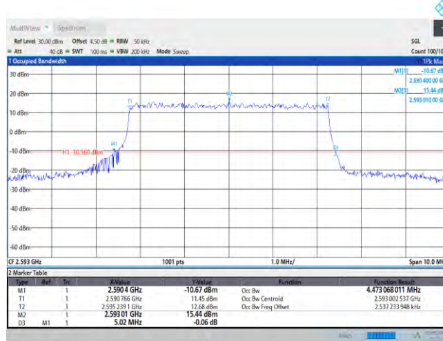
Band41-5MHz-QPSK-40620-25RB#0
