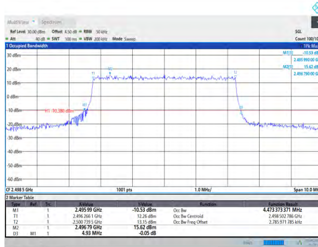
Band41-5MHz-QPSK-39675-25RB#0
