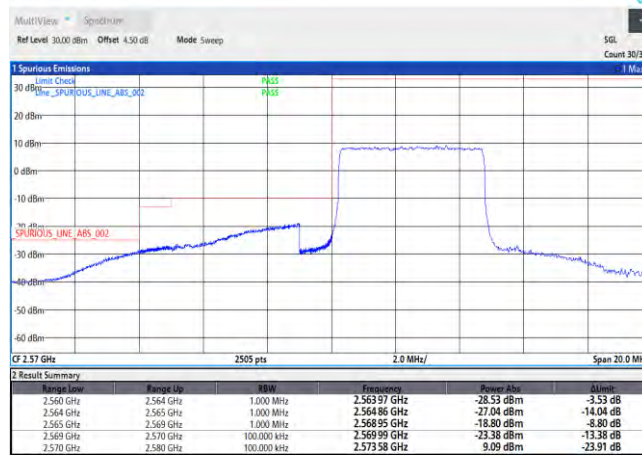
Band38-5MHz-QPSK-37775-25RB#0
