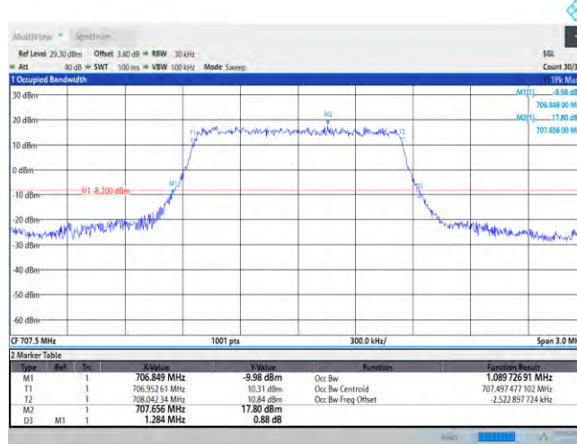
Band12-1.4MHz-QPSK-23095-6RB#0
