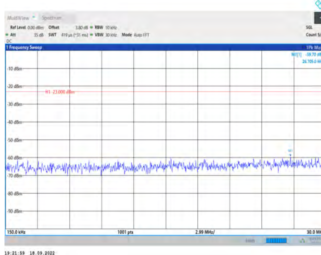
Band5-10MHz-QPSK-20450-1RB#0-Range2:0.15~30MHz
