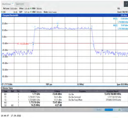
1-N66--15-15-L-3-DFT-16QAM-Outer_Full-75@0-Ant 1-13.417-14.250≤15-PASS
