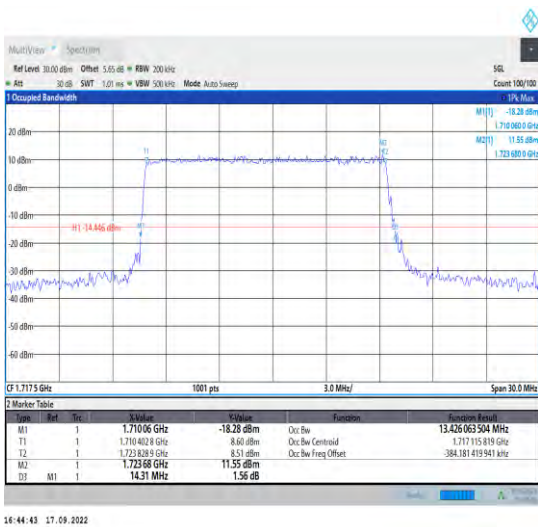
1-N66--15-15-L-5-DFT-256QAM-Outer_Full-75@0-A nt1-13.426-14.310≤15-PASS
