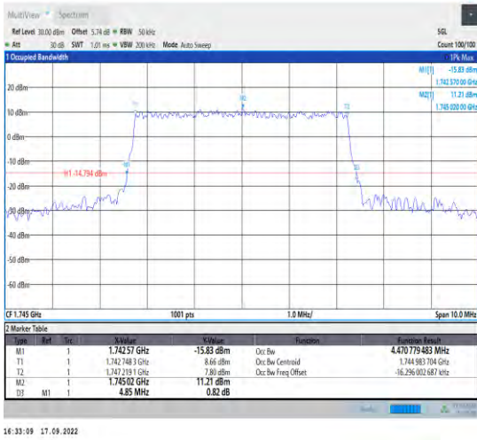
1-N66--15-5-M-8-CP-64QAM-Outer_Full-25@0-Ant1 -4.471-4.850-≤5-PASS
