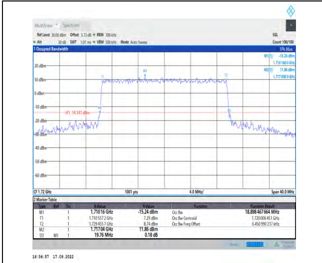
1-N66--15-20-L-8-CP-64QAM-Outer_Full-106@0-An t1-18.898-19.760-<20-PASS
