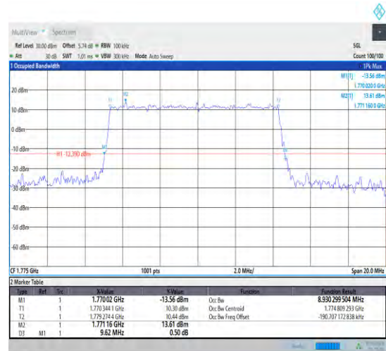
1-N66--15-10-H-1-DFT-QPSK-Outer_Full-50@0-Ant 1-8.915-9.500-≤10-PASS
