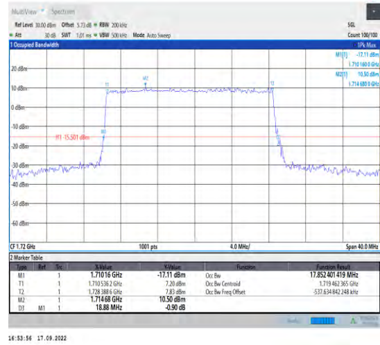
1-N66--15-20-L-5-DFT-256QAM-Outer_Full-100@0-A Ant1-17.852-18.880-≤20-PASS
