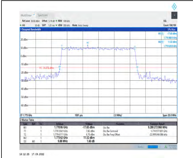
1-N66--15-10-H-8-CP-64QAM-Outer_Full-52@0-Ant 1-9.28-9.880≤10-PASS
