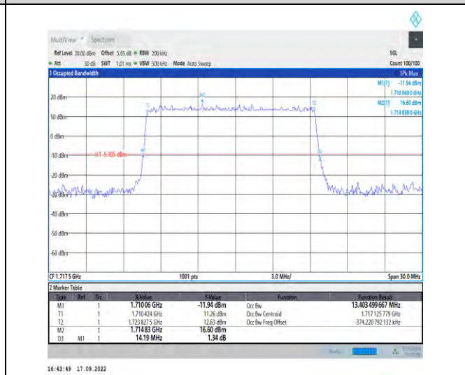
1-N66--15-15-L-2-DFT-PI2BPSK-Outer_Full-75@0-A nt1-13.403-14.190≤15-PASS
