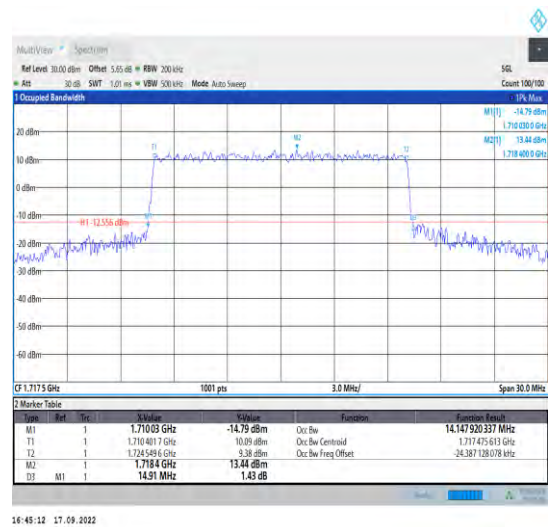
1-N66--15-15-L-6-CP-QPSK-Outer_Full-79@0-Ant1 14.148-14.910≤15-PASS
