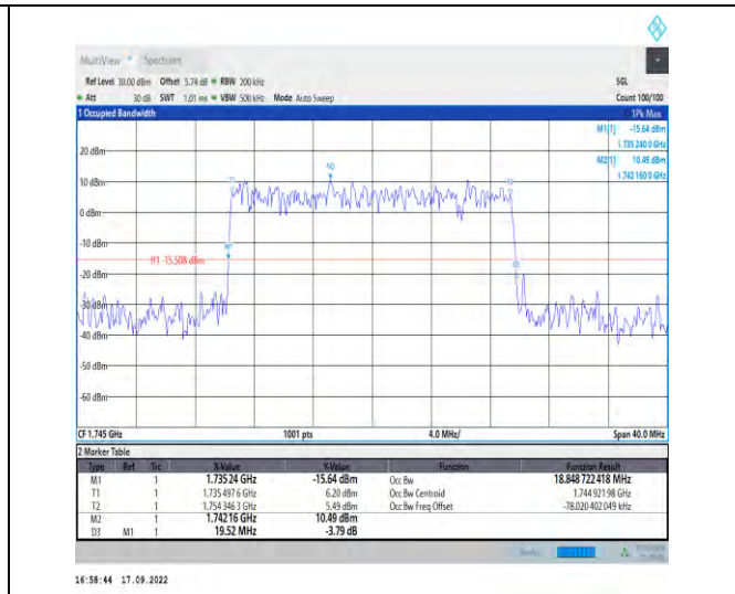
1-N66--15-20-M-8-CP-64QAM-Outer_Full-106@0-A nt1-18.849-19.520-≤20-PASS
