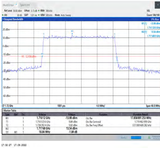
1-N66--15-20-L-4-DFT-64QAM-Outer_Full-100@0-A nt1-17.859-18.840-≤20-PASS
