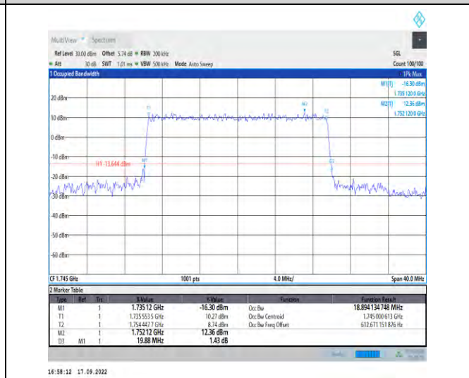
1-N66--15-20-M-6-CP-QPSK-Outer_Full-106@0-Ant 1-18.894-19.880-≤20-PASS
