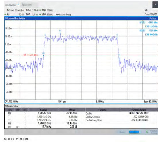
1-N66--15-15-H-6-CP-QPSK-Outer_Full-79@0-Ant1- 14.06-14.700≤15-PASS
