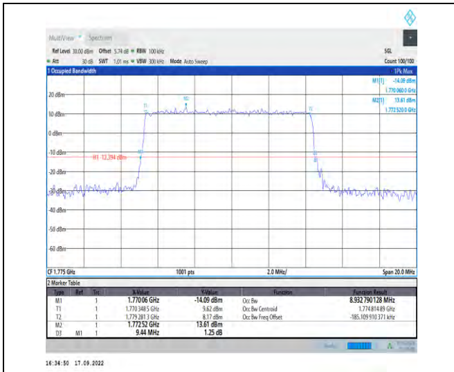
1-N66--15-10-H-4-DFT-64QAM-Outer_Full-50@0-An t1-8.933-9.440≤10-PASS
