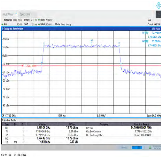
1-N66--15-15-H-7-CP-16QAM-Outer_Full-79@0-Ant 1-14.109-14.850≤15-PASS
