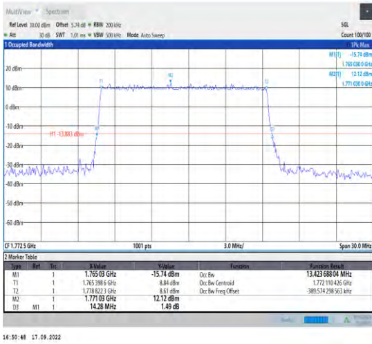
1-N66--15-15-H-5-DFT-256QAM-Outer_Full-75@0-A nt1-13.424-14.280≤15-PASS
