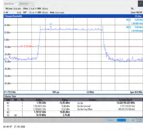
1-N66--15-15-H-2-DFT-PI2BPSK-Outer_Full-75@0-Ant t1-13.424-14.190≤15-PASS
