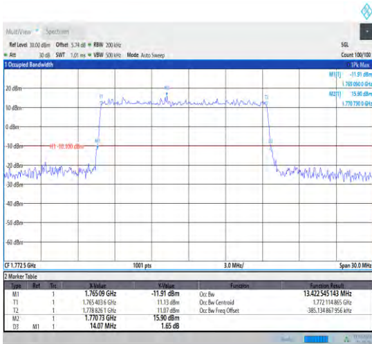
1-N66--15-15-H-1-DFT-QPSK-Outer_Full-75@0-Ant t1-13.425-14.160≤15-PASS
