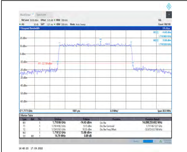
1-N66--15-15-L-7-CP-16QAM-Outer_Full-79@0-Ant 1-14.098-14.790≤15-PASS
