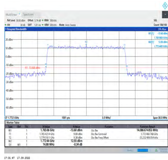
1-N66--15-15-H-8-CP-64QAM-Outer_Full-79@0-Ant 1-14.087-14.880≤15-PASS
