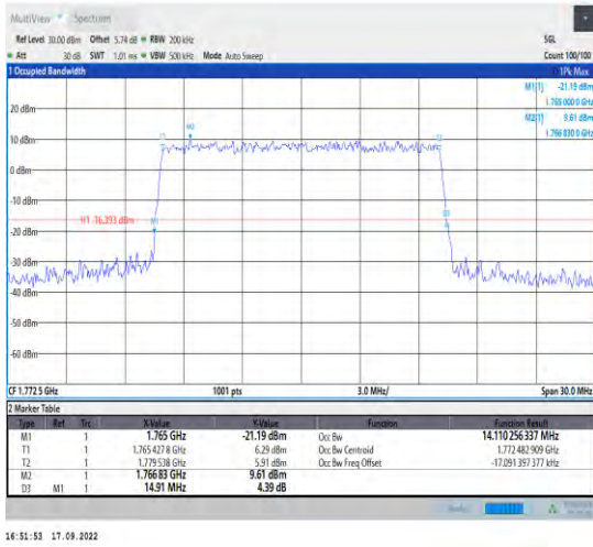
1-N66--15-15-H-9-CP-256QAM-Outer_Full-79@0-An t1-14.11-14.910-≤15-PASS
