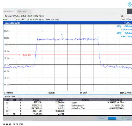
1-N66--15-15-M-9-CP-256QAM-Outer_Full-79@0-A nt1-14.119-14.940≤15-PASS
