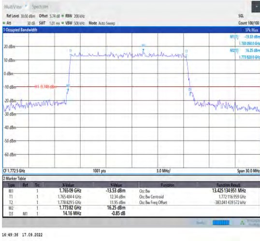
1-N66--15-15-H-1-DFT-QPSK-Outer_Full-75@0-Ant t1-13.425-14.160≤15-PASS
