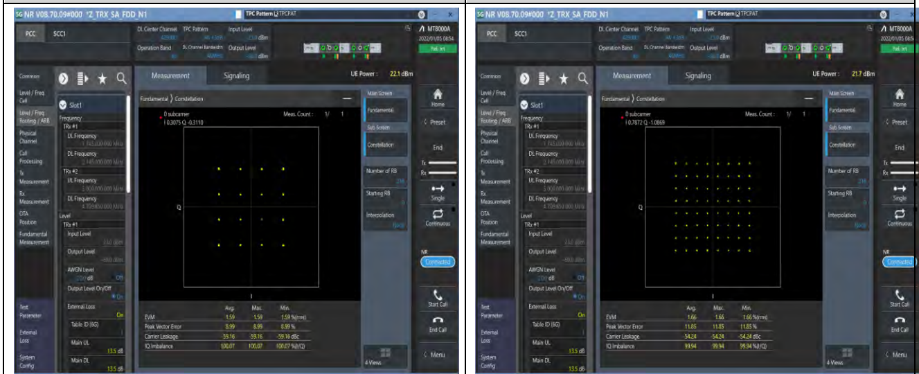
1-N66-PC3-15-40-M-3-DFT-16QAM-Outer_Full-216 @0-see graph-PASS
