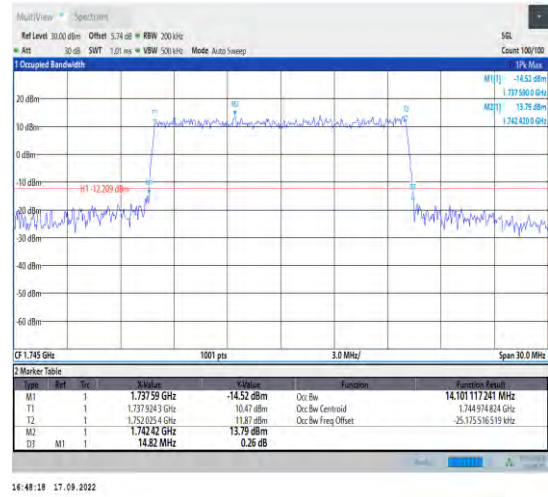
1-N66--15-15-M-7-CP-16QAM-Outer_Full-79@0-Ant 1-14.101-14.820≤15-PASS
