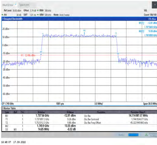
1-N66--15-15-M-6-CP-QPSK-Outer_Full-79@0-Ant1 -14.115-14.850≤15-PASS
