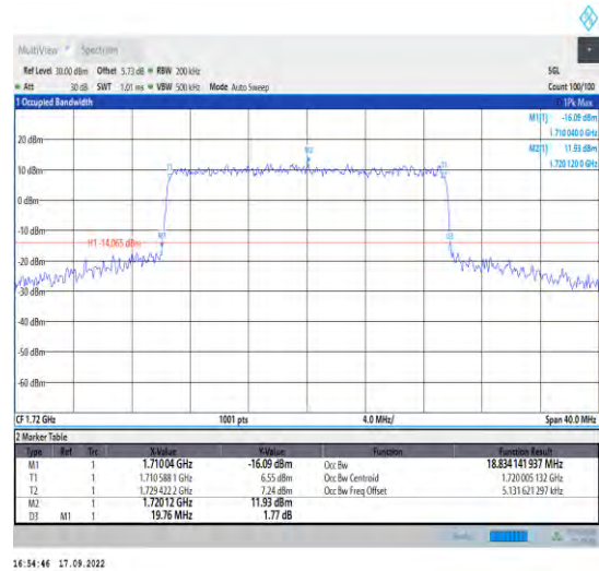
1-N66--15-20-L-7-CP-16QAM-Outer_Full-106@0-Ant1 t1-18.834-19.760-≤20-PASS
