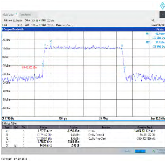
1-N66--15-15-M-8-CP-64QAM-Outer_Full-79@0-Ant 1-14.095-14.940≤15-PASS
