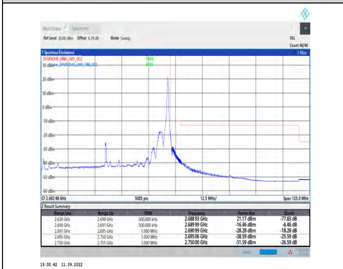
1-N41--30-60-H-5-CP-QPSK-Edge_1RB_Right-1@161-Ant1-1--PASS-see graph
