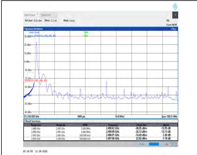
1-N41--30-100-L-1-DFT-PI2BPSK-Edge_1RB_Left-1@0-Ant1-1--PASS-see graph
