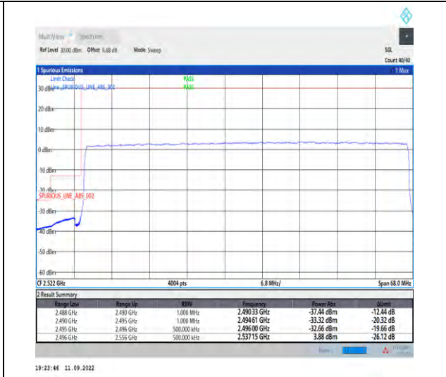
1-N41--30-60-L-3-DFT-PI2BPSK-Outer_Full-162@0-Ant1-1--PASS-see graph
