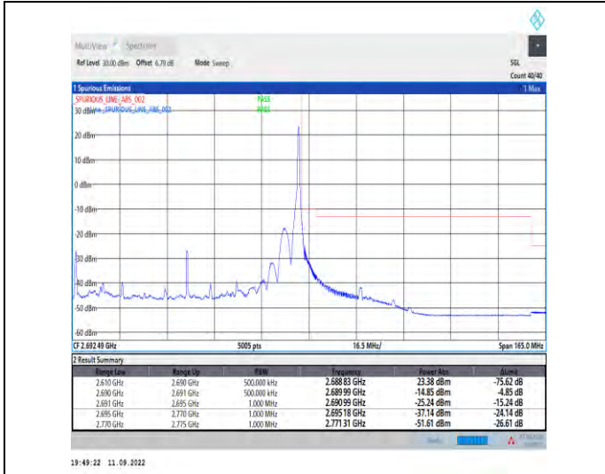
1-N41--30-80-H-2-DFT-PI2BPSK-Edge_1RB_Right-1@216-Ant1-1--PASS-see graph
