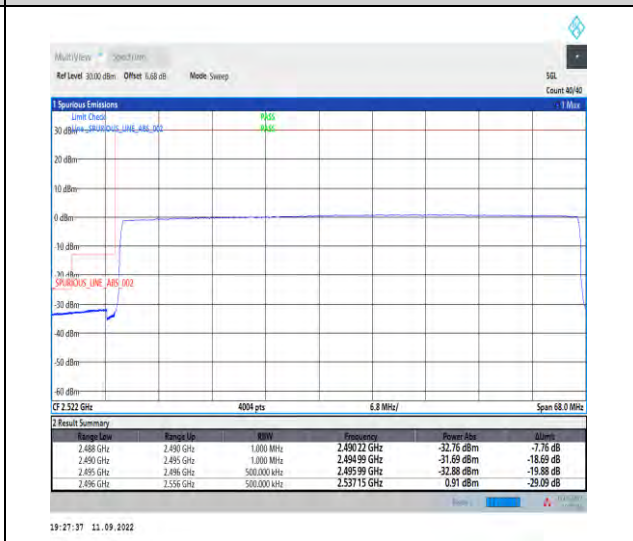
1-N41--30-60-L-6-CP-QPSK-Outer_Full-162@0-Ant1-1--PASS-see graph
