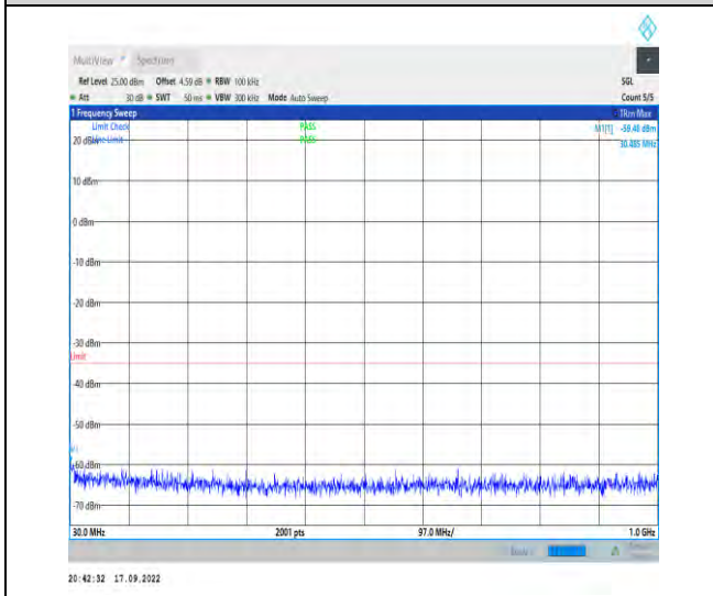
1-N41--30-100-L-1-DFT-PI2BPSK-Inner_1RB_Left-1 @1-30-1000-Ant1-30.49--59.48--35-PASS
