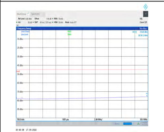
1-N41--30-100-M-1-DFT-PI2BPSK-Inner_1RB_Left-1 @ 1-0.15-30-Ant1-29.76--75.69--45-PASS
