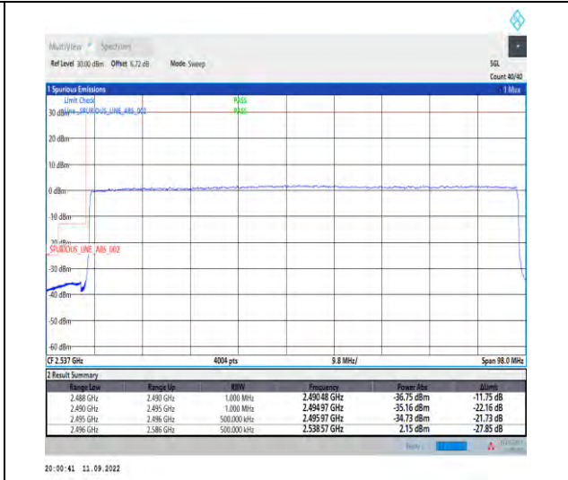
1-N41--30-90-L-3-DFT-PI2BPSK-Outer_Full-243@0-Ant1-1--PASS-see graph
