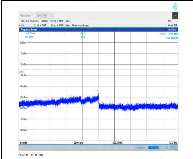
1-N41--30-100-L-1-DFT-PI2BPSK-Inner_1RB_Left-1 @ 1-3000-12000-Ant1-7484.70--47.49--25-PASS
