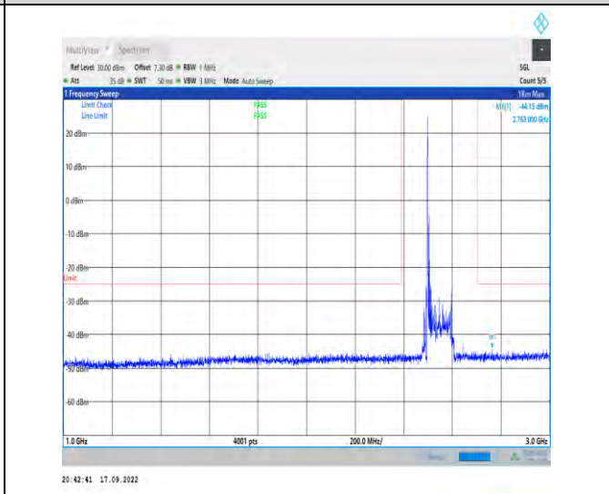
1-N41--30-100-L-1-DFT-PI2BPSK-Inner_1RB_Left-1 @1-1000-3000-Ant1-2763.00--44.15--25-PASS
