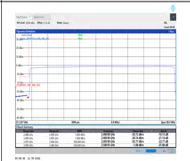
1-N41--30-90-L-6-CP-QPSK-Outer_Full-245@0-Ant1-1--PASS-see graph
