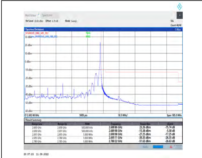
1-N41--30-90-H-2-DFT-PI2BPSK-Edge_1RB_Right-1@244-Ant1-1--PASS-see graph
