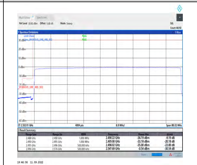
1-N41--30-80-L-6-CP-QPSK-Outer_Full-217@0-Ant1-1--PASS-see graph
