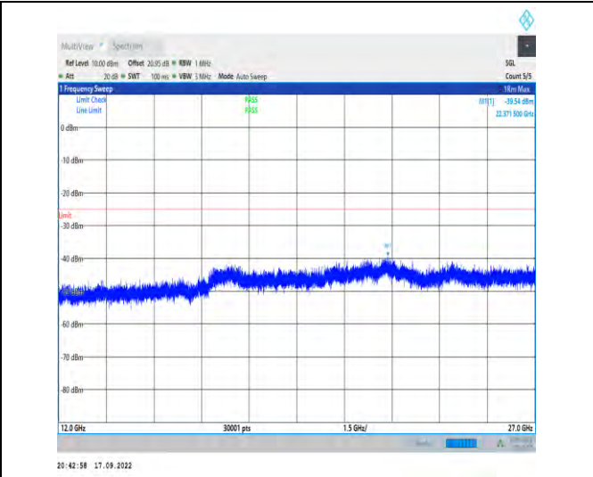
1-N41--30-100-L-1-DFT-PI2BPSK-Inner_1RB_Left-1 @ 1-12000-27000-Ant1-22371.50--39.54--25-PASS
