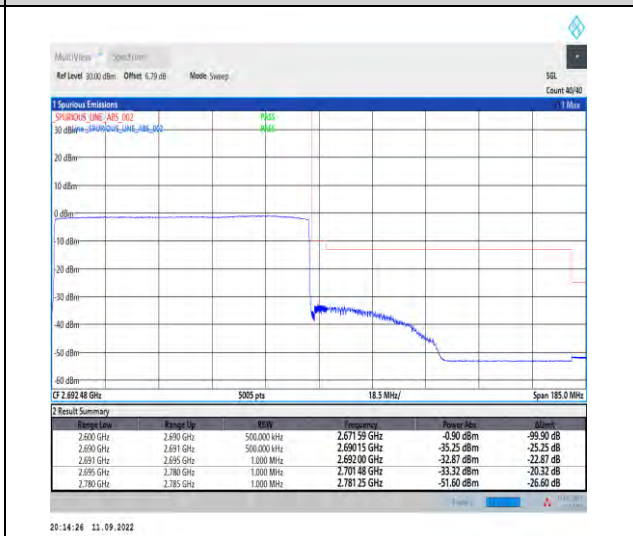
1-N41--30-90-H-6-CP-QPSK-Outer_Full-245@0-Ant1-1--PASS-see graph
