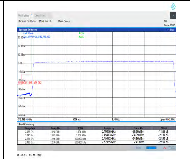
1-N41--30-80-L-3-DFT-PI2BPSK-Outer_Full-216@0-Ant1-1--PASS-see graph
