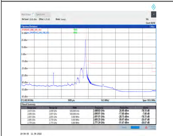
1-N41--30-80-H-5-CP-QPSK-Edge_1RB_Right-1@216-Ant1-1--PASS-see graph
