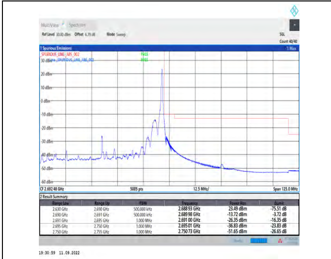
1-N41--30-60-H-2-DFT-PI2BPSK-Edge_1RB_Right-1@161-Ant1-1--PASS-see graph
