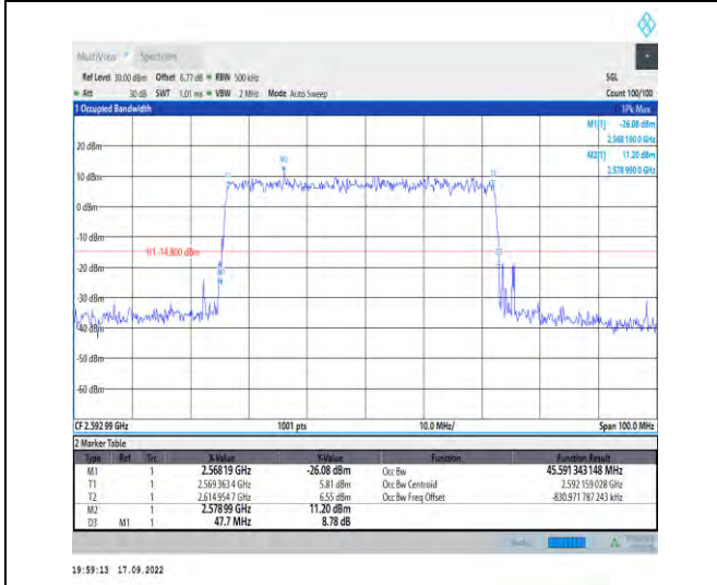
1-N41--30-50-M-5-DFT-256QAM-Outer_Full-128@0-Ant1 Ant1-45.591-47.700-≤50-PASS
