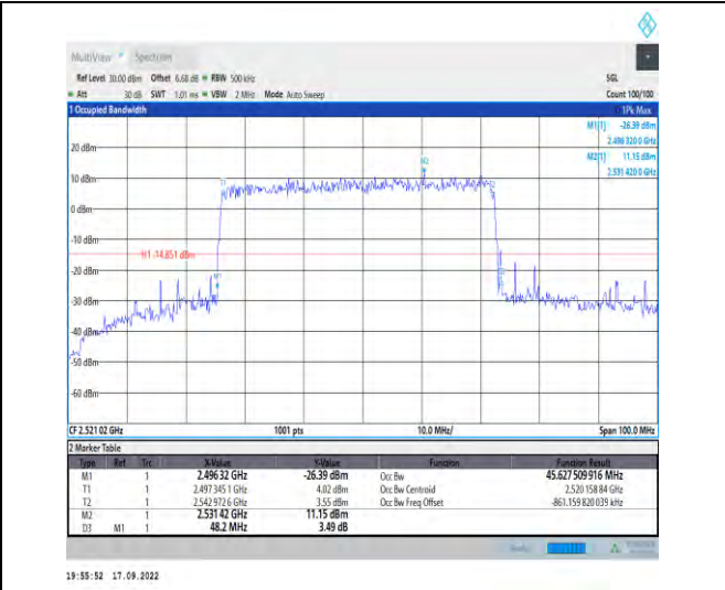
1-N41--30-50-L-5-DFT-256QAM-Outer_Full-128@0- Ant1-45.628-48.200-≤50-PASS
