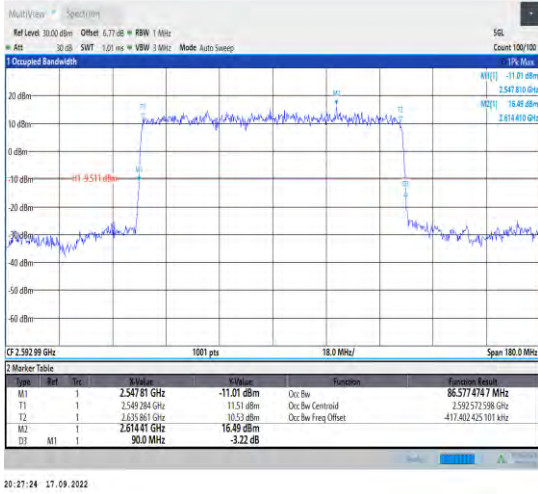
1-N41--30-90-M-2-DFT-PI2BPSK-Outer_Full-243@0-A -Ant1-86.577-90.000-≤90-PASS
