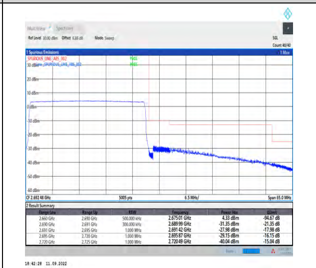
1-N41--30-30-H-6-CP-QPSK-Outer_Full-78@0-Ant1-1--PASS-see graph
