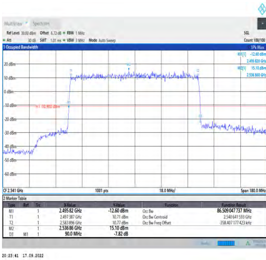
1-N41--30-90-L-1-DFT-QPSK-Outer_Full-243@0-Ant 1-86.509-90.000-≤90-PASS
