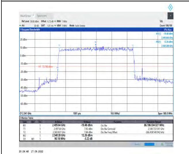
1-N41--30-90-L-5-DFT-256QAM-Outer_Full-243@0-A Ant1-86.186-90.180-≤90-PASS
