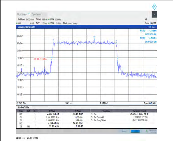
1-N41--30-40-H-4-DFT-64QAM-Outer_Full-100@0-A nt1-35.679-37.360-≤40-PASS
