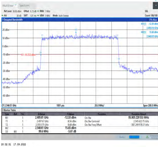
1-N41--30-100-L-2-DFT-PI2BPSK-Outer_Full-270@0-A -Ant1-95.905-99.600-≤100-PASS
