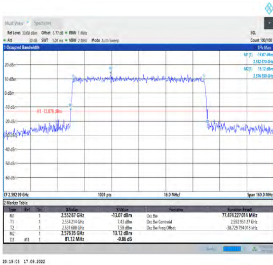
1-N41--30-80-M-7-CP-16QAM-Outer_Full-217@0-Ant 1-77.474-81.120-<80-PASS
