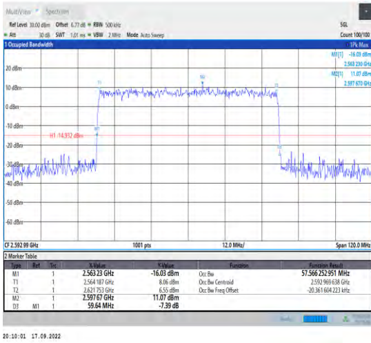
1-N41--30-60-M-8-CP-64QAM-Outer_Full-162@0-An t1-57.566-59.640-≤60-PASS
