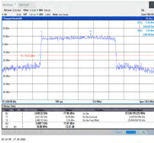
1-N41--30-60-H-7-CP-16QAM-Outer_Full-162@0-An t1-57.536-59.880-≤60-PASS
