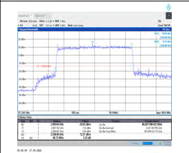
1-N41--30-90-L-6-CP-QPSK-Outer_Full-245@0-Ant1 -86.838-90.720-≤90-PASS
