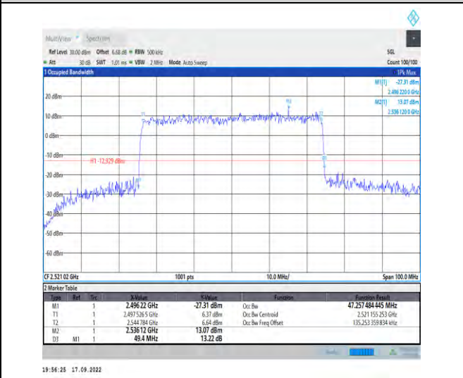
1-N41--30-50-L-7-CP-16QAM-Outer_Full-133@0-An t1-47.257-49.400-≤50-PASS
