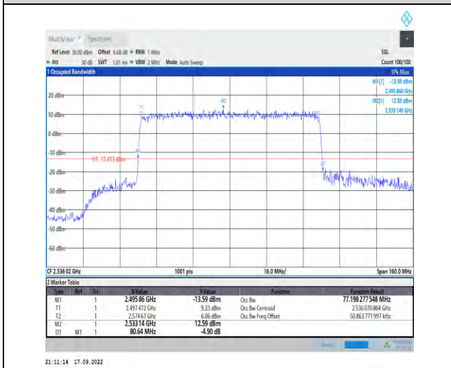
1-N41--30-80-L-8-CP-64QAM-Outer_Full-217@0-Ant1 1-77.198-80.640-≤80-PASS
