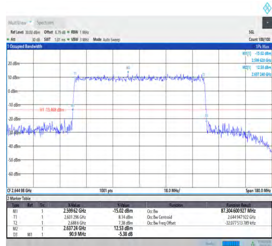
1-N41--30-90-H-6-CP-QPSK-Outer_Full-245@0-Ant 1-87.055-90.720-<90-PASS
