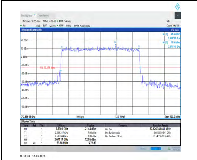
1-N41--30-60-H-3-DFT-16QAM-Outer_Full-162@0-A nt1-57.626-59.880-≤60-PASS
