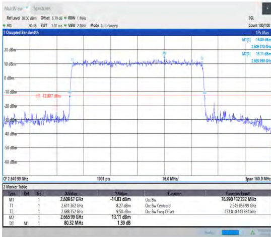
1-N41--30-80-H-4-DFT-64QAM-Outer_Full-216@0-A nt1-76.99-80.320-≤80-PASS
