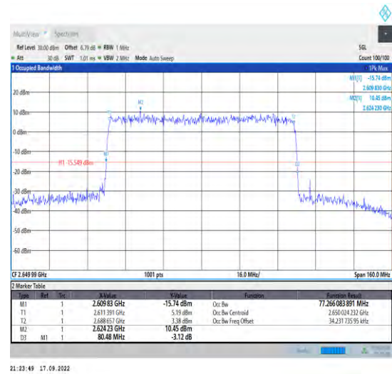
1-N41--30-80-H-9-CP-256QAM-Outer_Full-217@0-Ant nt1-77.266-80.480-≤80-PASS
