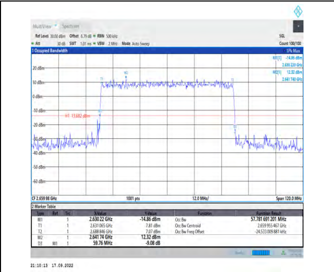
1-N41--30-60-H-4-DFT-64QAM-Outer_Full-162@0-A nt1-57.782-59.760-≤60-PASS
