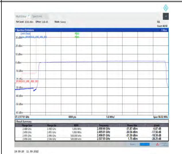
1-N41--30-50-L-6-CP-QPSK-Outer_Full-133@0-Ant1-1--PASS-see graph
