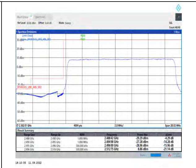
1-N41--30-20-L-3-DFT-PI2BPSK-Outer_Full-50@0 -Ant1-1--PASS-see graph
