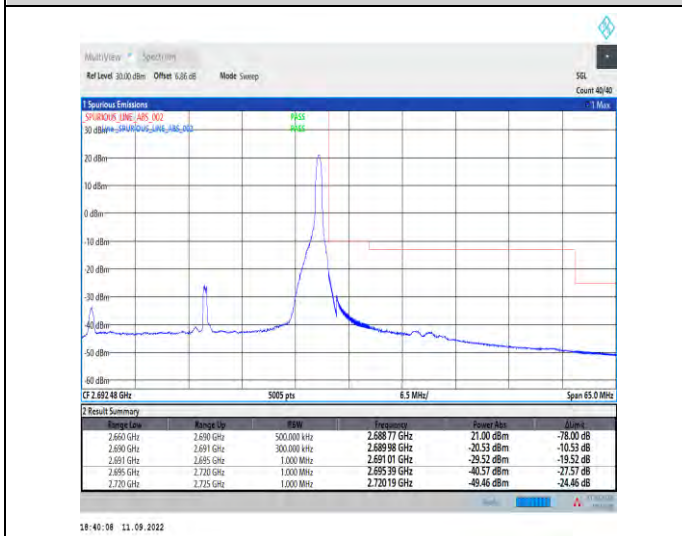
1-N41--30-30-H-5-CP-QPSK-Edge_1RB_Right-1@77-Ant1-1--PASS-see graph
