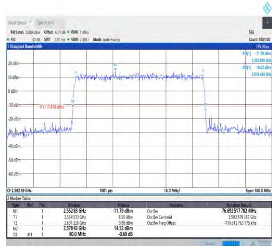
1-N41--30-80-M-2-DFT-PI2BPSK-Outer_Full-216@0-Ant1-76.971-80.480-≤80-PASS
