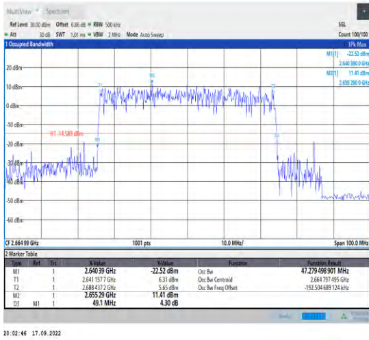
1-N41--30-50-H-6-CP-QPSK-Outer_Full-133@0-Ant t1-47.279-49.100-≤50-PASS
