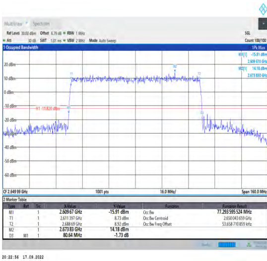
1-N41--30-80-H-8-CP-64QAM-Outer_Full-217@0-Ant t1-77.294-80.640-≤80-PASS
