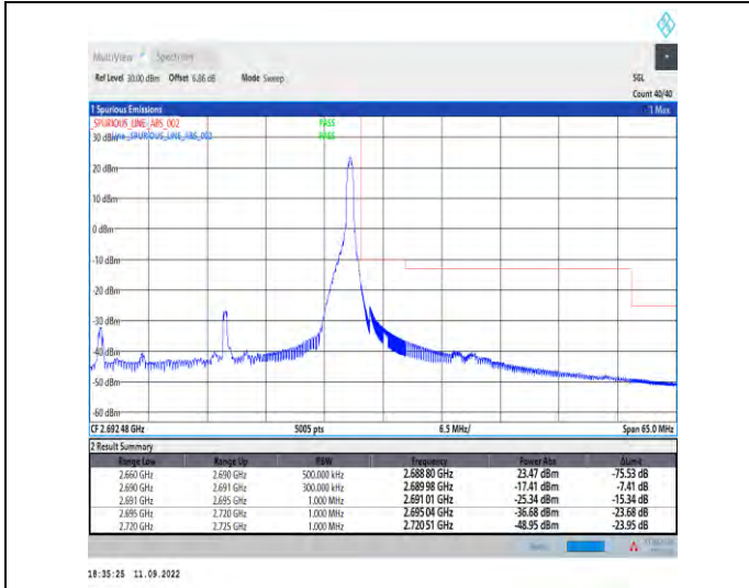
1-N41--30-30-H-2-DFT-PI2BPSK-Edge_1RB_Right-1@77-Ant1-1--PASS-see graph
