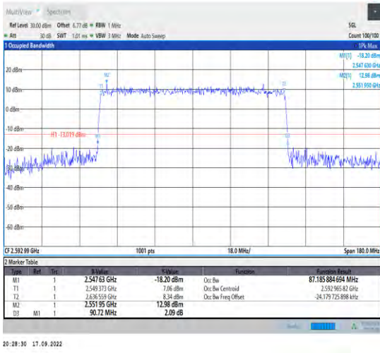
1-N41--30-90-M-6-CP-QPSK-Outer_Full-245@0-Ant 1-87.186-90.720-≤90-PASS
