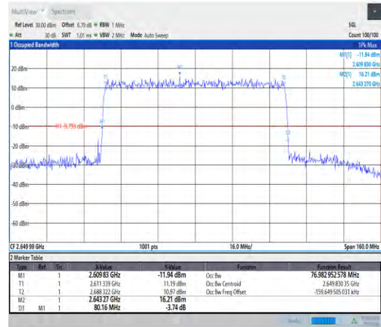
1-N41--30-80-H-1-DFT-QPSK-Outer_Full-216@0-An t1-76.983-80.160-≤80-PASS
