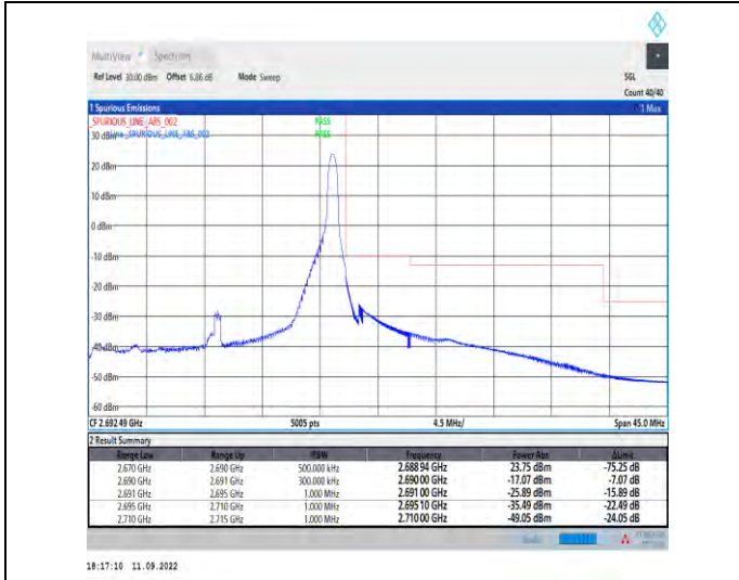
1-N41--30-20-H-2-DFT-PI2BPSK-Edge_1RB_Right-1@50-Ant1-1--PASS-see graph
