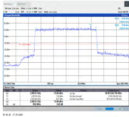
1-N41--30-100-L-1-DFT-QPSK-Outer_Full-270@0-A nt1-95.813-99.800-≤100-PASS
