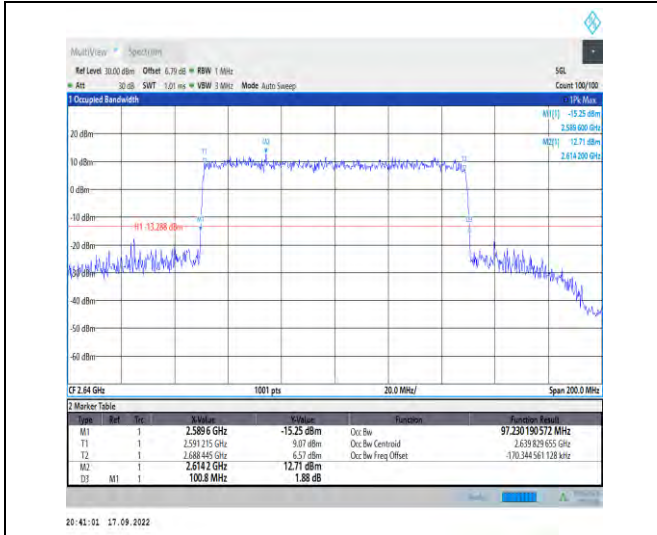
1-N41--30-100-H-6-CP-QPSK-Outer_Full-273@0-An t1-97.23-100.800-≤100-PASS
