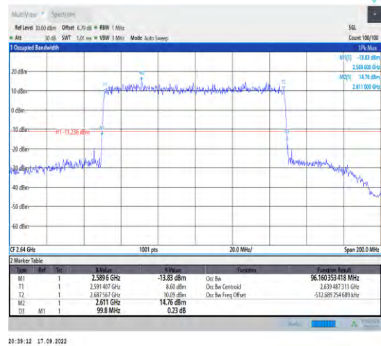
1-N41--30-100-H-1-DFT-QPSK-Outer_Full-270@0-A nt1-96.16-99.800-≤100-PASS
