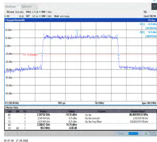
1-N41--30-90-M-1-DFT-QPSK-Outer_Full-243@0-An t1-86.47-90.000-≤90-PASS
