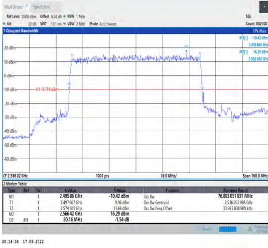
1-N41--30-80-L-2-DFT-PI2BPSK-Outer_Full-216@0-A Ant1-76.893-80.160-≤80-PASS
