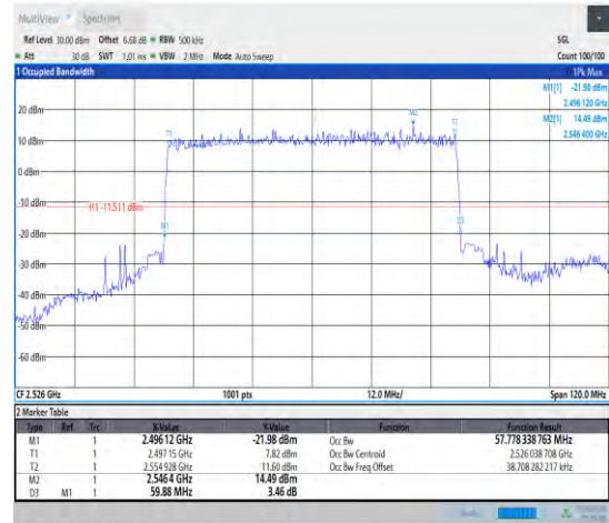
1-N41--30-60-L-2-DFT-PI2BPSK-Outer_Full-162@0-Ant 1-57.778-59.880-≤60-PASS
