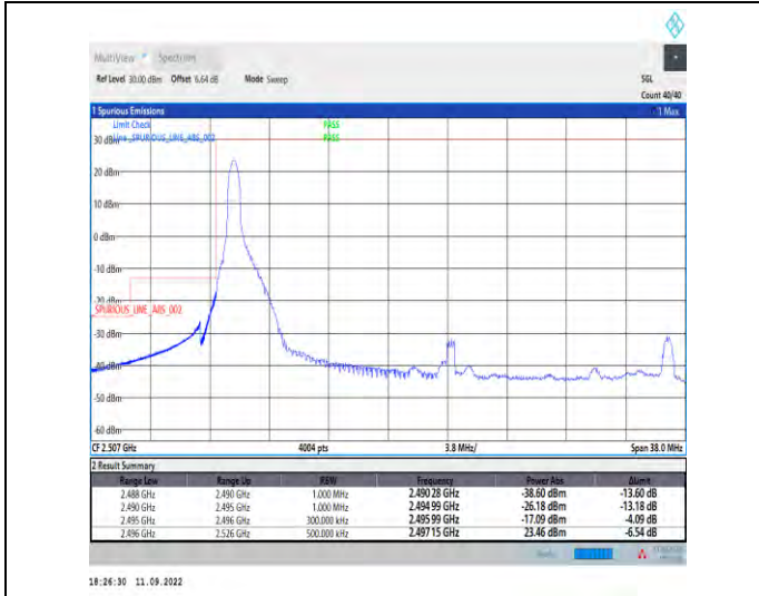
1-N41--30-30-L-1-DFT-PI2BPSK-Edge_1RB_Left-1@0 -Ant1-1--PASS-see graph
