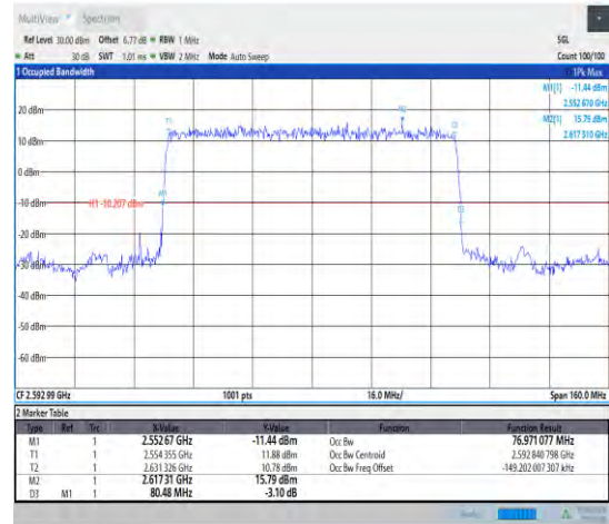
1-N41--30-80-M-2-DFT-PI2BPSK-Outer_Full-216@0-Ant1-76.971-80.480-≤80-PASS
