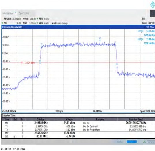
1-N41--30-80-L-4-DFT-64QAM-Outer_Full-216@0-A Ant1-76.791-80.160-≤80-PASS
