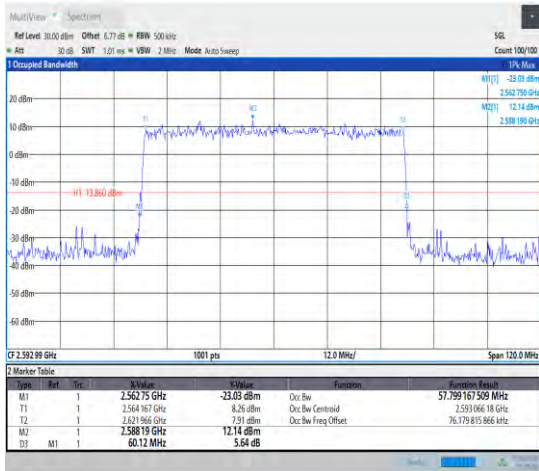
1-N41--30-60-M-4-DFT-64QAM-Outer_Full-162@0-A nt1-57.799-60.120-≤60-PASS
