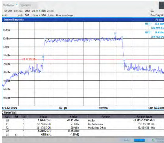
1-N41--30-50-L-8-CP-64QAM-Outer_Full-133@0-Ant 1-47.346-49.800-≤50-PASS
