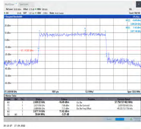
1-N41--30-60-H-8-CP-64QAM-Outer_Full-162@0-An t1-57.75-59.640-≤60-PASS
