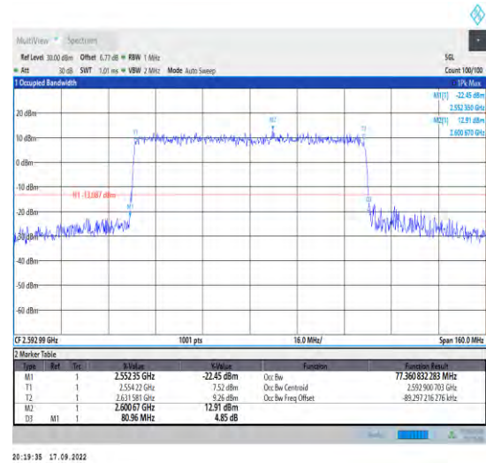
1-N41--30-80-M-8-CP-64QAM-Outer_Full-217@0-Ant 1-77.361-80.960-<80-PASS
