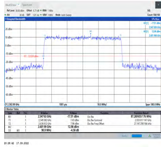
1-N41--30-90-M-7-CP-16QAM-Outer_Full-245@0-A nt1-87.27-90.900-≤90-PASS
