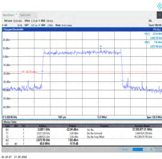
1-N41--30-60-H-9-CP-256QAM-Outer_Full-162@0-A nt1-57.596-60.000-≤60-PASS
