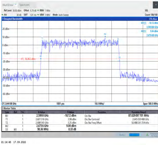
1-N41--30-90-H-9-CP-256QAM-Outer_Full-245@0-A nt1-87.029-90.360-≤90-PASS
