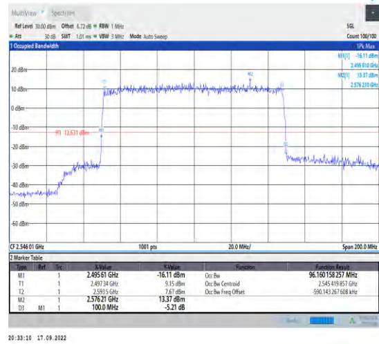
1-N41--30-100-L-3-DFT-16QAM-Outer_Full-270@0-A Ant1-96.16-100.000-≤100-PASS
