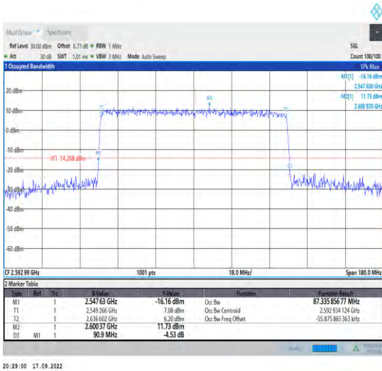
1-N41--30-90-M-8-CP-64QAM-Outer_Full-245@0-An t1-87.336-90.900-≤90-PASS
