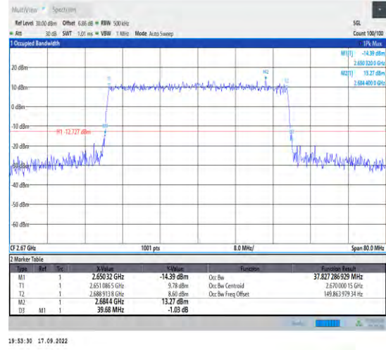
1-N41--30-40-H-6-CP-QPSK-Outer_Full-106@0-Ant 1-37.827-39.680-<40-PASS
