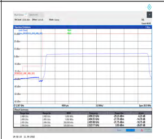
1-N41--30-30-L-6-CP-QPSK-Outer_Full-78@0-Ant 1-1--PASS-see graph
