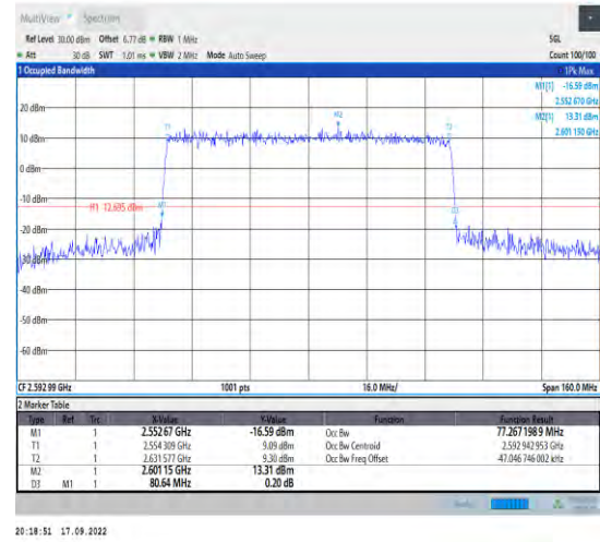
1-N41--30-80-M-6-CP-QPSK-Outer_Full-217@0-Ant 1-77.267-80.640-<80-PASS
