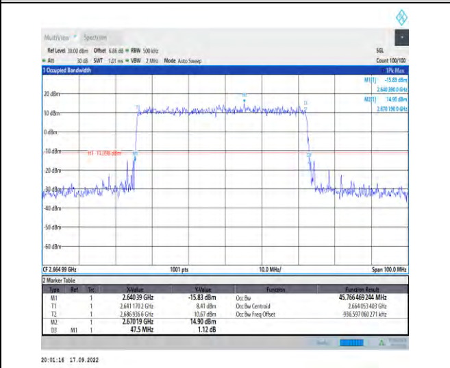
1-N41--30-50-H-1-DFT-QPSK-Outer_Full-128@0-An t1-45.766-47.500-≤50-PASS
