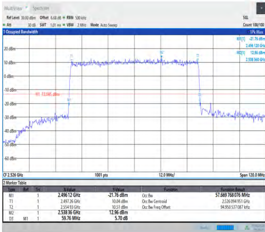
1-N41--30-60-L-1-DFT-QPSK-Outer_Full-162@0-Ant 1-57.67-59.760-≤60-PASS
