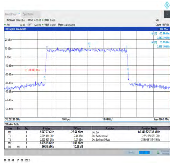
1-N41--30-90-M-5-DFT-256QAM-Outer_Full-243@0-A Ant1-86.341-90.360-≤90-PASS
