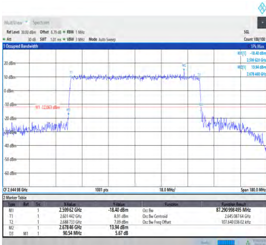
1-N41--30-90-H-5-DFT-256QAM-Outer_Full-243@0-Ant1-86.43-90.000-<90-PASS
