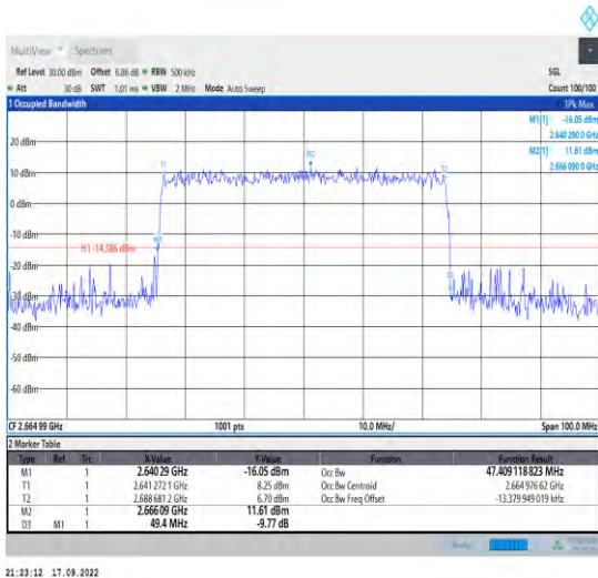
1-N41--30-50-H-8-CP-64QAM-Outer_Full-133@0-An t1-47.409-49.400-≤50-PASS
