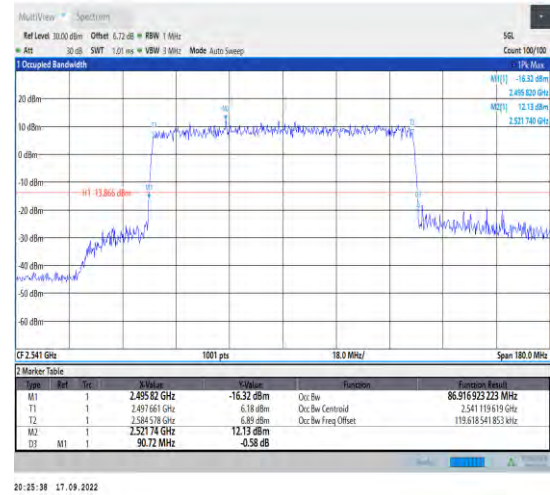
1-N41--30-90-L-8-CP-64QAM-Outer_Full-245@0-An t1-86.917-90.720-≤90-PASS
