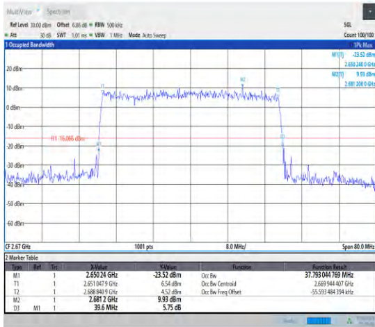
1-N41--30-40-H-9-CP-256QAM-Outer_Full-106@0-A nt1-37.793-39.600-≤40-PASS
