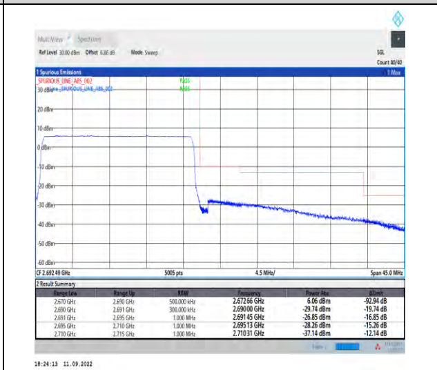
1-N41--30-20-H-6-CP-QPSK-Outer_Full-51@0-Ant1-1--PASS-see graph
