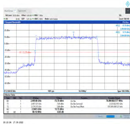
1-N41--30-80-L-5-DFT-256QAM-Outer_Full-216@0-A Ant1-76.985-80.160-≤80-PASS
