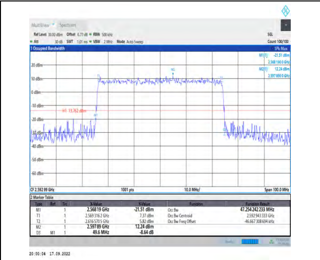
1-N41--30-50-M-8-CP-64QAM-Outer_Full-133@0-A nt1-47.254-49.600-≤50-PASS
