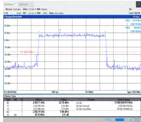
1-N41--30-60-M-5-DFT-256QAM-Outer_Full-162@0-A Ant1-57.89-59.760-≤60-PASS
