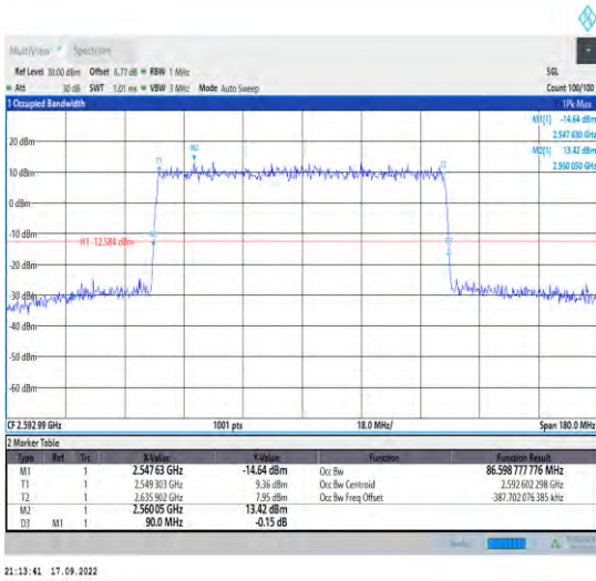
1-N41--30-90-M-4-DFT-64QAM-Outer_Full-243@0-A nt1-86.599-90.000-≤90-PASS
