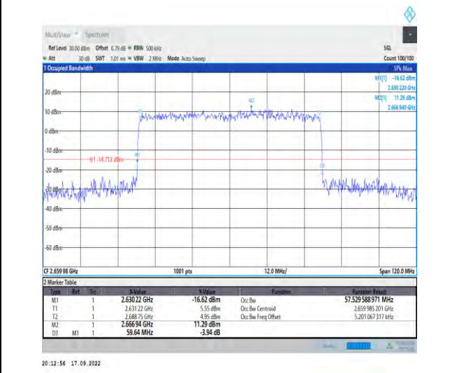
1-N41--30-60-H-6-CP-QPSK-Outer_Full-162@0-Ant 1-57.53-59.640-≤60-PASS
