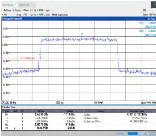
1-N41--30-80-M-9-CP-256QAM-Outer_Full-217@0-A nt1-77.462-80.480-≤80-PASS
