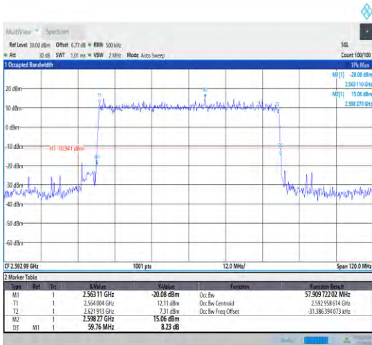
1-N41--30-60-L-9-CP-256QAM-Outer_Full-162@0-A nt1-57.815-59.640-≤60-PASS
