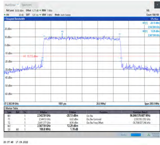
1-N41--30-100-M-8-CP-64QAM-Outer_Full-273@0-A Ant1-96.847-100.800-≤100-PASS
