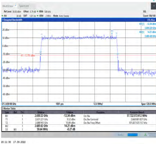
1-N41--30-60-H-1-DFT-QPSK-Outer_Full-162@0-An t1-57.722-59.640-≤60-PASS
