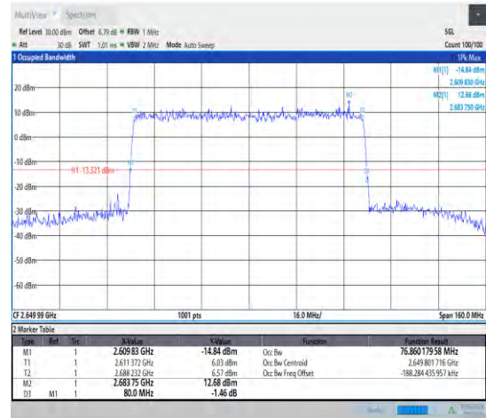
1-N41--30-80-H-5-DFT-256QAM-Outer_Full-216@0-Ant1-76.86-80.000-≤80-PASS
