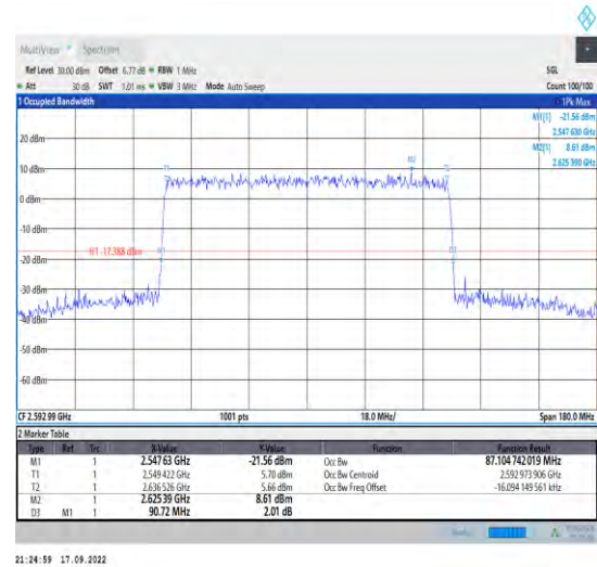
1-N41--30-90-M-9-CP-256QAM-Outer_Full-245@0-Ant Ant1-87.105-90.720-≤90-PASS
