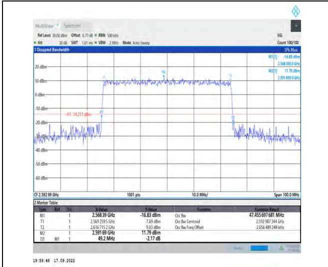
1-N41--30-50-M-7-CP-16QAM-Outer_Full-133@0-An t1-47.456-49.200-≤50-PASS
