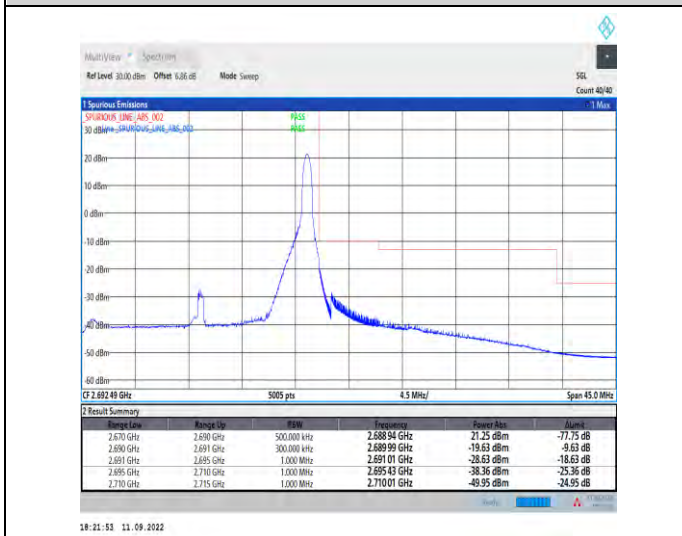
1-N41--30-20-H-5-CP-QPSK-Edge_1RB_Right-1@50-Ant1-1--PASS-see graph
