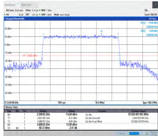
1-N41--30-90-H-6-CP-QPSK-Outer_Full-245@0-Ant 1-87.055-90.720-<90-PASS
