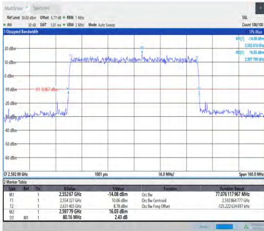
1-N41--30-80-M-1-DFT-QPSK-Outer_Full-216@0-An t1-77.076-80.160-≤80-PASS
