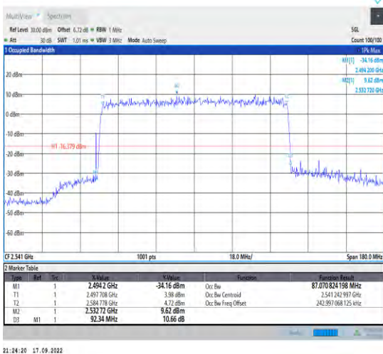
1-N41--30-90-L-9-CP-256QAM-Outer_Full-245@0-A nt1-87.071-92.340-≤90-PASS
