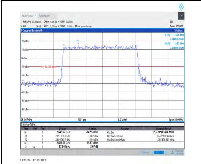
1-N41--30-40-H-1-DFT-QPSK-Outer_Full-100@0-An t1-35.729-37.840-≤40-PASS
