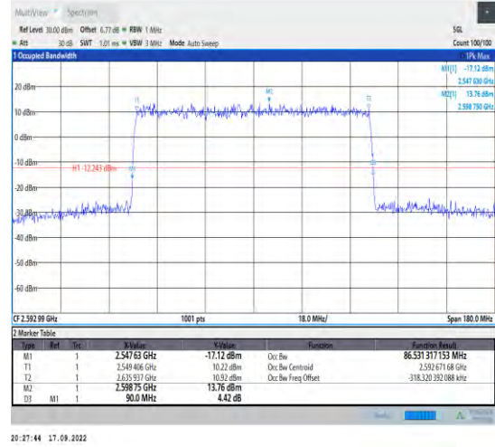
1-N41--30-90-M-3-DFT-16QAM-Outer_Full-243@0-A nt1-86.531-90.000-≤90-PASS
