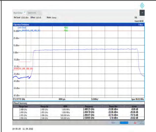
1-N41--30-50-L-3-DFT-PI2BPSK-Outer_Full-128@0-Ant1-1--PASS-see graph
