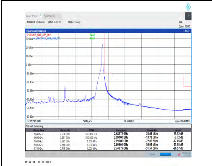
1-N41--30-50-H-2-DFT-PI2BPSK-Edge_1RB_Right-1@132-Ant1-1--PASS-see graph
