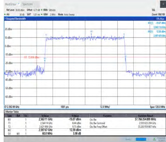
1-N41--30-60-M-1-DFT-QPSK-Outer_Full-162@0-An t1-57.766-60.000-≤60-PASS
