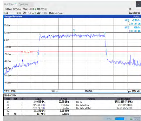
1-N41--30-50-L-9-CP-256QAM-Outer_Full-133@0-Ant nt1-47.352-49.700-≤50-PASS
