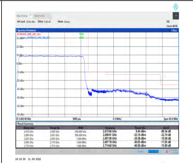
1-N41--30-20-H-3-DFT-PI2BPSK-Outer_Full-50@0-Ant1-1--PASS-see graph
