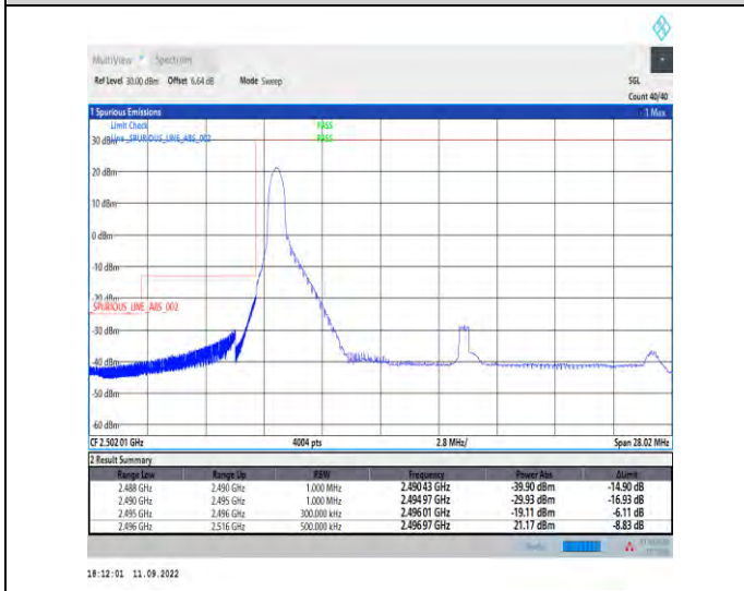
1-N41--30-20-L-4-CP-QPSK-Edge_1RB_Left-1@0-Ant 1-1--PASS-see graph
