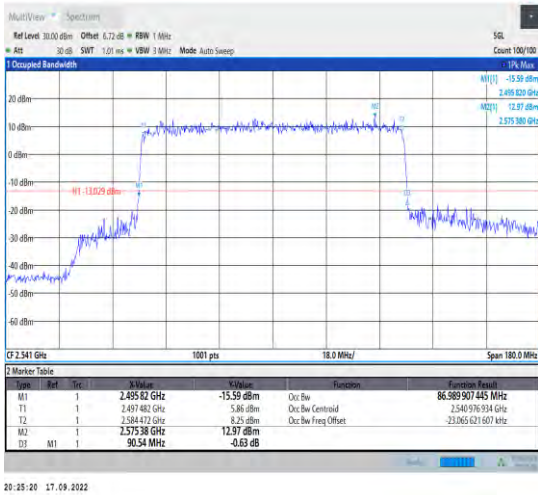
1-N41--30-90-L-7-CP-16QAM-Outer_Full-245@0-Ant 1-86.99-90.540-≤90-PASS
