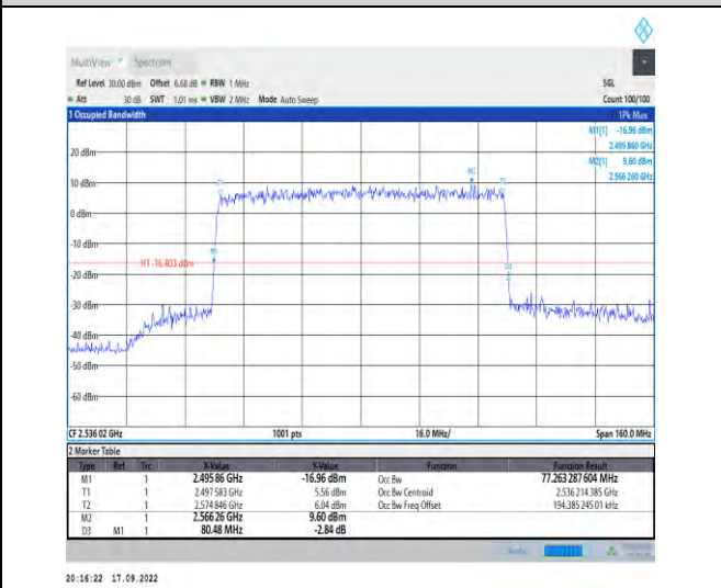
1-N41--30-80-L-9-CP-256QAM-Outer_Full-217@0-Ant1 -77.263-80.480-≤80-PASS
