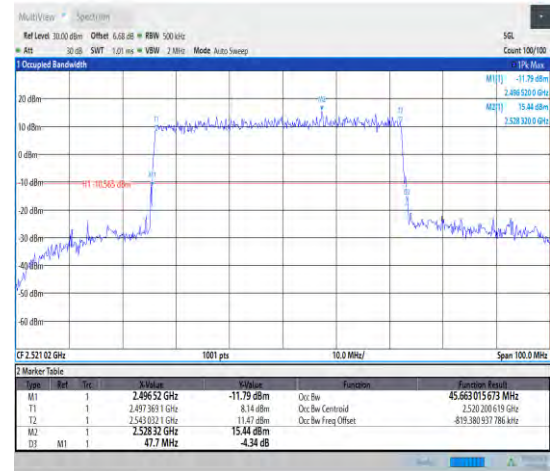
1-N41--30-50-L-1-DFT-QPSK-Outer_Full-128@0-Ant 1-45.663-47.700-≤50-PASS
