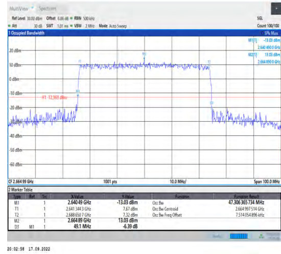
1-N41--30-50-H-7-CP-16QAM-Outer_Full-133@0-An t1-47.306-49.100-≤50-PASS
