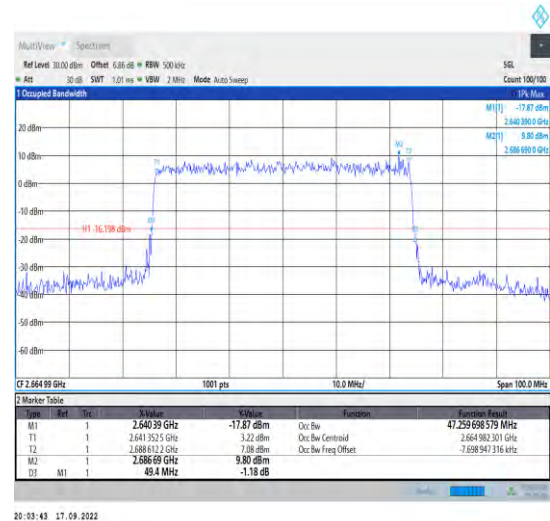
1-N41--30-50-H-9-CP-256QAM-Outer_Full-133@0-A nt1-47.26-49.400-≤50-PASS
