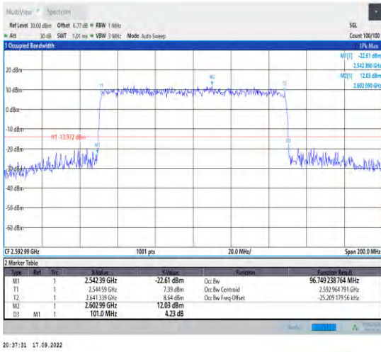
1-N41--30-100-M-7-CP-16QAM-Outer_Full-273@0-A nt1-96.749-101.000-≤100-PASS
