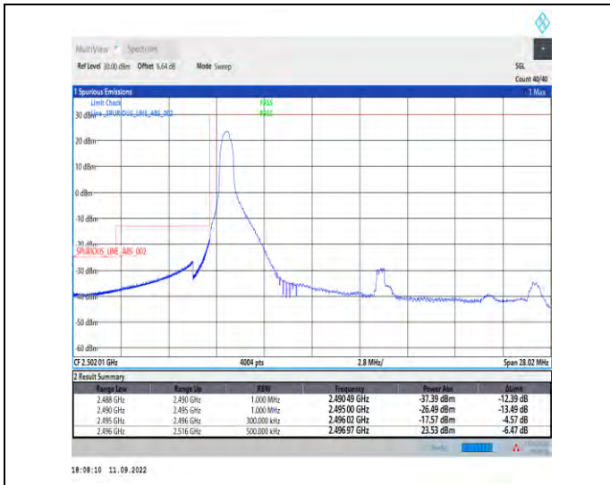
1-N41--30-20-L-1-DFT-PI2BPSK-Edge_1RB_Left-1@0 -Ant1-1--PASS-see graph
