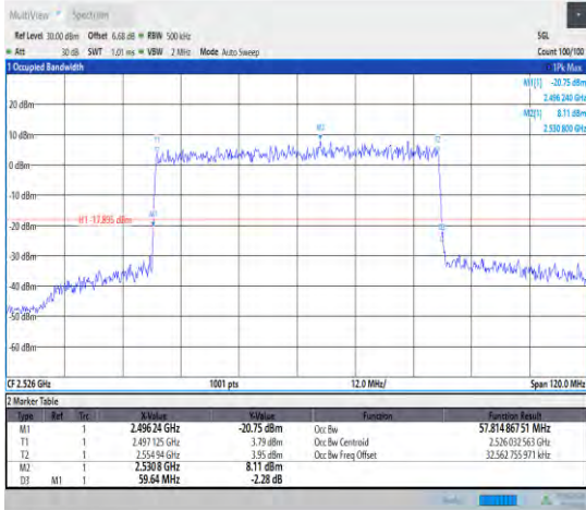
1-N41--30-60-L-9-CP-256QAM-Outer_Full-162@0-A nt1-57.815-59.640-≤60-PASS
