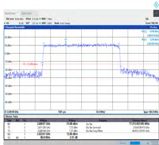
1-N41--30-80-H-5-DFT-256QAM-Outer_Full-216@0-Ant1-76.86-80.000-≤80-PASS
