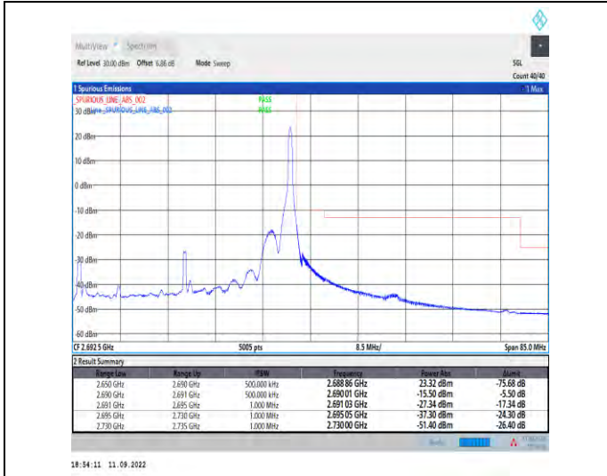
1-N41--30-40-H-2-DFT-PI2BPSK-Edge_1RB_Right-1@105-Ant1-1--PASS-see graph
