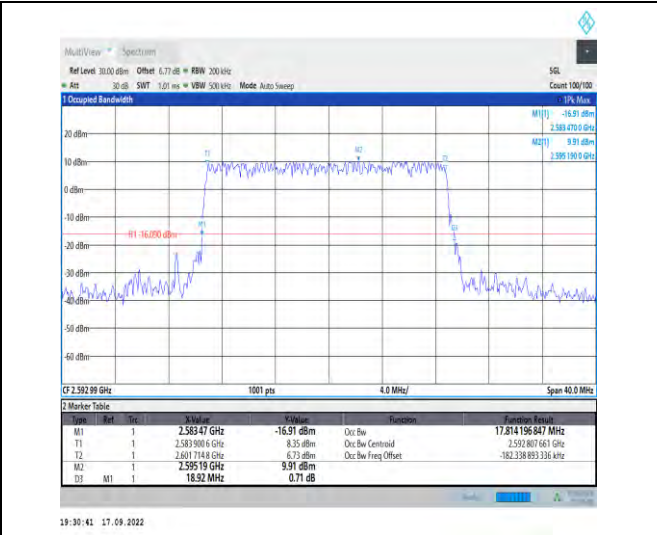
1-N41--30-20-M-5-DFT-256QAM-Outer_Full-50@0-Ant nt1-17.814-18.920-≤20-PASS
