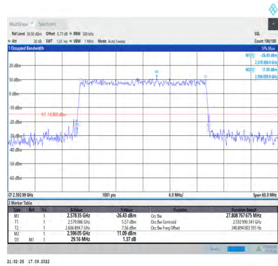
1-N41--30-30-M-8-CP-64QAM-Outer_Full-78@0-Ant 1-27.809-29.160-≤30-PASS
