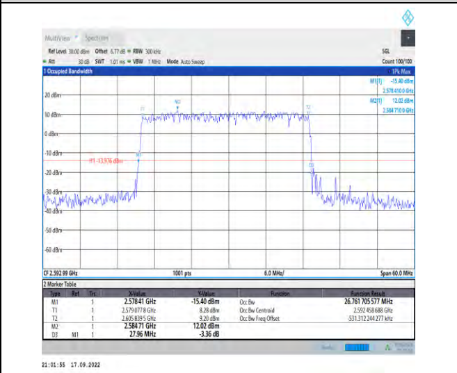
1-N41--30-30-M-4-DFT-64QAM-Outer_Full-75@0-Ant 1-26.762-27.960-≤30-PASS
