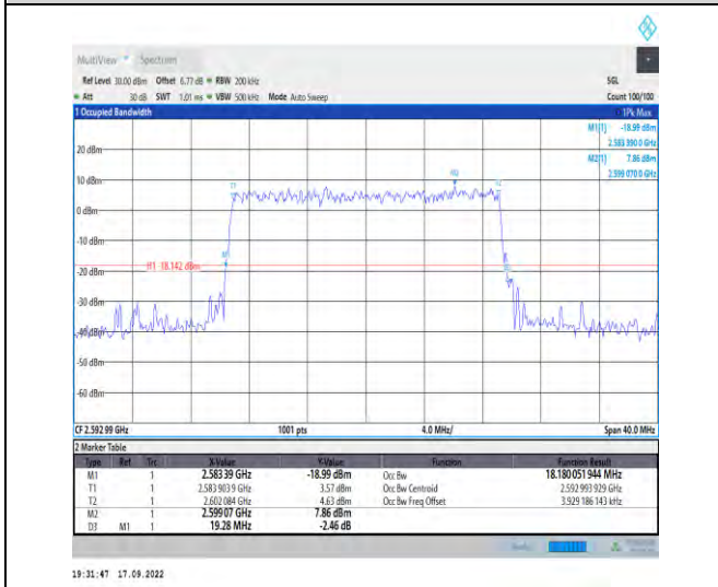
1-N41--30-20-M-6-CP-QPSK-Outer_Full-51@0-Ant1 15.925-16.440-≤20-PASS
