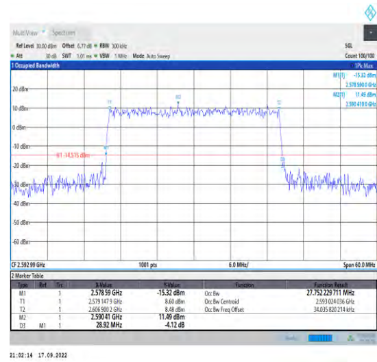
1-N41--30-30-M-6-CP-QPSK-Outer_Full-78@0-Ant1 -27.752-28.920-≤30-PASS
