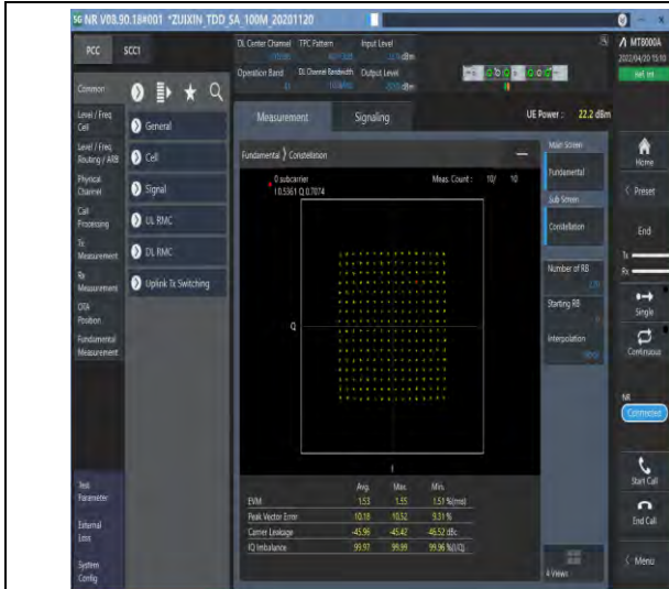
1-N41--30-100-M-5-DFT-256QAM-Outer_Full-270@0-Ant1-see graph-PASS
