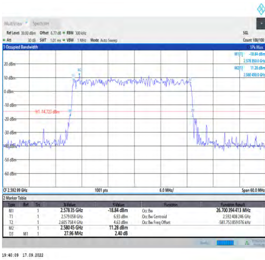
1-N41--30-30-M-5-DFT-256QAM-Outer_Full-75@0-A nt1-26.7-27.960-≤30-PASS
