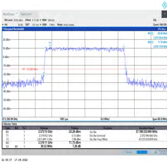
1-N41--30-40-M-8-CP-64QAM-Outer_Full-106@0-An t1-37.789-39.520-<40-PASS
