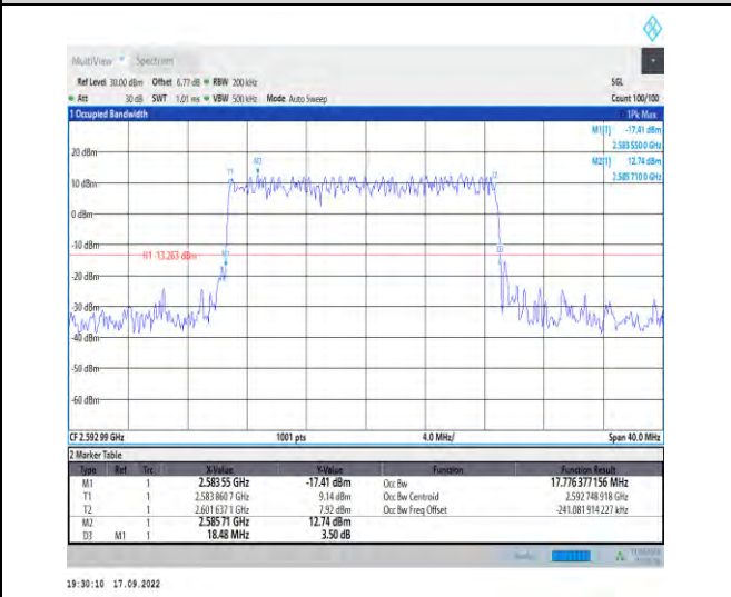
1-N41--30-20-M-3-DFT-16QAM-Outer_Full-50@0-Ant t1-17.776-18.480-≤20-PASS
