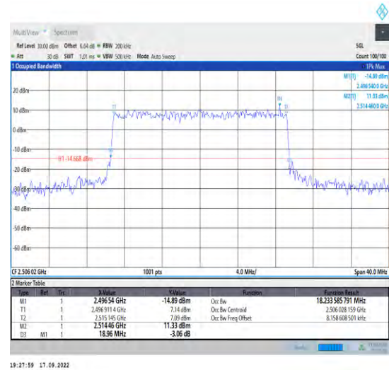
1-N41--30-20-L-8-CP-64QAM-Outer_Full-51@0-Ant1 1-18.234-18.960-≤20-PASS
