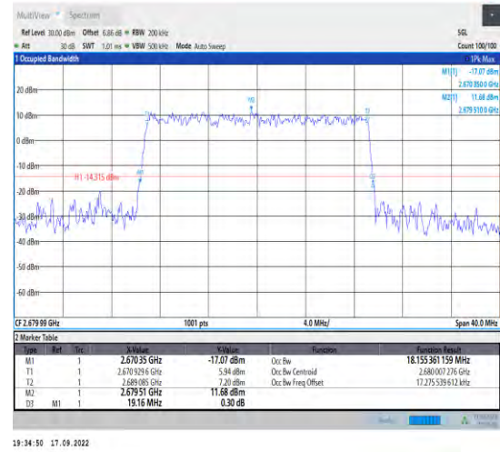
1-N41--30-20-H-8-CP-64QAM-Outer_Full-51@0-Ant 1-18.155-19.160-≤20-PASS
