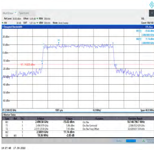
1-N41--30-20-L-7-CP-16QAM-Outer_Full-51@0-Ant1 -18.147-19.360-≤20-PASS
