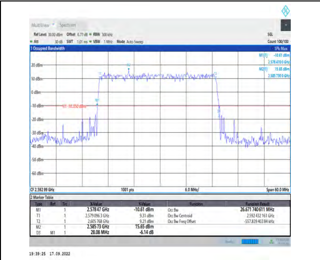
1-N41--30-30-M-2-DFT-PI2BPSK-Outer_Full-75@0-Ant 1-26.672-28.080-≤30-PASS
