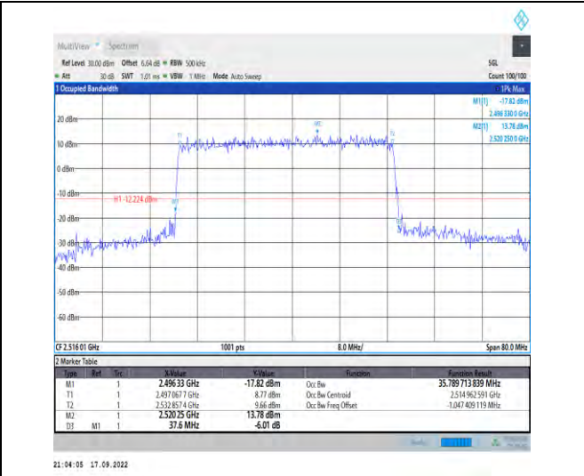
1-N41--30-40-L-4-DFT-64QAM-Outer_Full-100@0-A nt1-35.79-37.600-≤40-PASS
