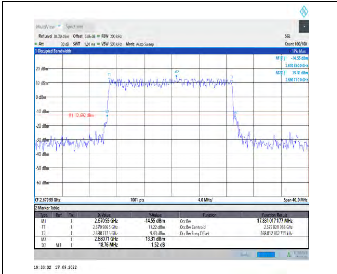
1-N41--30-20-H-3-DFT-16QAM-Outer_Full-50@0-An t1-17.831-18.760-≤20-PASS
