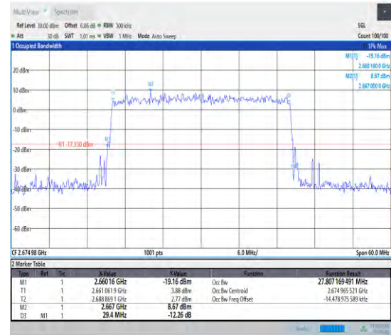
1-N41--30-30-H-9-CP-256QAM-Outer_Full-78@0-Ant t1-27.807-29.400-≤30-PASS
