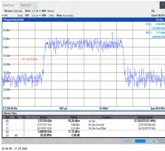
1-N41--30-40-M-6-CP-QPSK-Outer_Full-106@0-Ant 1-37.523-39.280-<40-PASS
