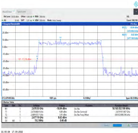
1-N41--30-20-H-9-CP-256QAM-Outer_Full-51@0-An t1-18.165-19.200-≤20-PASS
