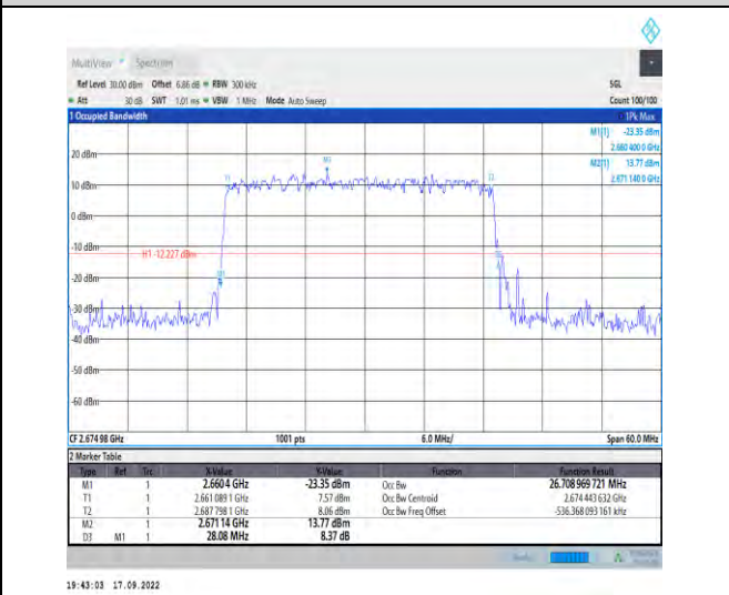
1-N41--30-30-H-3-DFT-16QAM-Outer_Full-75@0-Ant t1-26.709-28.080-≤30-PASS
