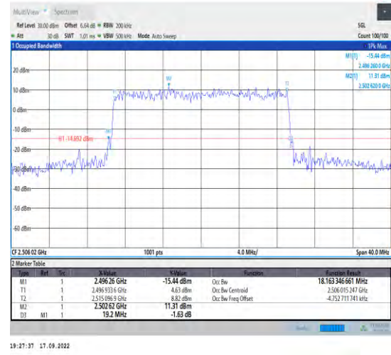
1-N41--30-20-L-6-CP-QPSK-Outer_Full-51@0-Ant1- 18.163-19.200-≤20-PASS
