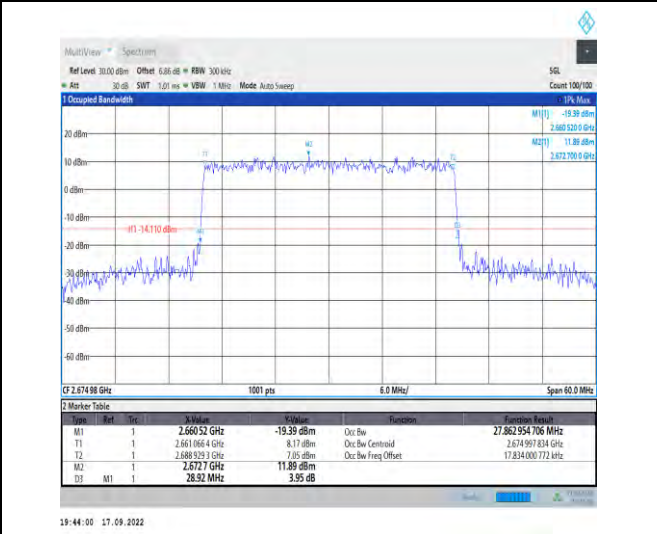
1-N41--30-30-H-7-CP-16QAM-Outer_Full-78@0-Ant 1-27.863-28.920<=30-PASS
