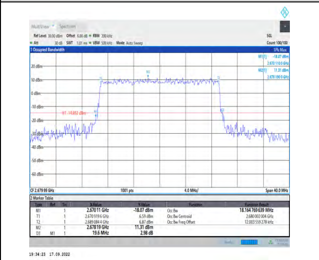
1-N41--30-20-H-6-CP-QPSK-Outer_Full-51@0-Ant1 18.165-19.600-≤20-PASS
