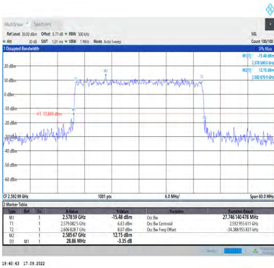
1-N41--30-30-M-7-CP-16QAM-Outer_Full-78@0-Ant 1-27.746-28.860-≤30-PASS
