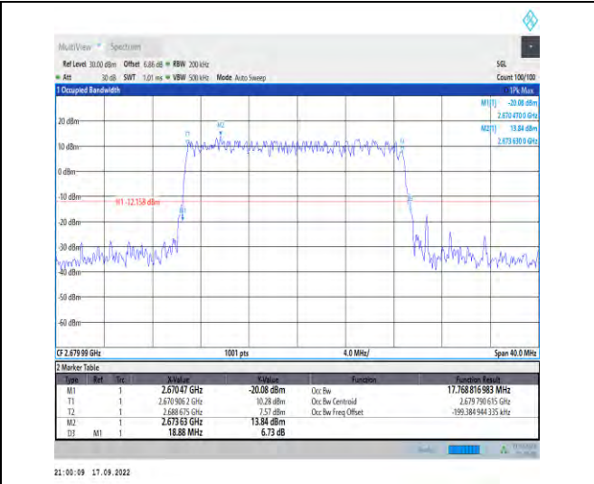
1-N41--30-20-H-4-DFT-64QAM-Outer_Full-50@0-An t1-17.769-18.880-≤20-PASS
