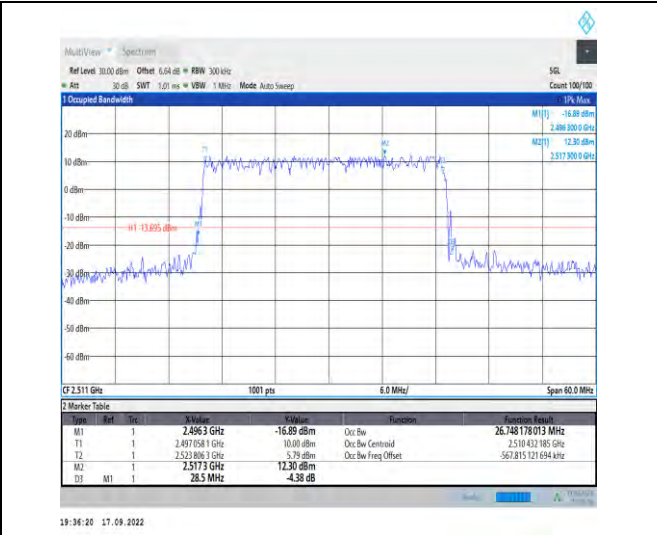
1-N41--30-30-L-3-DFT-16QAM-Outer_Full-75@0-Ant 1-26.748-28.500-≤30-PASS
