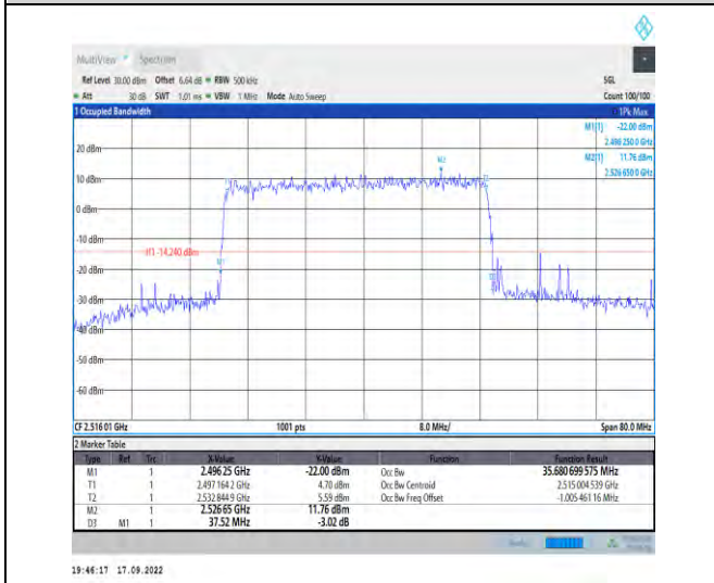
1-N41--30-40-L-5-DFT-256QAM-Outer_Full-100@0-A Ant1-35.681-37.520-≤40-PASS
