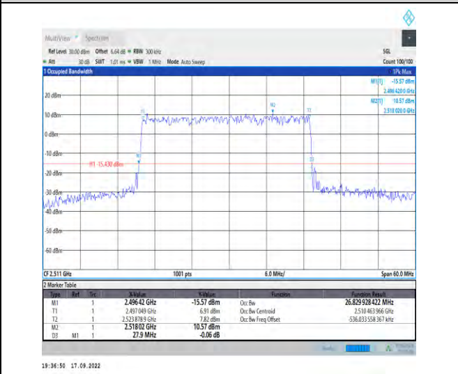
1-N41--30-30-L-5-DFT-256QAM-Outer_Full-75@0-A nt1-26.83-27.900-≤30-PASS
