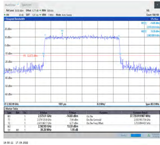
1-N41--30-40-M-7-CP-16QAM-Outer_Full-106@0-A nt1-37.736-39.280-<40-PASS
