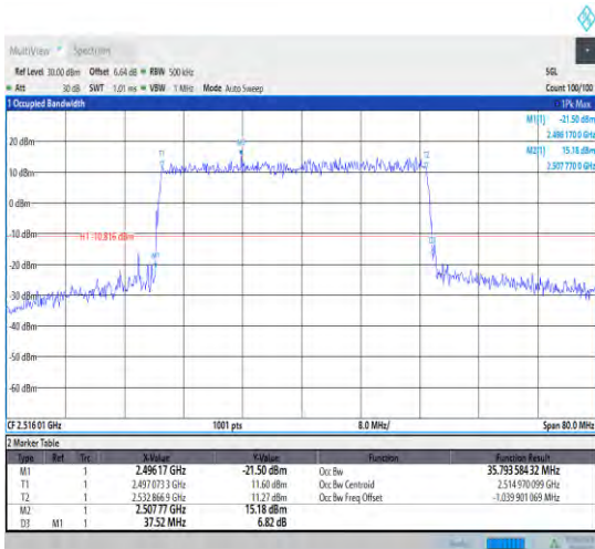
1-N41--30-30-H-8-CP-64QAM-Outer_Full-78@0-Ant 1-27.855-28.860-≤30-PASS
