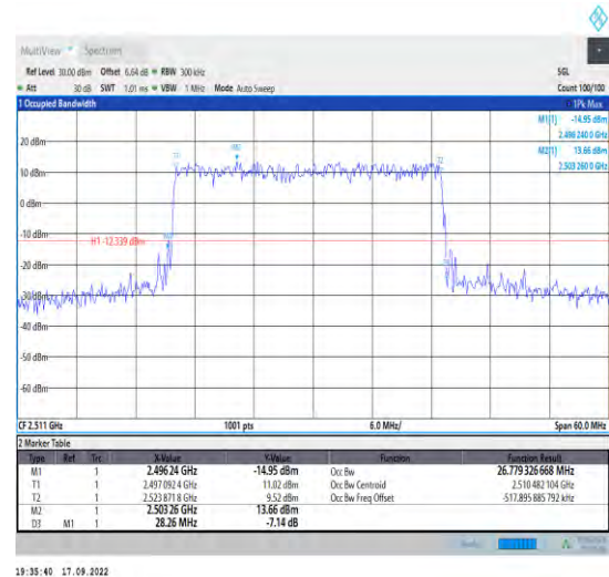
1-N41--30-30-L-1-DFT-QPSK-Outer_Full-75@0-Ant1 -26.779-28.260-≤30-PASS
