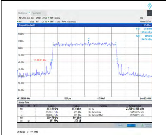
1-N41--30-30-M-9-CP-256QAM-Outer_Full-78@0-Ant t1-27.793-29.100-≤30-PASS
