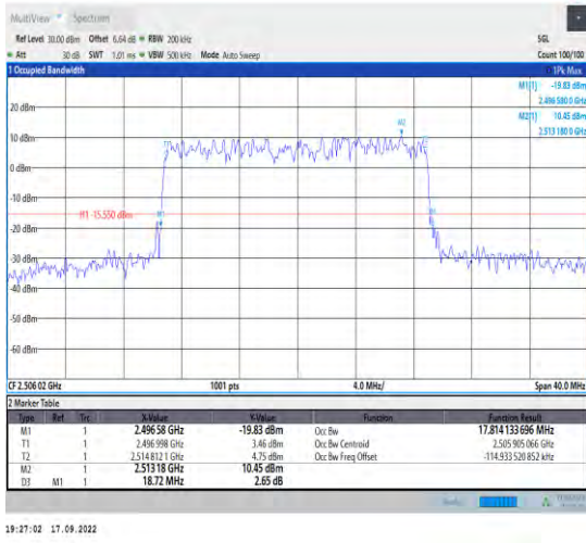
1-N41--30-20-L-5-DFT-256QAM-Outer_Full-50@0-A nt1-17.814-18.720-≤20-PASS
