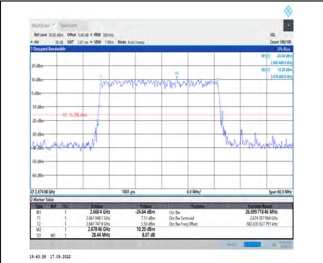
1-N41--30-30-H-5-DFT-256QAM-Outer_Full-75@0-A nt1-26.7-28.440<=30-PASS
