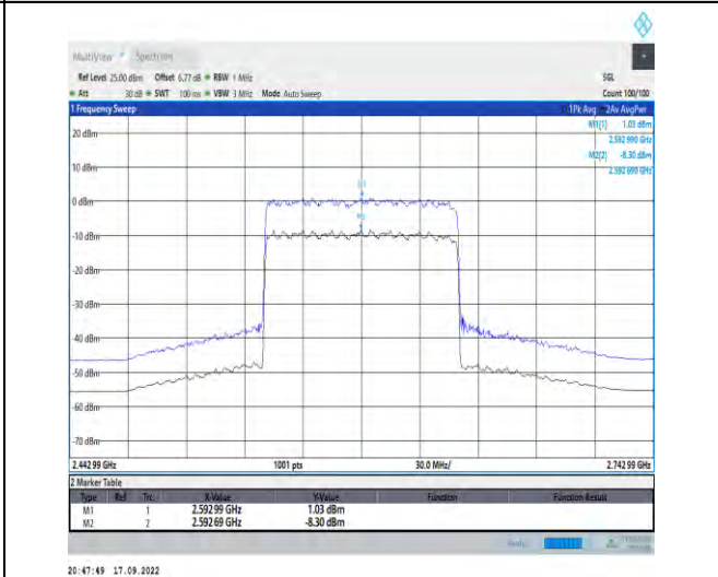
1-N41--30-100-M-2-CP-256QAM-Outer_Full-273@0-Ant1-9.33-100%-0.00-9.33-PASS- \leq 13
