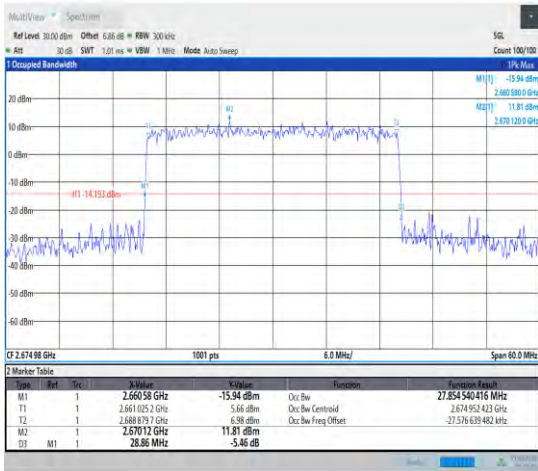
1-N41--30-30-H-8-CP-64QAM-Outer_Full-78@0-Ant 1-27.855-28.860-≤30-PASS
