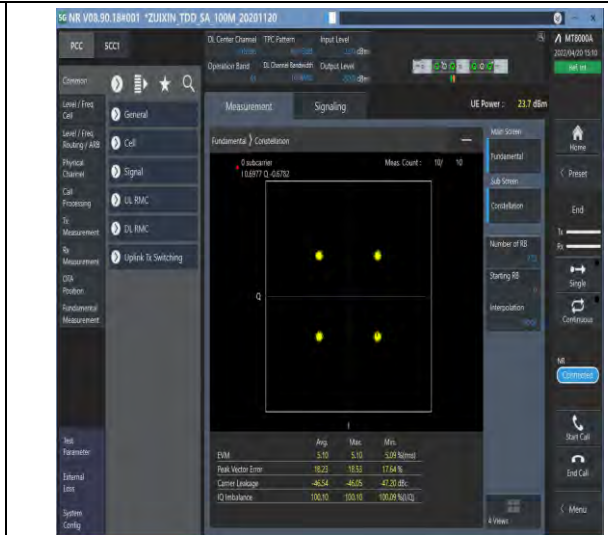
1-N41--30-100-M-6-CP-QPSK-Outer_Full-273@0-Ant1-see graph-PASS
