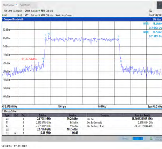
1-N41--30-20-H-7-CP-16QAM-Outer_Full-51@0-Ant 1-18.167-19.360-≤20-PASS
