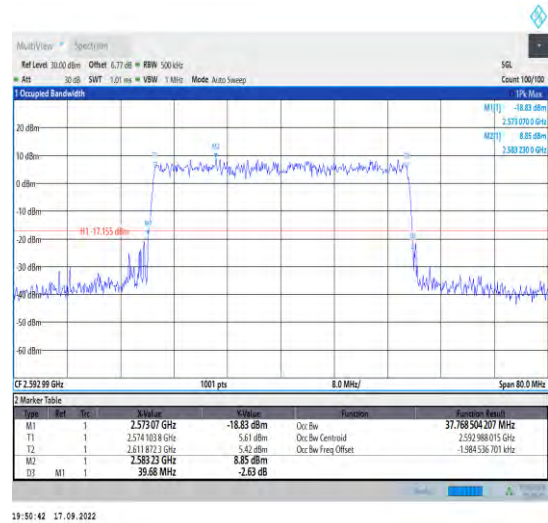
1-N41--30-40-M-9-CP-256QAM-Outer_Full-106@0-Ant 1-37.769-39.680-<40-PASS
