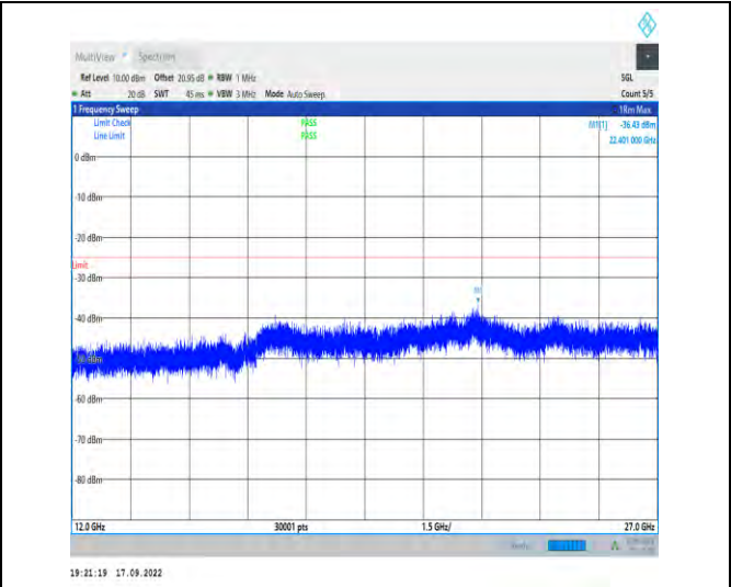
1-N38--30-40-H-1-DFT-PI2BPSK-Inner_1RB_Left-1 @ 1-12000-27000-Ant1-22401.00--36.43--25-PASS
