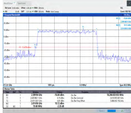
1-N38--30-20-H-8-CP-64QAM-Outer_Full-51@0-Ant 1-18.246-19.480-≤20-PASS
