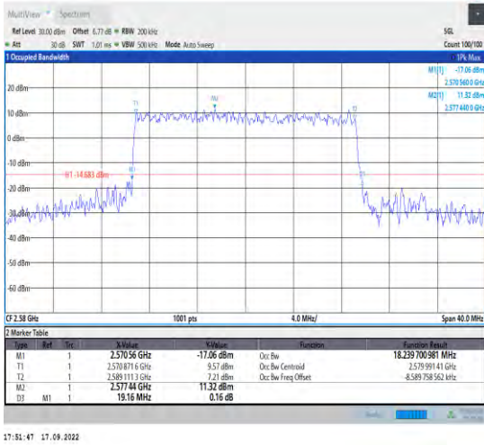
1-N38--30-20-L-7-CP-16QAM-Outer_Full-51@0-Ant1 -18.24-19.160-≤20-PASS
