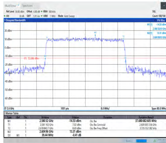
1-N38--30-40-H-8-CP-64QAM-Outer_Full-106@0-An t1-37.681-39.440-<40-PASS
