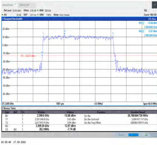
1-N38--30-30-H-4-DFT-64QAM-Outer_Full-75@0-A t1-26.769-28.200<=30-PASS
