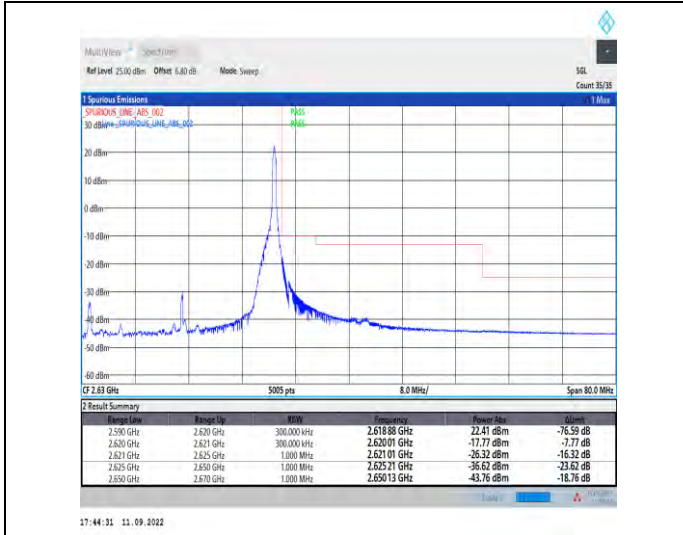
1-N38--30-30-H-2-DFT-PI2BPSK-Edge_1RB_Right-1@77-Ant1-1--PASS-see graph
