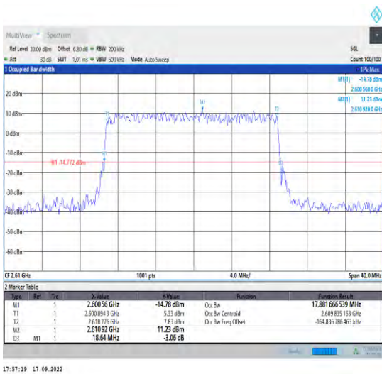
1-N38--30-20-H-5-DFT-256QAM-Outer_Full-50@0-A nt1-17.882-18.640-≤20-PASS
