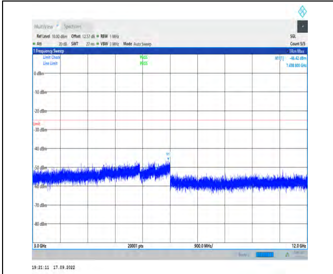
1-N38--30-40-H-1-DFT-PI2BPSK-Inner_1RB_Left-1 @ 1-3000-12000-Ant1-7438.80--46.42--25-PASS
