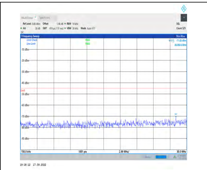
1-N38--30-40-L-1-DFT-PI2BPSK-Inner_1RB_Left-1@ 1-0.15-30-Ant1-28.06--71.63--45-PASS
