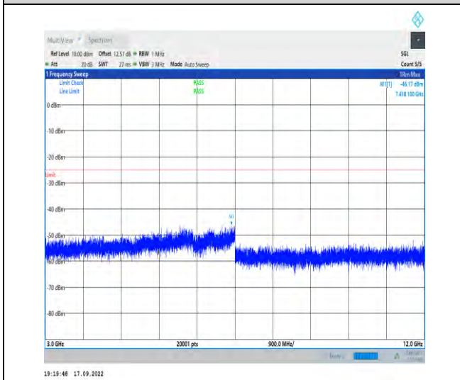
1-N38--30-40-M-1-DFT-PI2BPSK-Inner_1RB_Left-1 @1-3000-12000-Ant1-7418.10--46.17--25-PASS
