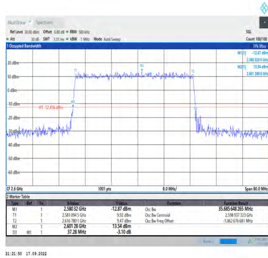
1-N38--30-40-H-4-DFT-64QAM-Outer_Full-100@0-A nt1-35.686-37.280-<40-PASS
