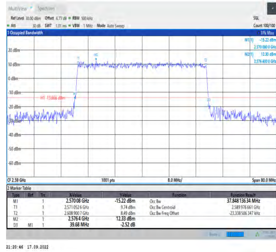
1-N38--30-40-L-8-CP-64QAM-Outer_Full-106@0-An t1-37.848-39.680-<40-PASS
