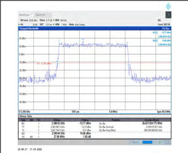
1-N38--30-30-M-2-DFT-PI2BPSK-Outer_Full-75@0-Ant1 1-26.657-27.960-<30-PASS
