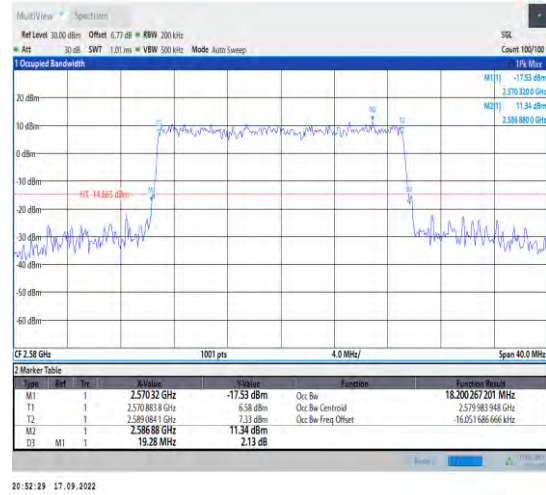
1-N38--30-20-L-8-CP-64QAM-Outer_Full-51@0-Ant 1-18.2-19.280-≤20-PASS
