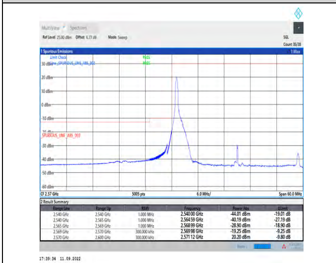
1-N38--30-30-L-4-CP-QPSK-Edge_1RB_Left-1@0-Ant1-1--PASS-see graph
