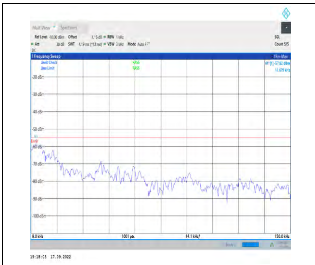
1-N38--30-40-L-1-DFT-PI2BPSK-Inner_1RB_Left-1 @1-0.009-0.15-Ant1-0.01--57.82--55-PASS
