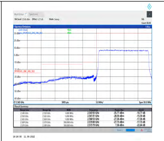
1-N38--30-20-L-3-DFT-PI2BPSK-Outer_Full-50@0-Ant1-1--PASS-see graph
