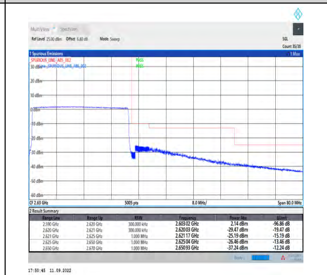
1-N38--30-30-H-6-CP-QPSK-Outer_Full-78@0-Ant1-1--PASS-see graph
