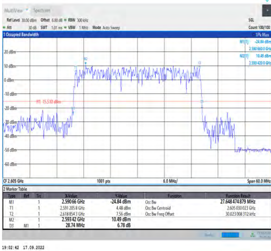
1-N38--30-30-H-6-CP-QPSK-Outer_Full-78@0-Ant1- 27.648-28.740<=30-PASS
