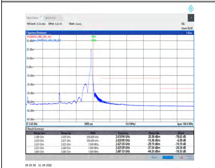
1-N38--30-40-H-5-CP-QPSK-Edge_1RB_Right-1@105-Ant1-1--PASS-see graph
