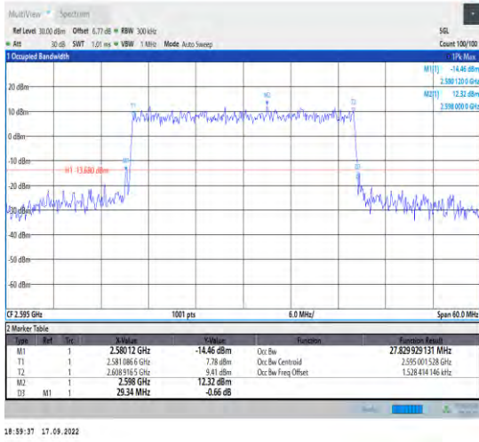
1-N38--30-30-M-7-CP-16QAM-Outer_Full-78@0-Ant 1-27.83-29.340-≤30-PASS
