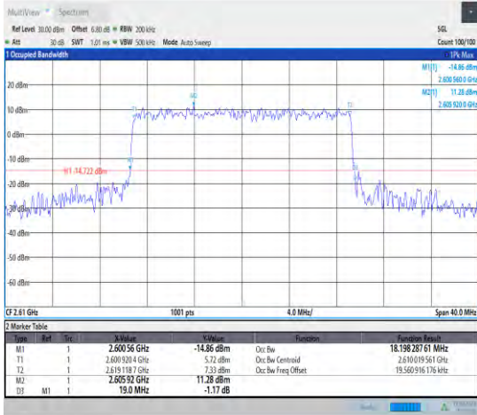
1-N38--30-20-H-7-CP-16QAM-Outer_Full-51@0-Ant 1-18.198-19.000-≤20-PASS
