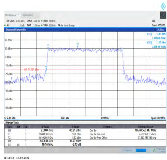
1-N38--30-20-H-6-CP-QPSK-Outer_Full-51@0-Ant1 18.248-19.160-≤20-PASS
