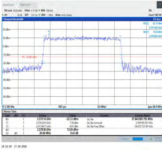
1-N38--30-40-M-8-CP-64QAM-Outer_Full-106@0-An t1-37.843-39.440-<40-PASS
