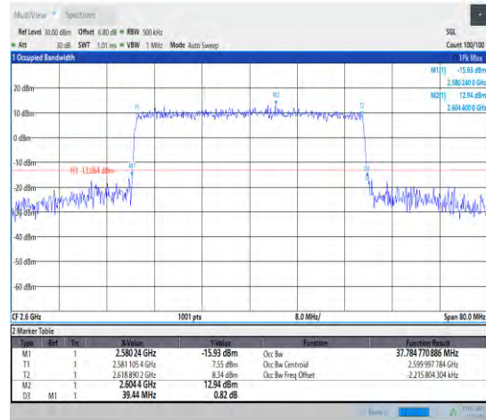
1-N38--30-40-H-6-CP-QPSK-Outer_Full-106@0-Ant 1-37.785-39.440-<40-PASS
