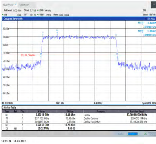
1-N38--30-40-L-7-CP-16QAM-Outer_Full-106@0-Ant 1-37.76-39.520-<40-PASS
