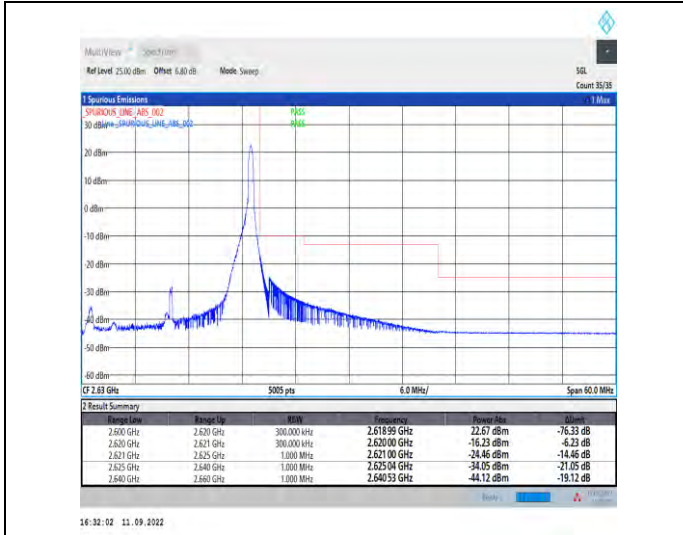
1-N38--30-20-H-2-DFT-PI2BPSK-Edge_1RB_Right-1@50-Ant1-1--PASS-see graph
