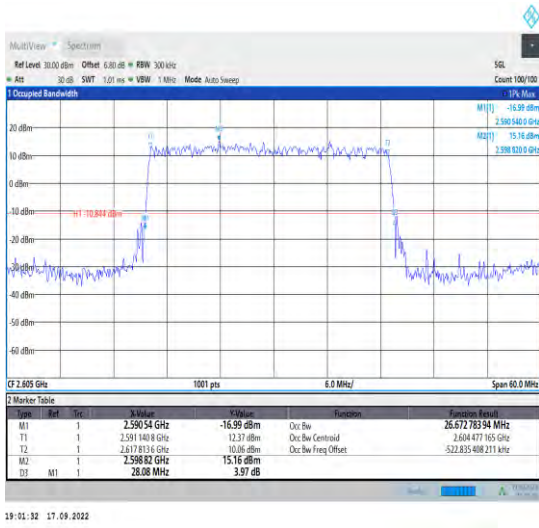
1-N38--30-30-H-2-DFT-PI2BPSK-Outer_Full-75@0-Ant1 Ant1-26.673-28.080<30-PASS
