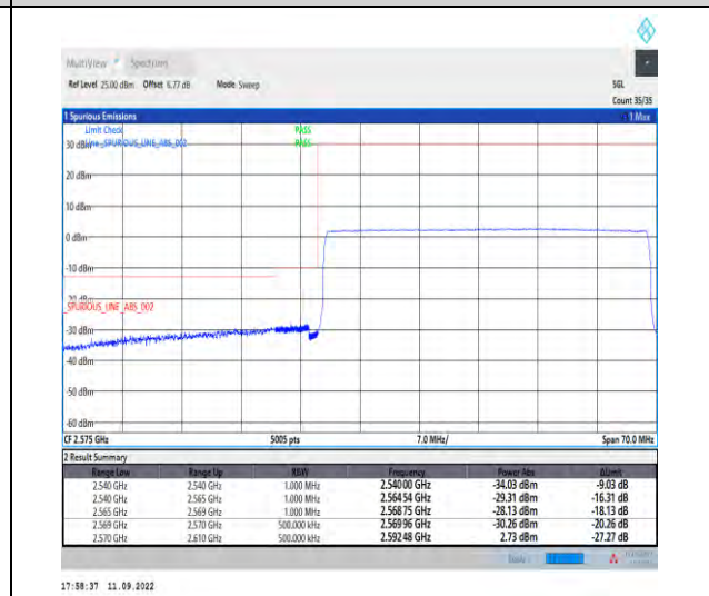
1-N38--30-40-L-6-CP-QPSK-Outer_Full-106@0-Ant1-1--PASS-see graph
