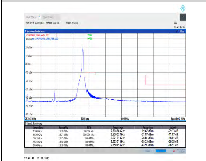
1-N38--30-30-H-5-CP-QPSK-Edge_1RB_Right-1@77-Ant1-1--PASS-see graph
