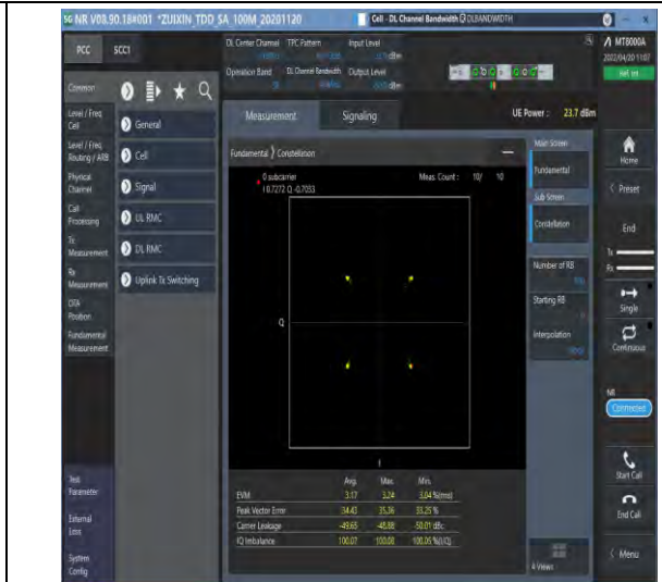
1-N38--30-40-M-2-DFT-QPSK-Outer_Full-100@0-A nt1-see graph-PASS
