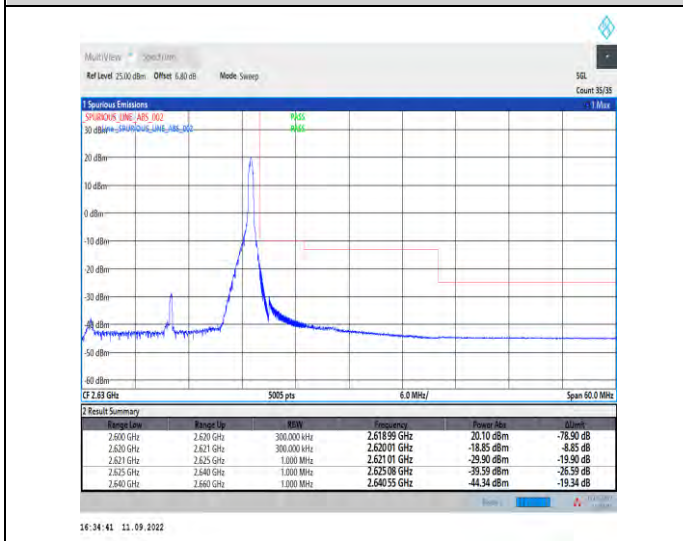
1-N38--30-20-H-5-CP-QPSK-Edge_1RB_Right-1@50-Ant1-1--PASS-see graph
