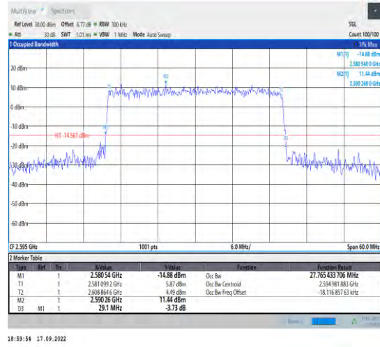
1-N38--30-30-M-8-CP-64QAM-Outer_Full-78@0-Ant 1-27.765-29.100-≤30-PASS
