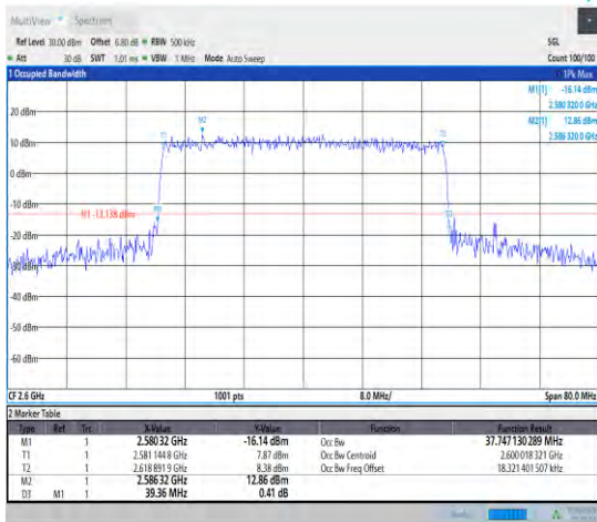
1-N38--30-40-H-7-CP-16QAM-Outer_Full-106@0-An t1-37.747-39.360-<40-PASS
