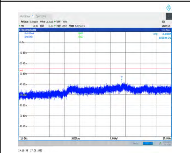
1-N38--30-40-M-1-DFT-PI2BPSK-Inner_1RB_Left-1 @1-12000-27000-Ant1-22108.00--36.39--25-PASS
