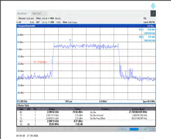
1-N38--30-30-H-9-CP-256QAM-Outer_Full-78@0-Ant t1-27.7-29.040-≤30-PASS
