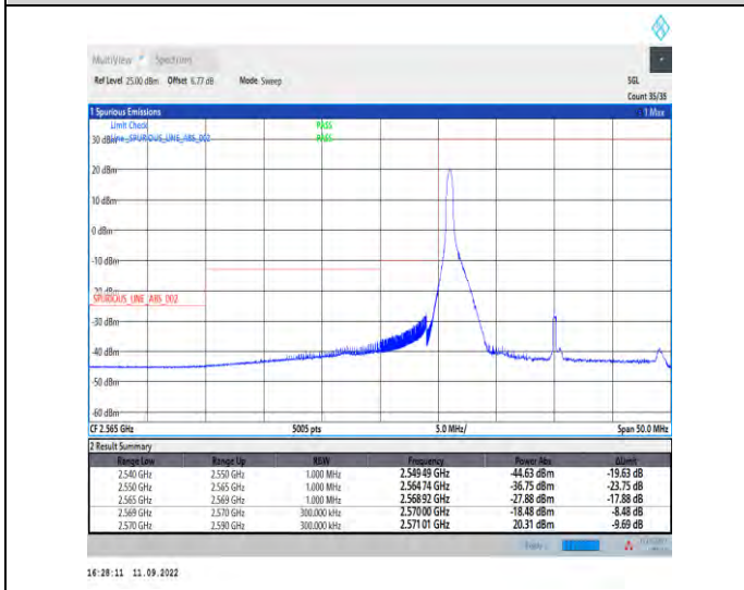
1-N38--30-20-L-4-CP-QPSK-Edge_1RB_Left-1@0-Ant1-1--PASS-see graph
