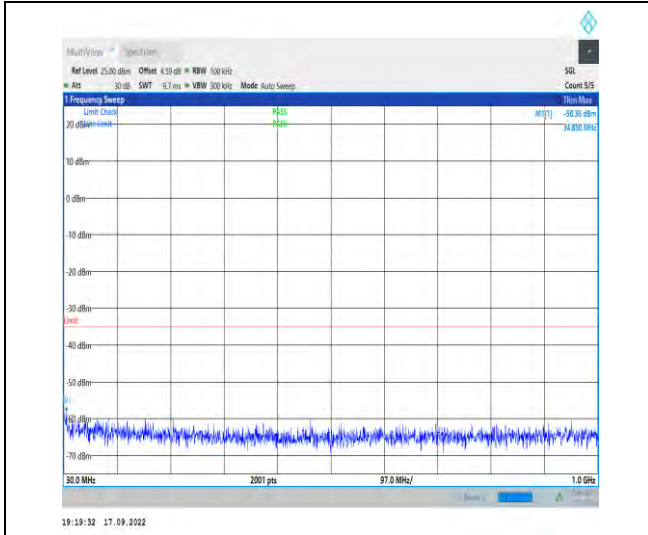
1-N38--30-40-M-1-DFT-PI2BPSK-Inner_1RB_Left-1 @1-30-1000-Ant1-34.85--58.36--35-PASS
