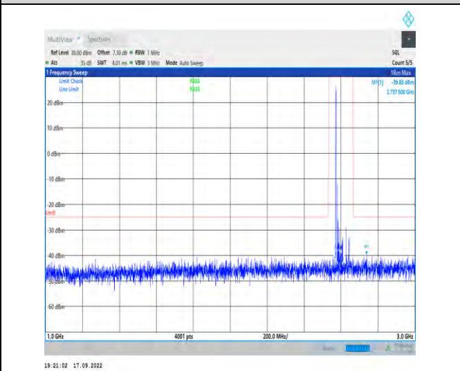
1-N38--30-40-H-1-DFT-PI2BPSK-Inner_1RB_Left-1 @ 1-1000-3000-Ant1-2737.50--39.83--25-PASS
