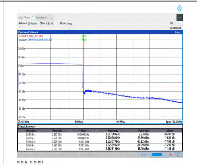
1-N38--30-40-H-6-CP-QPSK-Outer_Full-106@0-Ant1-1--PASS-see graph
