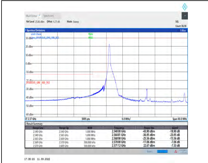
1-N38--30-30-L-1-DFT-PI2BPSK-Edge_1RB_Left-1@0-Ant1-1--PASS-see graph
