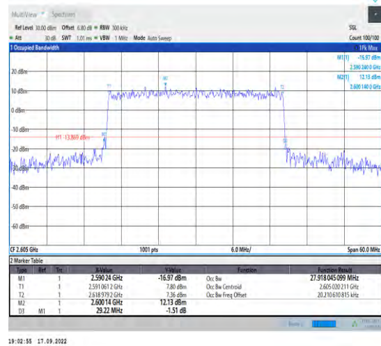
1-N38--30-30-H-7-CP-16QAM-Outer_Full-78@0-Ant 1-27.918-29.220<=30-PASS
