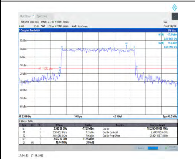
1-N38--30-20-M-7-CP-16QAM-Outer_Full-51@0-Ant 1-18.236-19.440-≤20-PASS
