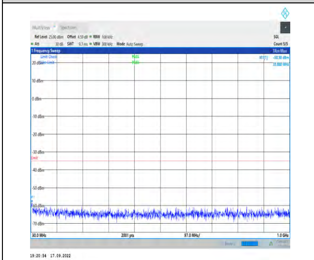
1-N38--30-40-H-1-DFT-PI2BPSK-Inner_1RB_Left-1 @ 1-30-1000-Ant1-33.88--58.58--35-PASS
