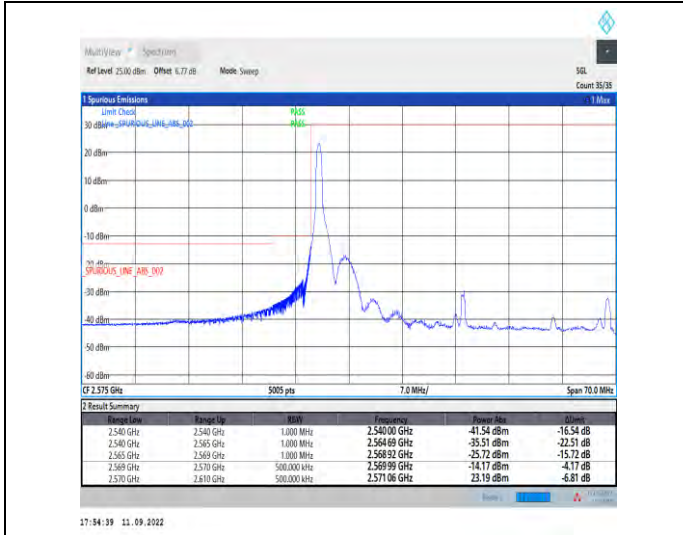
1-N38--30-40-L-1-DFT-PI2BPSK-Edge_1RB_Left-1@0-Ant1-1--PASS-see graph
