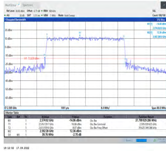
1-N38--30-40-M-7-CP-16QAM-Outer_Full-106@0-A nt1-37.8-39.760-<40-PASS
