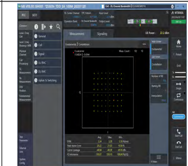
1-N38--30-40-M-4-DFT-64QAM-Outer_Full-100@0-A Ant1-see graph-PASS
