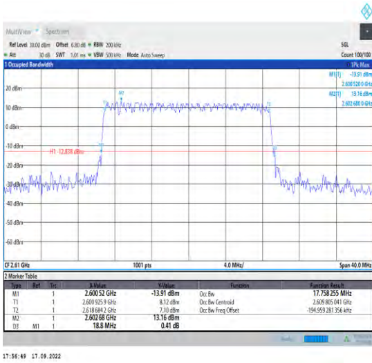
1-N38--30-20-H-3-DFT-16QAM-Outer_Full-50@0-An t1-17.758-18.800-≤20-PASS
