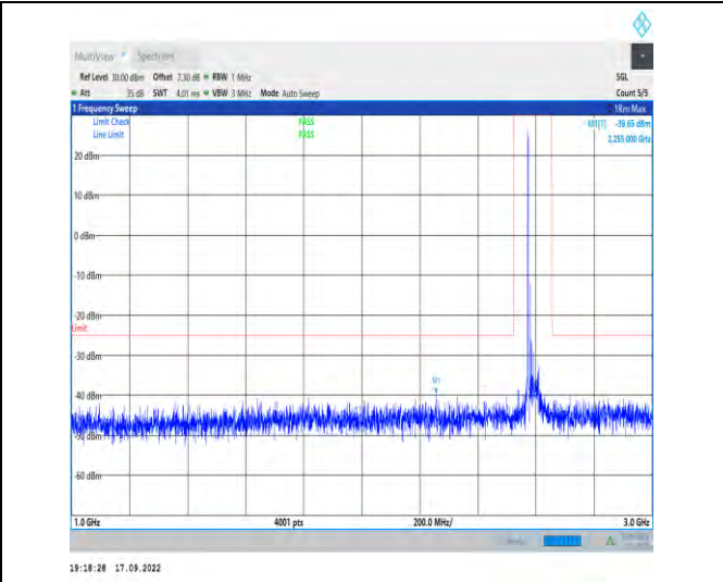
1-N38--30-40-M-1-DFT-PI2BPSK-Inner_1RB_Left-1 @1-1000-3000-Ant1-2187.00--39.72--25-PASS
