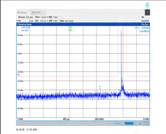
1-N38--30-40-L-1-DFT-PI2BPSK-Inner_1RB_Left-1@ 1-1000-3000-Ant1-2255.00--39.65--25-PASS
