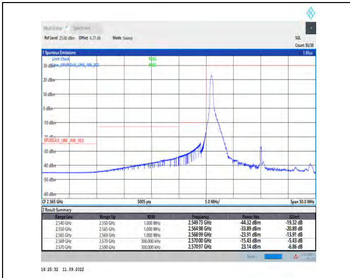
1-N38--30-20-L-1-DFT-PI2BPSK-Edge_1RB_Left-1@0-Ant1-1--PASS-see graph
