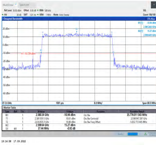
1-N38--30-40-H-1-DFT-QPSK-Outer_Full-100@0-An t1-35.776-37.440-<40-PASS
