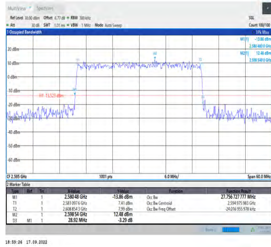
1-N38--30-30-M-6-CP-QPSK-Outer_Full-78@0-Ant1 -27.757-28.920-≤30-PASS
