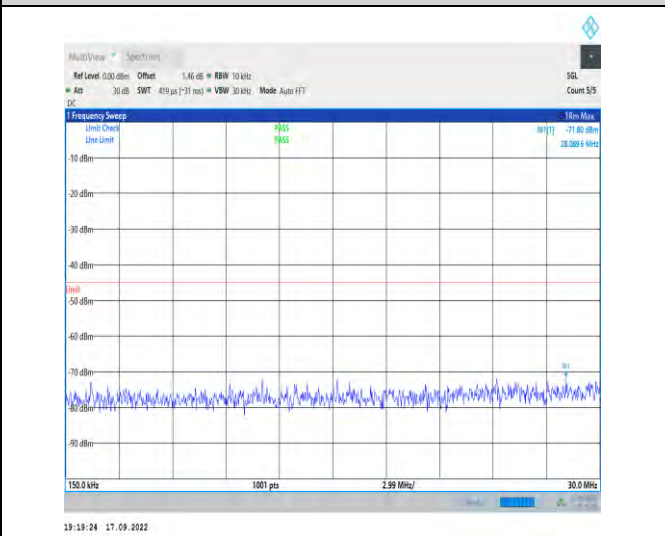
1-N38--30-40-M-1-DFT-PI2BPSK-Inner_1RB_Left-1 @ 1-0.15-30-Ant1-28.09--71.80--45-PASS
