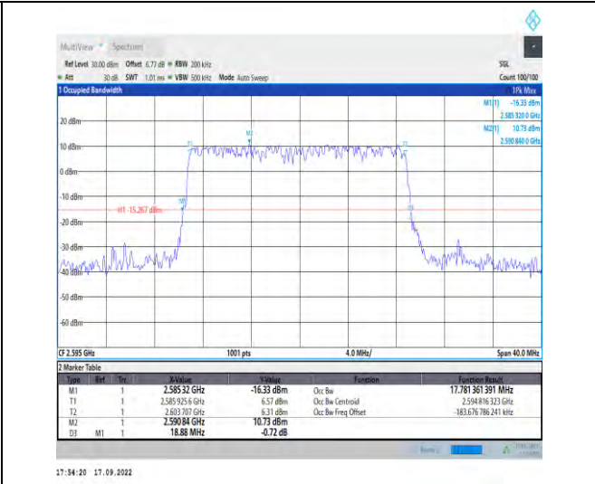
1-N38--30-20-M-5-DFT-256QAM-Outer_Full-50@0-Ant Ant1-17.781-18.880-≤20-PASS
