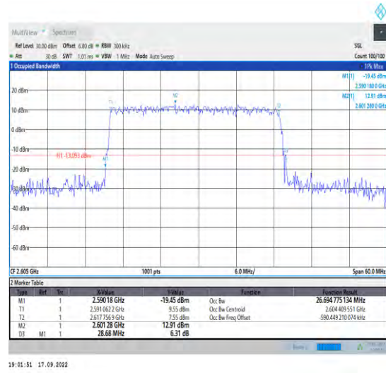
1-N38--30-30-H-3-DFT-16QAM-Outer_Full-75@0-Ant t1-26.695-28.680<30-PASS
