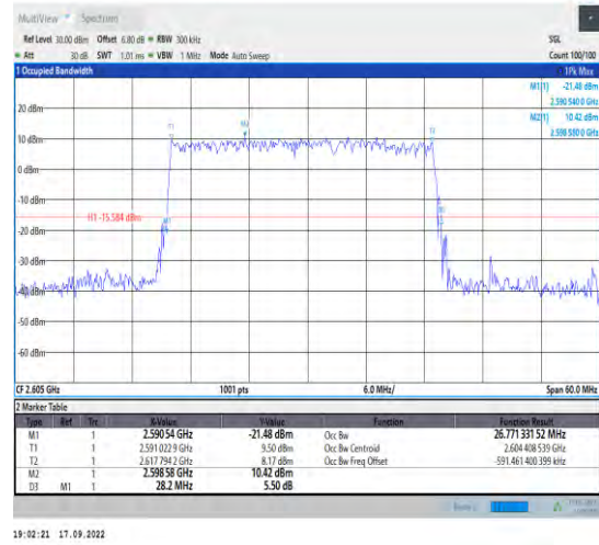
1-N38--30-30-H-5-DFT-256QAM-Outer_Full-75@0-A nt1-26.771-28.200<=30-PASS
