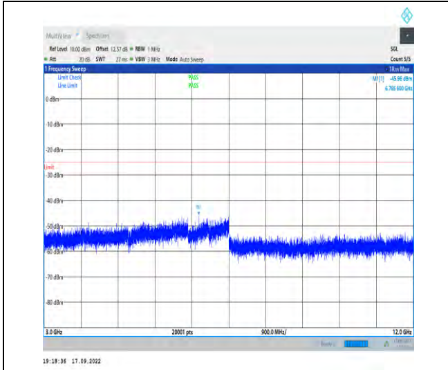
1-N38--30-40-L-1-DFT-PI2BPSK-Inner_1RB_Left-1 @ 1-3000-12000-Ant1-6765.60--45.96--25-PASS
