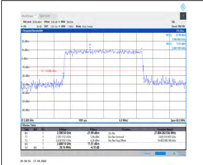
1-N38--30-30-H-8-CP-64QAM-Outer_Full-78@0-Ant 1-27.804-29.160-≤30-PASS
