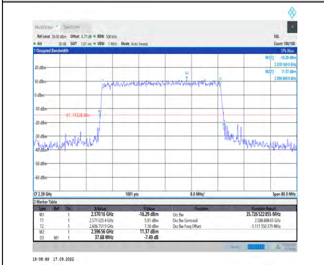
1-N38--30-40-L-5-DFT-256QAM-Outer_Full-100@0-A Ant1-35.727-37.680-≤40-PASS
