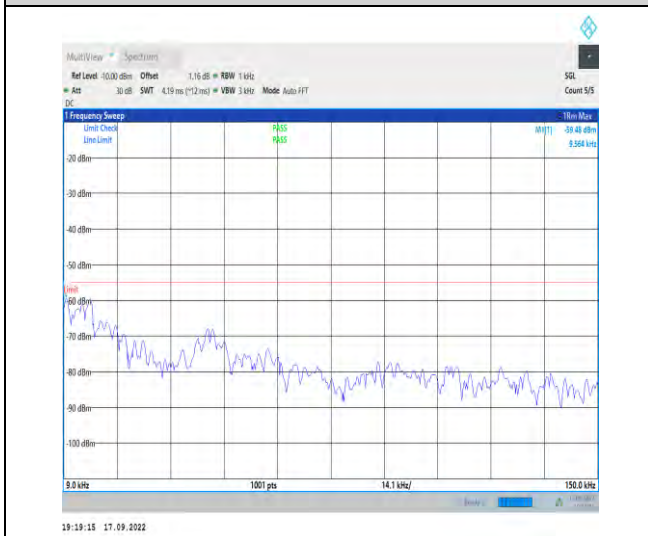
1-N38--30-40-M-1-DFT-PI2BPSK-Inner_1RB_Left-1 @ 1-0.009-0.15-Ant1-0.01--59.48--55-PASS
