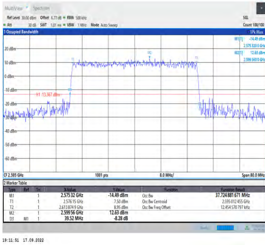
1-N38--30-40-M-6-CP-QPSK-Outer_Full-106@0-Ant 1-37.725-39.520-<40-PASS
