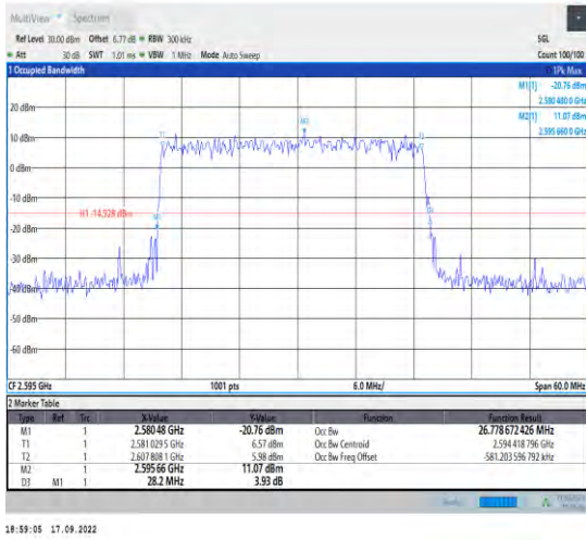
1-N38--30-30-M-5-DFT-256QAM-Outer_Full-75@0-A nt1-26.779-28.200-≤30-PASS
