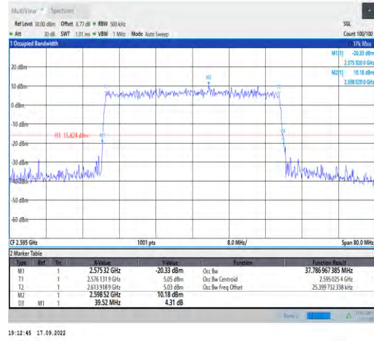
1-N38--30-40-M-9-CP-256QAM-Outer_Full-106@0-Ant Ant1-37.787-39.520-<40-PASS
