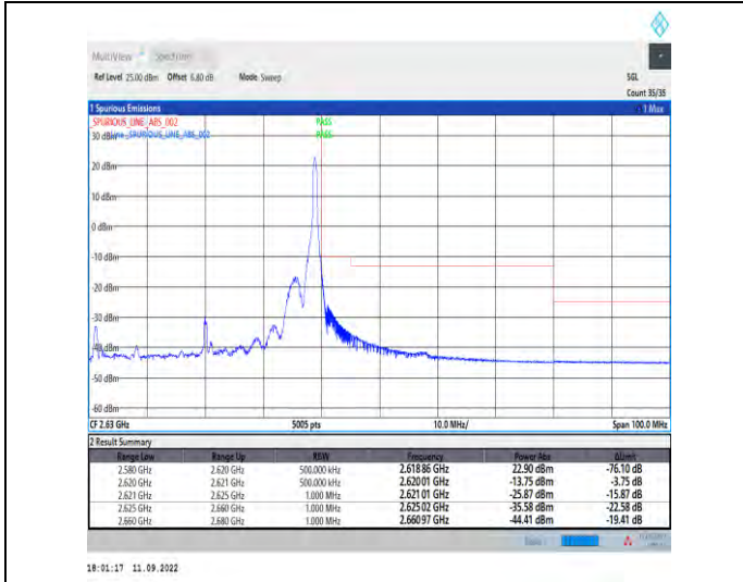
1-N38--30-40-H-2-DFT-PI2BPSK-Edge_1RB_Right-1@105-Ant1-1--PASS-see graph
