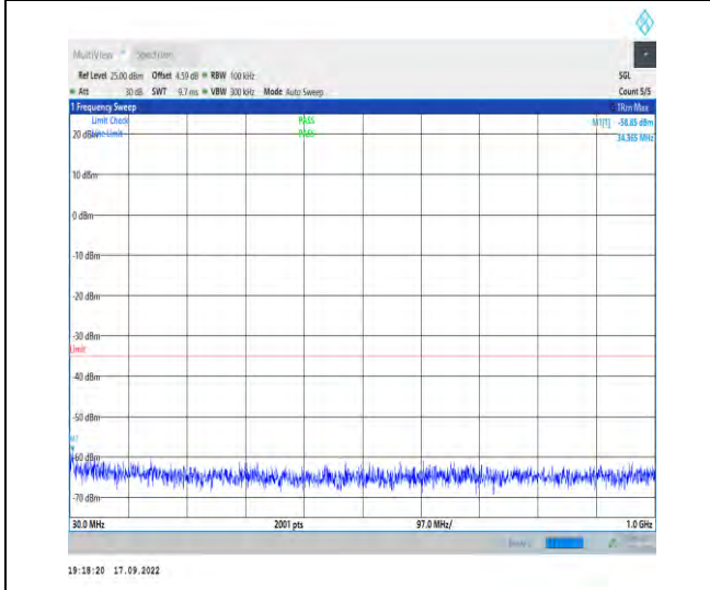
1-N38--30-40-L-1-DFT-PI2BPSK-Inner_1RB_Left-1 @1-30-1000-Ant1-34.37--58.85--35-PASS
