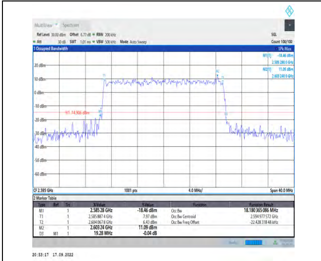
1-N38--30-20-M-8-CP-64QAM-Outer_Full-51@0-Ant 1-18.18-19.280-<20-PASS
