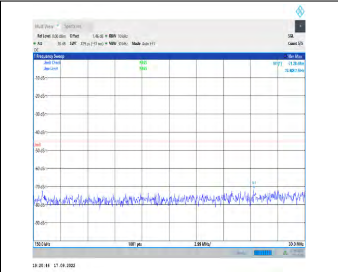
1-N38--30-40-H-1-DFT-PI2BPSK-Inner_1RB_Left-1 @ 1-0.15-30-Ant1-24.39--71.28--45-PASS
