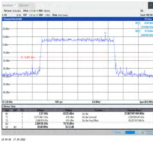
1-N38--30-40-L-9-CP-256QAM-Outer_Full-106@0-A nt1-37.868-39.680-<40-PASS
