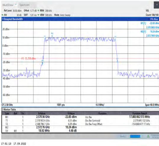
1-N38--30-20-L-5-DFT-256QAM-Outer_Full-50@0-A nt1-17.883-18.920-≤20-PASS
