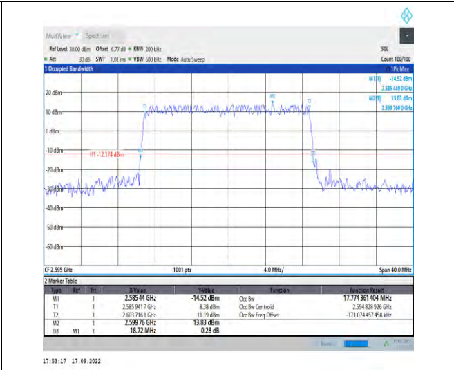
1-N38--30-20-M-1-DFT-QPSK-Outer_Full-50@0-Ant 1-17.774-18.720-<20-PASS
