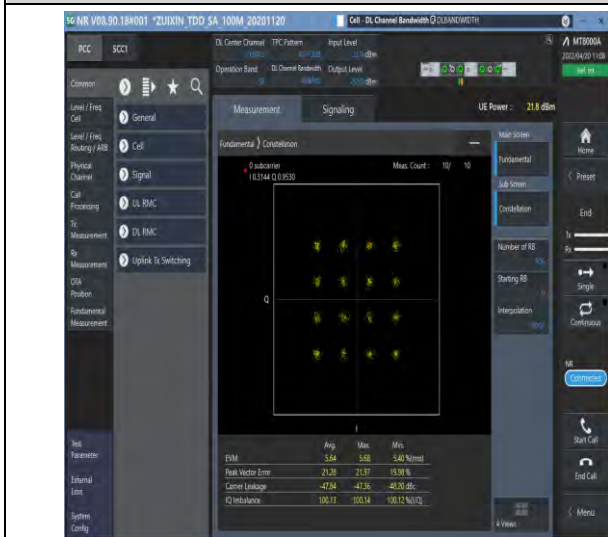
1-N38--30-40-M-7-CP-16QAM-Outer_Full-106@0-Ant1-see graph-PASS
