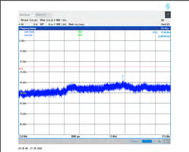
1-N38--30-40-L-1-DFT-PI2BPSK-Inner_1RB_Left-1 @ 1-12000-27000-Ant1-22288.50--37.48--25-PASS
