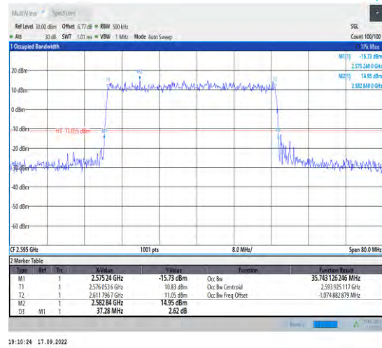
1-N38--30-40-M-1-DFT-QPSK-Outer_Full-100@0-An t1-35.743-37.280-<40-PASS
