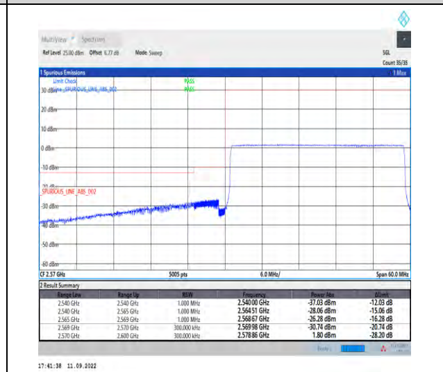
1-N38--30-30-L-6-CP-QPSK-Outer_Full-78@0-Ant1-1--PASS-see graph
