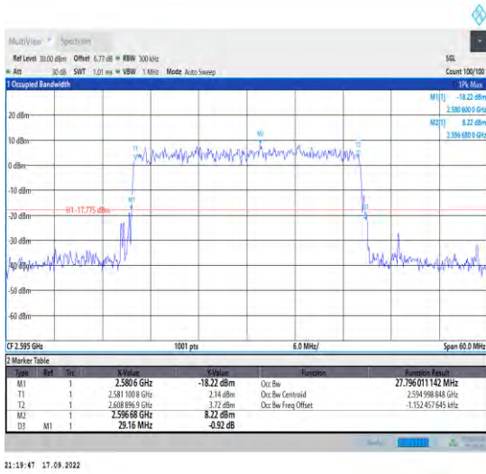
1-N38--30-30-M-9-CP-256QAM-Outer_Full-78@0-Ant t1-27.796-29.160<30-PASS
