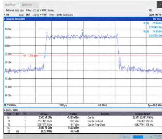
1-N38--30-30-L-1-DFT-QPSK-Outer_Full-75@0-Ant1 -26.611-28.020-≤30-PASS
