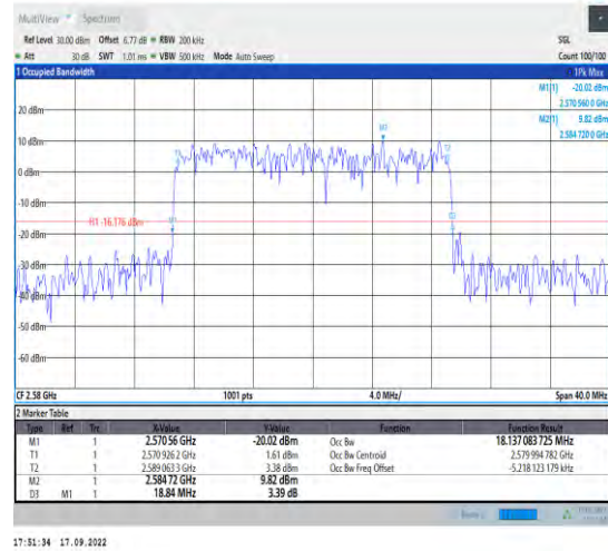
1-N38--30-20-L-6-CP-QPSK-Outer_Full-51@0-Ant1- 18.137-18.840-≤20-PASS
