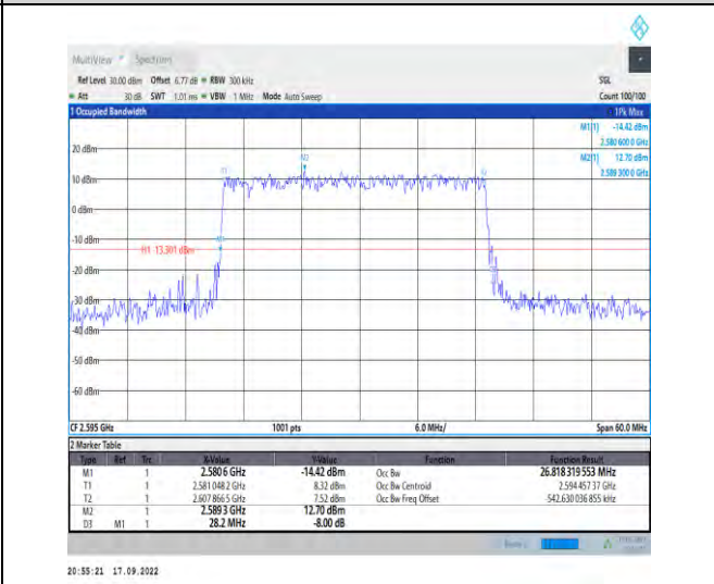
1-N38--30-30-M-4-DFT-64QAM-Outer_Full-75@0-A nt1-26.818-28.200-<30-PASS
