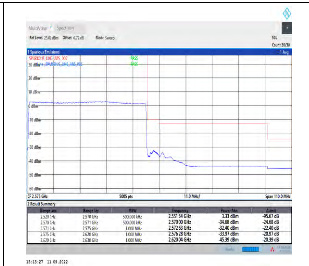
1-N7--15-50-H-3-DFT-PI2BPSK-Outer_Full-270@ 0-Ant1-1--PASS-see graph
