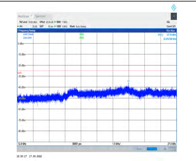
1-N7--15-50-H-1-DFT-PI2BPSK-Inner_1RB_Left-1@ 1-12000-27000-Ant1-22476.50--37.70--25-PASS
