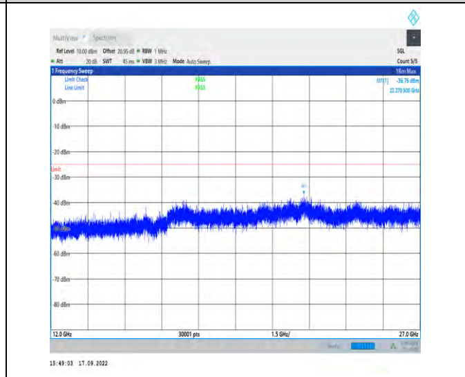
1-N7--15-50-M-1-DFT-PI2BPSK-Inner_1RB_Left-1@ 1-12000-27000-Ant1-22270.50--36.76--25-PASS
