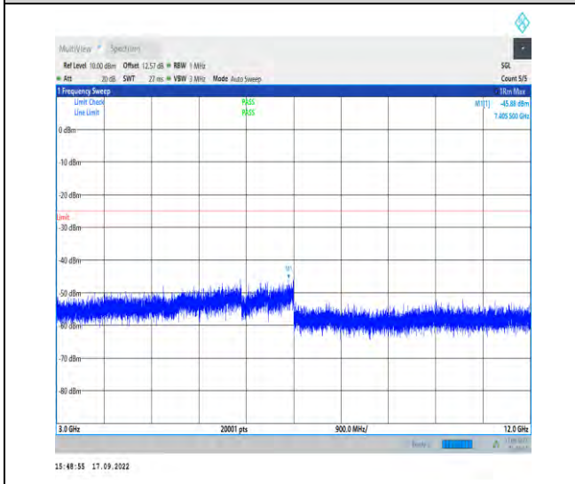
1-N7--15-50-M-1-DFT-PI2BPSK-Inner_1RB_Left-1 @1-3000-12000-Ant1-7405.50--45.88--25-PASS
