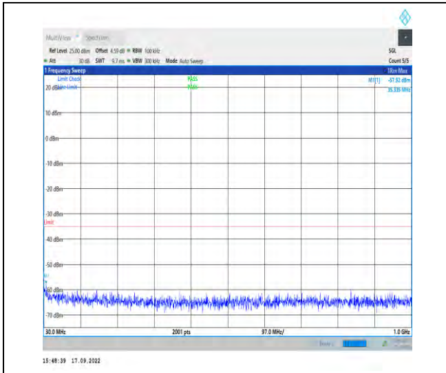
1-N7--15-50-M-1-DFT-PI2BPSK-Inner_1RB_Left-1 @1-30-1000-Ant1-35.34--57.92--35-PASS
