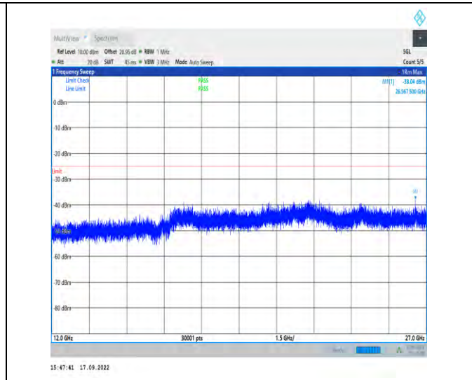
1-N7--15-50-L-1-DFT-PI2BPSK-Inner_1RB_Left-1@ -12000-27000-Ant1-26567.50--38.04--25-PASS
