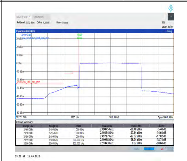
1-N7--15-40-L-6-CP-QPSK-Outer_Full-216@0-Ant1-1--PASS-see graph
