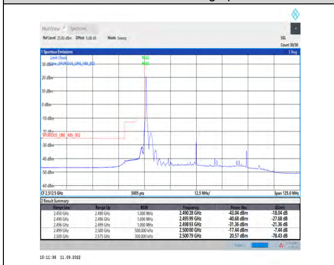
1-N7--15-50-L-4-CP-QPSK-Edge_1RB_Left-1@0-Ant1-1--PASS-see graph
