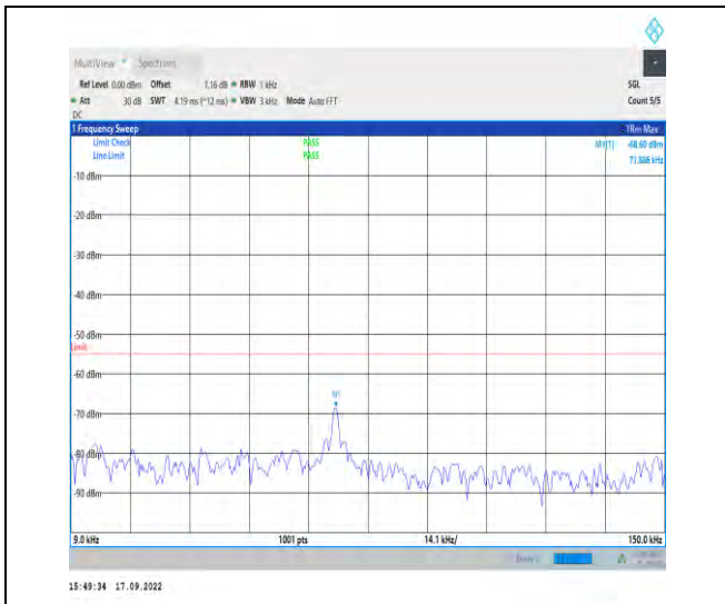
1-N7--15-50-H-1-DFT-PI2BPSK-Inner_1RB_Left-1 @ 1-0.009-0.15-Ant1-0.07--68.60--55-PASS
