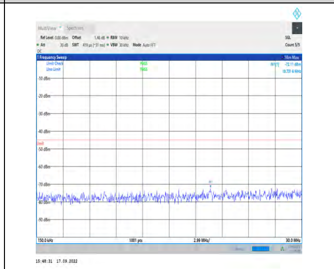
1-N7--15-50-M-1-DFT-PI2BPSK-Inner_1RB_Left-1@ 1-0.15-30-Ant1-19.73--72.11--45-PASS
