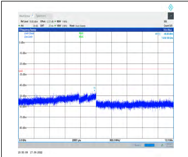
1-N7--15-50-H-1-DFT-PI2BPSK-Inner_1RB_Left-1 @1-3000-12000-Ant1-7418.10--46.06--25-PASS
