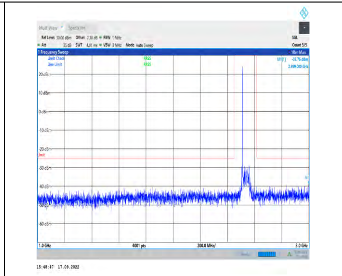
1-N7--15-50-M-1-DFT-PI2BPSK-Inner_1RB_Left-1@ 1-1000-3000-Ant1-2999.00--38.76--25-PASS
