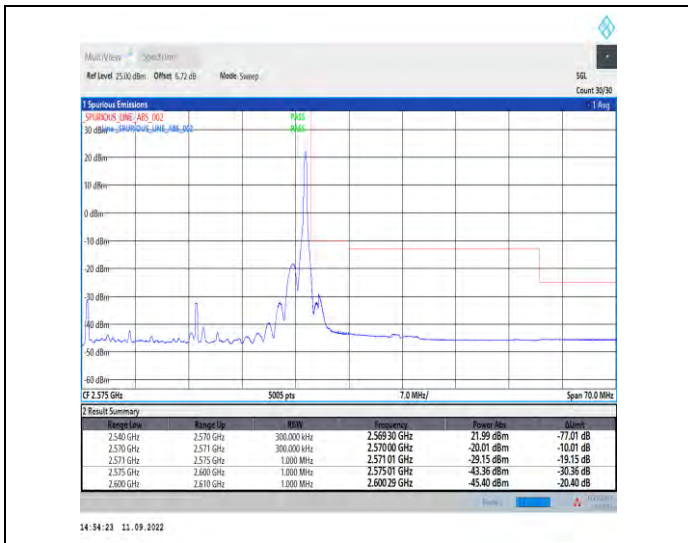
1-N7--15-30-H-2-DFT-PI2BPSK-Edge_1RB_Right-1@159-Ant1-1--PASS-see graph
