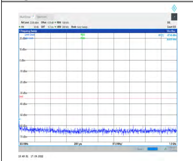
1-N7--15-50-H-1-DFT-PI2BPSK-Inner_1RB_Left-1 @ 1-30-1000-Ant1-30.97--57.45--35-PASS
