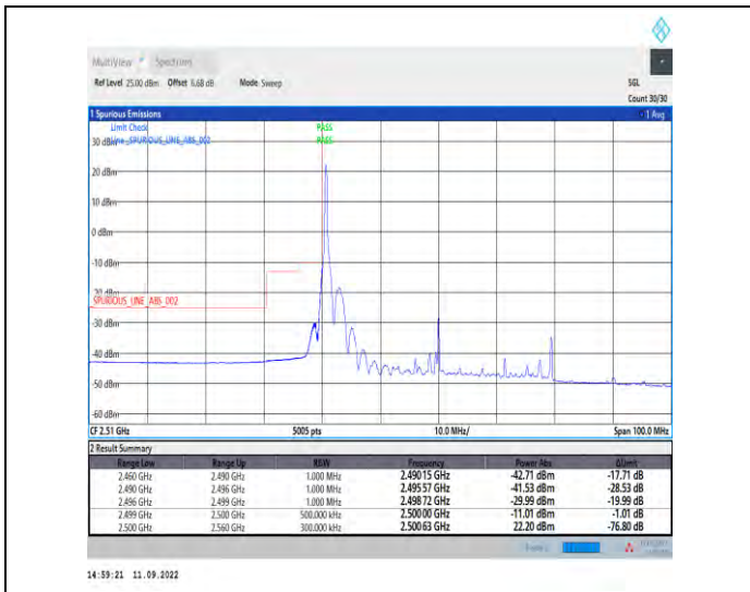
1-N7--15-40-L-1-DFT-PI2BPSK-Edge_1RB_Left-1@0-Ant1-1--PASS-see graph
