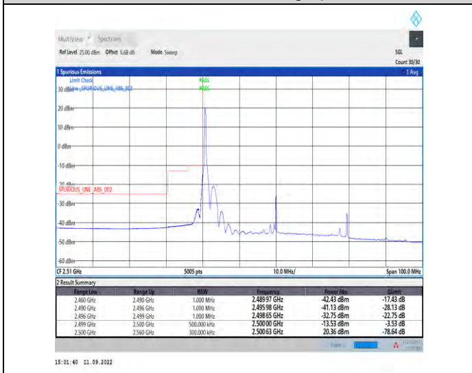
1-N7--15-40-L-4-CP-QPSK-Edge_1RB_Left-1@0-Ant1-1--PASS-see graph
