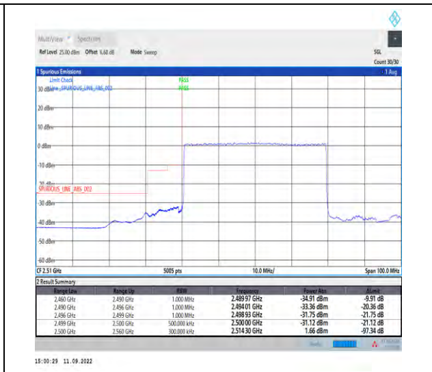
1-N7--15-40-L-3-DFT-PI2BPSK-Outer_Full-216@0-Ant1-1--PASS-see graph
