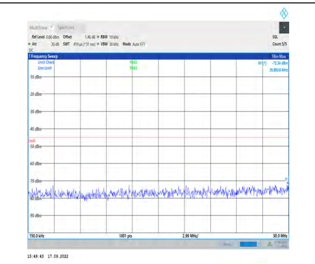
1-N7--15-50-H-1-DFT-PI2BPSK-Inner_1RB_Left-1 @ 1-0.15-30-Ant1-29.85--72.34--45-PASS
