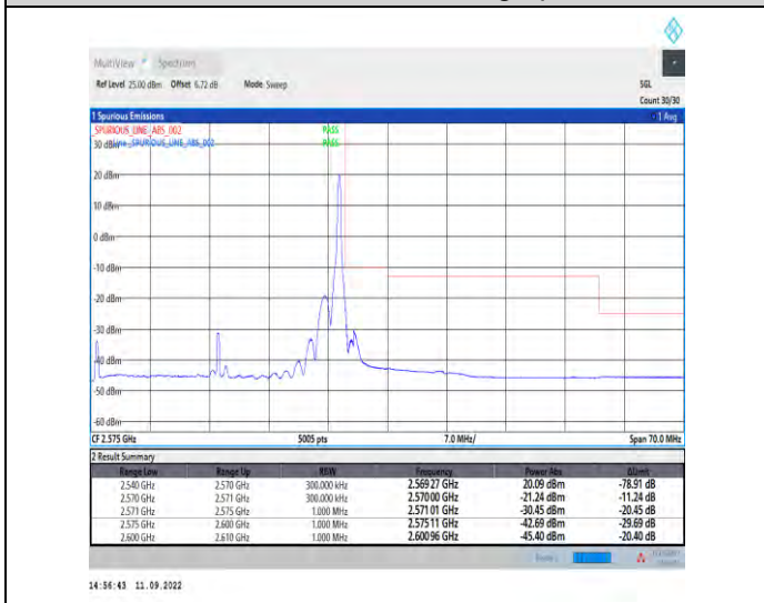
1-N7--15-30-H-5-CP-QPSK-Edge_1RB_Right-1@159-Ant1-1--PASS-see graph
