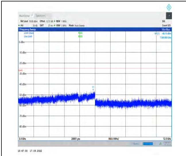
1-N7--15-50-L-1-DFT-PI2BPSK-Inner_1RB_Left-1@ 1-3000-12000-Ant1-7393.80--46.10--25-PASS
