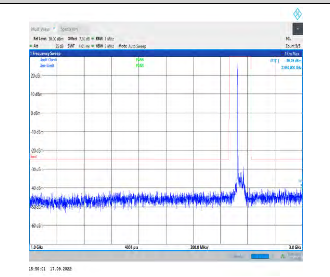
1-N7--15-50-H-1-DFT-PI2BPSK-Inner_1RB_Left-1 @ 1-1000-3000-Ant1-2992.00--39.49--25-PASS
