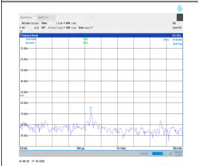
1-N7--15-50-M-1-DFT-PI2BPSK-Inner_1RB_Left-1 @1-0.009-0.15-Ant1-0.07--67.96--55-PASS
