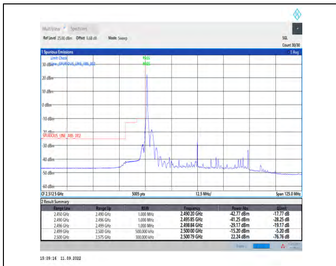
1-N7--15-50-L-1-DFT-PI2BPSK-Edge_1RB_Left-1@0-Ant1-1--PASS-see graph
