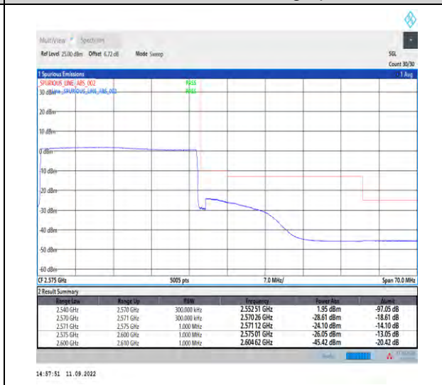
1-N7--15-30-H-6-CP-QPSK-Outer_Full-160@0-Ant1-1--PASS-see graph
