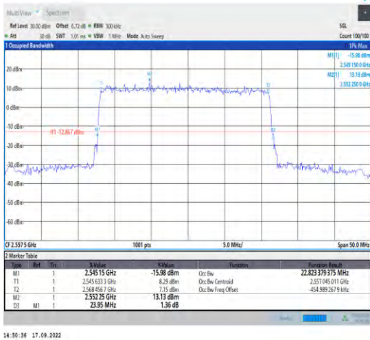
1-N7--15-25-H-5-DFT-256QAM-Outer_Full-128@0-A nt1-22.823-23.950-<25-PASS
