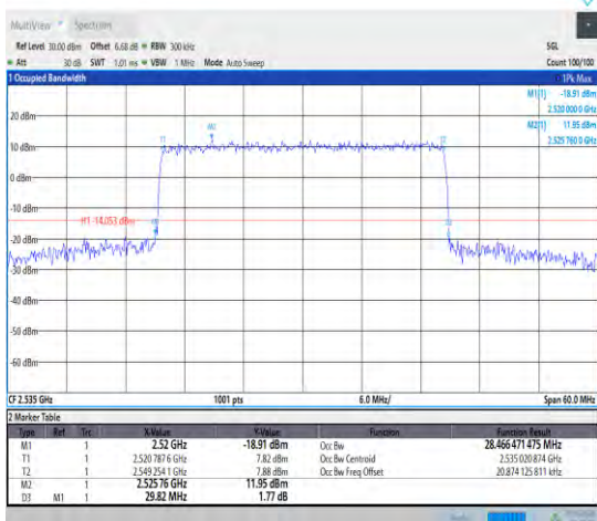
1-N7--15-30-M-7-CP-16QAM-Outer_Full-160@0-Ant 1-28.466-29.820-<30-PASS
