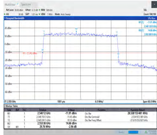
1-N7--15-30-H-1-DFT-QPSK-Outer_Full-160@0-Ant 1-28.538-29.760-≤30-PASS
