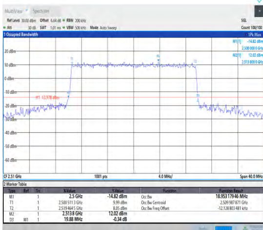
1-N7--15-20-L-6-CP-QPSK-Outer_Full-106@0-Ant1- 18.953-19.880-<20-PASS
