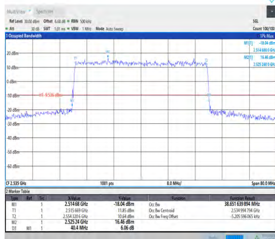
1-N7--15-40-M-1-DFT-QPSK-Outer_Full-216@0-Ant t1-38.652-40.400-≤40-PASS
