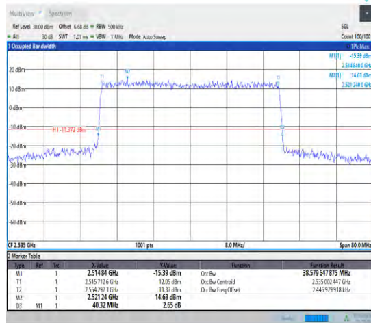
1-N7--15-40-M-3-DFT-16QAM-Outer_Full-216@0-An t1-38.58-40.320-<40-PASS
