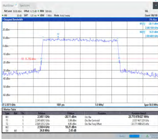
1-N7--15-25-H-9-CP-256QAM-Outer_Full-133@0-Ant t1-23.716-24.800-<25-PASS
