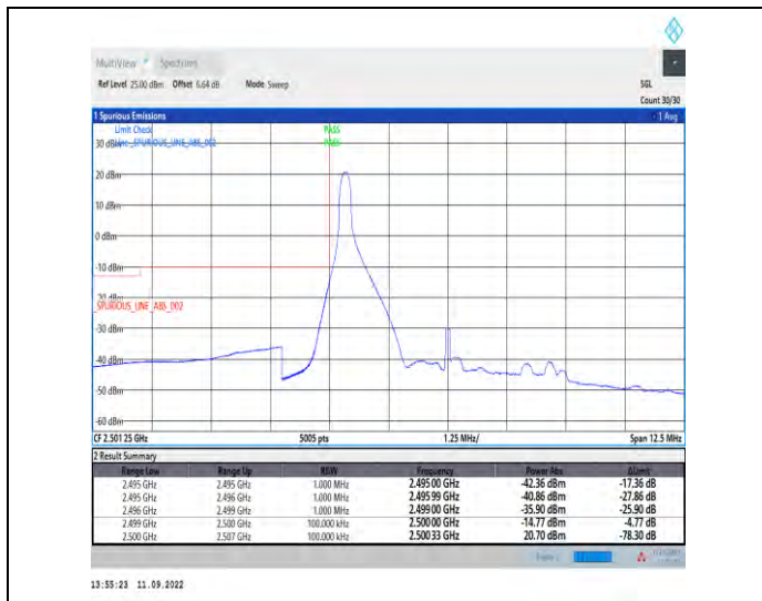
1-N7--15-5-L-1-DFT-PI2BPSK-Edge_1RB_Left-1@0-Ant1-1--PASS-see graph
