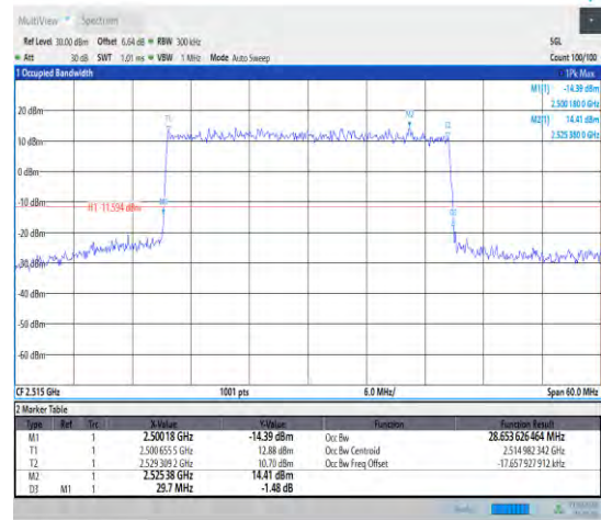
1-N7--15-30-L-1-DFT-QPSK-Outer_Full-160@0-Ant1 -28.654-29.700-<30-PASS
