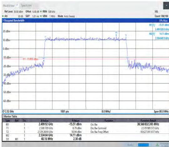
1-N7--15-40-L-7-CP-16QAM-Outer_Full-216@0-Ant t1-38.561-40.160-≤40-PASS
