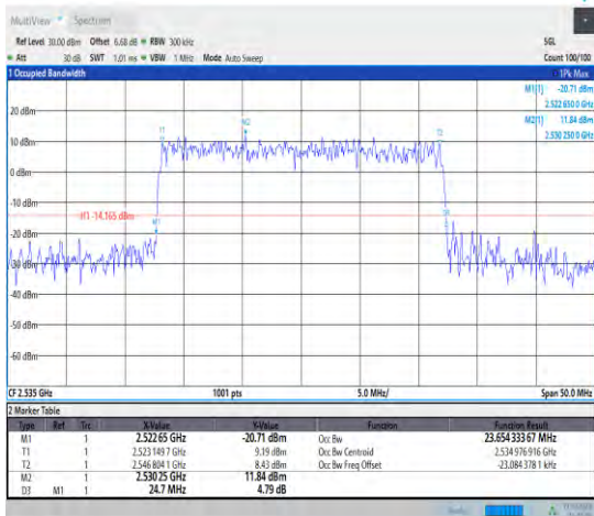
1-N7--15-25-M-6-CP-QPSK-Outer_Full-133@0-Ant1 -23.654-24.700-<25-PASS
