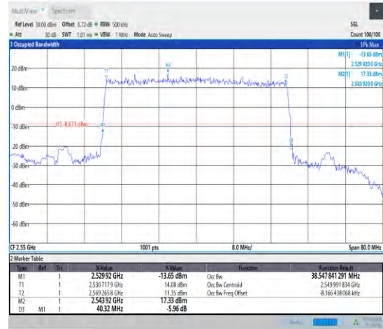
1-N7--15-40-H-2-DFT-PI2BPSK-Outer_Full-216@0-Ant t1-38.548-40.320-<40-PASS
