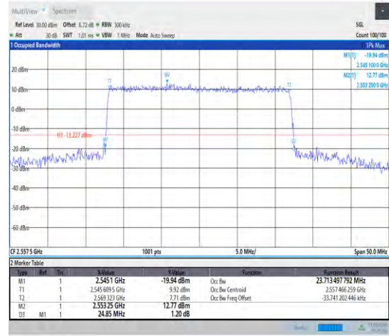
1-N7--15-25-H-8-CP-64QAM-Outer_Full-133@0-Ant 1-23.713-24.850-<25-PASS
