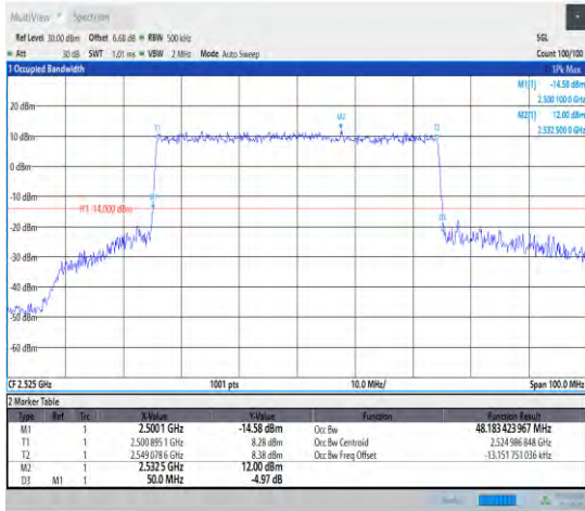
1-N7--15-50-L-8-CP-64QAM-Outer_Full-270@0-Ant 1-48.183-50.000-≤50-PASS
