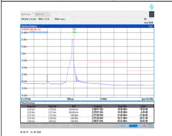
1-N7--15-20-H-5-CP-QPSK-Edge_1RB_Right-1@105-Ant1-1--PASS-see graph
