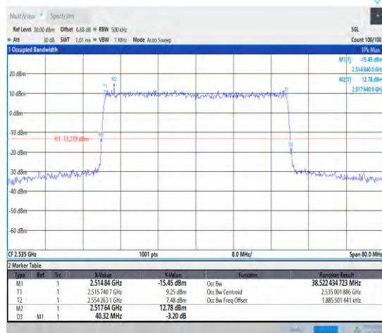
1-N7--15-40-M-5-DFT-256QAM-Outer_Full-216@0-A nt1-38.522-40.320-<40-PASS
