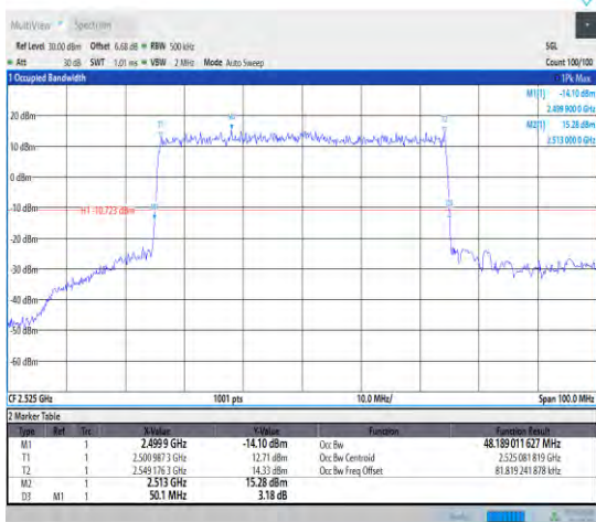
1-N7--15-50-L-2-DFT-PI2BPSK-Outer_Full-270@0-A nt1-48.189-50.100-<50-PASS
