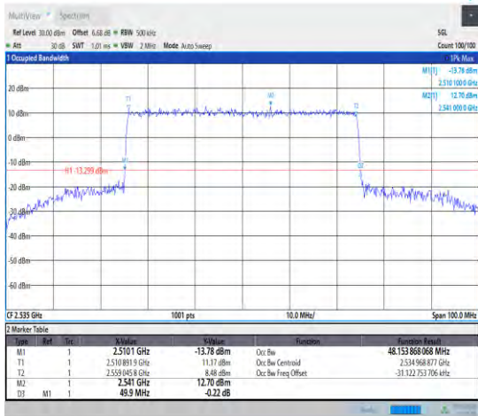
1-N7--15-50-M-7-CP-16QAM-Outer_Full-270@0-Ant 1-48.154-49.900-≤50-PASS
