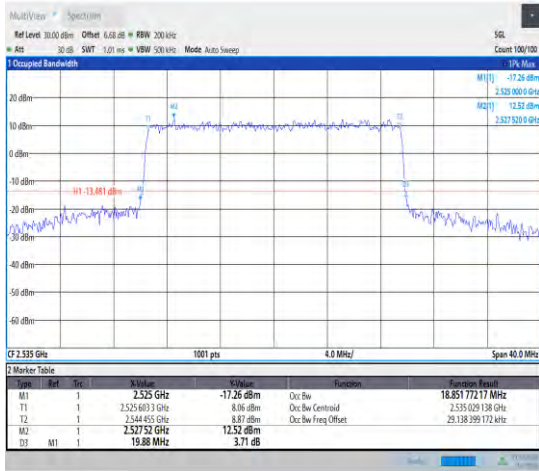
1-N7--15-20-M-7-CP-16QAM-Outer_Full-106@0-Ant 1-18.852-19.880-≤20-PASS
