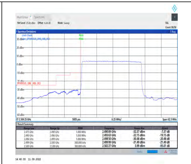
1-N7--15-25-L-3-DFT-PI2BPSK-Outer_Full-128@0-Ant1-1--PASS-see graph
