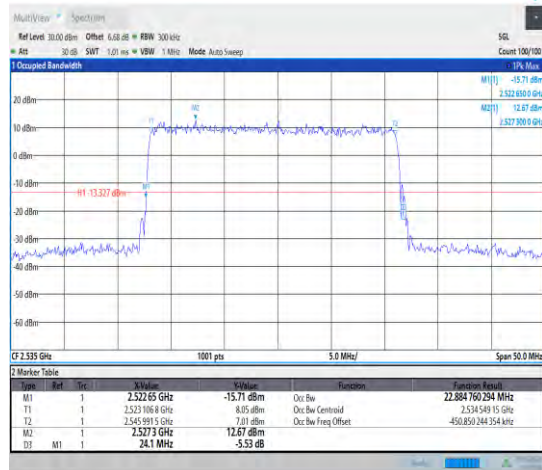
1-N7--15-25-M-5-DFT-256QAM-Outer_Full-128@0-A nt1-22.885-24.100-<25-PASS
