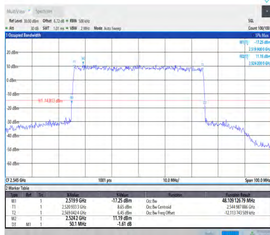
1-N7--15-50-H-5-DFT-256QAM-Outer_Full-270@0-A nt1-48.109-50.100-≤50-PASS
