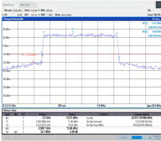
1-N7--15-25-L-1-DFT-QPSK-Outer_Full-128@0-Ant1 -22.915-24.100-≤25-PASS
