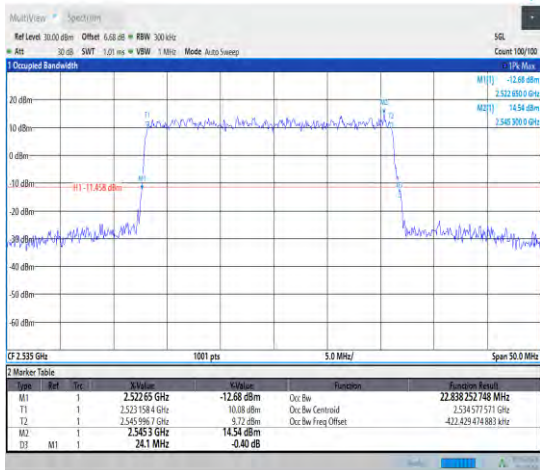
1-N7--15-25-M-4-DFT-64QAM-Outer_Full-128@0-An t1-22.838-24.100-<25-PASS
