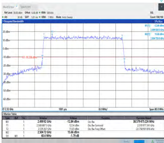
1-N7--15-40-L-1-DFT-QPSK-Outer_Full-216@0-Ant1 1-38.579-40.400-≤40-PASS
