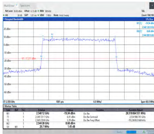
1-N7--15-30-H-9-CP-256QAM-Outer_Full-160@0-Ant 1-28.518-29.700-≤30-PASS
