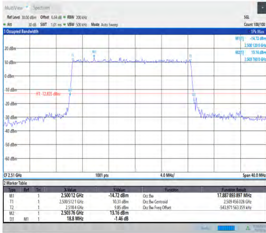
1-N7--15-20-L-4-DFT-64QAM-Outer_Full-100@0-Ant 1-17.888-18.800-<20-PASS
