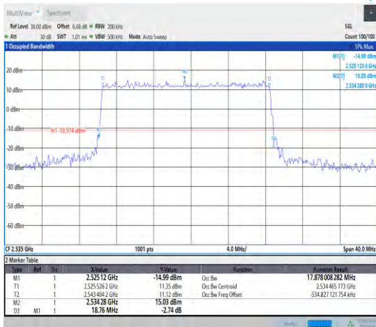
1-N7--15-20-M-1-DFT-QPSK-Outer_Full-100@0-Ant 1-17.878-18.760-≤20-PASS
