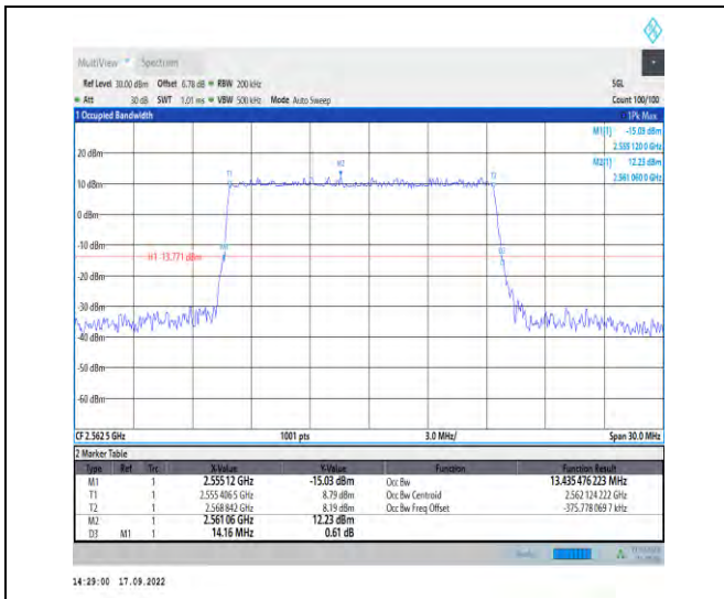
1-N7--15-15-H-5-DFT-256QAM-Outer_Full-75@0-An t1-13.435-14.160-≤15-PASS
