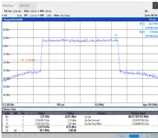
1-N7--15-50-M-9-CP-256QAM-Outer_Full-270@0-A nt1-48.212-50.100-≤50-PASS
