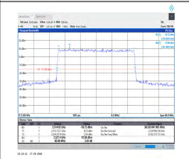
1-N7--15-40-M-9-CP-256QAM-Outer_Full-216@0-Ant nt1-38.535-40.080-≤40-PASS
