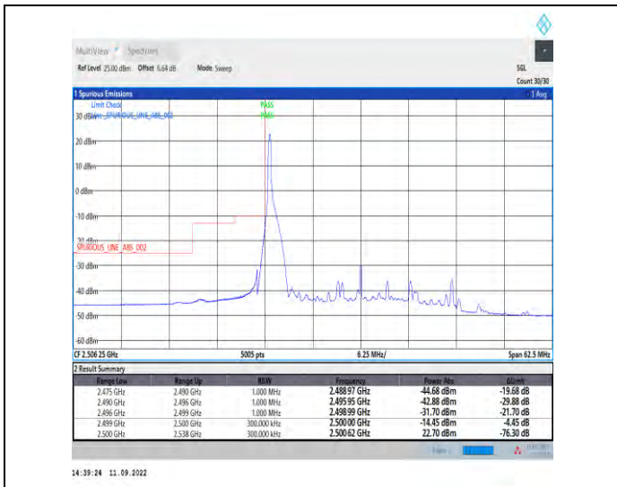
1-N7--15-25-L-1-DFT-PI2BPSK-Edge_1RB_Left-1@0-Ant1-1--PASS-see graph
