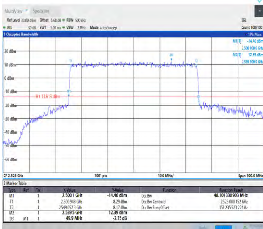
1-N7--15-50-L-6-CP-QPSK-Outer_Full-270@0-Ant1- 48.104-49.900-≤50-PASS
