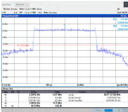
1-N7--15-40-H-7-CP-16QAM-Outer_Full-216@0-Ant 1-38.471-40.160-<=40-PASS
