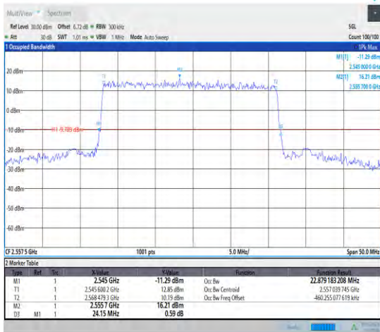
1-N7--15-25-H-1-DFT-QPSK-Outer_Full-128@0-Ant 1-22.879-24.150-≤25-PASS
