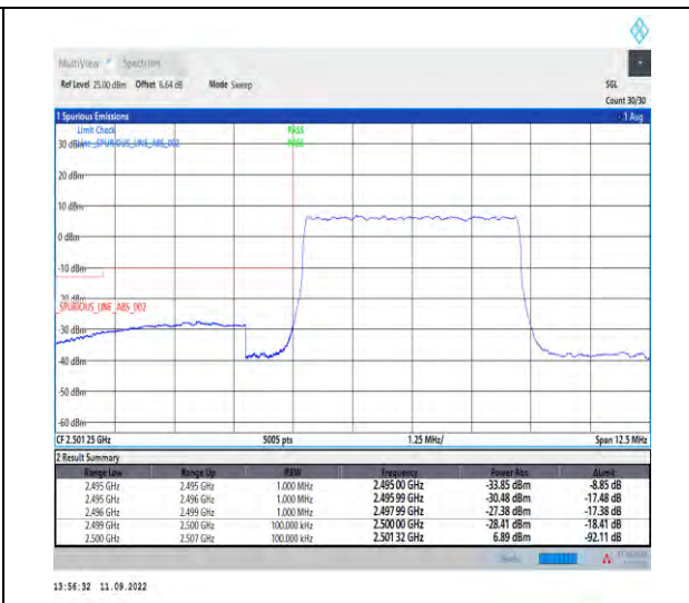
1-N7--15-5-L-3-DFT-PI2BPSK-Outer_Full-25@0-Ant1-1--PASS-see graph
