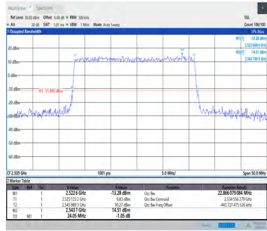
1-N7--15-25-M-3-DFT-16QAM-Outer_Full-128@0-Ant t1-22.866-24.050-<25-PASS
