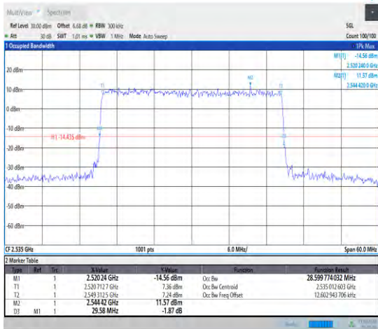
1-N7--15-30-M-5-DFT-256QAM-Outer_Full-160@0-A nt1-28.6-29.580-<30-PASS
