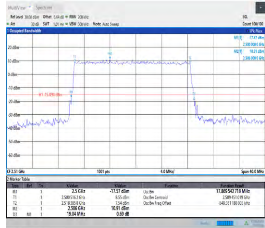
1-N7--15-20-L-5-DFT-256QAM-Outer_Full-100@0-A nt1-17.87-19.040-<20-PASS
