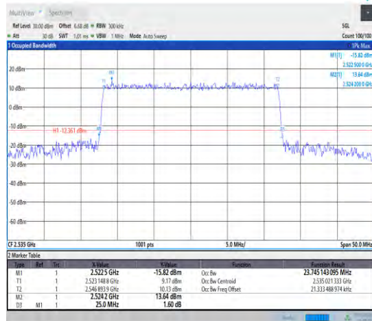
1-N7--15-25-M-7-CP-16QAM-Outer_Full-133@0-Ant 1-23.745-25.000-<25-PASS
