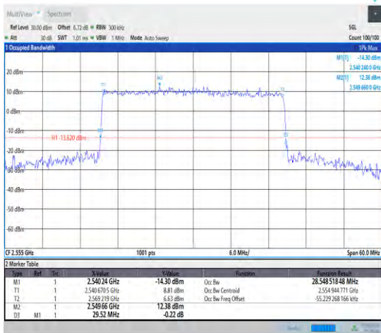
1-N7--15-30-H-8-CP-64QAM-Outer_Full-160@0-Ant 1-28.549-29.520-≤30-PASS
