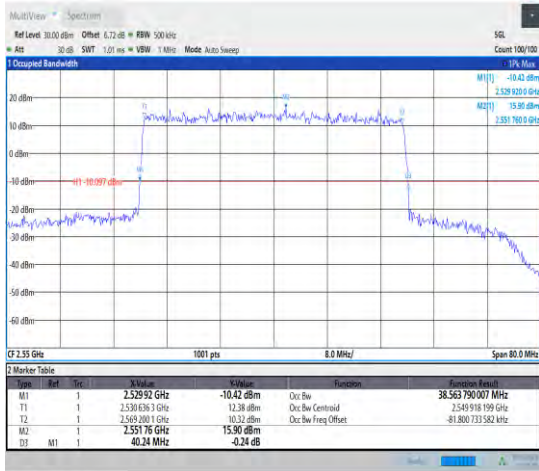
1-N7--15-40-H-1-DFT-QPSK-Outer_Full-216@0-Ant t1-38.564-40.240-<40-PASS
