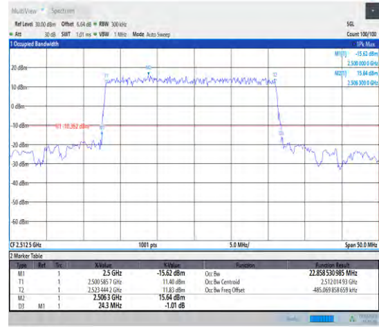
1-N7--15-25-L-2-DFT-PI2BPSK-Outer_Full-128@0-Ant1 -22.859-24.300-≤25-PASS
