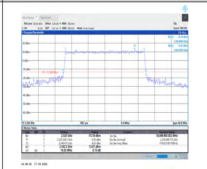
1-N7--15-20-M-6-CP-QPSK-Outer_Full-106@0-Ant1 -18.948-19.920-<20-PASS
