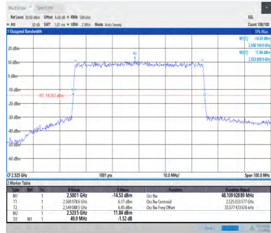
1-N7--15-50-L-5-DFT-256QAM-Outer_Full-270@0-A nt1-48.11-49.900-≤50-PASS
