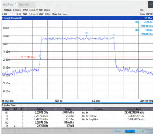
1-N7--15-30-M-9-CP-256QAM-Outer_Full-160@0-A nt1-28.539-29.760-≤30-PASS
