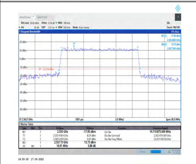
1-N7--15-15-H-8-CP-64QAM-Outer_Full-79@0-Ant1-1 14.111-14.910-≤15-PASS
