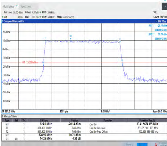
1-N5--15-15-L-5-DFT-256QAM-Outer_Full-75@0-An t1-13.413-14.250≤15-PASS
