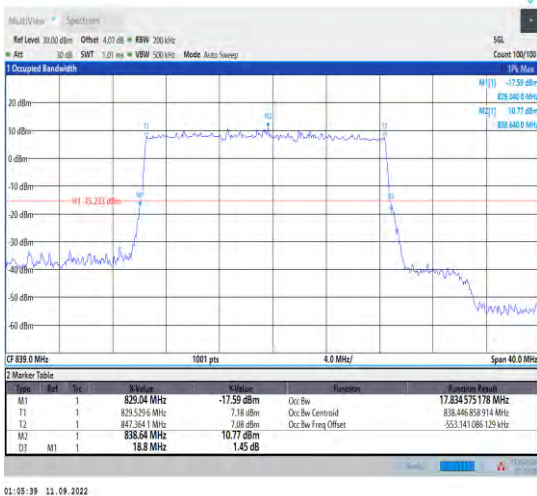
1-N5--15-20-H-8-CP-64QAM-Outer_Full-106@0-Ant 1-39.502-40.000-≤20-PASS
