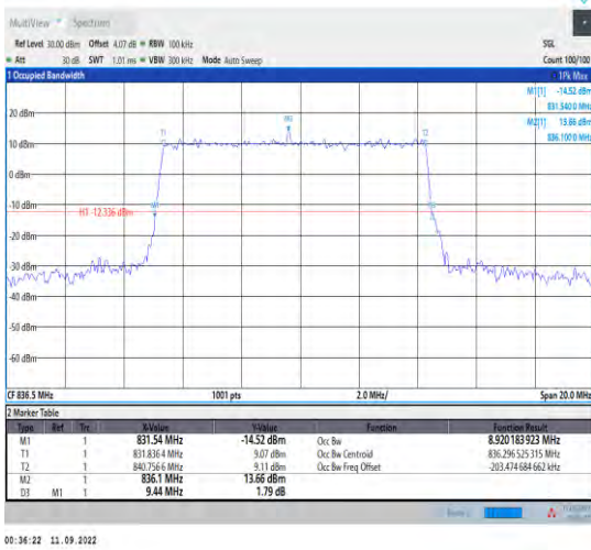
1-N5--15-10-M-3-DFT-16QAM-Outer_Full-50@0-Ant 1-8.92-9.440-≤10-PASS
