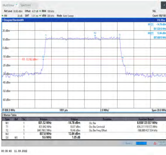
1-N5--15-10-M-1-DFT-QPSK-Outer_Full-50@0-Ant1 -8.938-9.600-≤10-PASS
