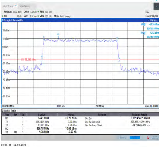
1-N5--15-10-L-8-CP-64QAM-Outer_Full-52@0-Ant1- 9.289-9.780-≤10-PASS
