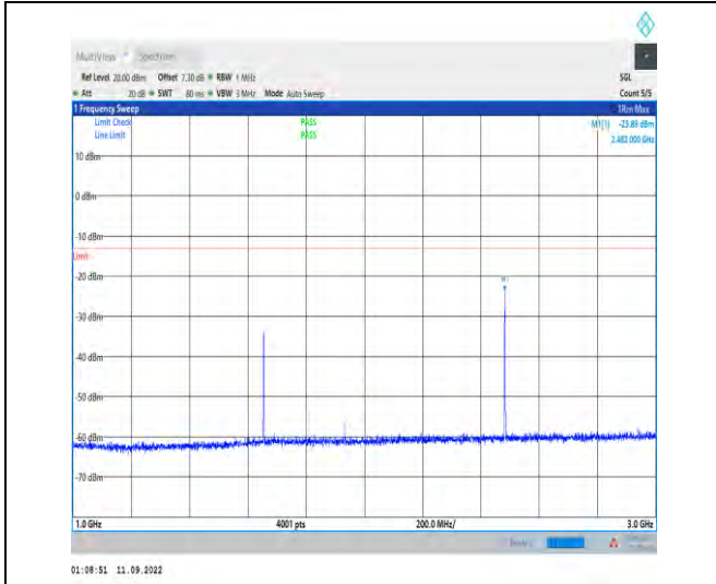
1-N5--15-20-M-1-DFT-PI2BPSK-Inner_1RB_Left-1@ 1-1000-3000-Ant1-2482.00--23.89--13-PASS
