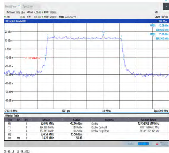
1-N5--15-15-L-2-DFT-PI2BPSK-Outer_Full-75@0-Ant t1-13.453-14.220-≤15-PASS
