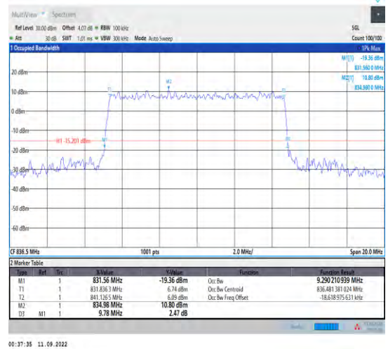
1-N5--15-10-M-8-CP-64QAM-Outer_Full-52@0-Ant1 -9.29-9.780-≤10-PASS
