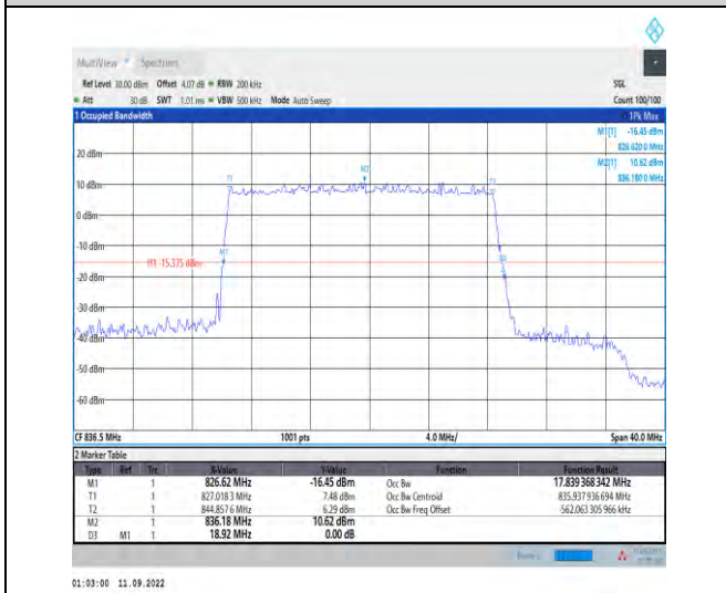
1-N5--15-20-M-5-DFT-256QAM-Outer_Full-100@0-A Ant1-17.839-18.920-≤20-PASS
