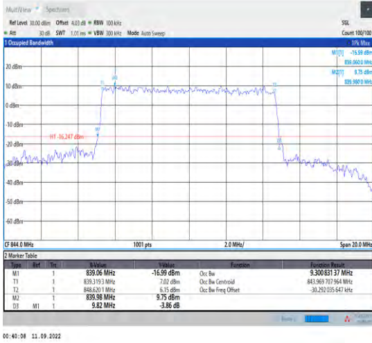
1-N5--15-10-H-8-CP-64QAM-Outer_Full-52@0-Ant1 -9.301-9.820-≤10-PASS
