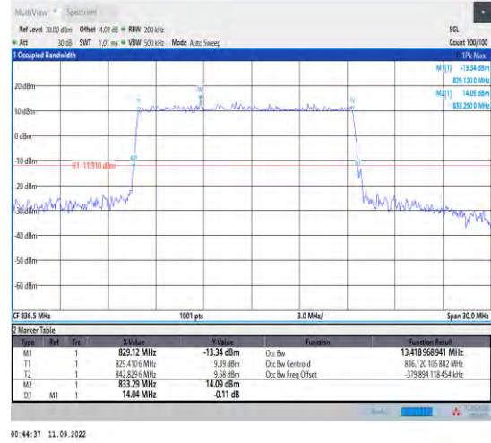
1-N5--15-15-M-3-DFT-16QAM-Outter_Full-75@0-Ant t1-13.419-14.040-≤15-PASS
