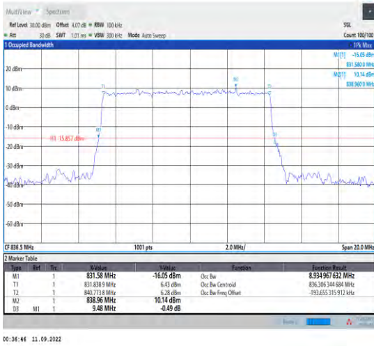
1-N5--15-10-M-5-DFT-256QAM-Outer_Full-50@0-A nt1-8.935-9.480-≤10-PASS
