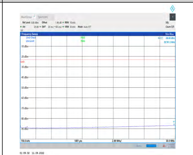
1-N5--15-20-H-1-DFT-PI2BPSK-Inner_1RB_Left-1@ 1-0.15-30-Ant1-29.76--86.64--23-PASS
