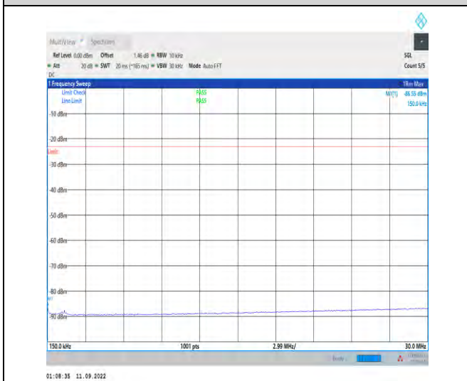
1-N5--15-20-M-1-DFT-PI2BPSK-Inner_1RB_Left-1@ 1-0.15-30-Ant1-0.15--86.55--23-PASS
