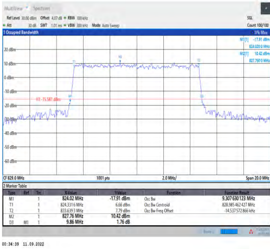
1-N5--15-10-L-6-CP-QPSK-Outer_Full-52@0-Ant1-9 308-9.860-≤10-PASS
