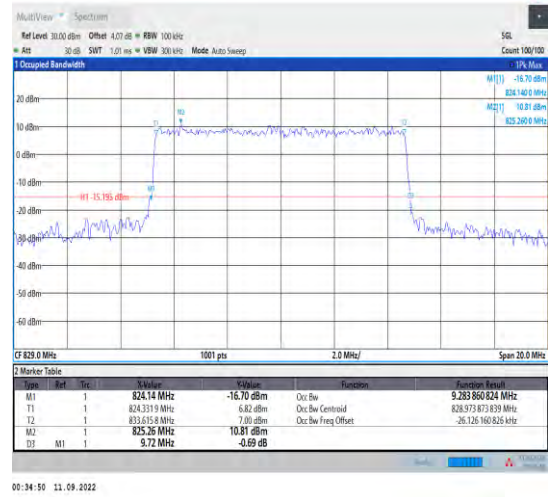
1-N5--15-10-L-7-CP-16QAM-Outer_Full-52@0-Ant1- 9.284-9.720-≤10-PASS
