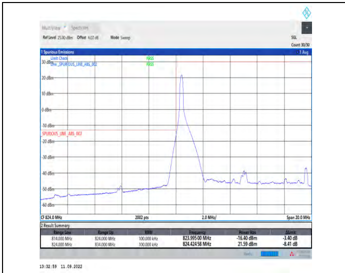
1-N5--15-10-L-1-DFT-PI2BPSK-Edge_1RB_Left-1@0-Ant1-1-seegraph-PASS-see graph
