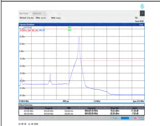
1-N5--15-10-H-5-CP-QPSK-Edge_1RB_Right-1@51-Ant1-1-seegraph-PASS-see graph
