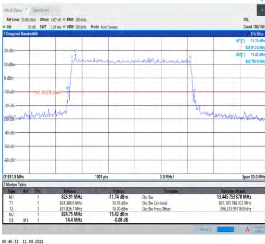
1-N5--15-15-L-1-DFT-QPSK-Outer_Full-75@0-Ant1- 13.446-14.400-≤15-PASS
