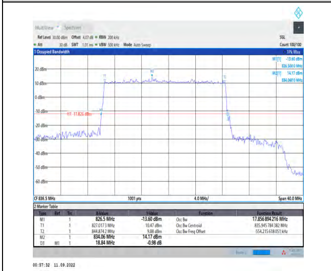
1-N5--15-20-M-1-DFT-QPSK-Outer_Full-100@0-Ant 1-17.857-18.840-≤20-PASS
