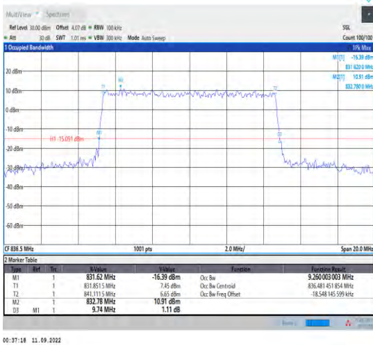
1-N5--15-10-M-7-CP-16QAM-Outer_Full-52@0-Ant1 -9.26-9.740-≤10-PASS
