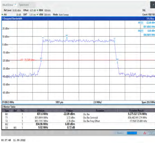
1-N5--15-10-M-9-CP-256QAM-Outer_Full-52@0-Ant 1-9.275-9.920-≤10-PASS
