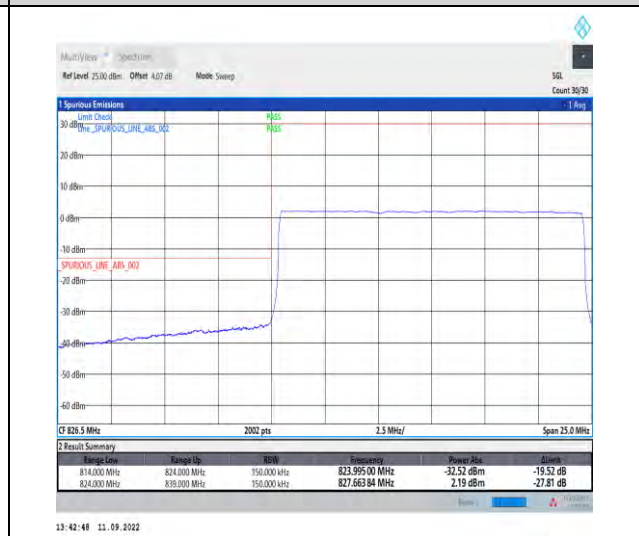
1-N5--15-15-L-6-CP-QPSK-Outer_Full-79@0-Ant1-1-seegraph-PASS-see graph
