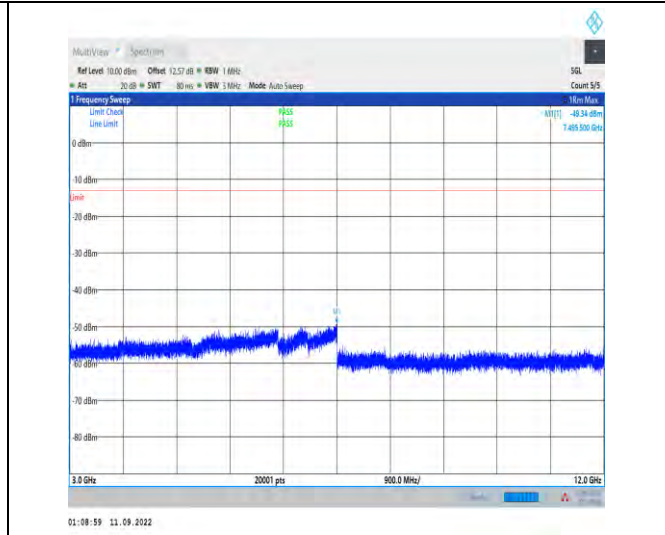
1-N5--15-20-M-1-DFT-PI2BPSK-Inner_1RB_Left-1@ 1-3000-12000-Ant1-7495.50--49.34--13-PASS
