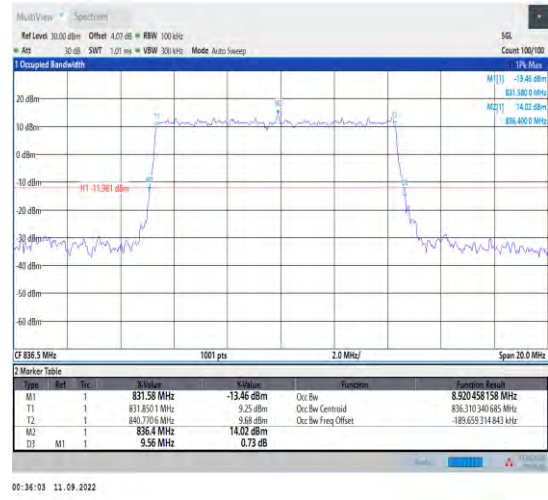
1-N5--15-10-M-2-DFT-PI2BPSK-Outer_Full-50@0-A nt1-8.92-9.560-≤10-PASS
