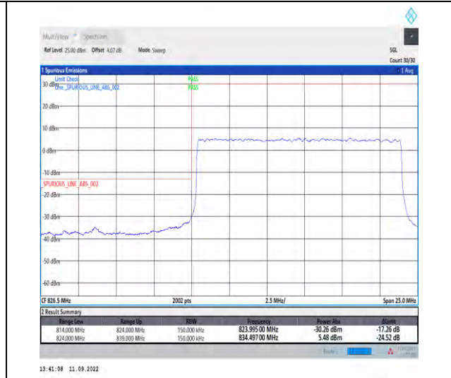
1-N5--15-15-L-3-DFT-PI2BPSK-Outer_Full-75@0-Ant1-1-seegraph-PASS-see graph
