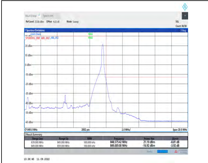
1-N5--15-10-H-2-DFT-PI2BPSK-Edge_1RB_Right-1@51-Ant1-1-seegraph-PASS-see graph
