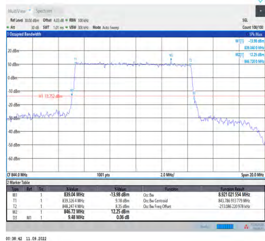
1-N5--15-10-H-3-DFT-16QAM-Outer_Full-50@0-Ant 1-8.921-9.480-≤10-PASS
