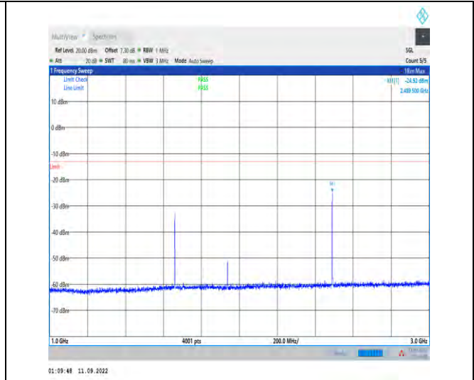
1-N5--15-20-H-1-DFT-PI2BPSK-Inner_1RB_Left-1@ 1-1000-3000-Ant1-2489.50--24.92--13-PASS
