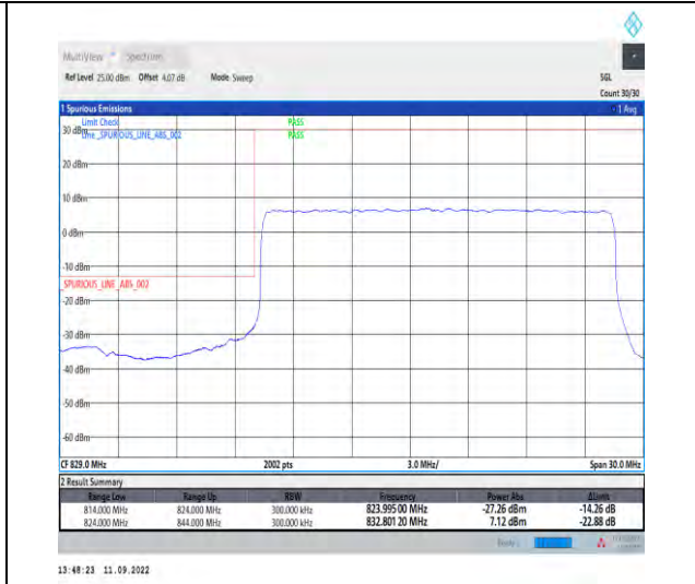
1-N5--15-20-L-3-DFT-PI2BPSK-Outer_Full-100@0-Ant1-1-seegraph-PASS-see graph
