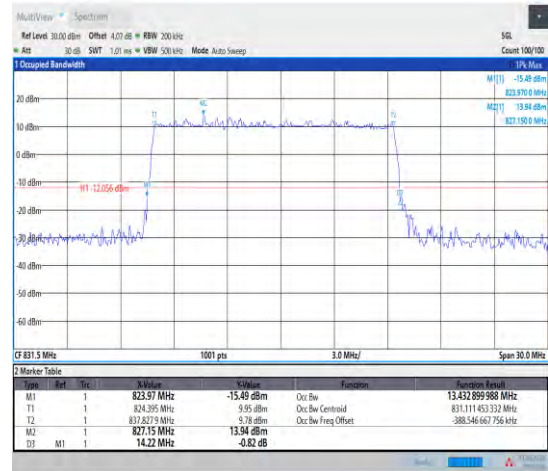
1-N5--15-15-L-4-DFT-64QAM-Outer_Full-75@0-Ant1 -13.433-14.220≤15-PASS
