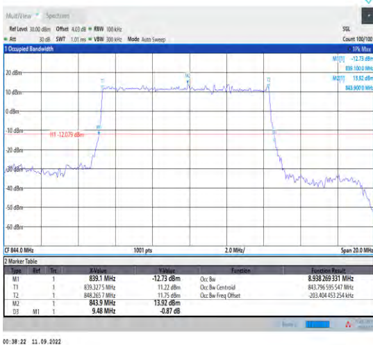
1-N5--15-10-H-2-DFT-PI2BPSK-Outer_Full-50@0-A nt1-8.938-9.480-≤10-PASS
