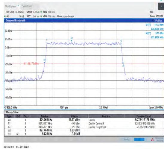
1-N5--15-10-L-9-CP-256QAM-Outer_Full-52@0-Ant1- -9.272-9.820-≤10-PASS
