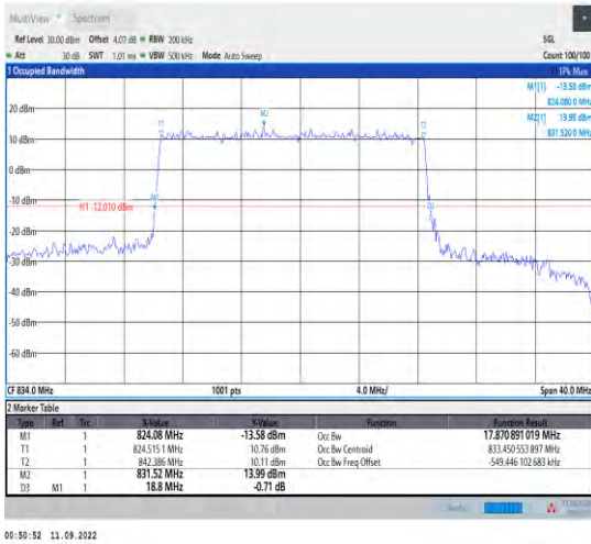
1-N5--15-20-L-4-DFT-64QAM-Outer_Full-100@0-An t1-39.601-40.000-<20-PASS
