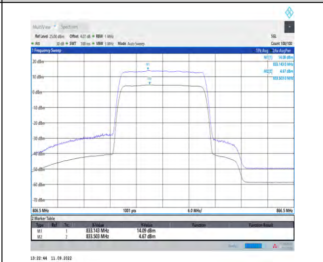
1-N5--15-20-M-2-CP-256QAM-Outer_Full-106@0-A nt1-9.42-100%-0.00-9.42-PASS-≤13
