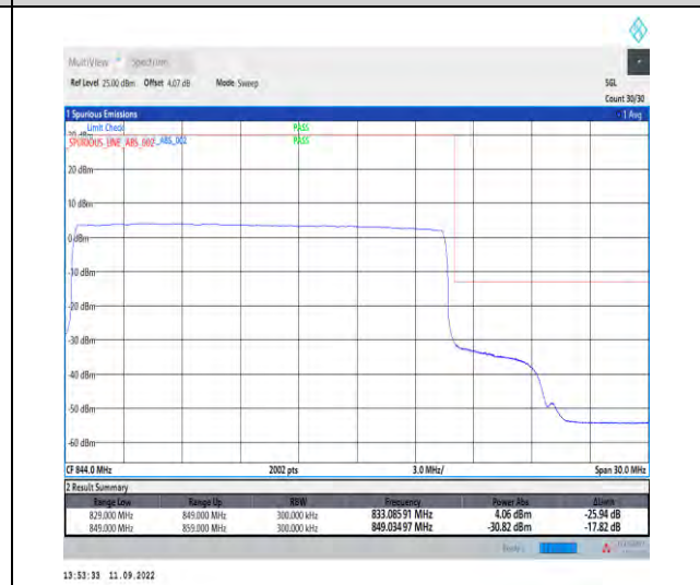
1-N5--15-20-H-6-CP-QPSK-Outer_Full-106@0-Ant1-1-seegraph-PASS-see graph
