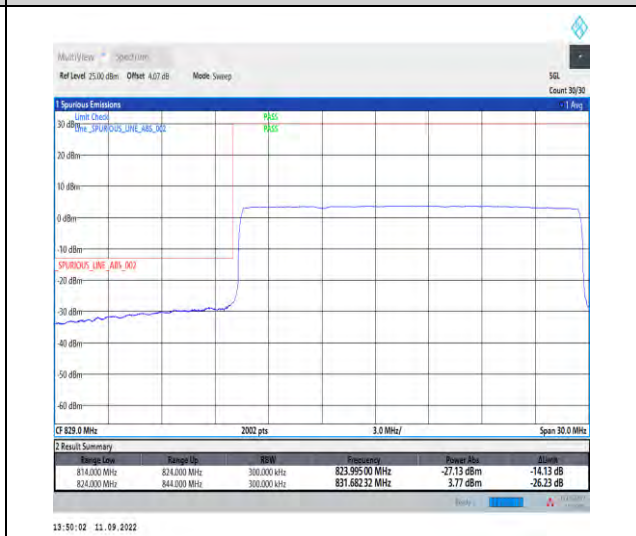
1-N5--15-20-L-6-CP-QPSK-Outer_Full-106@0-Ant1-1-seegraph-PASS-see graph
