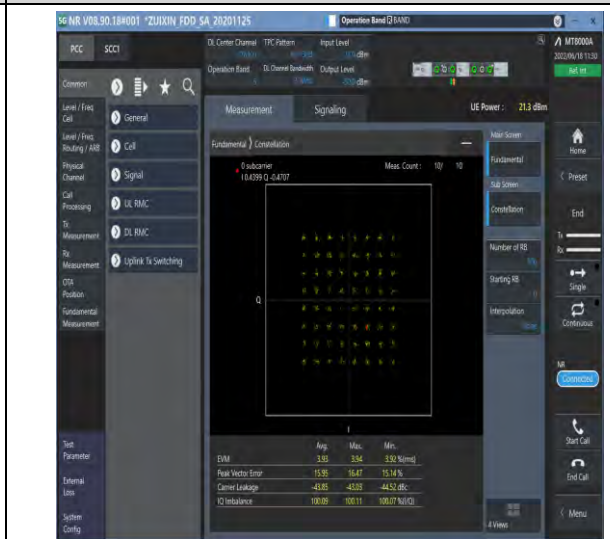
1-N5--15-20-M-8-CP-64QAM-Outer_Full-106@0-Ant t1-see graph-PASS
