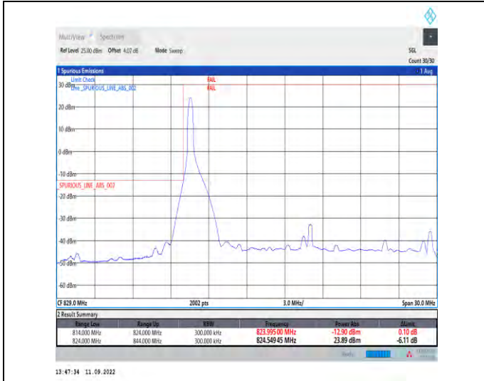
1-N5--15-20-L-1-DFT-PI2BPSK-Edge_1RB_Left-1@0-Ant1-1-seegraph-PASS-see graph
