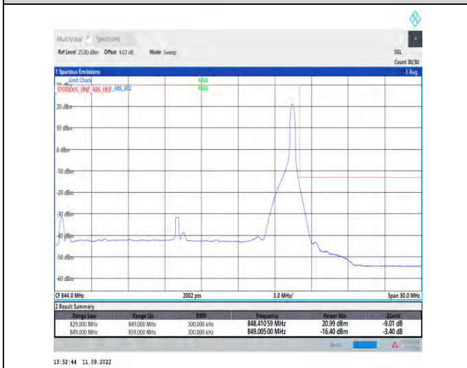
1-N5--15-20-H-5-CP-QPSK-Edge_1RB_Right-1@105-Ant1-1-seegraph-PASS-see graph
