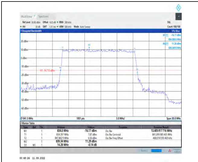
1-N5--15-15-H-5-DFT-256QAM-Outer_Full-75@0-An t1-13.406-14.280≤15-PASS
