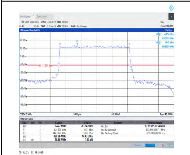
1-N5--15-20-L-2-DFT-PI2BPSK-Outer_Full-100@0-A nt1-17.894-18.680-≤20-PASS
