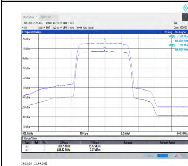
1-N5--15-20-M-1-DFT-256QAM-Outer_Full-100@0-A nt1-8.55-100%-0.00-8.55-PASS-≤13
