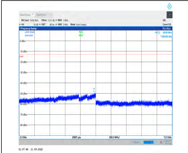
1-N5--15-20-L-1-DFT-PI2BPSK-Inner_1RB_Left-1@ 1-3000-12000-Ant1-7406.85--48.96--13-PASS
