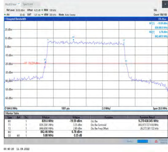
1-N5--15-10-H-9-CP-256QAM-Outer_Full-52@0-Ant 1-9.27-9.880-≤10-PASS
