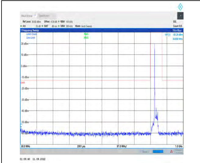
1-N5--15-20-H-1-DFT-PI2BPSK-Inner_1RB_Left-1@ 1-30-1000-Ant1-34.85--55.29--13-PASS
