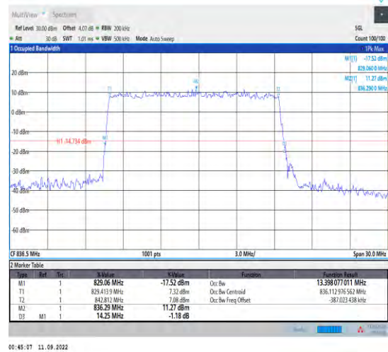
1-N5--15-15-M-5-DFT-256QAM-Outter_Full-75@0-Ant t1-13.398-14.250-≤15-PASS
