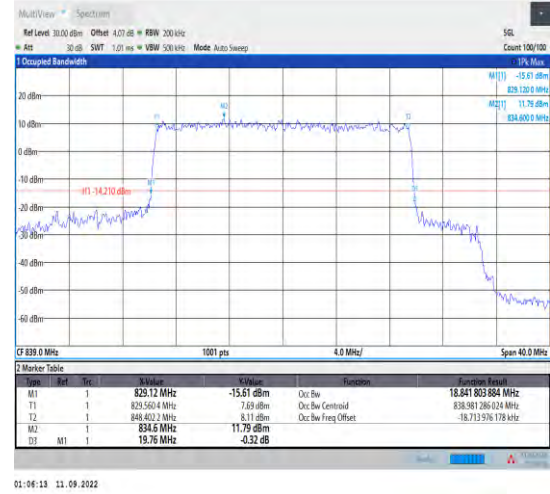
1-N5--15-20-H-7-CP-16QAM-Outer_Full-106@0-Ant 1-18.842-19.760-≤20-PASS
