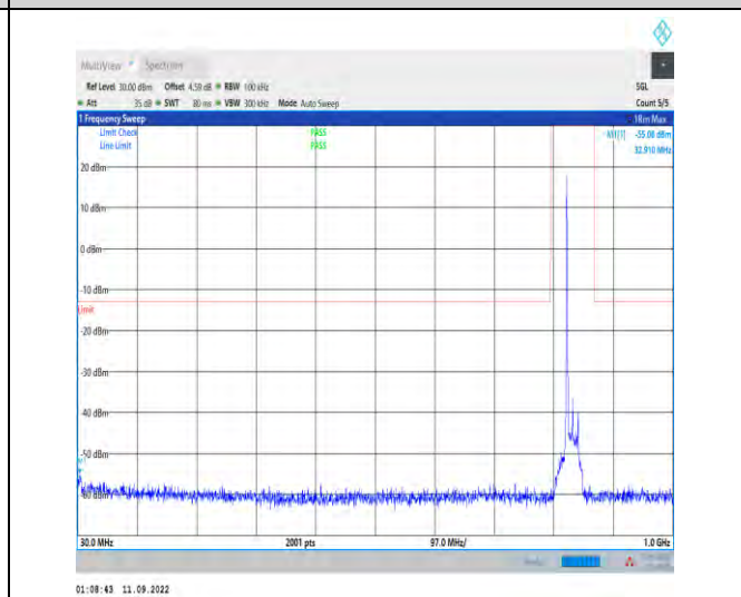
1-N5--15-20-M-1-DFT-PI2BPSK-Inner_1RB_Left-1@ 1-30-1000-Ant1-32.91--55.08--13-PASS
