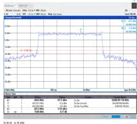
1-N5--15-20-L-7-CP-16QAM-Outer_Full-106@0-Ant1 -18.899-19.960-<20-PASS
