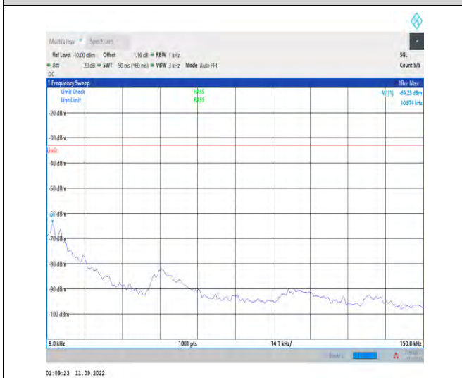
1-N5--15-20-H-1-DFT-PI2BPSK-Inner_1RB_Left-1@ 1-0.009-0.15-Ant1-0.01--64.23--33-PASS
