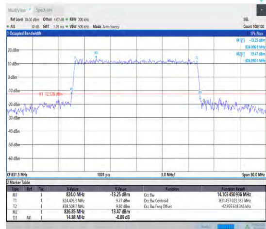
1-N5--15-15-L-6-CP-QPSK-Outer_Full-79@0-Ant1-1 4.103-14.880≤15-PASS
