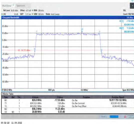
1-N5--15-20-L-6-CP-QPSK-Outer_Full-106@0-Ant1- 18.918-20.080-<20-PASS
