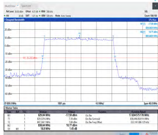
1-N5--15-20-H-5-DFT-256QAM-Outer_Full-100@0-A nt1-17.835-18.800-<20-PASS
