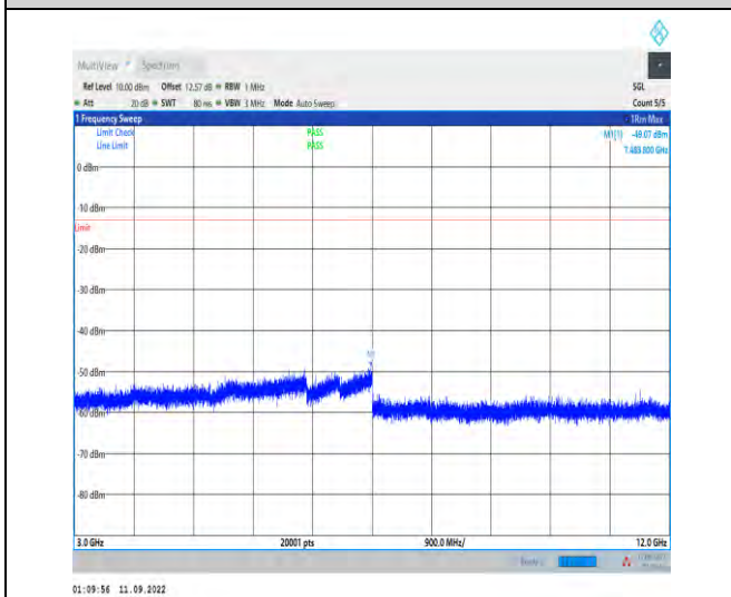
1-N5--15-20-H-1-DFT-PI2BPSK-Inner_1RB_Left-1@ 1-3000-12000-Ant1-7483.80--49.07--13-PASS
