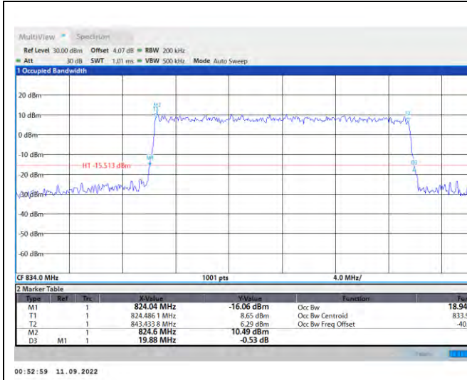
1-N5--15-20-L-8-CP-64QAM-Outer_Full-106@0-Ant 1-18.948-19.880-≤20-PASS
