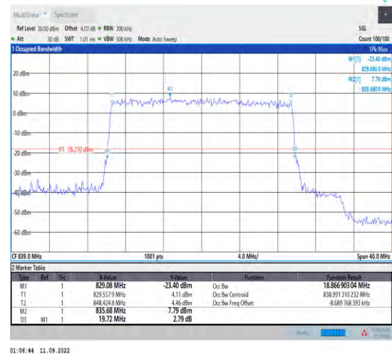
1-N5--15-20-H-9-CP-256QAM-Outer_Full-106@0-Ant t1-18.867-19.720-≤20-PASS
