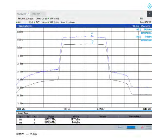
1-N5--15-20-L-2-CP-256QAM-Outer_Full-106@0-An t1-9.31-100%-0.00-9.31-PASS-≤13
