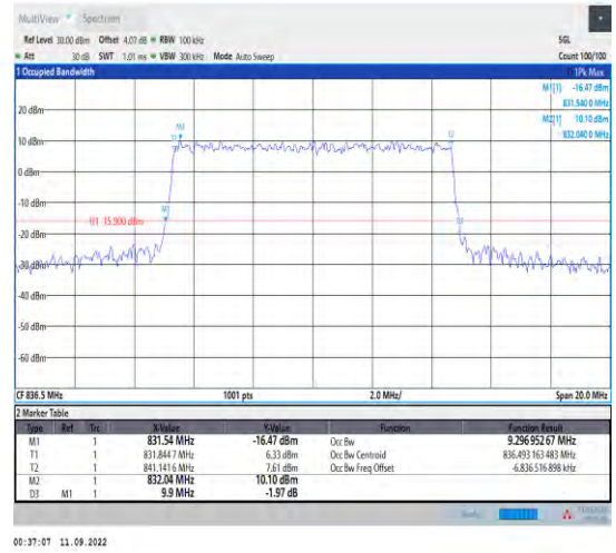
1-N5--15-10-M-6-CP-QPSK-Outer_Full-52@0-Ant1-9 .297-9.900-≤10-PASS
