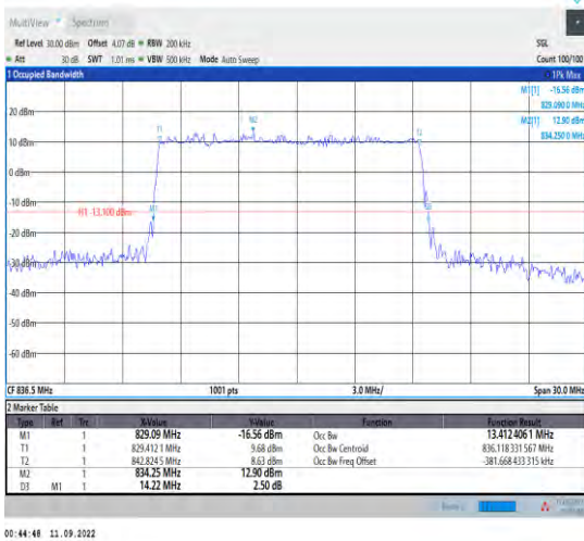
1-N5--15-15-M-4-DFT-64QAM-Outter_Full-75@0-Ant t1-13.412-14.220-≤15-PASS
