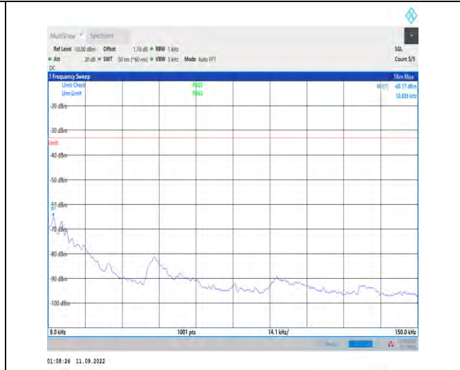
1-N5--15-20-M-1-DFT-PI2BPSK-Inner_1RB_Left-1@ 1-0.009-0.15-Ant1-0.01--65.17--33-PASS
