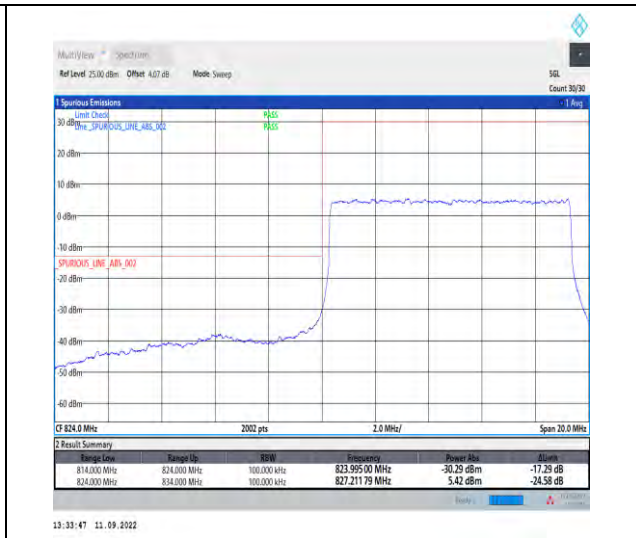
1-N5--15-10-L-3-DFT-PI2BPSK-Outer_Full-50@0-Ant1-1-seegraph-PASS-see graph
