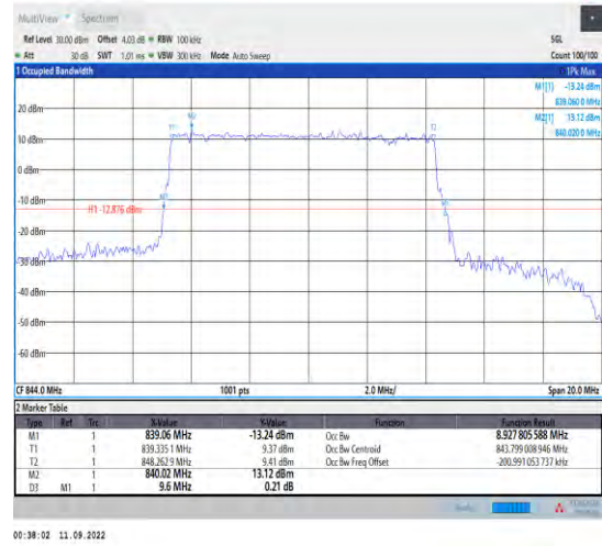
1-N5--15-10-H-1-DFT-QPSK-Outer_Full-50@0-Ant1 8.928-9.600-≤10-PASS
