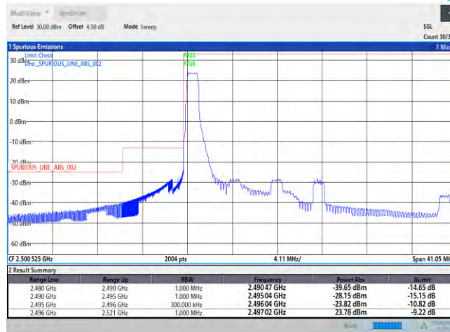
41-41-10MHz-15MHz-QPSK-QPSK-39703-39823-50RB#0-75RB#0
