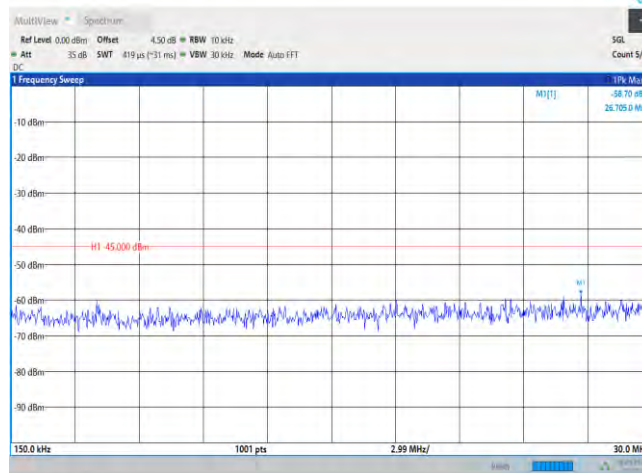
41-41-20MHz-20MHz-QPSK-QPSK-39750-39948-1RB#0-0RB#0-0.15~30MHz
