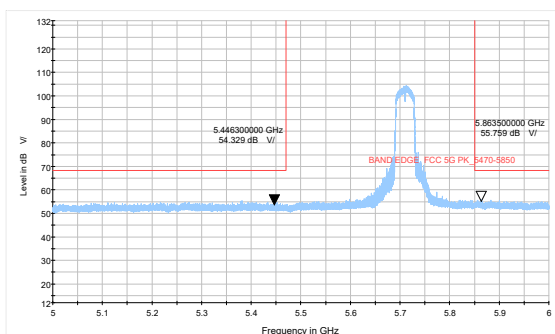
802.11ac VHT40-Channel 142: Peak
