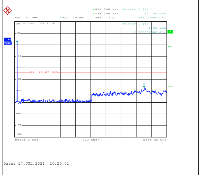
Conducted Spurious Emission Plot on Bluetooth LE 2Mbps GFSK Channel 19
