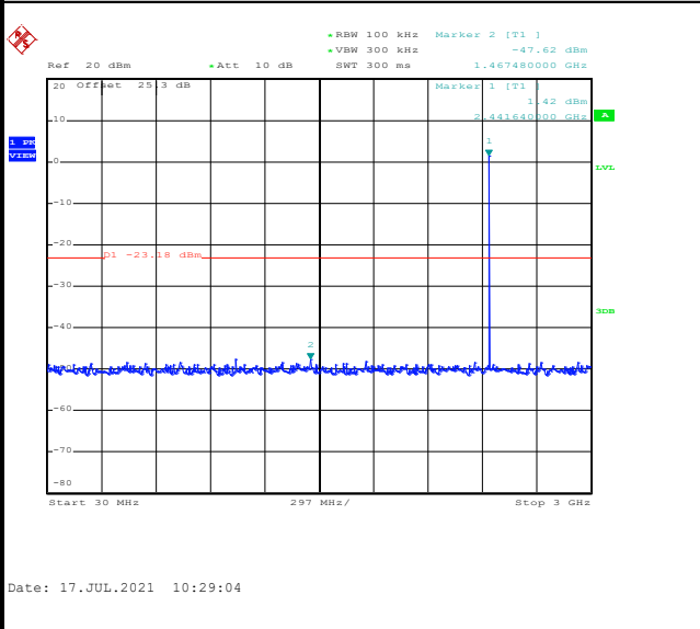
Conducted Spurious Emission Plot on Bluetooth LE 2Mbps GFSK Channel 19
