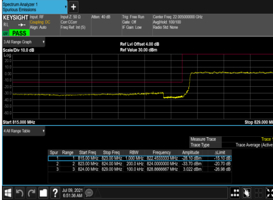
N5(20M)_DFT-s-OFDM_BPSK_Outer_Full_Low_CH
