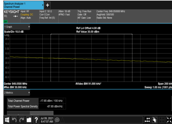
N5(10M)_DFT-s-OFDM_QPSK_Edge_1RB_Right_High_CH_CHP_ASS
