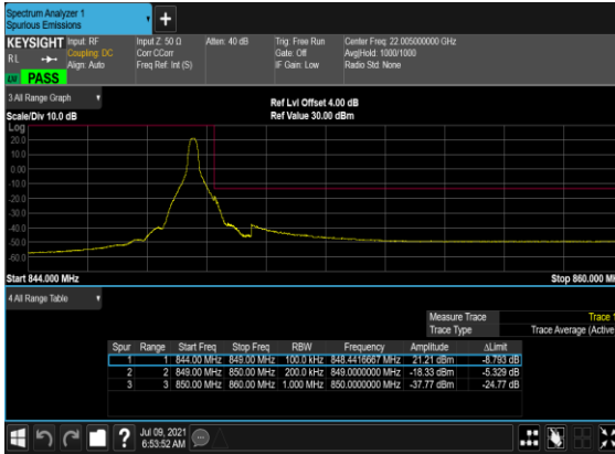
N5(20M)_DFT-s-OFDM_BPSK_Edge_1RB_Right_High_CH
