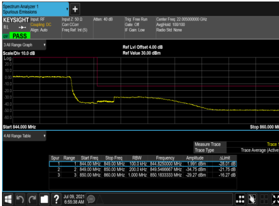
N5(20M)_DFT-s-OFDM_BPSK_Outer_Full_High_CH
