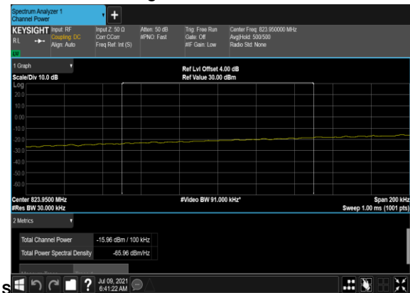
N5(10M)_DFT-s-OFDM_BPSK_Edge_1RB_Left_Low_CH_CHP_PAS
