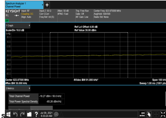
N5(5M)_DFT-s- OFDM_QPSK_Edge_1RB_Left_Low_CH_CHP_PAS
