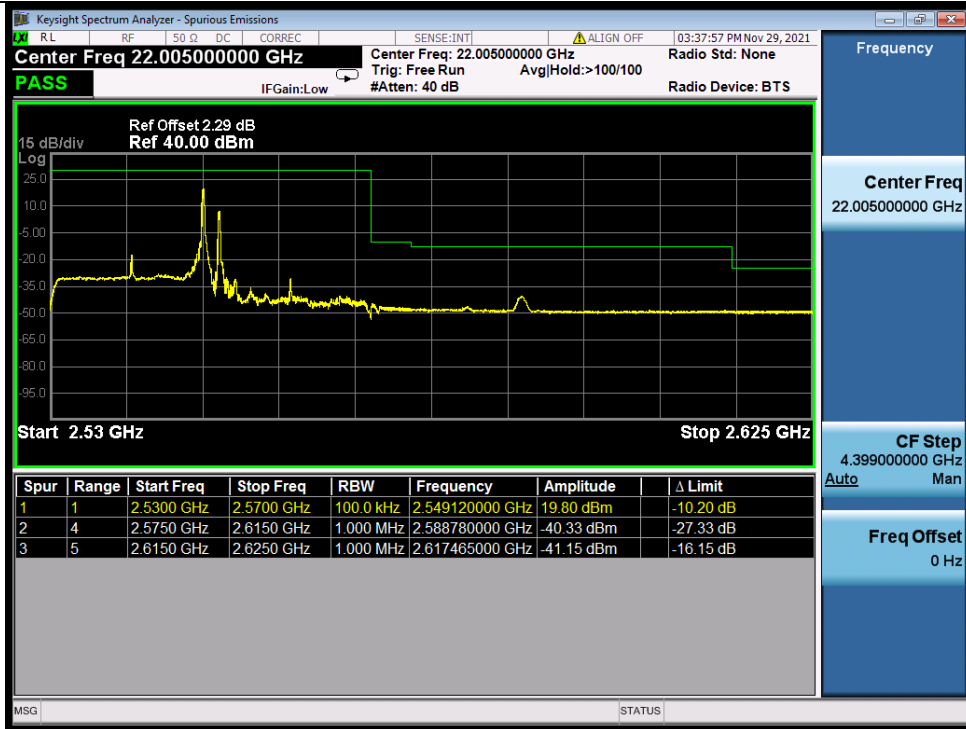
Band_7C_16QAM_HCH_20M+20M_RB_FULL_0_NTNV
