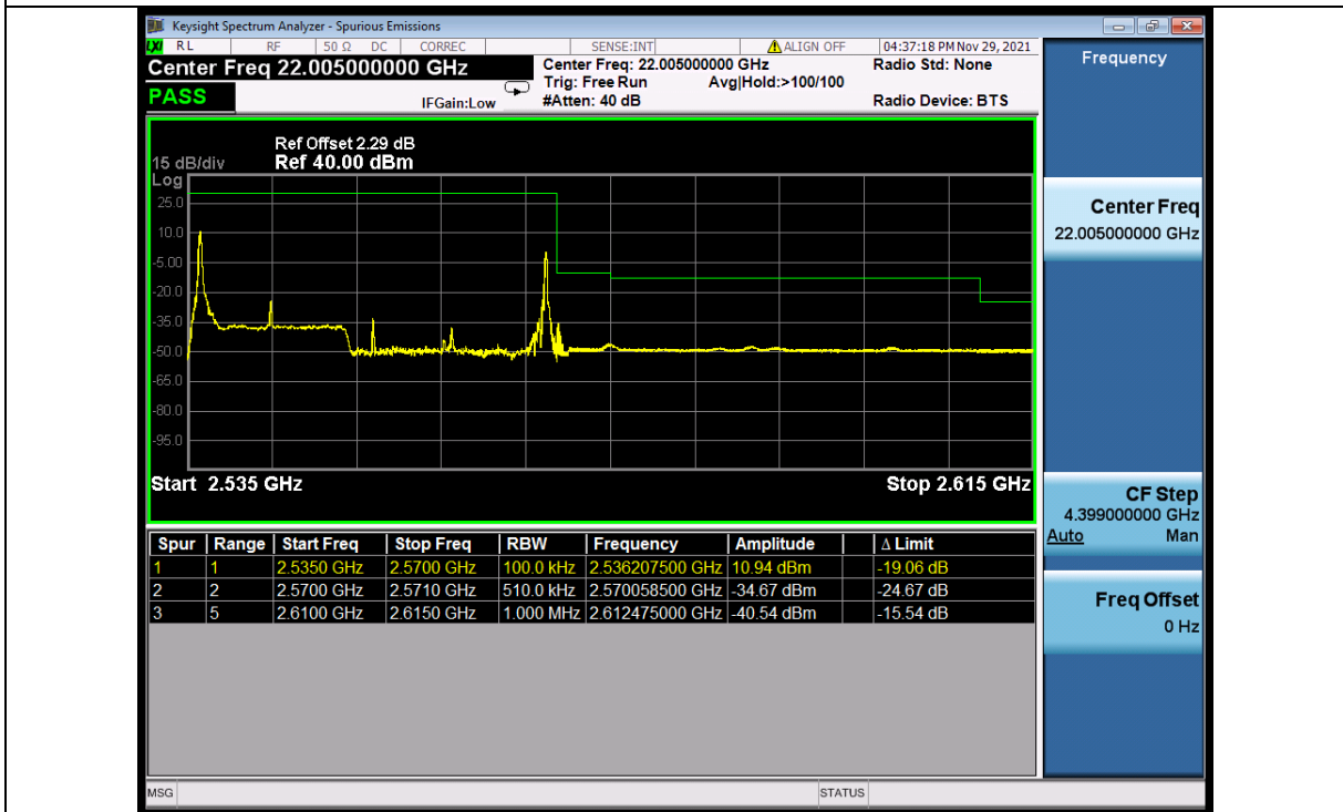
Band_7C_QPSK_HCH_15M+20M_RB_1_74/1_0_NTNV
