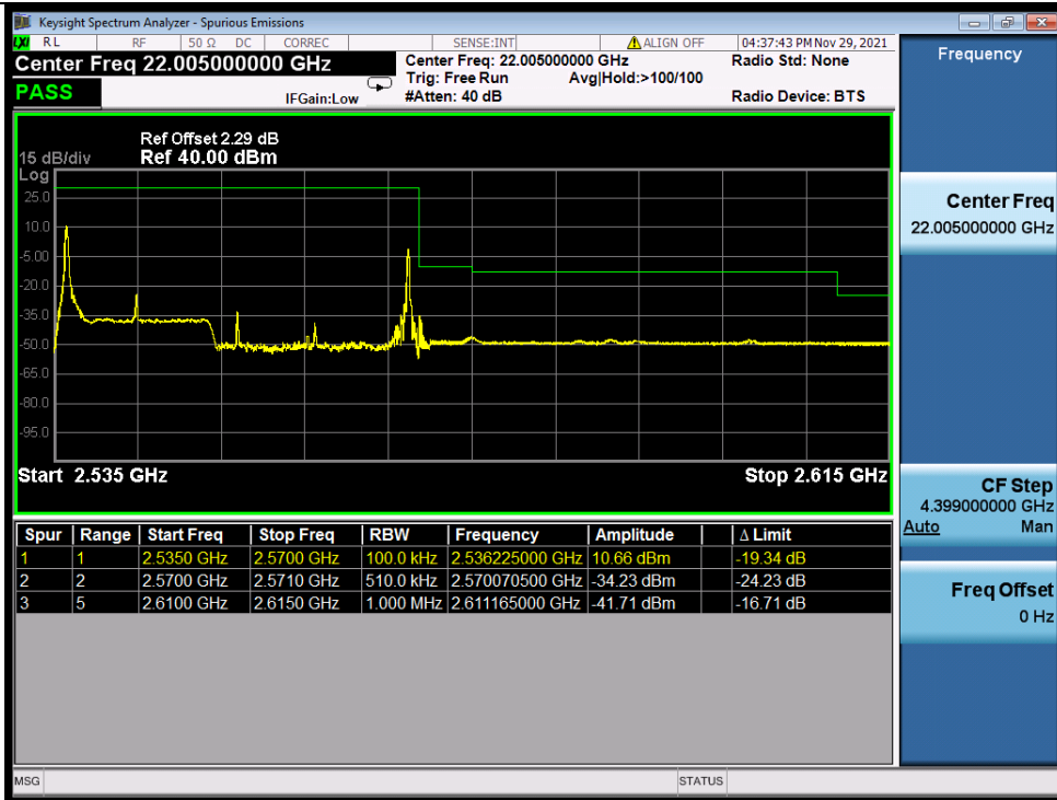
Band_7C_16QAM_HCH_15M+20M_RB_1_74/1_0_NTNV
