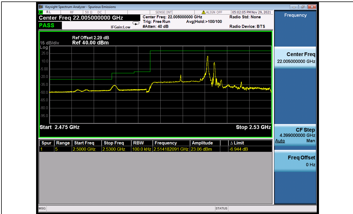
Band_7C_64QAM_LCH_15M+15M_RB_FULL_0_NTNV
