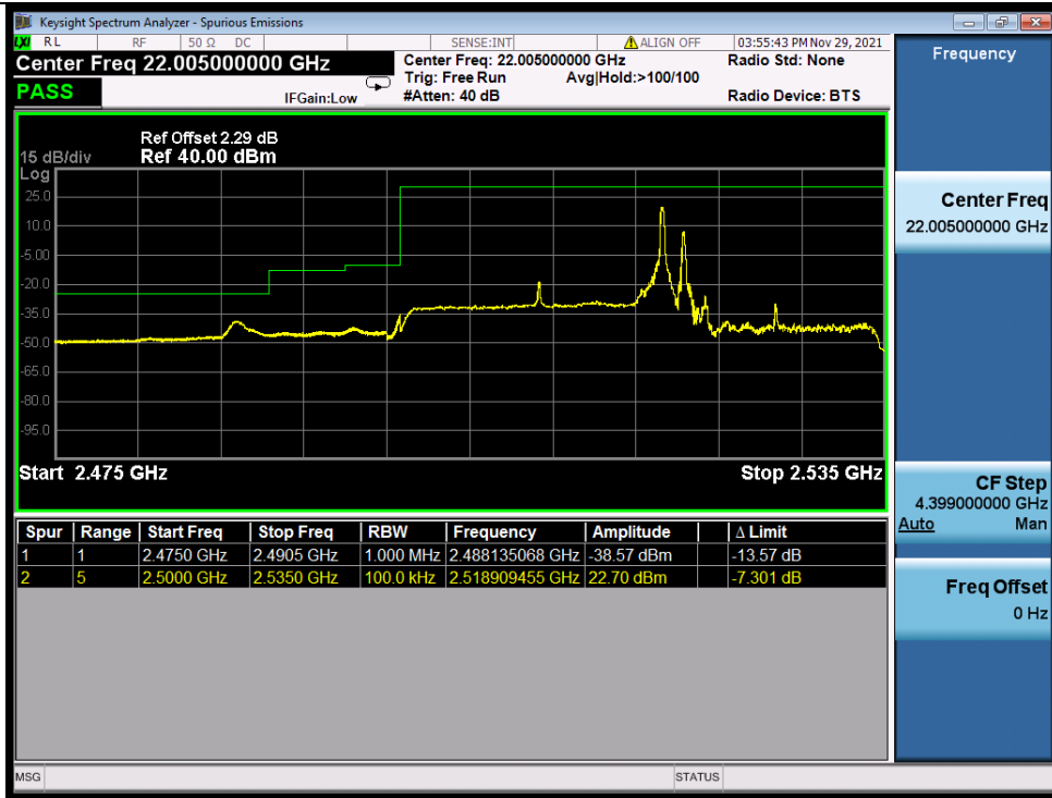
Band_7C_64QAM_LCH_20M+15M_RB_FULL_0_NTNV
