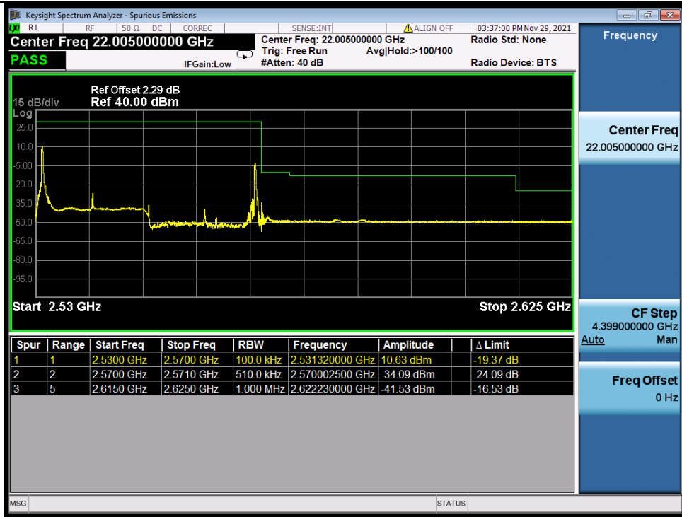
Band_7C_64QAM_HCH_20M+20M_RB_1_99/1_0_NTNV
