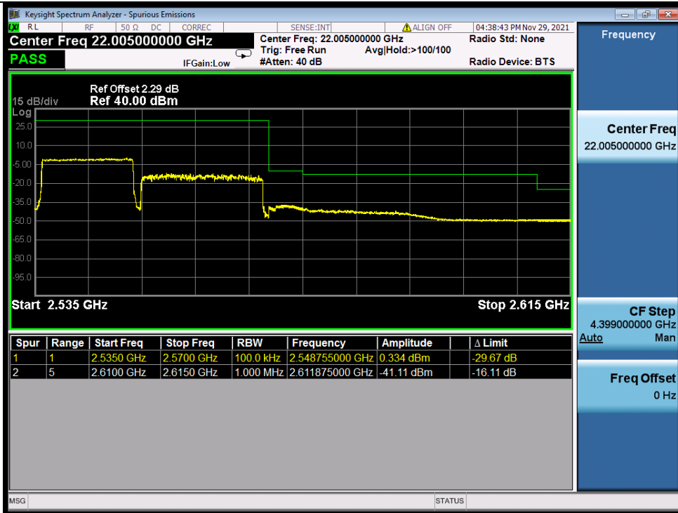
Band_7C_64QAM_LCH_15M+20M_RB_1_0/1_99_NTNV
