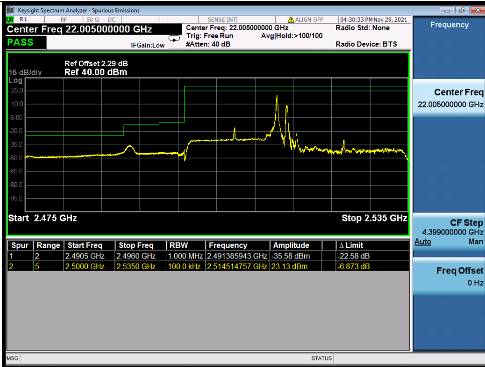
Band_7C_16QAM_LCH_15M+20M_RB_FULL_0_NTNV
