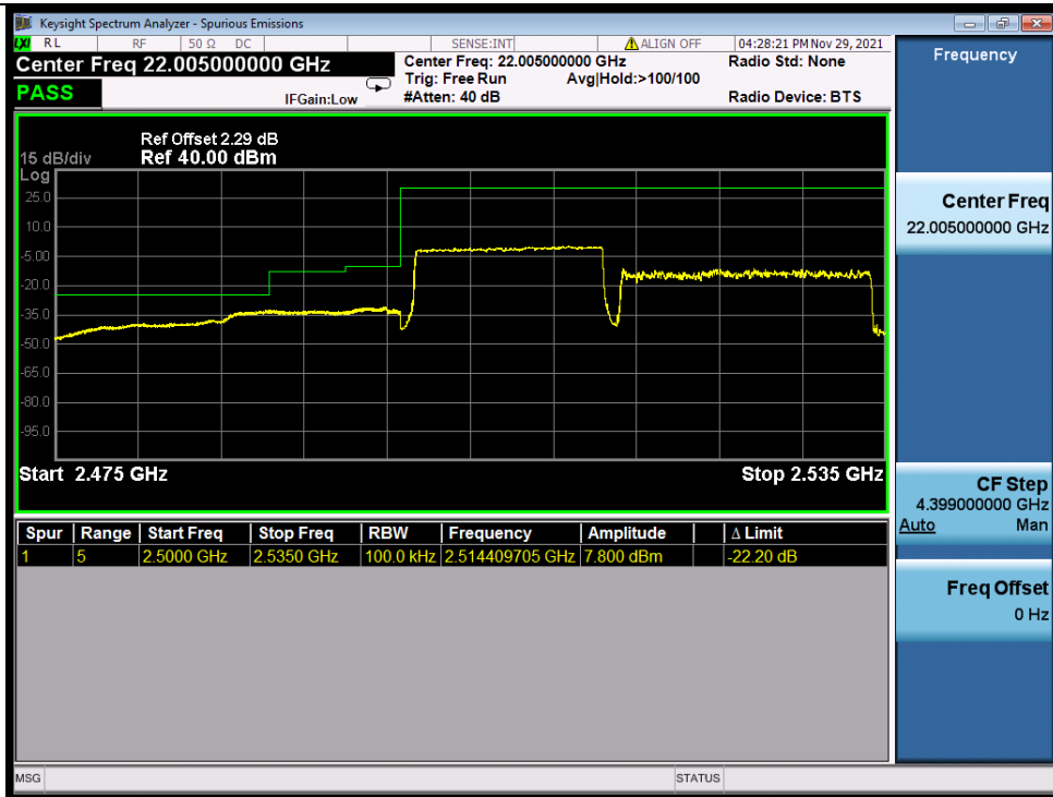
Band_7C_64QAM_HCH_15M+20M_RB_1_0/1_99_NTNV
