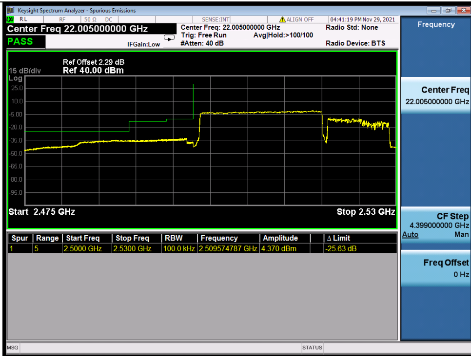
Band_7C_16QAM_HCH_20M+10M_RB_1_0/1_49_NTNV
