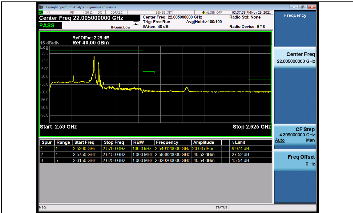
Band_7C_QPSK_HCH_20M+20M_RB_FULL_0_NTNV
