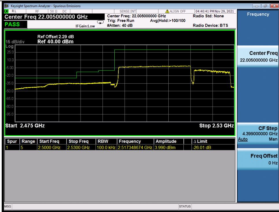
Band_7C_QPSK_LCH_20M+10M_NTNV
