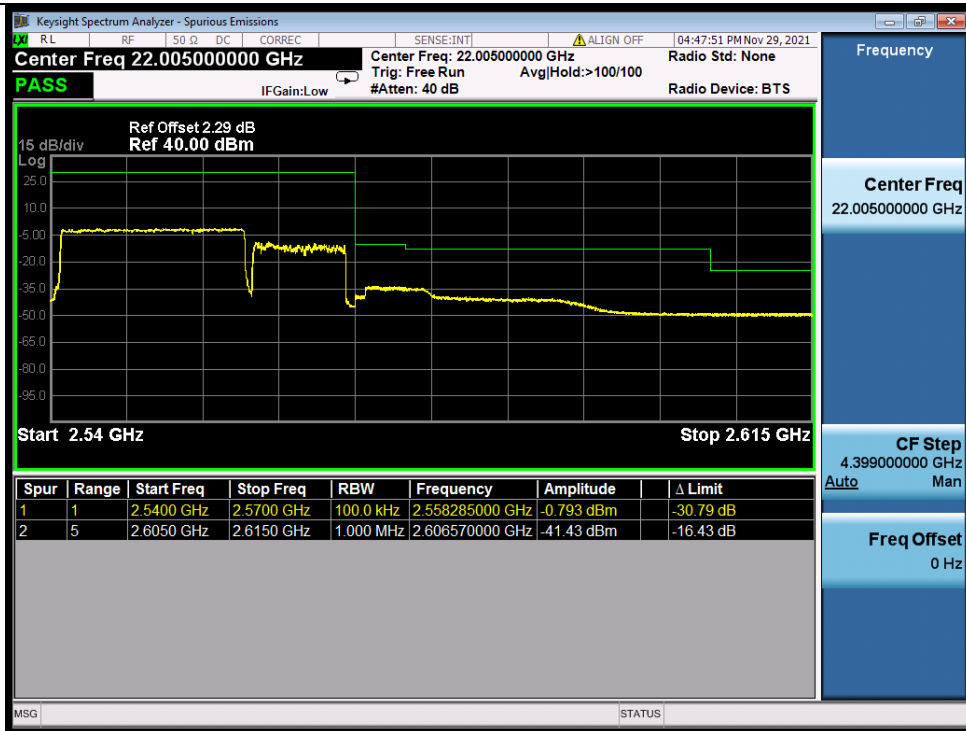
Band_7C_QPSK_HCH_20M+10M _NTNV
