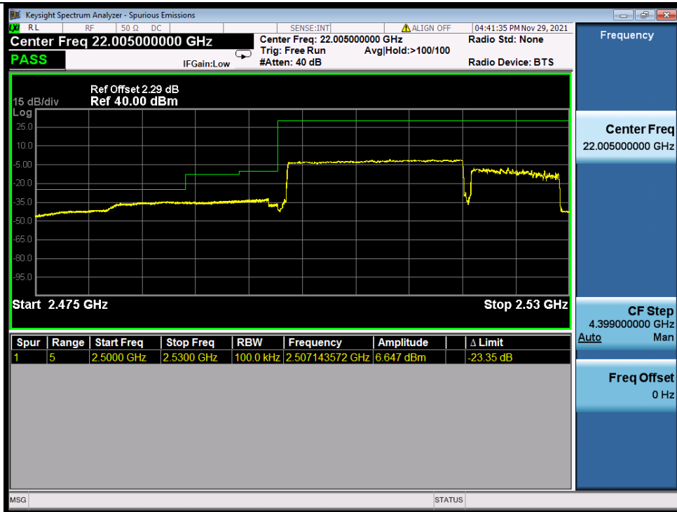
Band_7C_64QAM_HCH_20M+10M_RB_1_0/1_49_NTNV
