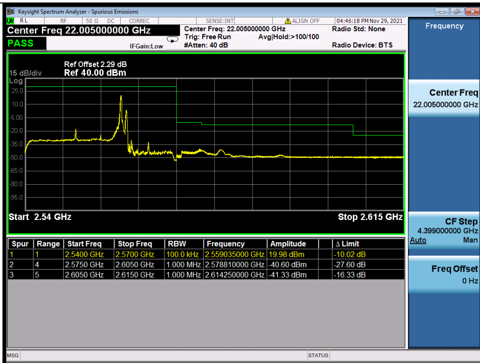
Band_7C_64QAM_HCH_20M+10M_RB_FULL_0_NTNV
