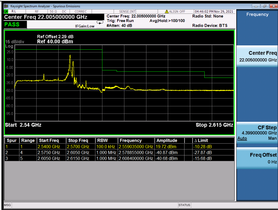
Band_7C_16QAM_HCH_20M+10M_RB_FULL_0_NTNV
