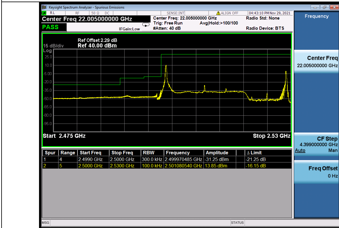
Band_7C_64QAM_LCH_20M+10M_RB_1_99/1_0_NTNV
