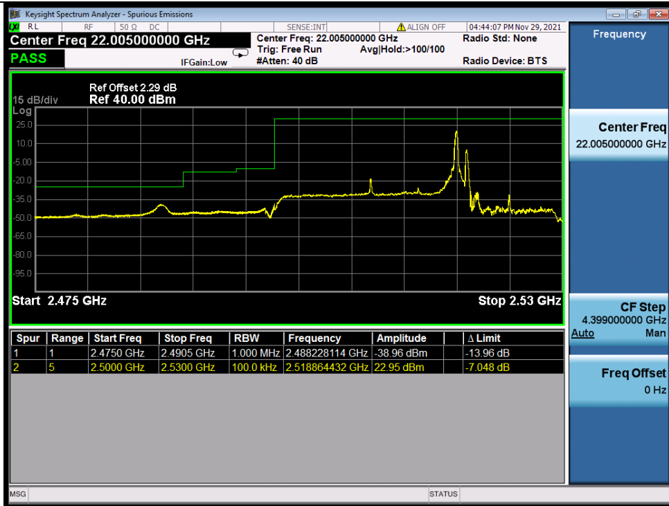
Band_7C_16QAM_LCH_20M+10M_RB_FULL_0_NTNV
