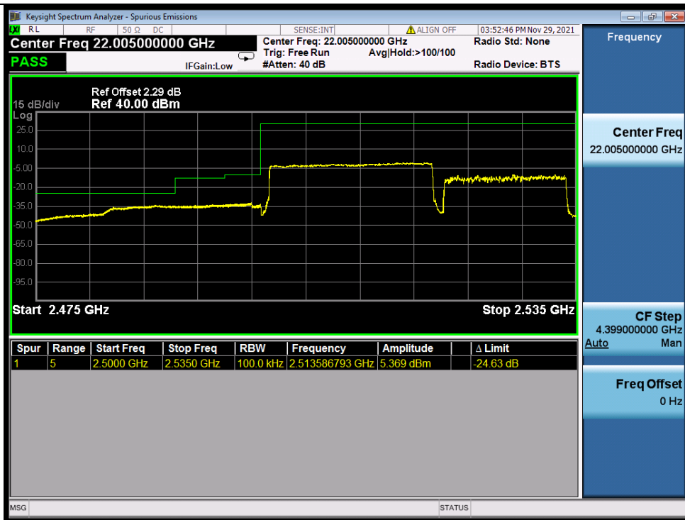
Band_7C_16QAM_HCH_20M+15M_RB_1_0/1_74_NTNV
