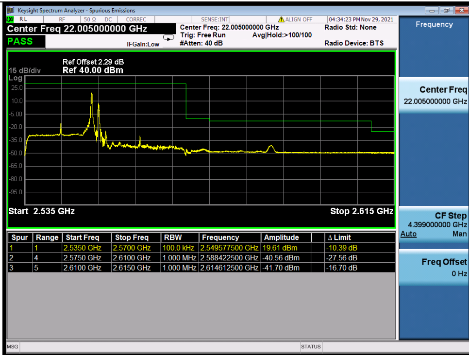
Band_7C_64QAM_HCH_15M+20M_RB_FULL_0_NTNV
