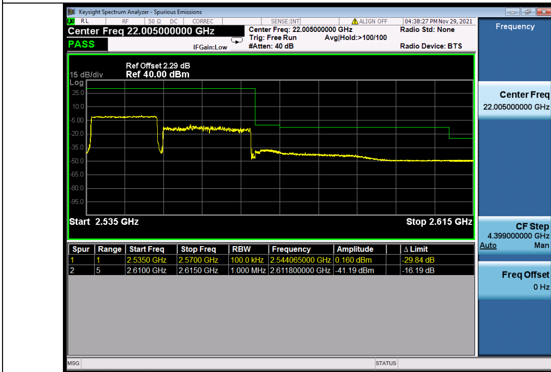
Band_7C_QPSK_HCH_15M+20M_NTNV
