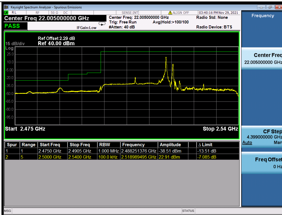
Band_7C_64QAM_LCH_20M+20M_RB_FULL_0_NTNV
