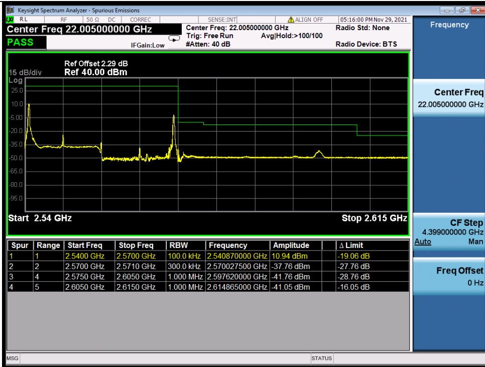
Band_7C_64QAM_HCH_15M+15M_RB_1_74/1_0_NTNV
