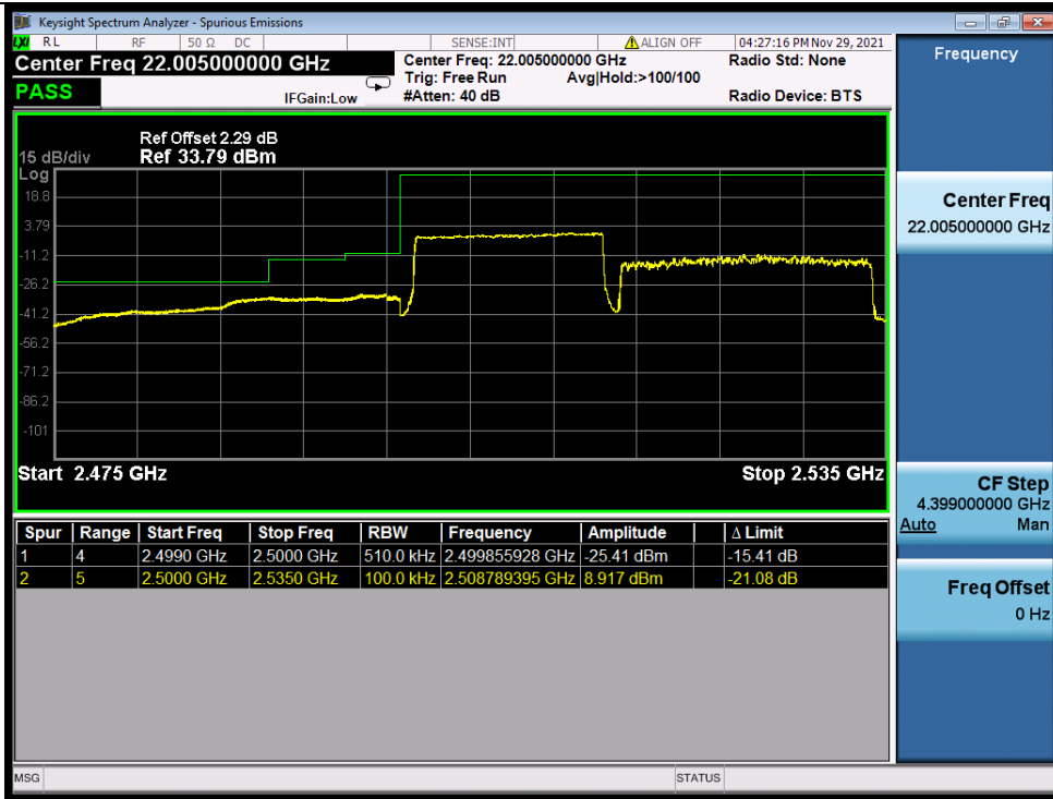
Band_7C_QPSK_LCH_15M+20M_NTNV
