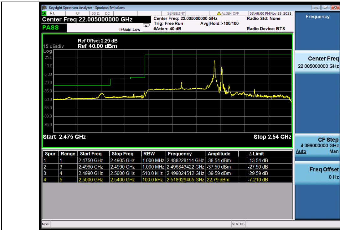
Band_7C_16QAM_LCH_20M+20M_RB_FULL_0_NTNV
