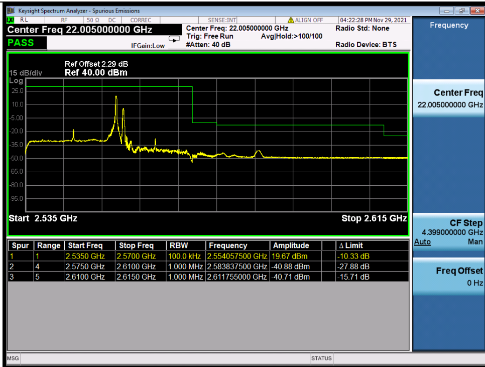
Band_7C_64QAM_HCH_20M+15M_RB_FULL_0_NTNV
