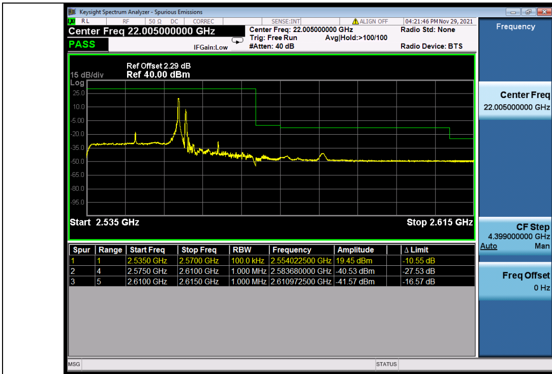
Band_7C_QPSK_HCH_20M+15M_RB_FULL_0_NTNV
