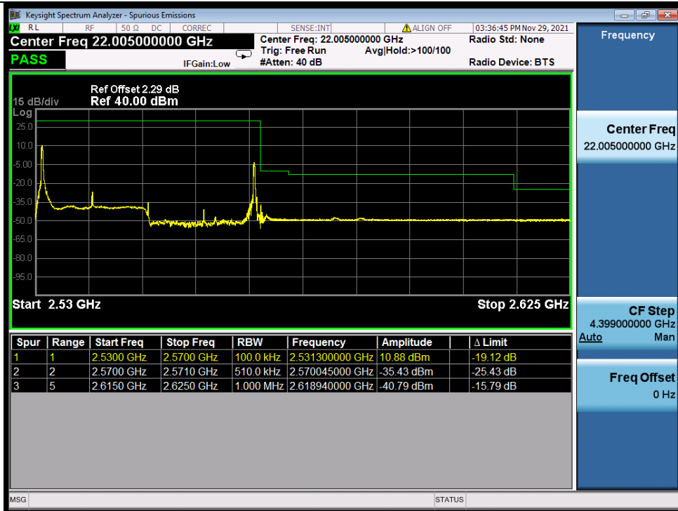
Band_7C_16QAM_HCH_20M+20M_RB_1_99/1_0_NTNV
