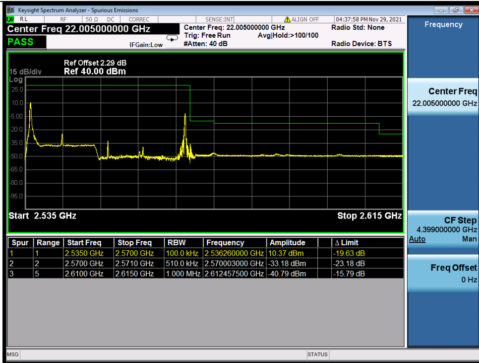
Band_7C_64QAM_HCH_15M+20M_RB_1_74/1_0_NTNV
