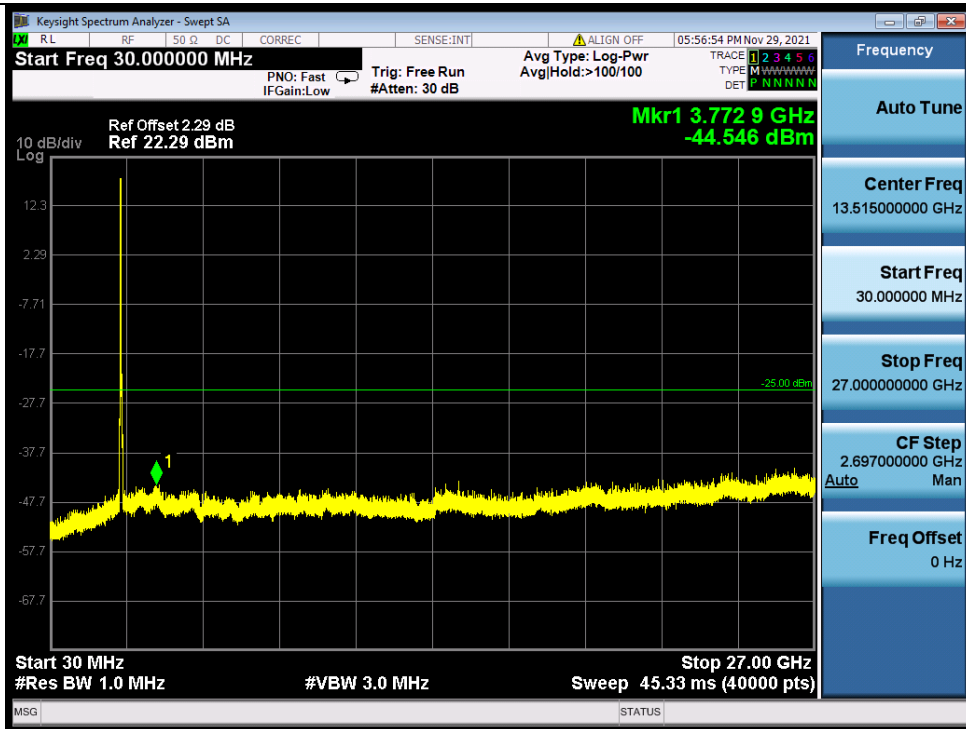
Band_7C_QPSK_MCH_20M+15M_NTNV
