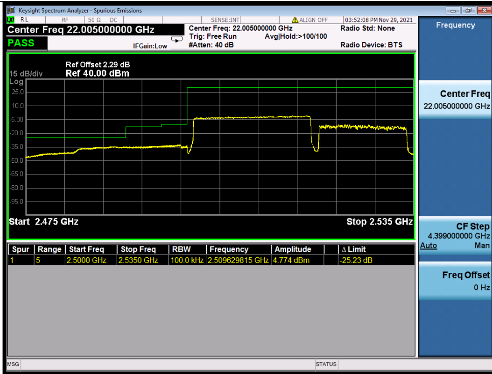
Band_7C_QPSK_LCH_20M+15M_NTNV
