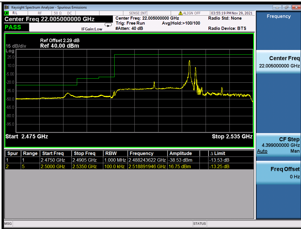
Band_7C_16QAM_LCH_20M+15M_RB_FULL_0_NTNV
