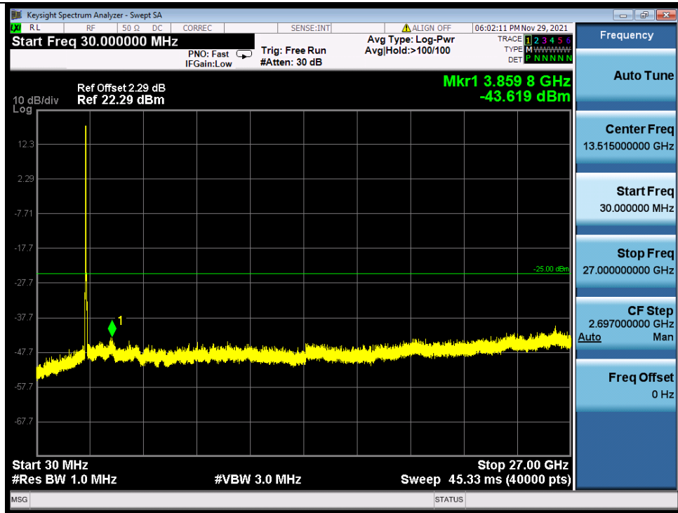
Band_7C_QPSK_MCH_15M+20M_NTNV
