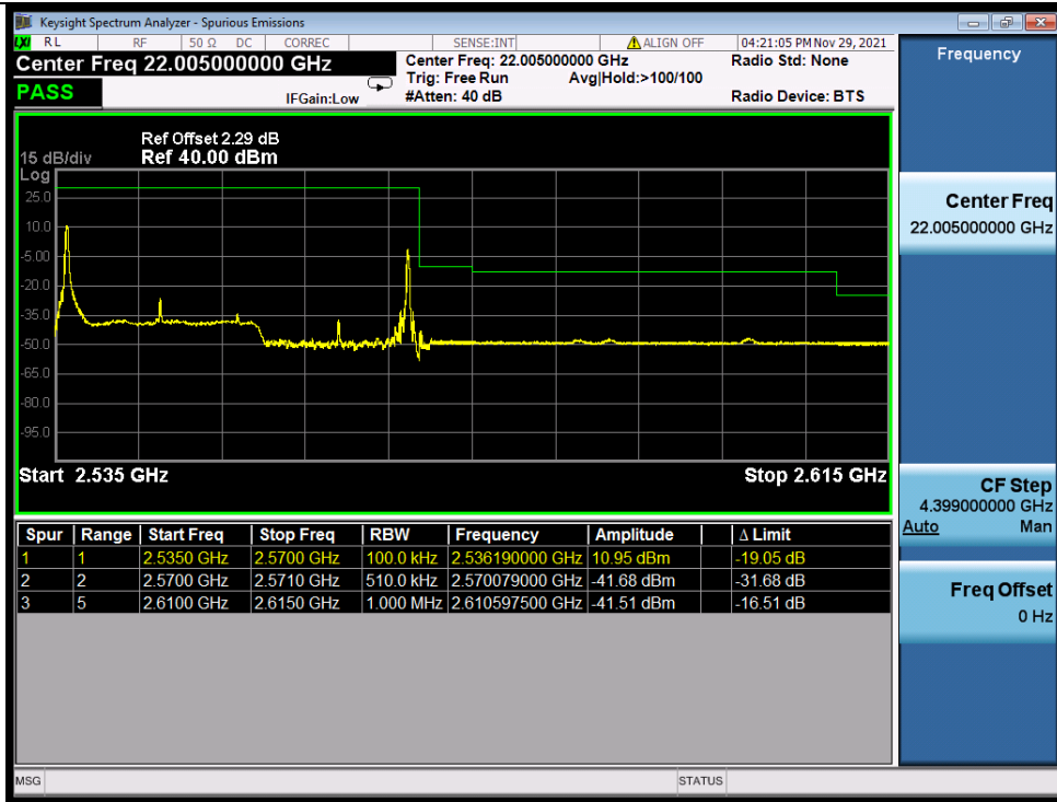
Band_7C_16QAM_HCH_20M+15M_RB_1_99/1_0_NTNV
