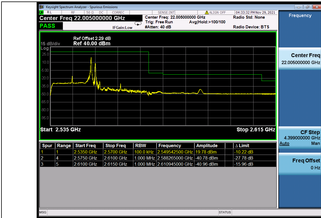
Band_7C_QPSK_HCH_15M+20M_RB_FULL_0_NTNV
