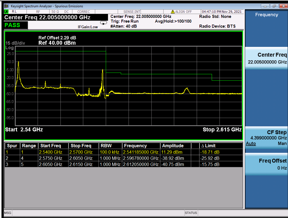
Band_7C_16QAM_HCH_20M+10M_RB_1_99/1_0_NTNV
