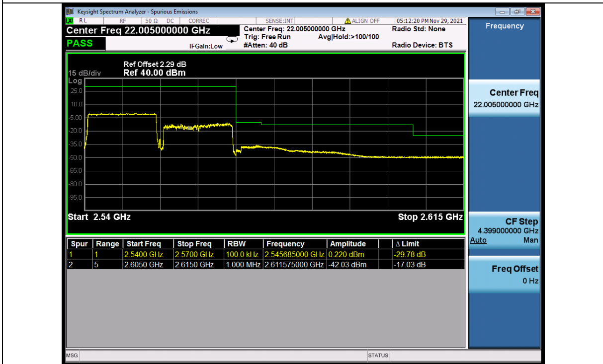
Band_7C_64QAM_HCH_15M+15M_RB_1_0/1_74_NTNV
