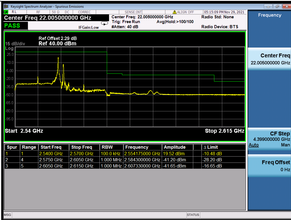
Band_7C_64QAM_HCH_15M+15M_RB_FULL_0_NTNV
