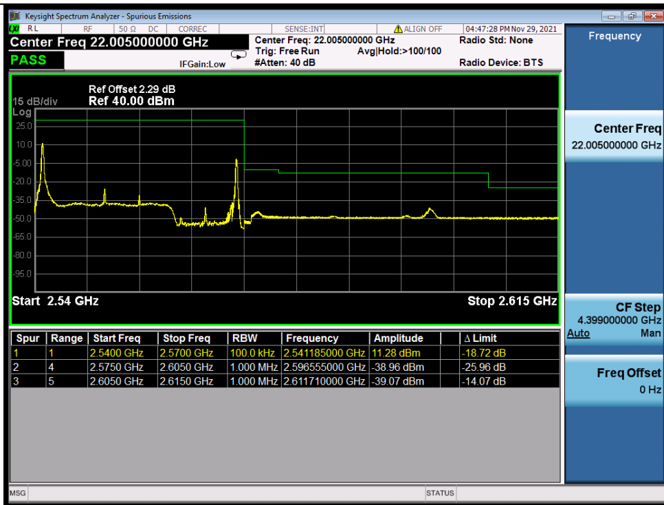
Band_7C_64QAM_HCH_20M+10M_RB_1_99/1_0_NTNV
