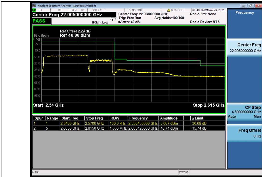
Band_7C_64QAM_LCH_20M+10M_RB_1_0/1_49_NTNV
