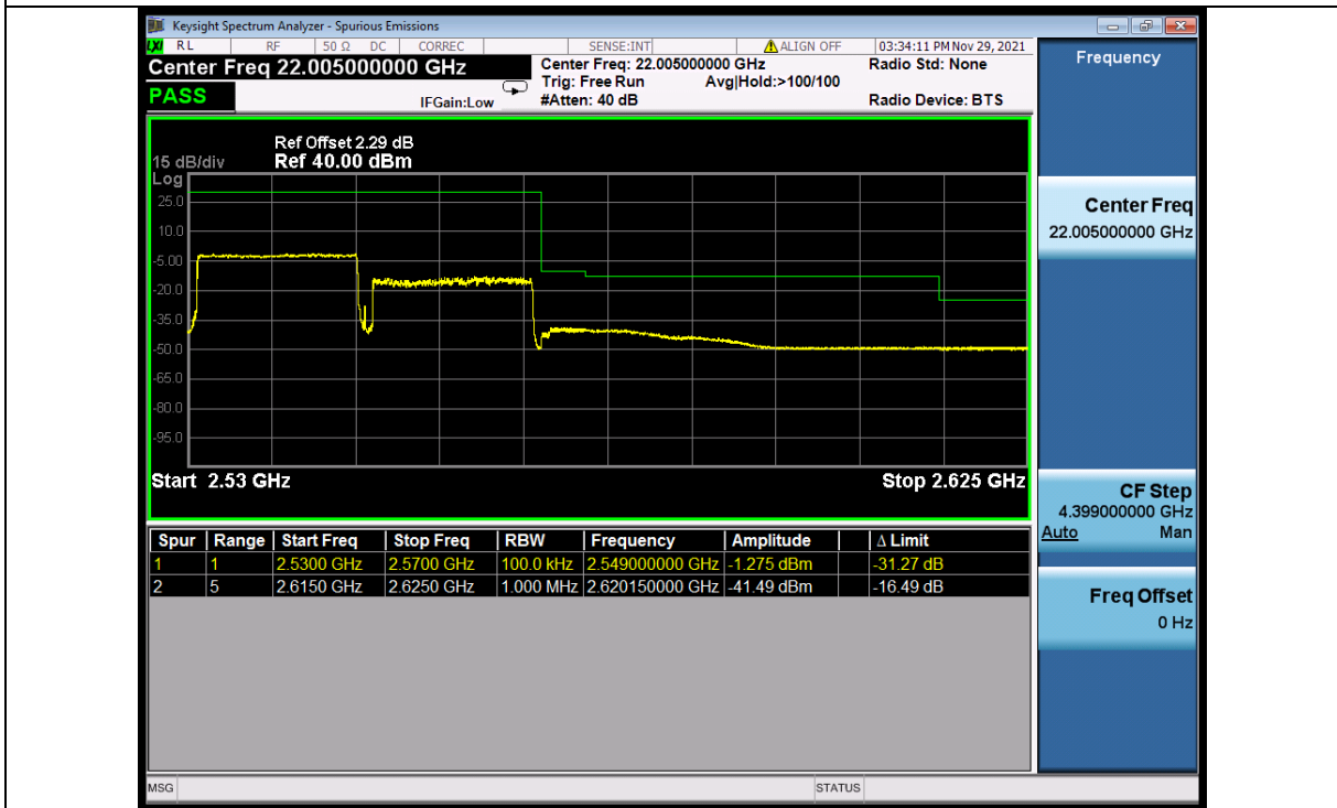
Band_7C_QPSK_HCH_20M+20M_NTNV
