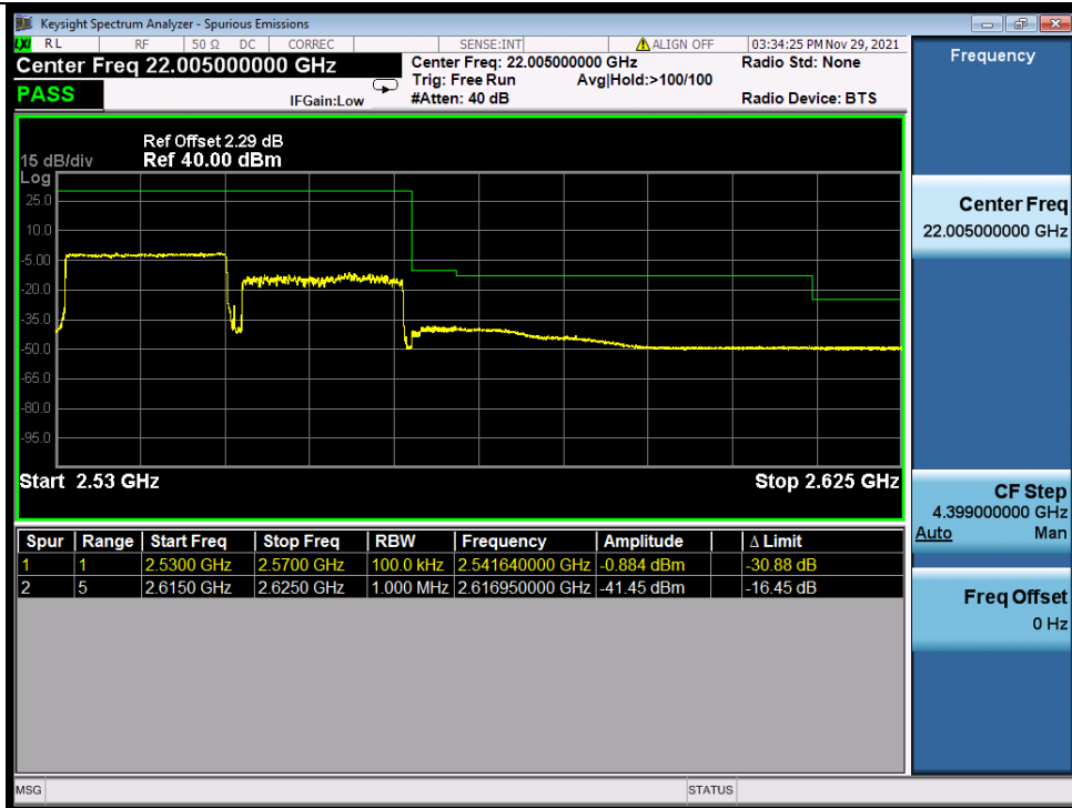
Band_7C_64QAM_LCH_20M+20M_RB_1_0/1_99_NTNV
