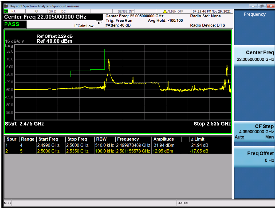
Band_7C_64QAM_LCH_15M+20M_RB_1_74/1_0_NTNV
