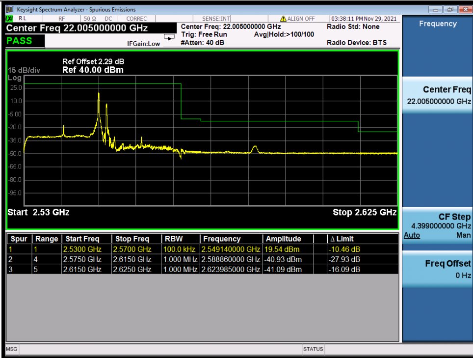
Band_7C_64QAM_HCH_20M+20M_RB_FULL_0_NTNV
