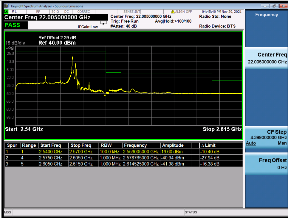
Band_7C_QPSK_HCH_20M+10M_RB_FULL_0_NTNV
