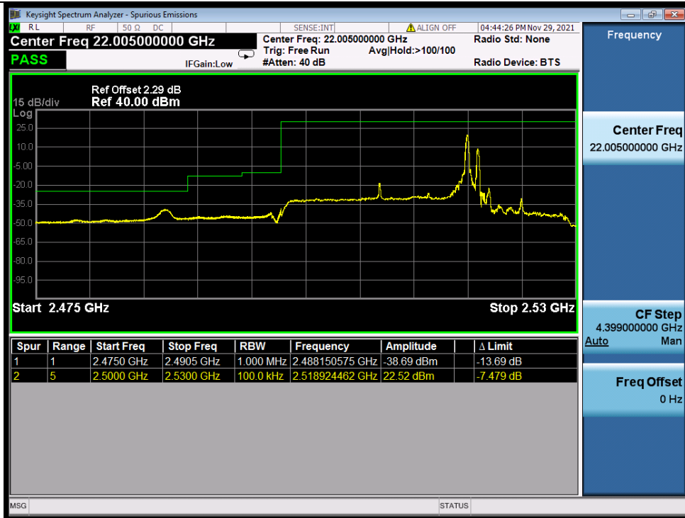
Band_7C_64QAM_LCH_20M+10M_RB_FULL_0_NTNV
