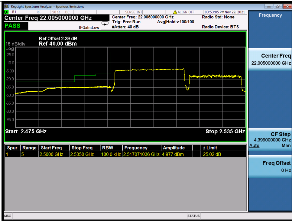
Band_7C_64QAM_HCH_20M+15M_RB_1_0/1_74_NTNV
