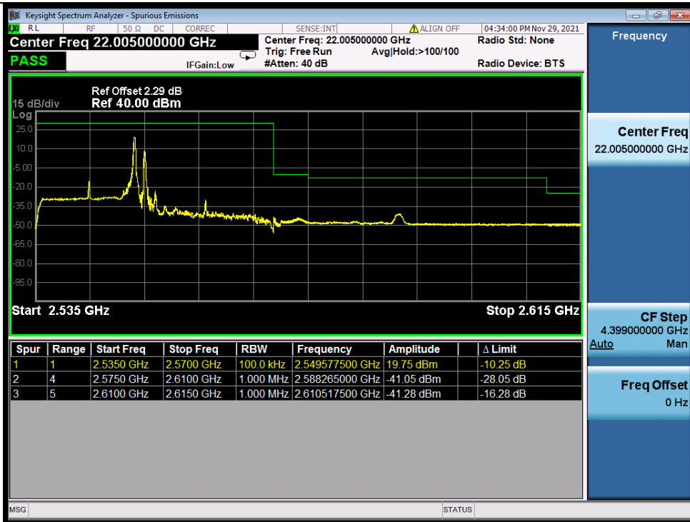
Band_7C_16QAM_HCH_15M+20M_RB_FULL_0_NTNV
