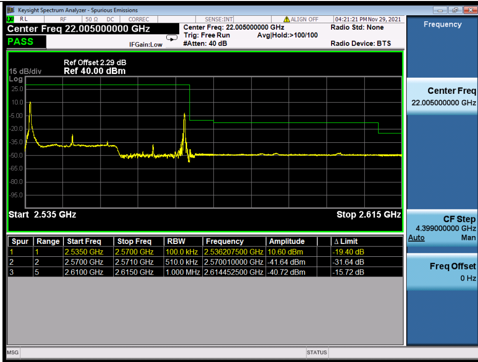
Band_7C_64QAM_HCH_20M+15M_RB_1_99/1_0_NTNV
