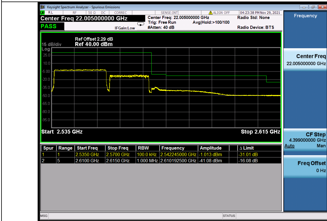
Band_7C_QPSK_HCH_20M+15M_NTNV
