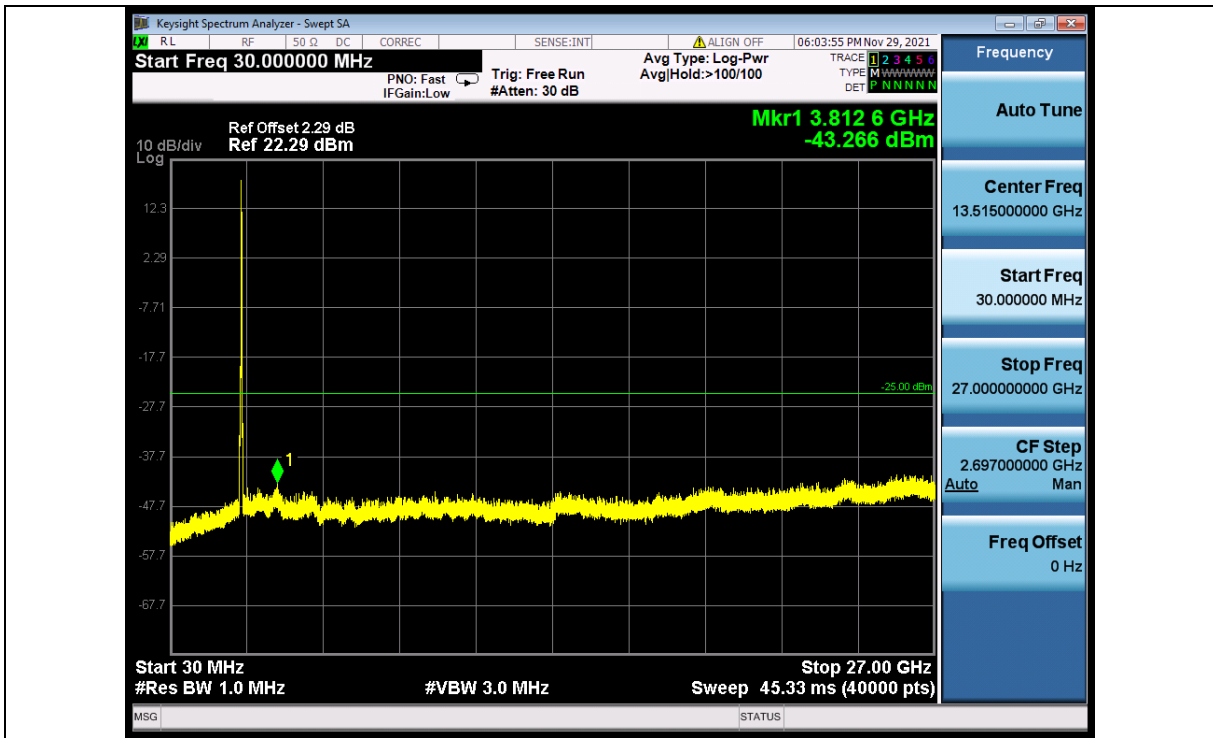
Band_7C_QPSK_HCH_15M+20M_RB_1_0/1_99_NTNV
