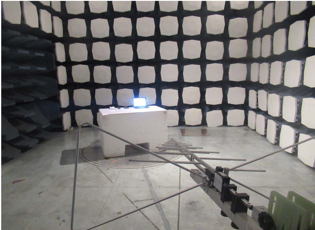
30MHz-1GHz
