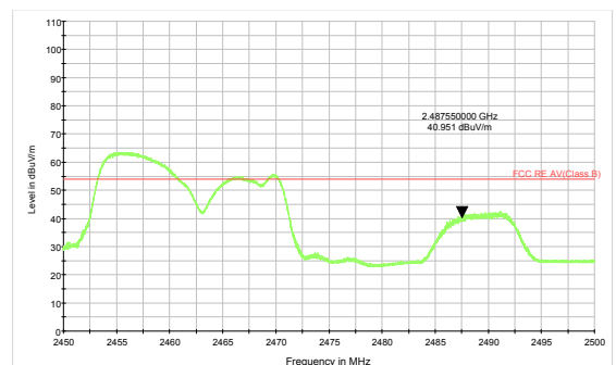
802.11g-Channel 11 Average
