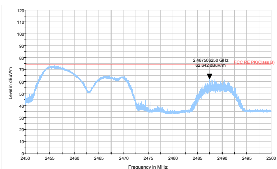
802.11g-Channel 11 Peak
