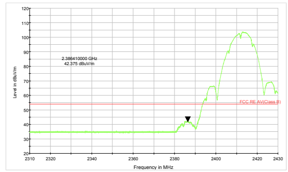
802.11b-Channel 1 Average
