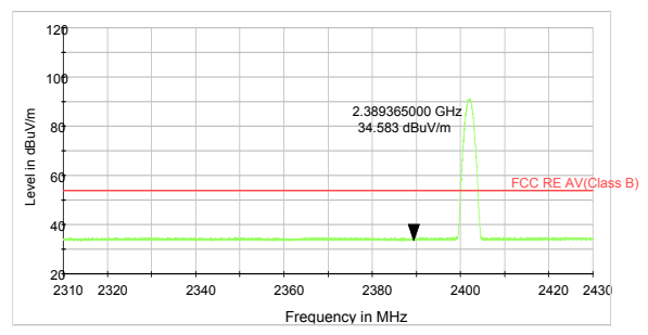
BLE (2M) Channel 0 Average
