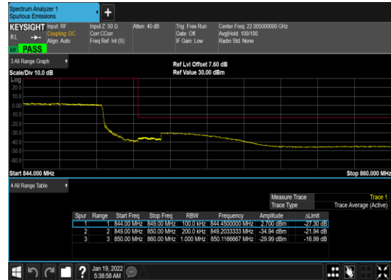
N5(20M)_DFT-s- OFDM_BPSK_Outer_Full_High_CH
