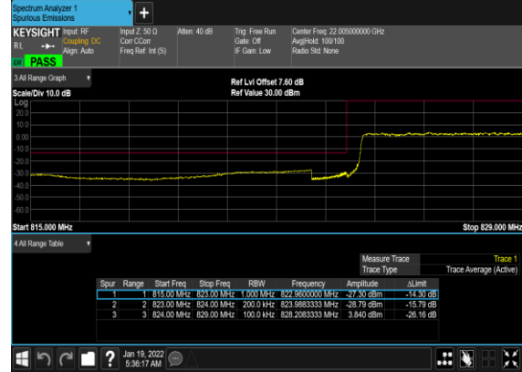
N5(20M)_DFT-s- OFDM_BPSK_Outer_Full_Low_CH
