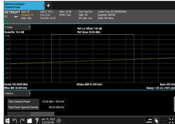
N5(20M)_DFT-s- OFDM_BPSK_Edge_1RB_Left_Low_CH_CHP_PA SS
