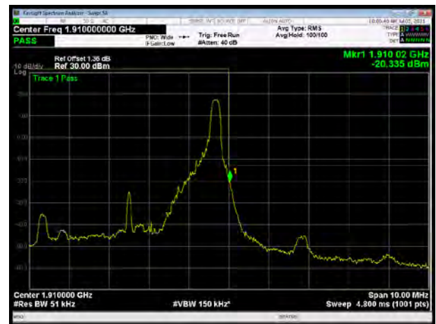
LTE Band 2 5MHz 64QAM 1RB CH-High
