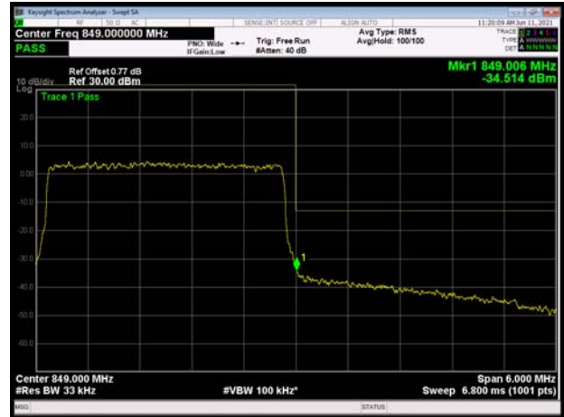
LTE Band 5 64QAM 5MHz CH-High 1RB
