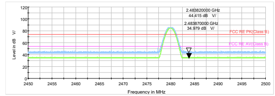
Bluetooth LE Channel 39 Peak & Average
