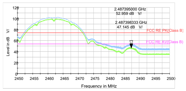
802.11b-Channel 11 Peak & Average
