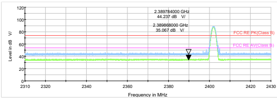
Bluetooth LE Channel 0 Peak & Average
