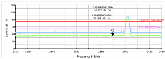
Bluetooth LE Channel 0 Peak &amp; Average
