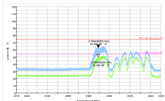
802.11n HT40 -Channel 3 Peak &amp; Average
