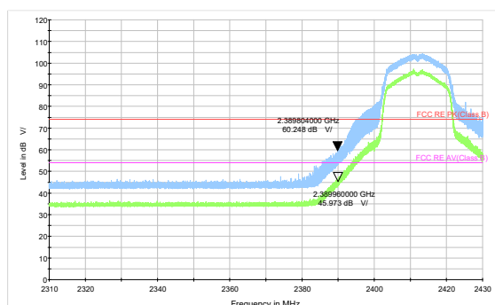
802.11n HT20 -Channel 1 Peak &amp; Average
