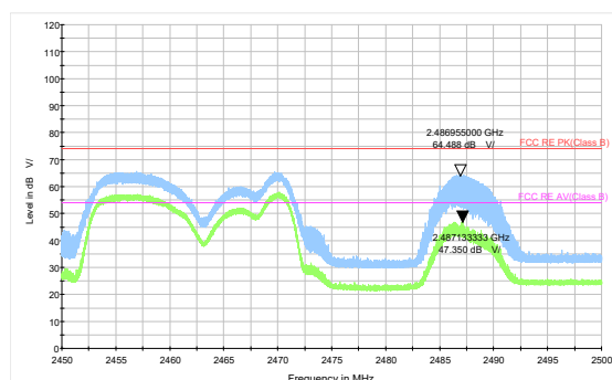
802.11n HT20 -Channel 11 Peak &amp; Average
