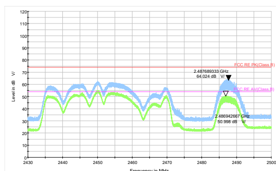
802.11n HT40 -Channel 9 Peak &amp; Average
