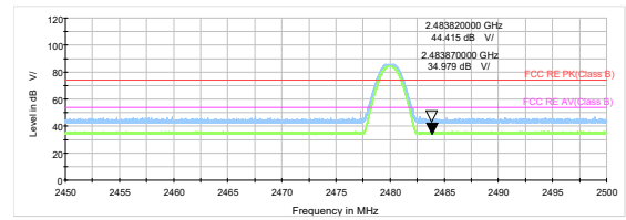
Bluetooth LE Channel 39 Peak &amp; Average
