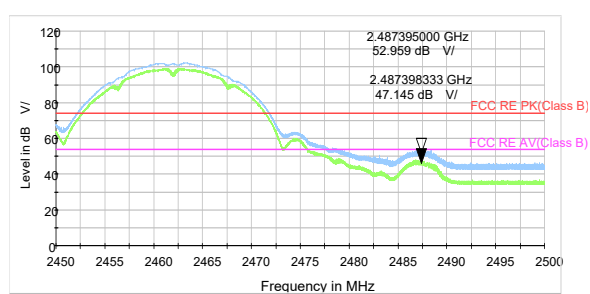
802.11b-Channel 11 Peak &amp; Average
