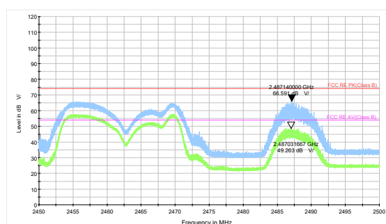
802.11g-Channel 11 Peak &amp; Average
