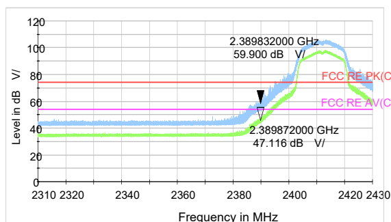
802.11g-Channel 1 Peak &amp; Average
