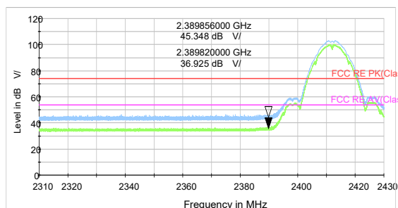
802.11b-Channel 1 Peak &amp; Average
