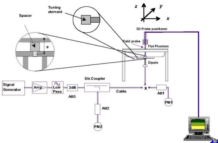
Fig 11.3.1 System Performance Check Setup
