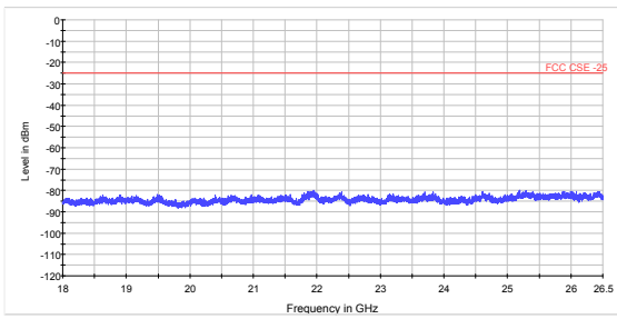
LTE Band 38 5MHz CH-Low 18GHz~26.5GHz
