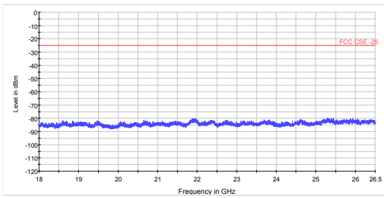
LTE Band 38 20MHz CH-Middle 18GHz~26.5GHz
