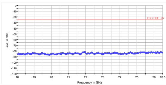
LTE Band 38 5MHz CH-High 18GHz~26.5GHz
