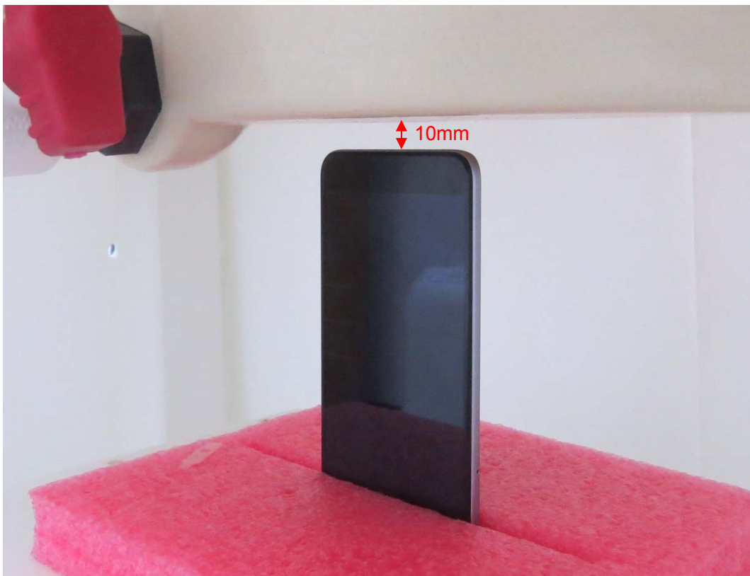
Picture 23: Bottom Side, the distance from handset to the bottom of the Phantom is 10mm
