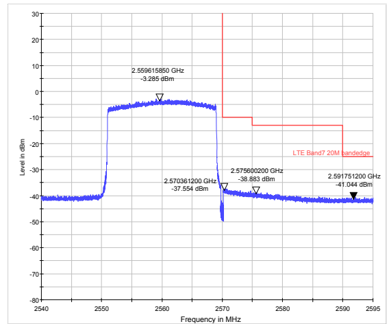
LTE Band 7 16QAM 20MHz CH-High, 100%RB
